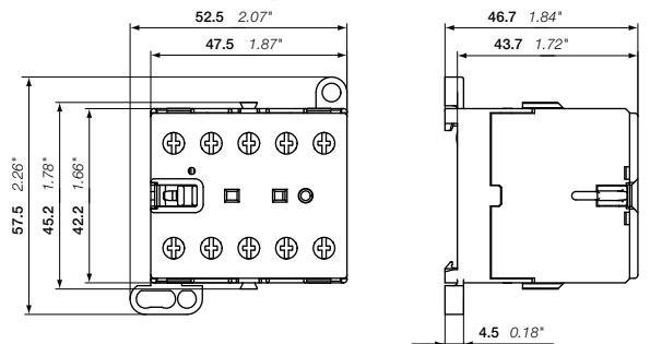
K6
