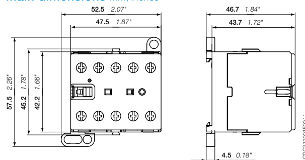
TKC6
