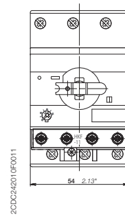
MS325 + HKF11
