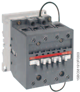
AE50-40-00
