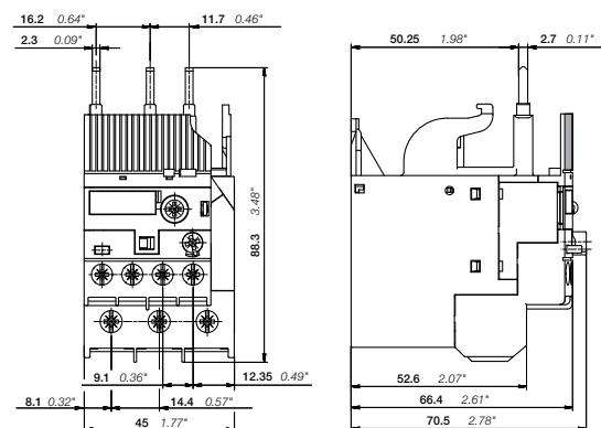
TF42
