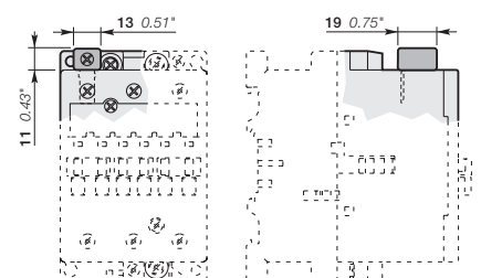
LK75-F
