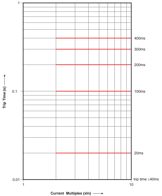
Short-Circuit I 2 t OFF (SR18G, SR18G/SR18Gi with display)
