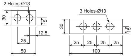
400 to 2000E, 800/1000/ 1250/1600C/H & 400/630/800/1000 /1250/1600S1 2000/2500C/H
