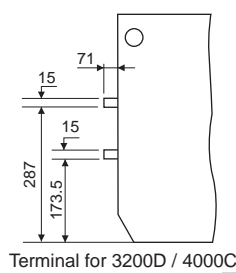
Terminal for 3200D / 4000C
