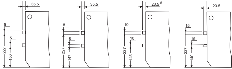
Terminal for 400/630 S1
