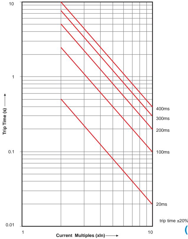
Short-Circuit I 2 t ON (SR18G, SR18G/SR18Gi with display)
