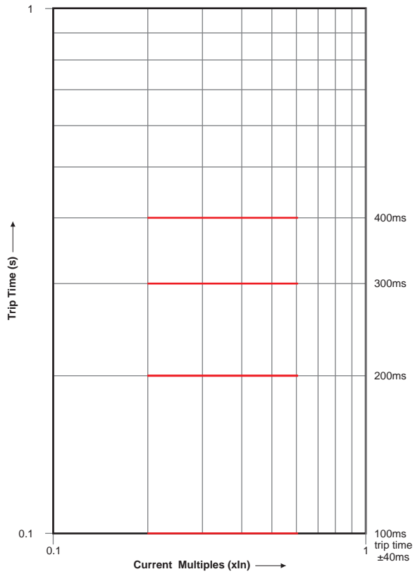
Earth Fault I 2 t OFF (SR18G, SR18G/SR18Gi with display)
