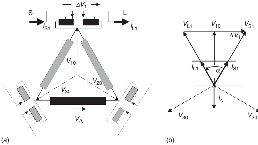
FIGURE 4.8 Single core symmetrical PST.
