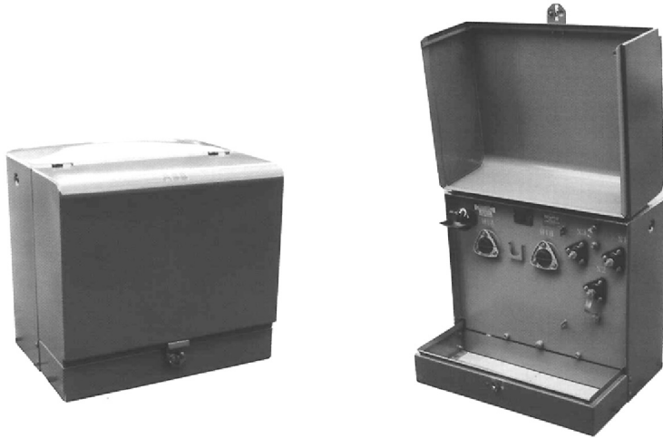
FIGURE 3.26 Typical Type 1 loop-feed system. (By permission of ABB Inc., Raleigh, NC.)
