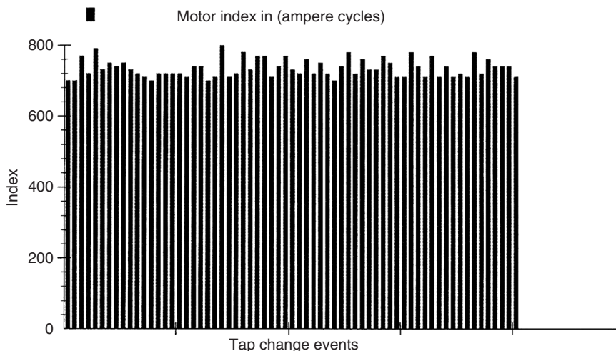
FIGURE 23.8 Sample motor-current-index curve.
