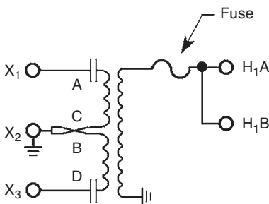
FIGURE 3.19 Two-primary bushing. (By permission of Pacific Gas and Electric Company, San Francisco, CA.)
