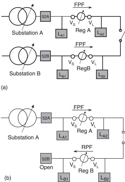
FIGURE 17.7 (a) Step-voltage regulator in routine application. (b) Step-voltage regulator in reverse power-flow application.
