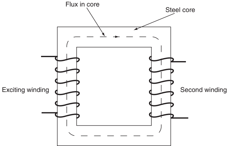
FIGURE 1.3 Two coils applied on a steel core.
