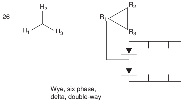
FIGURE 5.3 ANSI Circuit 26. (From ANSI/IEEE C57.18.10-1998. © IEEE 1998. With permission.)
