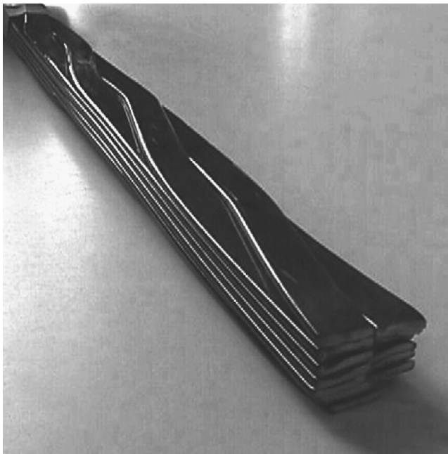
FIGURE 2.7 Continuously transposed cable (CTC).
