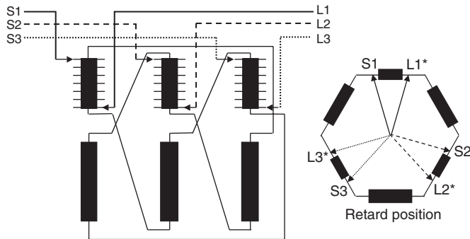
FIGURE 4.11 Delta-hexagonal PST.
