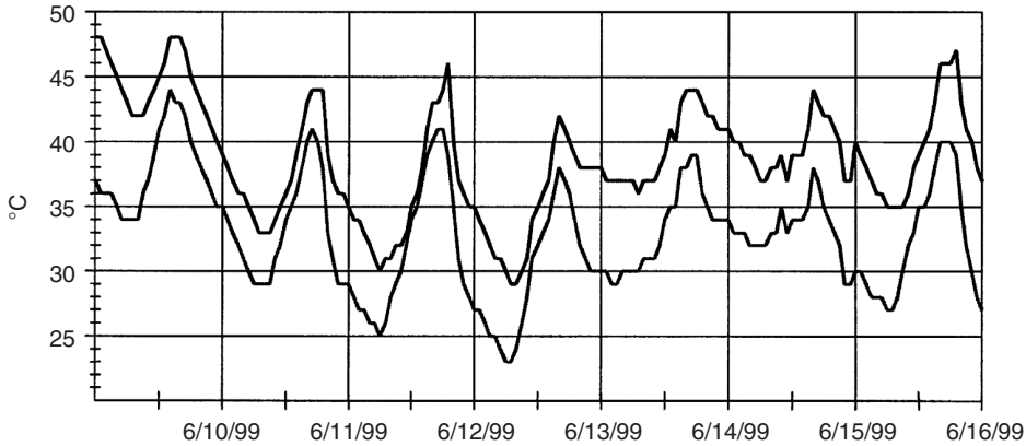
FIGURE 23.9 Sample differential-temperature measurement. The top trace is the main-tank top-oil temperature, and the bottom trace is the LTC compartment temperature.
