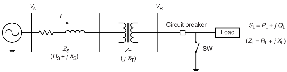
FIGURE 10.33 Radial system.
