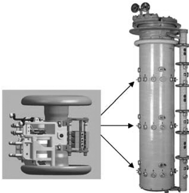
FIGURE 13.14 Resistor vacuum-type LTC for in-tank installations in oil-filled power transformers. (Photo courtesy of Maschinenfabrik Reinhausen GmbH.)
