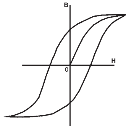
FIGURE 1.7 Hysteresis loop.
