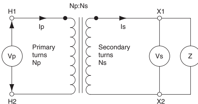
FIGURE 7.2 Ideal transformer.
