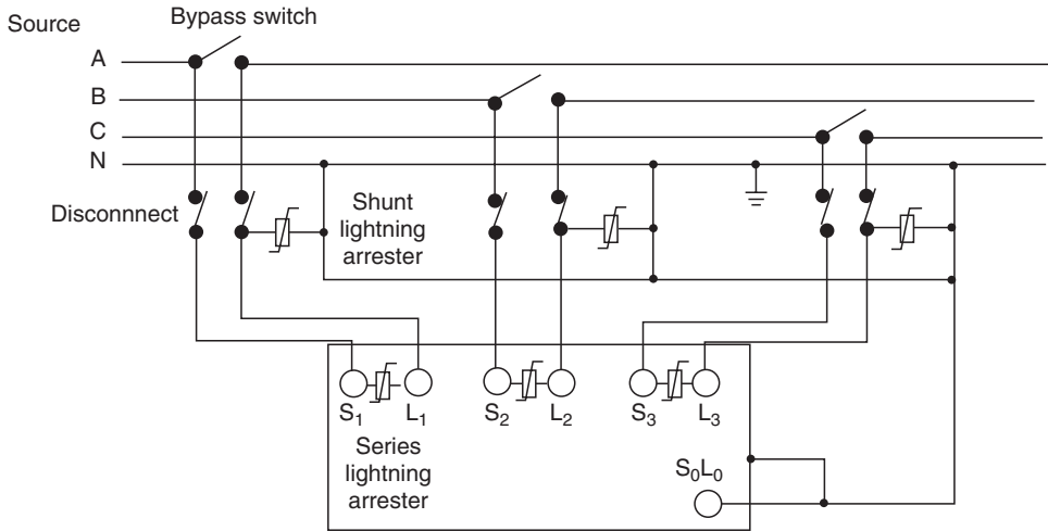
FIGURE 8.26 Connection of three-phase regulator regulating a three-phase, four-wire, multigrounded wye circuit.
