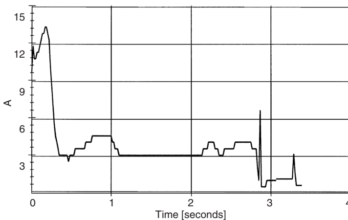
FIGURE 23.7 Load-tap-changer motor current during a tap-changing event.
