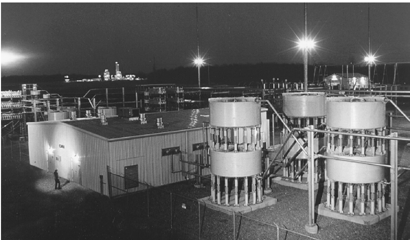
FIGURE 10.28 34 kV, 25 MVAR (per phase) thyristor controlled reactors.
