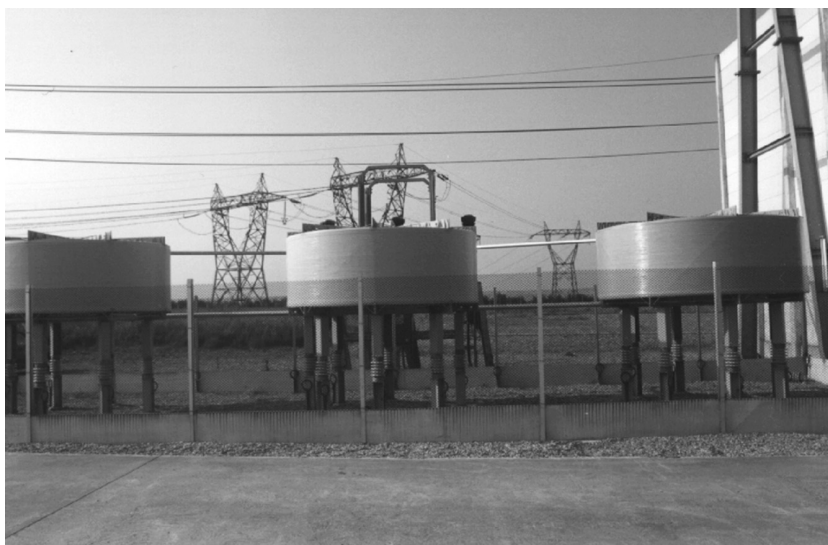
FIGURE 10.25 20 kV, 20 MVA (per phase) tertiary connection shunt reactors.
