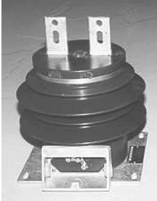
FIGURE 7.21 15-kV wound-type CT cast in epoxy resin. (Photo courtesy of Kuhlman Electric Corp.)
