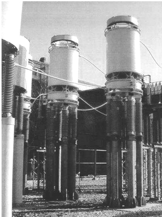
FIGURE 10.44 Tapped filter reactor with de-Q'ing rings.
