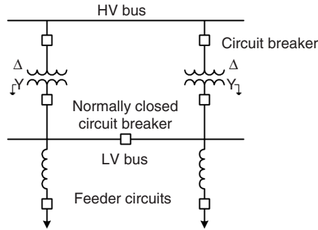
FIGURE 10.5 Typical phase reactor connection.
