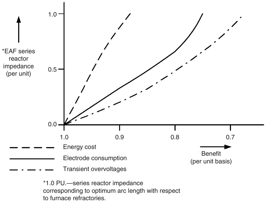
FIGURE 10.32 EAF series reactor benefits.
