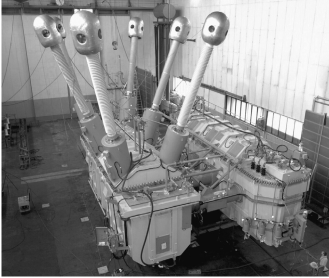
FIGURE 4.17 Two-tank PST at a test site (coolers not assembled) (650 MVA, 60 Hz, 525/525 \pm 20 \cdot 1.2^\circ kV). (By Courtesy of VAtech Transformatoren Weiz Austria (since 2005, Member of Siemens Group).)
