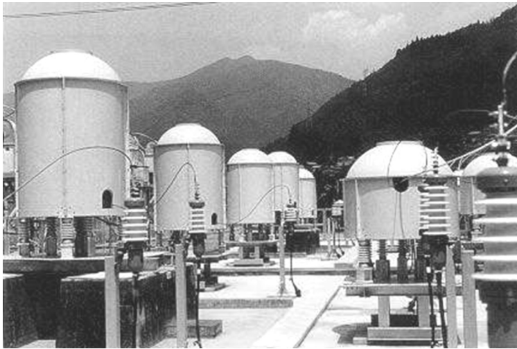
FIGURE 10.48 Installation of harmonic filter reactors for an HVDC project with a sound-shield enclosure.
