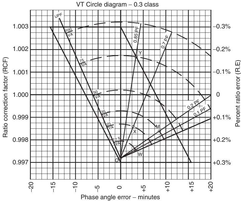
FIGURE 7.10 Voltage transformer circle diagram (fan curves).
