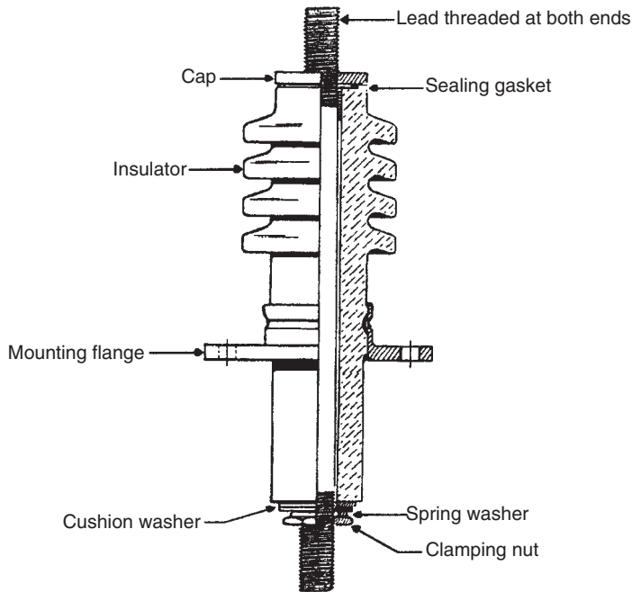
FIGURE 12.1 Solid-type bushing.
