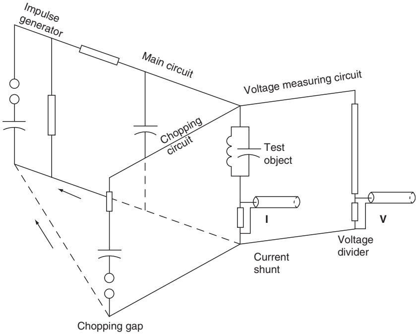
FIGURE 16.8 Impulse-test setup.
