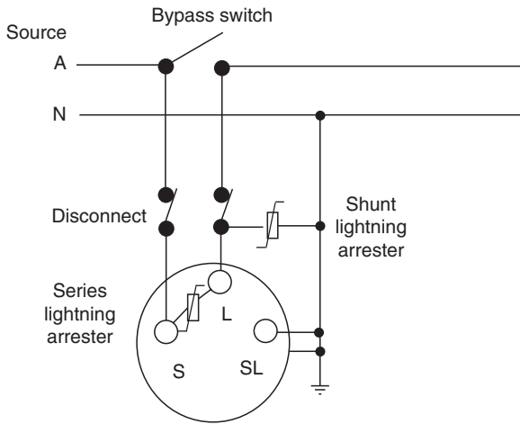
FIGURE 8.3 Voltage regulator connection in a single-phase circuit.
