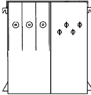
FIGURE 3.29 Radial-style live front. (By permission of Pacific Gas and Electric Company, San Francisco, CA.)
