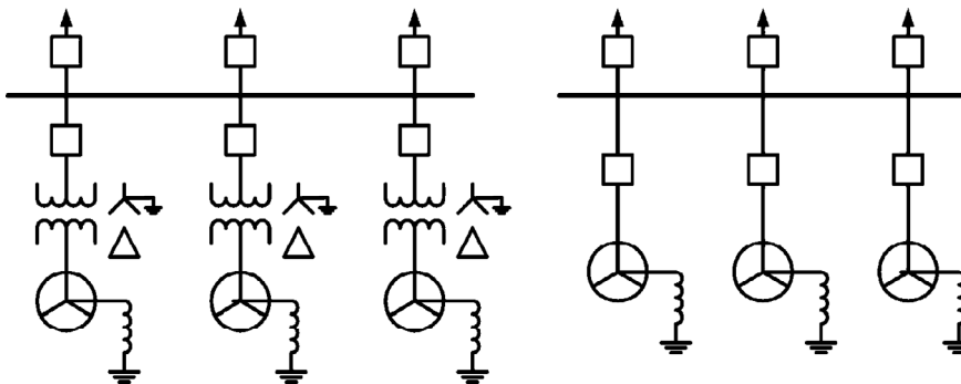
FIGURE 10.10 Two generator arrangements where a reactor can be used as a neutral grounding device; unit system (left) and three-wire system (right).
