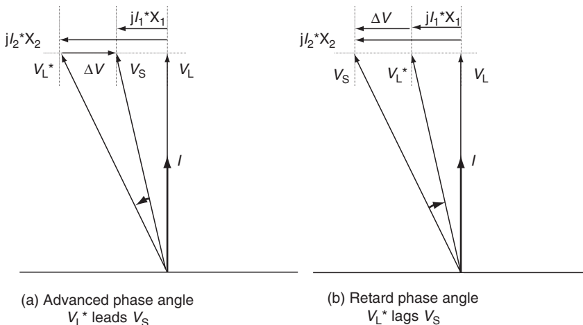
FIGURE 4.3 No-load voltage diagram of parallel systems.
