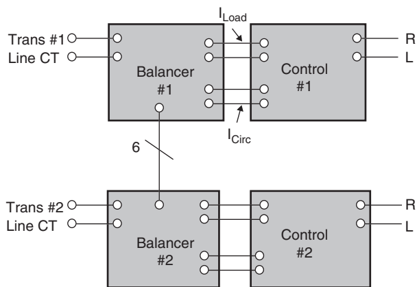
FIGURE 17.9 Control block diagram, paralleling by usual circulating-current method.
