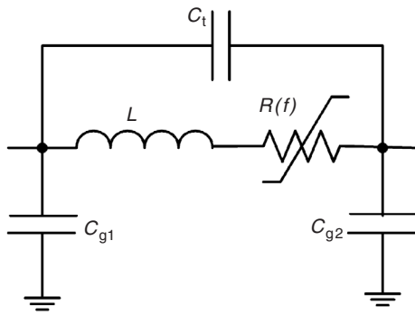
FIGURE 10.41 Reactor model for TRV studies where C_{g1} and C_{g2} are the stray capacitance of reactor terminals to ground. C_t , terminal to terminal stray capacitance; L , reactor inductance; R(f) , reactor frequency dependent resistance.
