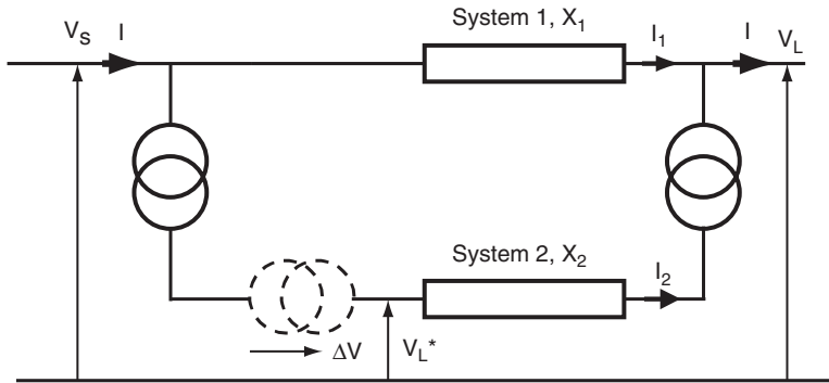
FIGURE 4.2 Parallel systems.
