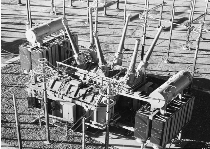
FIGURE 4.20 Two-tank PST with three coarse- and one fine-tap winding at field site (650 MVA, 60 Hz, 525/525 ± 12*1.2° kV). (By Courtesy of VATEch Transformatoren Weiz Austria (since 2005, Member of Siemens Group).)
