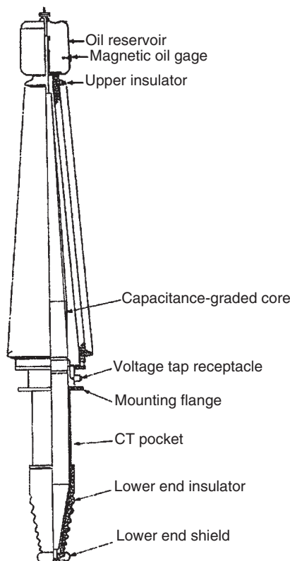
FIGURE 12.2 Oil-filled, capacitance-graded bushing.
