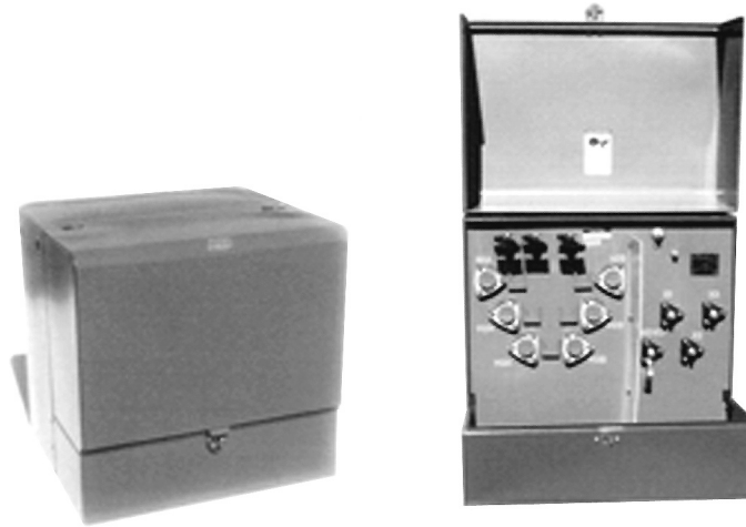
FIGURE 3.34 Mini three-phase in clamshell cabinet. (By permission of ABB Inc., Raleigh, NC.)
