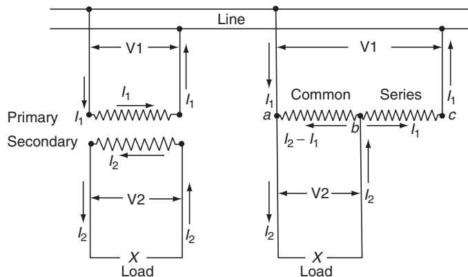
FIGURE 15.3 Current flow in double-wound transformer and autotransformer.
