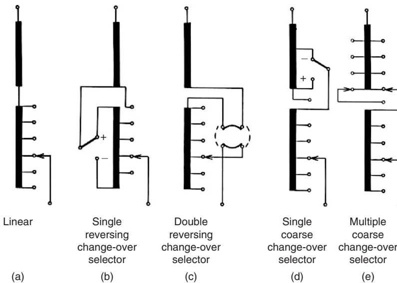
FIGURE 13.20 Basic arrangements of tap windings.
