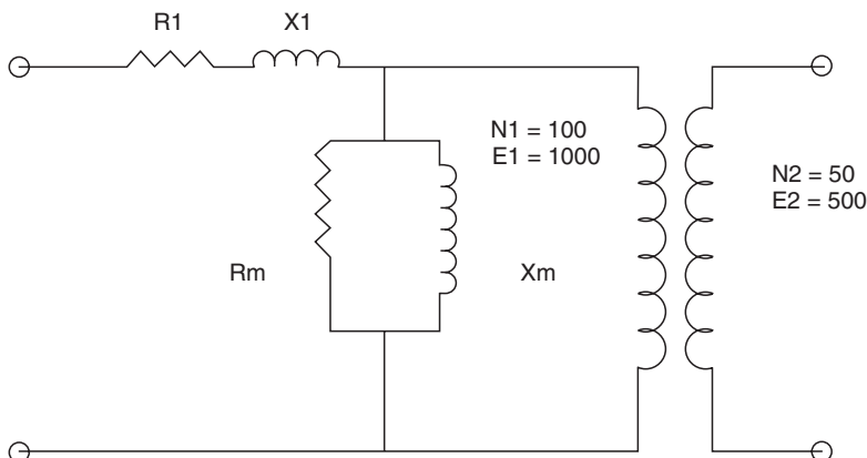
FIGURE 1.5 Equivalent circuit.
