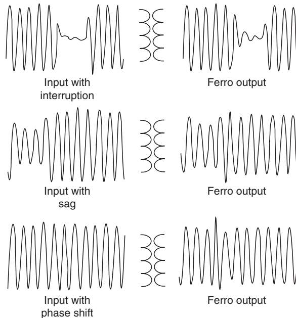
FIGURE 9.13 Output voltages (labeled ferro-output) resulting from voltage interruption, sag, and phase shift on the input.
