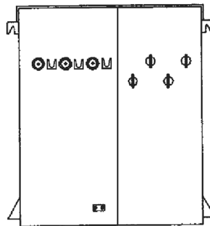
FIGURE 3.31 Radial-style dead front. (By permission of Pacific Gas and Electric Company, San Francisco, CA.)
