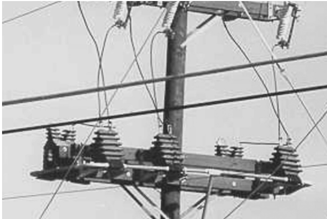
FIGURE 7.29 15-kV three-phase/four-wire metering rack with 3 VT and 3 CT. (Photo courtesy of Kuhlman Electric Corp.)
