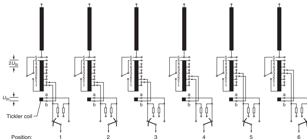
FIGURE 13.21 LTC for tap windings with tickler coil.
