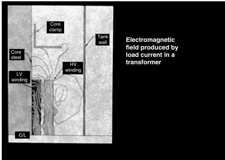
FIGURE 5.15 Transformer construction and electromagnetic leakage field.
