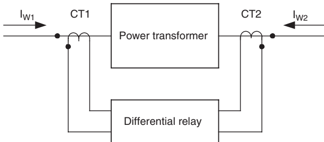
FIGURE 18.1 Typical differential-relay connection diagram.
