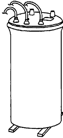
FIGURE 3.18 Single-phase round. (By permission of Pacific Gas and Electric Company, San Francisco, CA.)
