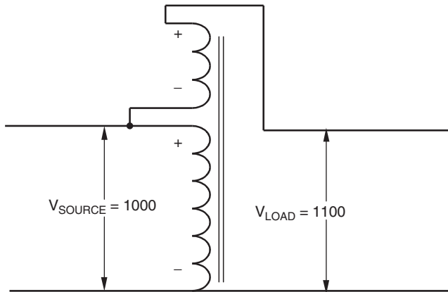
FIGURE 8.13 Step-up autotransformer.
