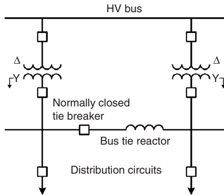
FIGURE 10.7 Typical bus tie reactor connection.
