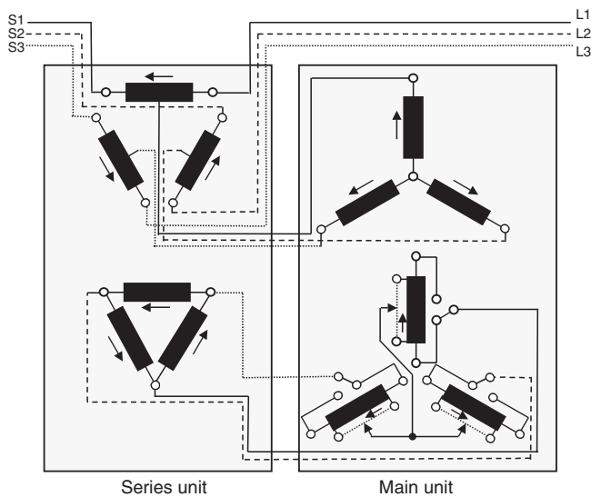
FIGURE 4.11 Delta-hexagonal PST.
