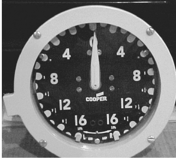
FIGURE 8.15 Tap-changer position indicator.
