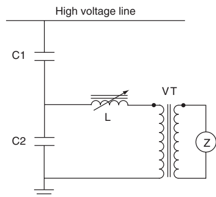
FIGURE 7.13 CCVT simplified circuit.
