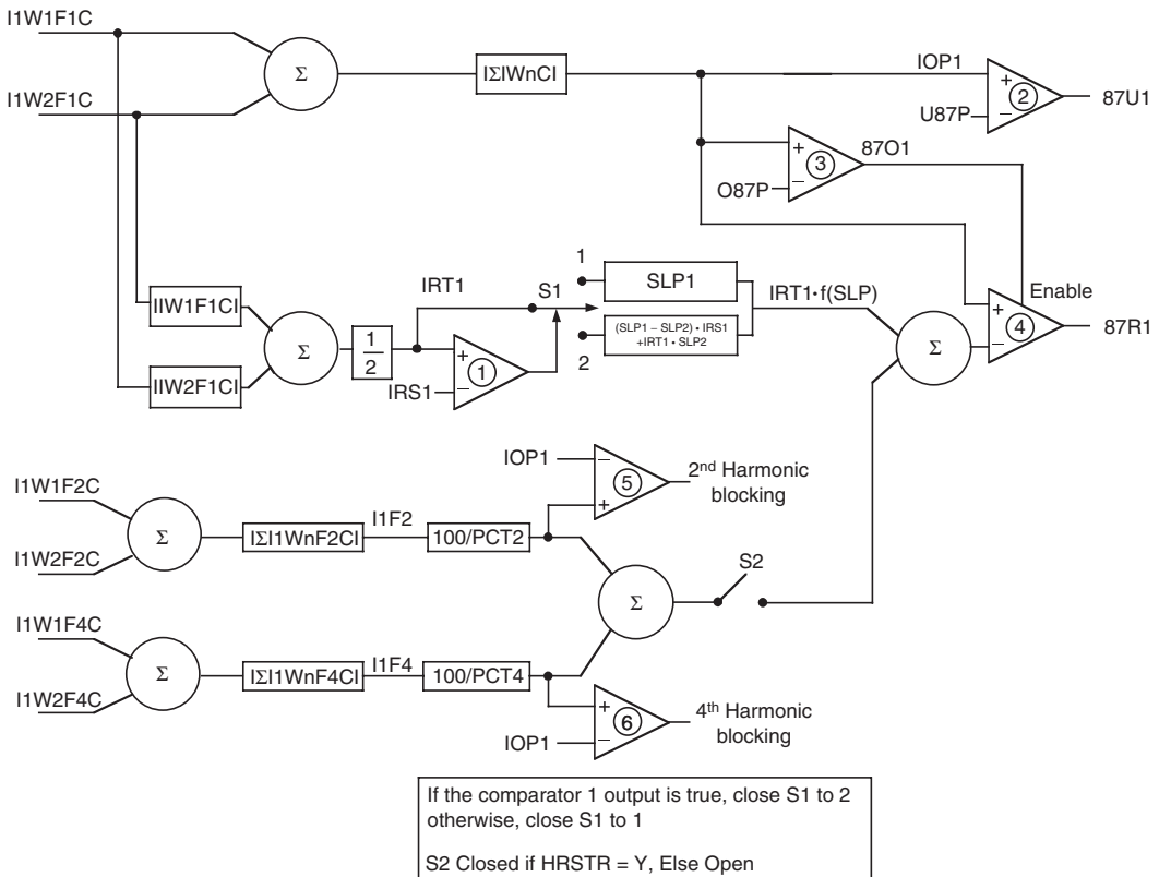
FIGURE 18.13 Even-harmonic restraint, 87R1, and unrestraint, 87U1, differential elements.
