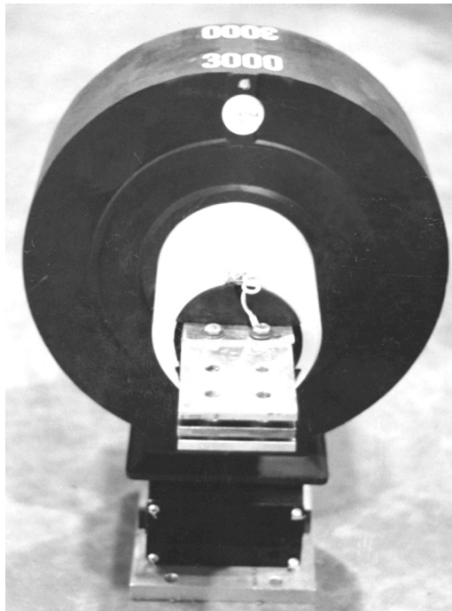
FIGURE 7.18 Bar-type CT. (Photo courtesy of Kuhlman Electric Corp.)
