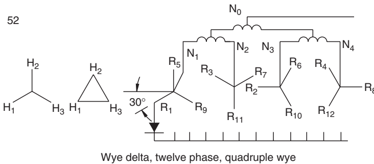
FIGURE 5.11 ANSI Circuit 52. (From ANSI/IEEE C57.18.10–1998. © IEEE 1998. With permission.)
