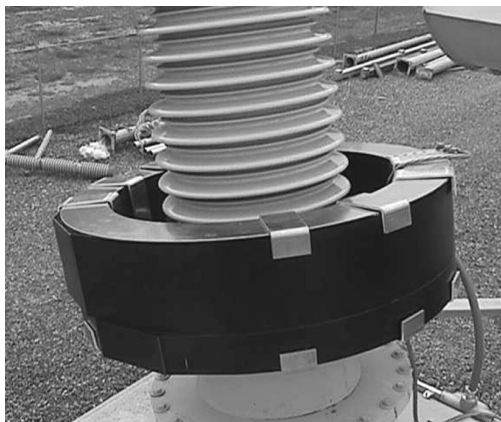
FIGURE 7.27 600-V-class slipover CT installed on high-voltage bushing with ground shield. Note the ground lead going back through the CT window to avoid shorted electrical turn. (Photo courtesy of Kuhlman Electric Corp.)
