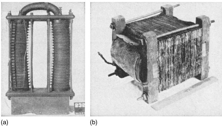
FIGURE 3.1 (a) Gaulard and Gibbs transformer; (b) William Stanley’s early transformer. (By permission of ABB Inc., Raleigh, NC.)
