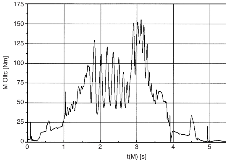
FIGURE 23.6 Sample torque curve.
