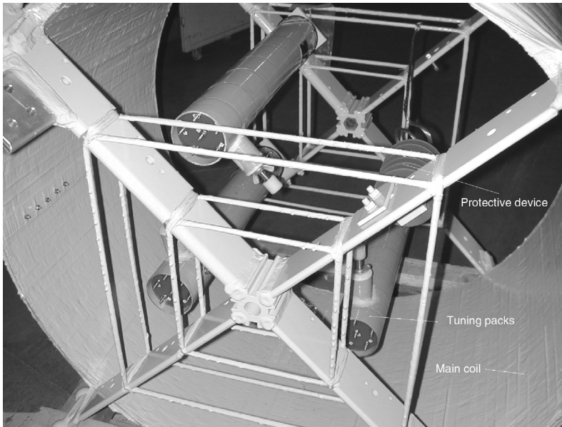
FIGURE 10.52 Internal view of line trap showing tuning device and protective device.
