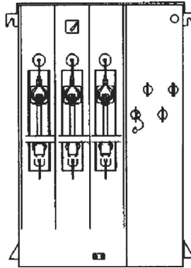
FIGURE 3.30 Loop-style live front. (By permission of Pacific Gas and Electric Company, San Francisco, CA.)
