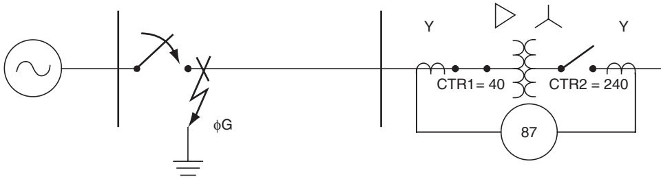
FIGURE 18.18 Transformer energization while A-phase is faulted.
