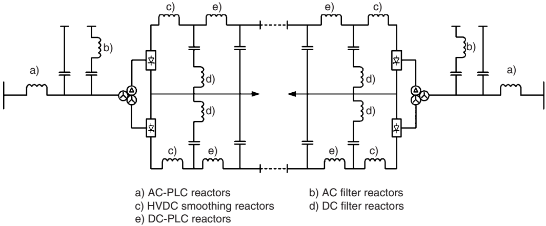
FIGURE 10.30 One line diagram of a typical HVDC bipole link illustrating reactor applications.
