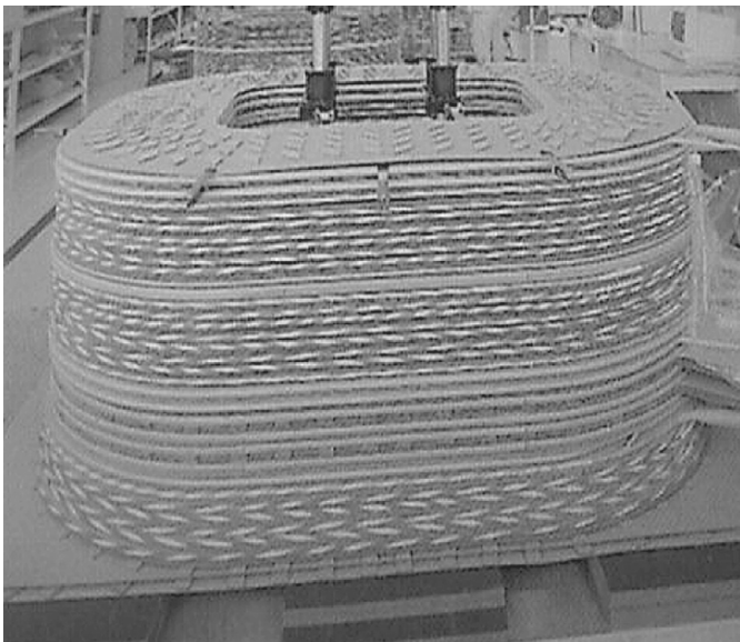
FIGURE 2.13 Stacked pancake windings.
