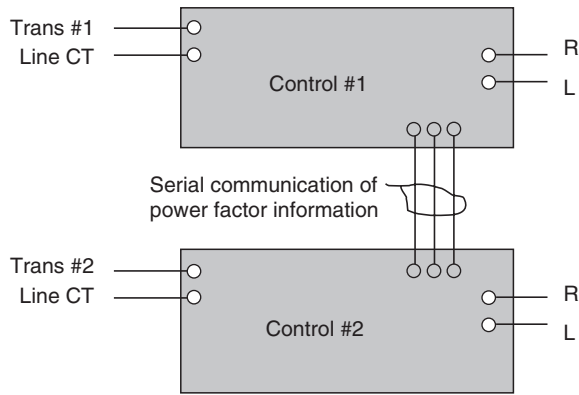
FIGURE 17.10 Control block diagram, paralleling by equal power factor, circulating-current method.
