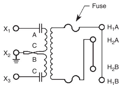
FIGURE 3.20 Four-primary bushing. (By permission of Pacific Gas and Electric Company, San Francisco, CA.)
