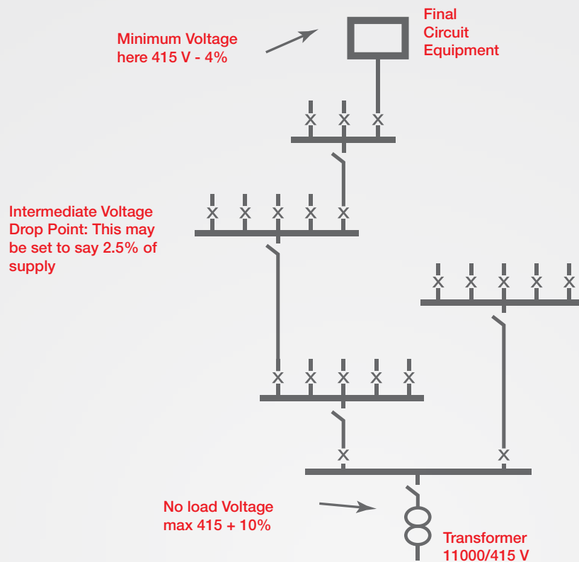
Figure 6.4: Voltage Drop
