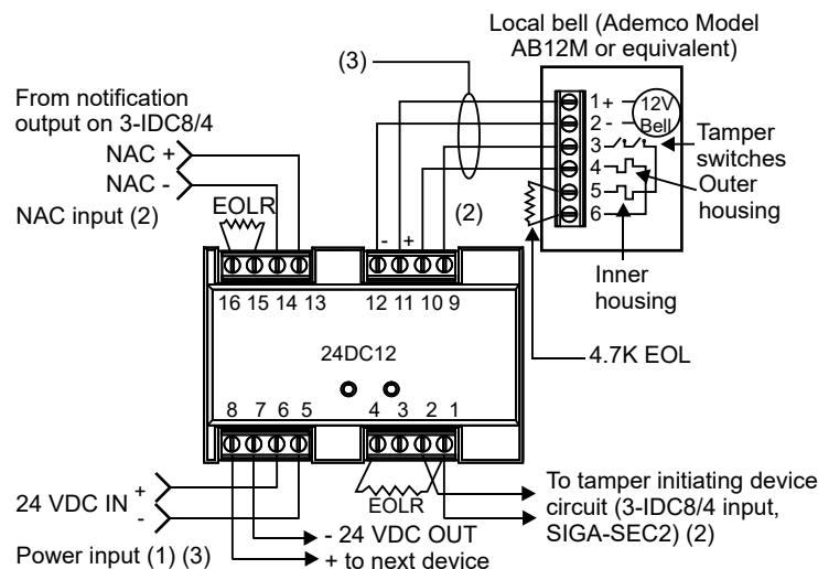
Figure 25: Connection to local bell
