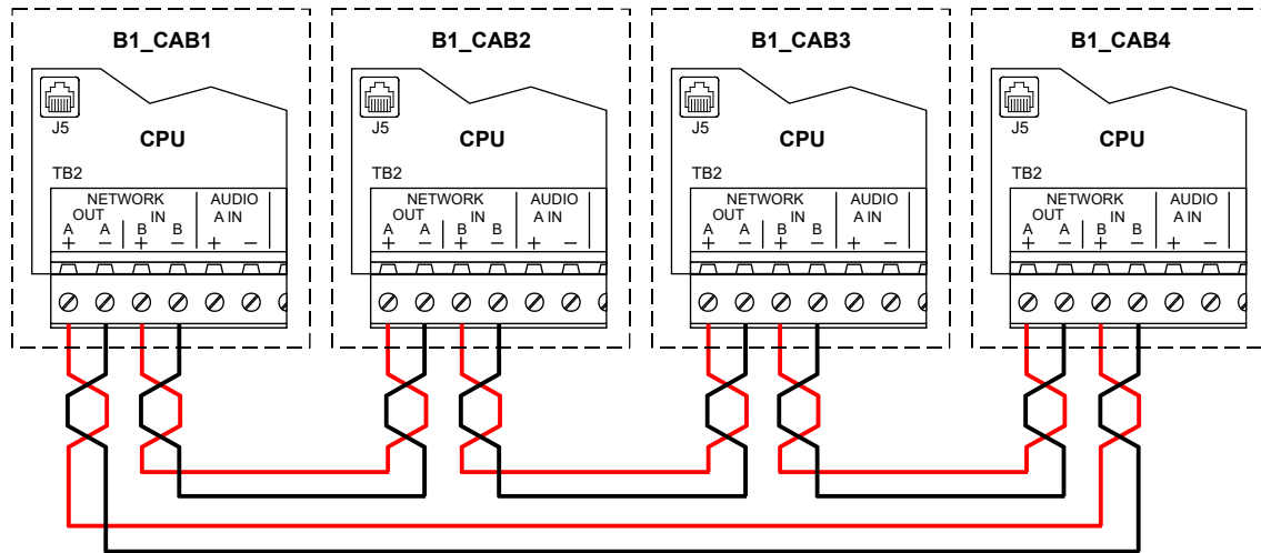
Figure 11: Typical Class A and Class X network data riser wiring using copper wire
