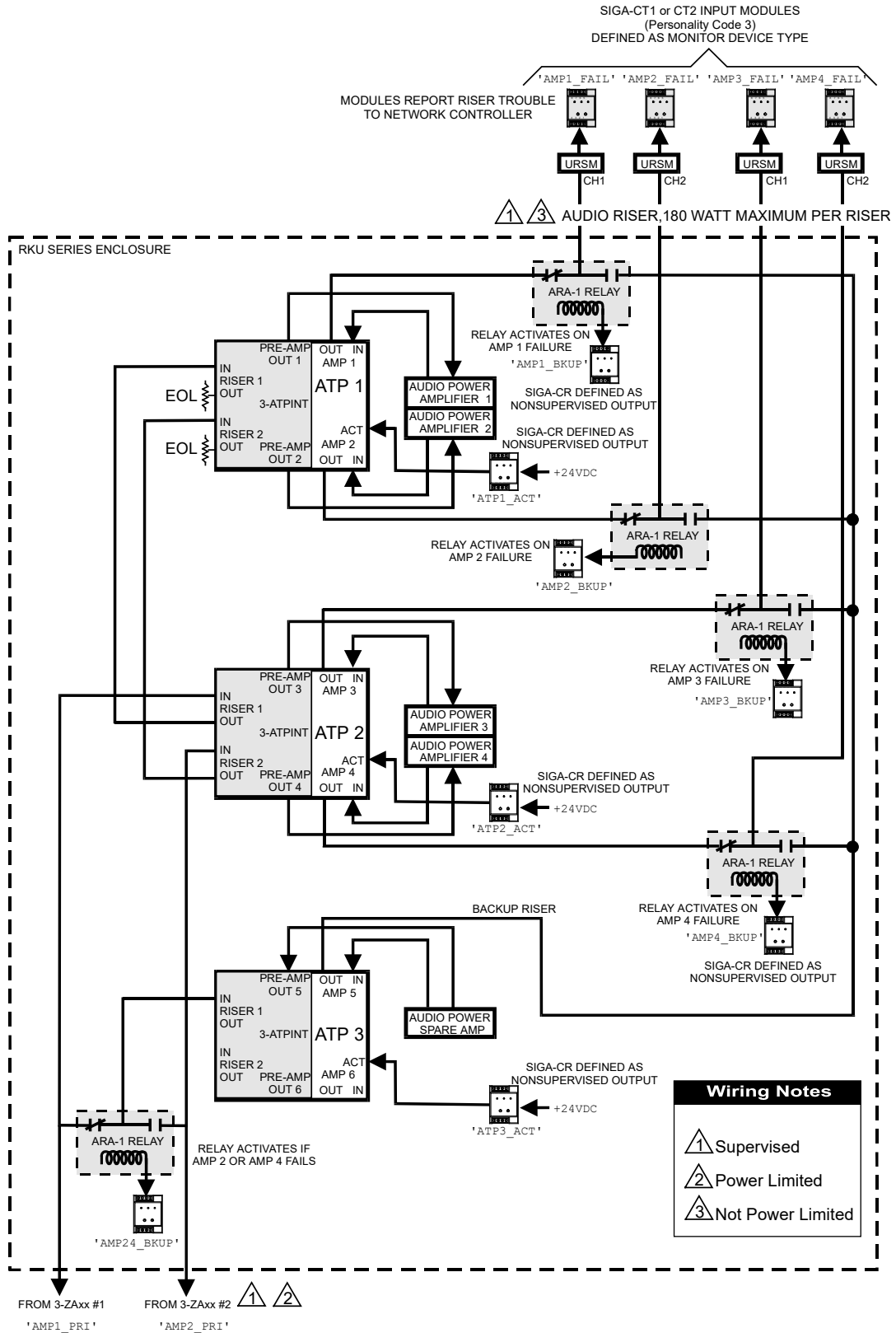
Figure 61: One spare amplifier in dual channel system
