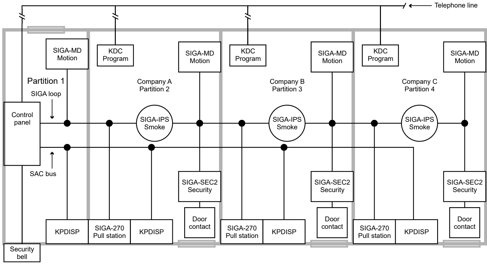
Figure 27: Multiple tenant security in a strip mall
