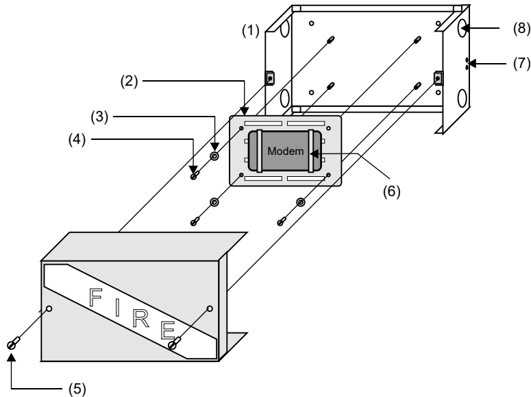
Figure 78: Suggested modem installation using an MFCA and SIGA-MP1
