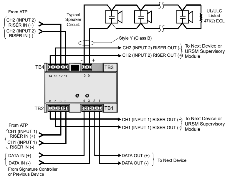
Figure 63: Two channel Class B wiring, SIGA-CC2 module
