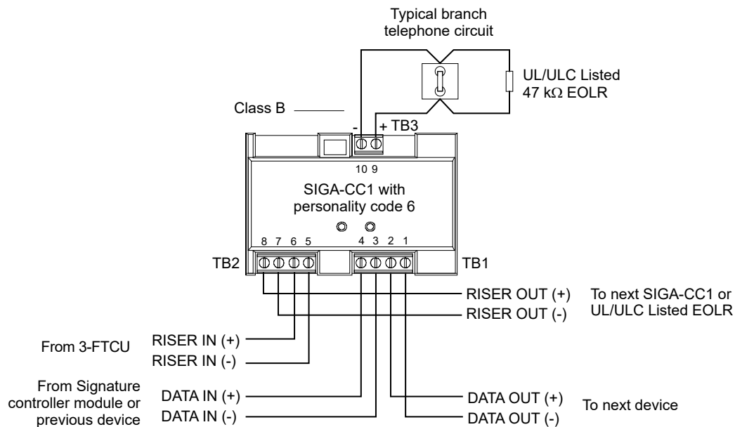
Figure 19: SIGA-CC1 with one phone installed
