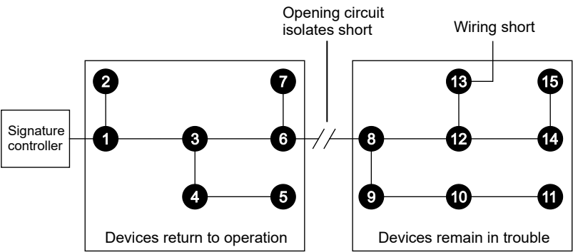
Figure 89: Isolating circuit short
