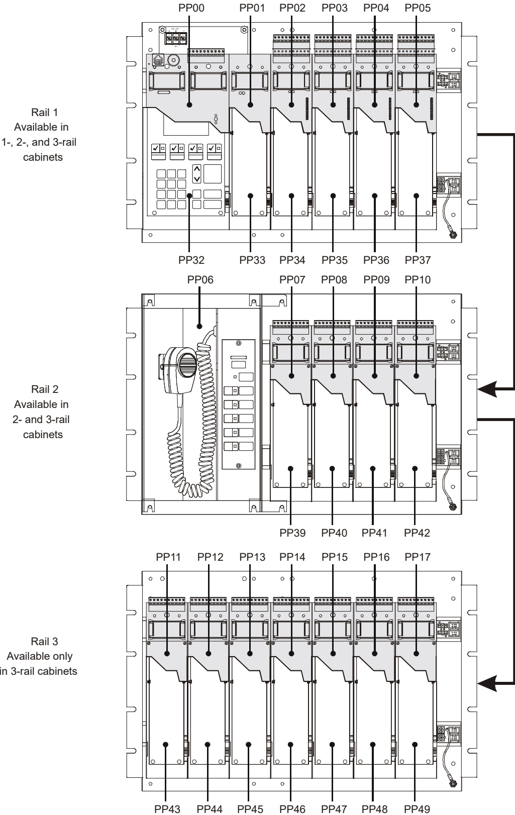
Figure 105: LRM addresses for 3-CHAS7, 3-ASU/CHAS4 (3-ASUMCC(-4MCC)), 3-CHAS7 configuration
