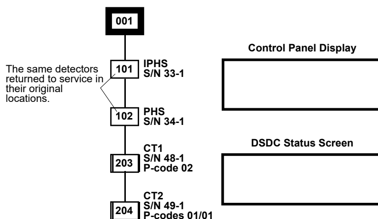
Figure 93: Detectors returned to service in original locations
