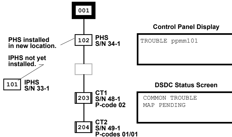
Figure 94: Partially restored circuit
