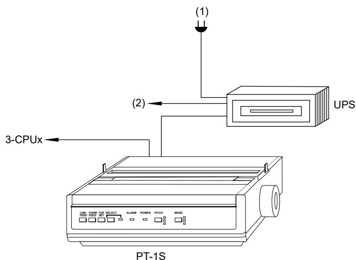
Figure 76: Printer uninterruptible power supply wiring
