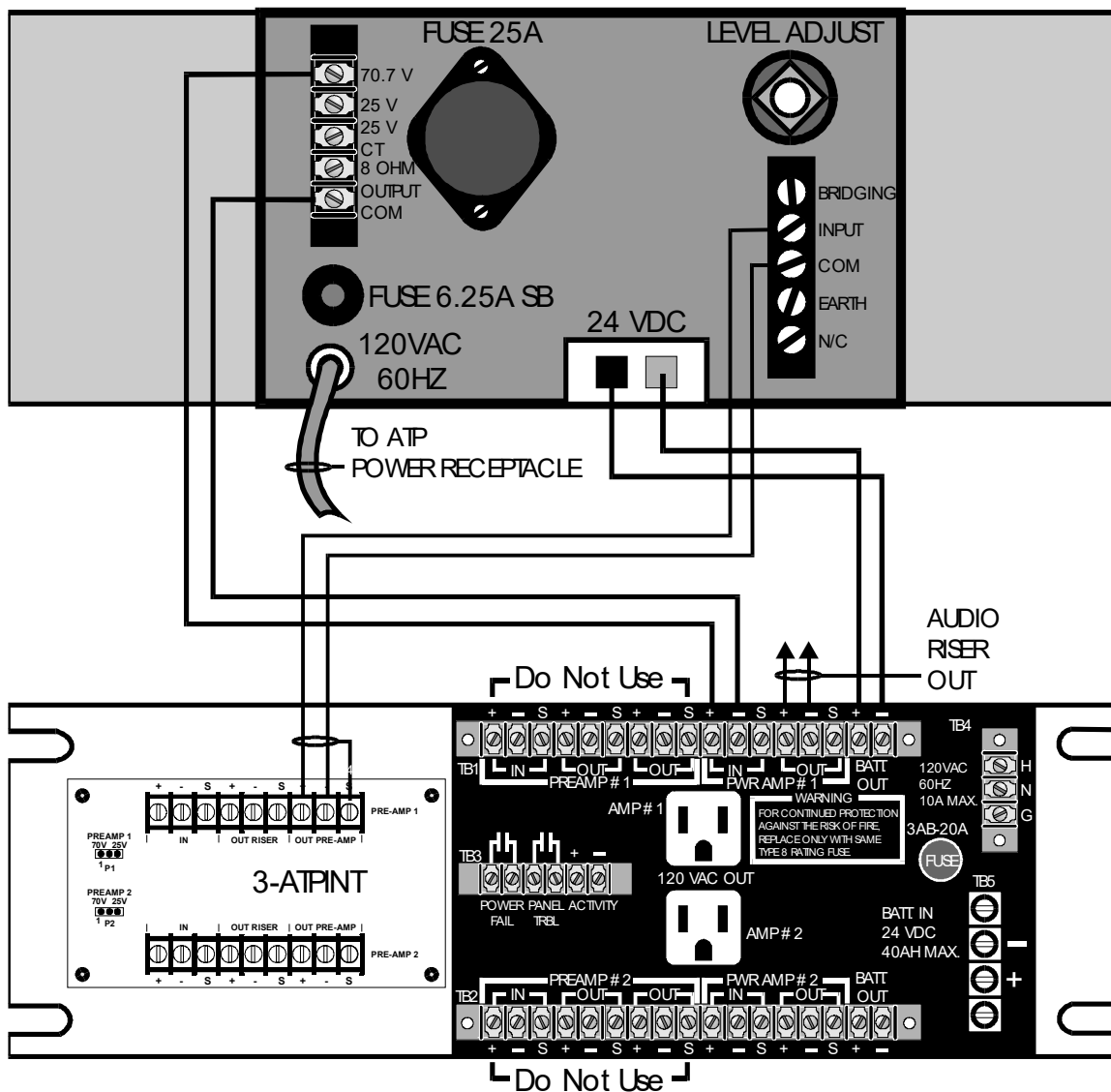
Figure 56: Wiring from Dukane amplifier to ATP
