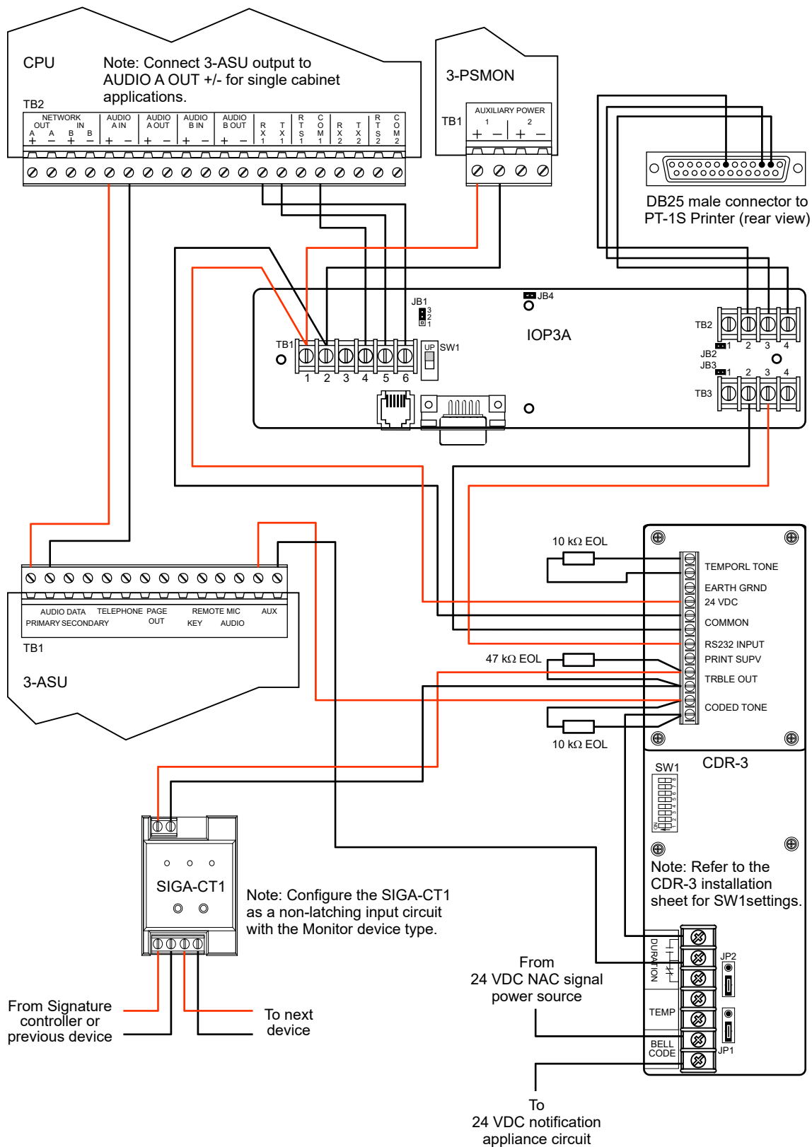
Figure 77: Application wiring diagram
