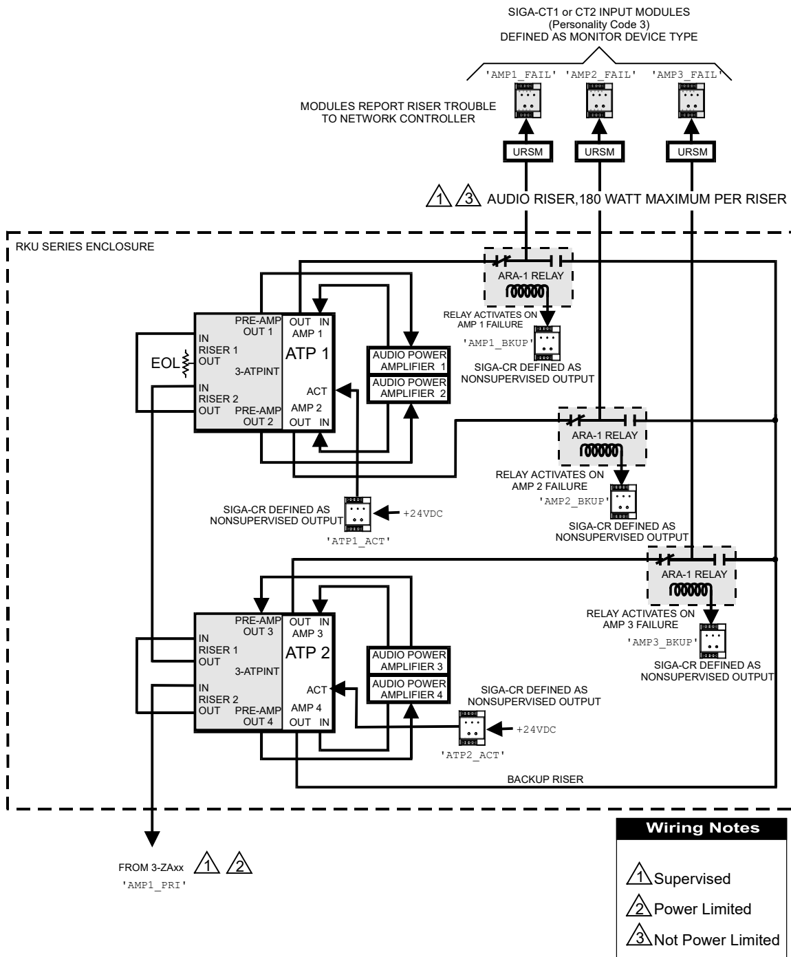
Figure 60: Amplifier bank with spare amplifier
