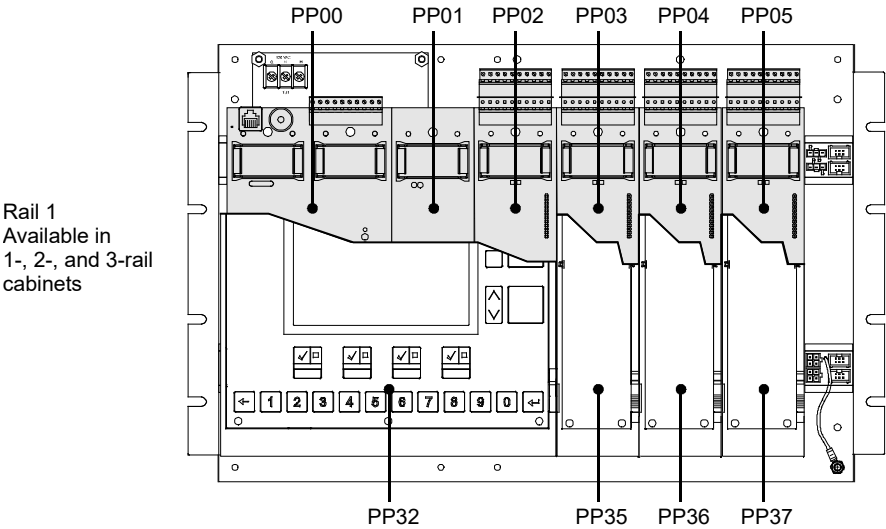
Figure 107: LRM addresses when using a 3-LCDXL1 Main LCD Display
