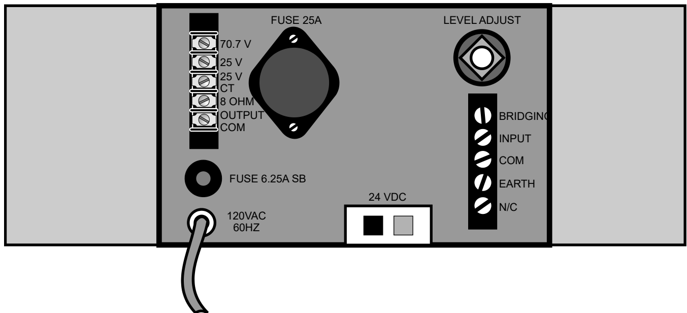
Figure 58: Dukane amplifier, rear view
