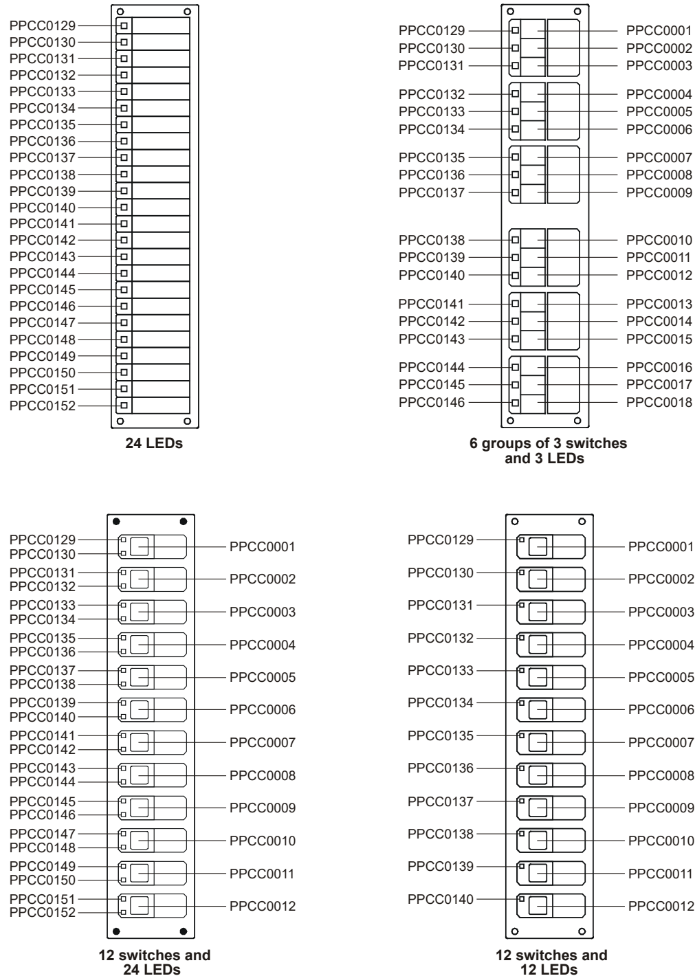
Figure 108: Control-display module switch and LED device addresses
