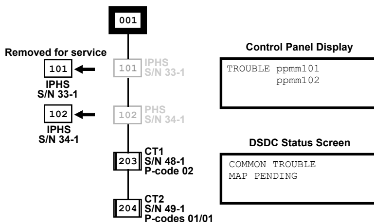
Figure 92: Detectors removed for service
