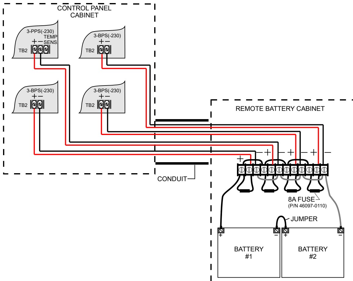
Figure 72: Remote battery cabinet wiring
