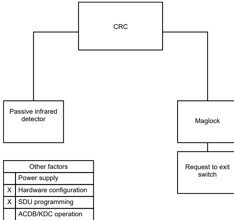
Figure 36: Maglock and peripherals
