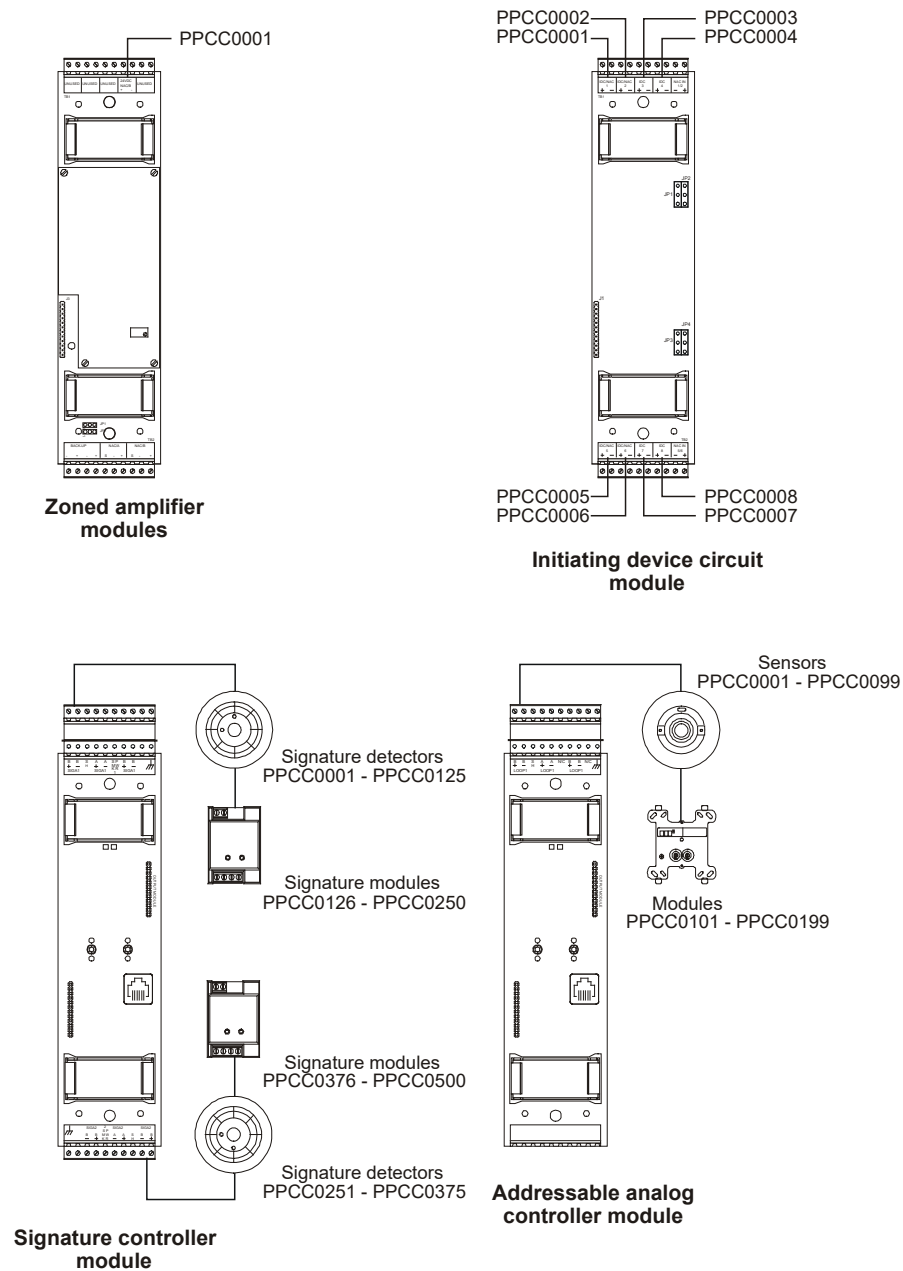
Figure 109: Rail module device addresses
