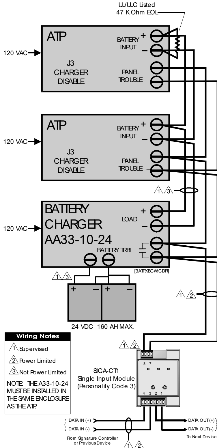
Figure 59: ATP external battery charger wiring
