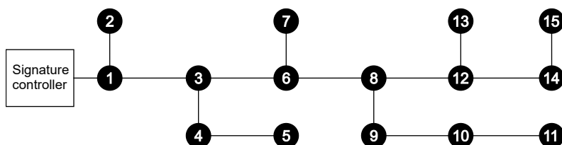
Figure 86: Normal circuit topology
