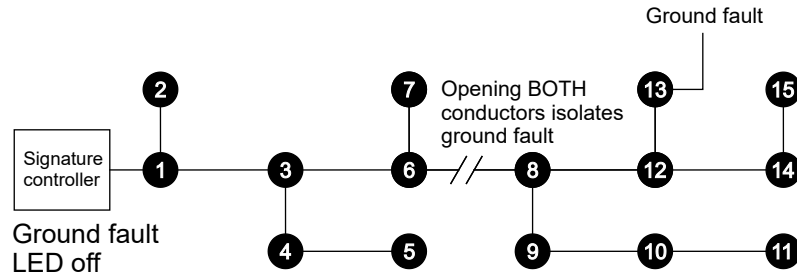
Figure 91: Ground fault isolation
