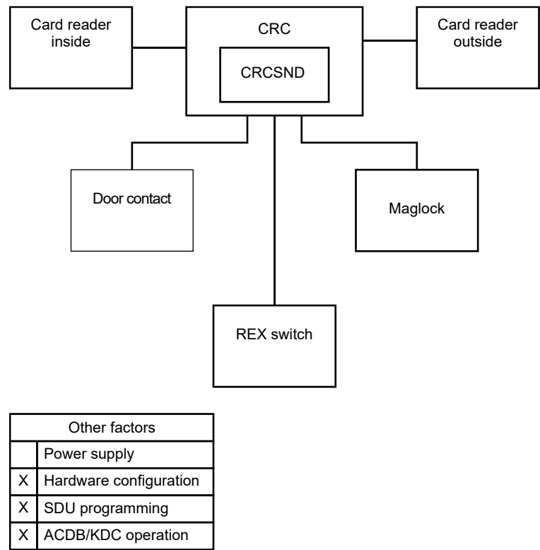
Figure 32: Delayed egress doorway
