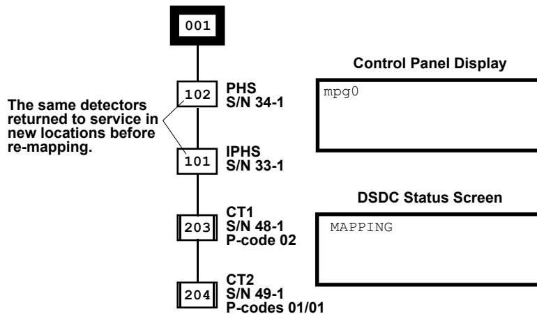
Figure 95: Detectors returned to new locations during re-mapping
