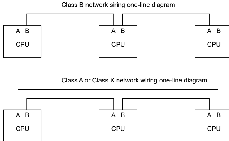
Figure 83: Network wiring one-line diagrams
