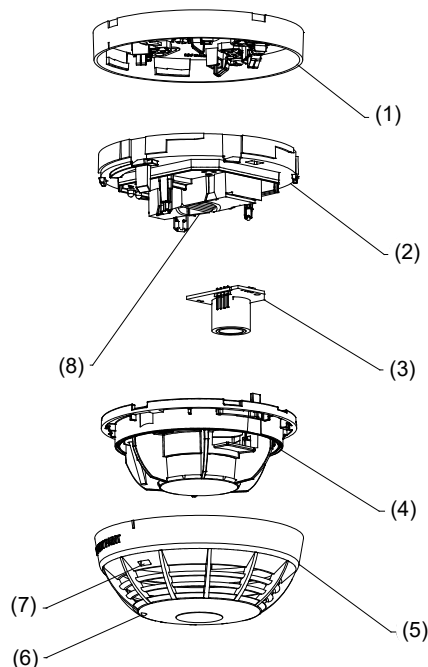
Figure 81: SIGA2 smoke detector with CO sensor
