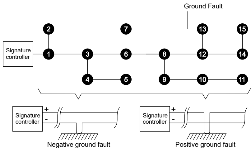
Figure 90: Signature signaling line circuit ground faults
