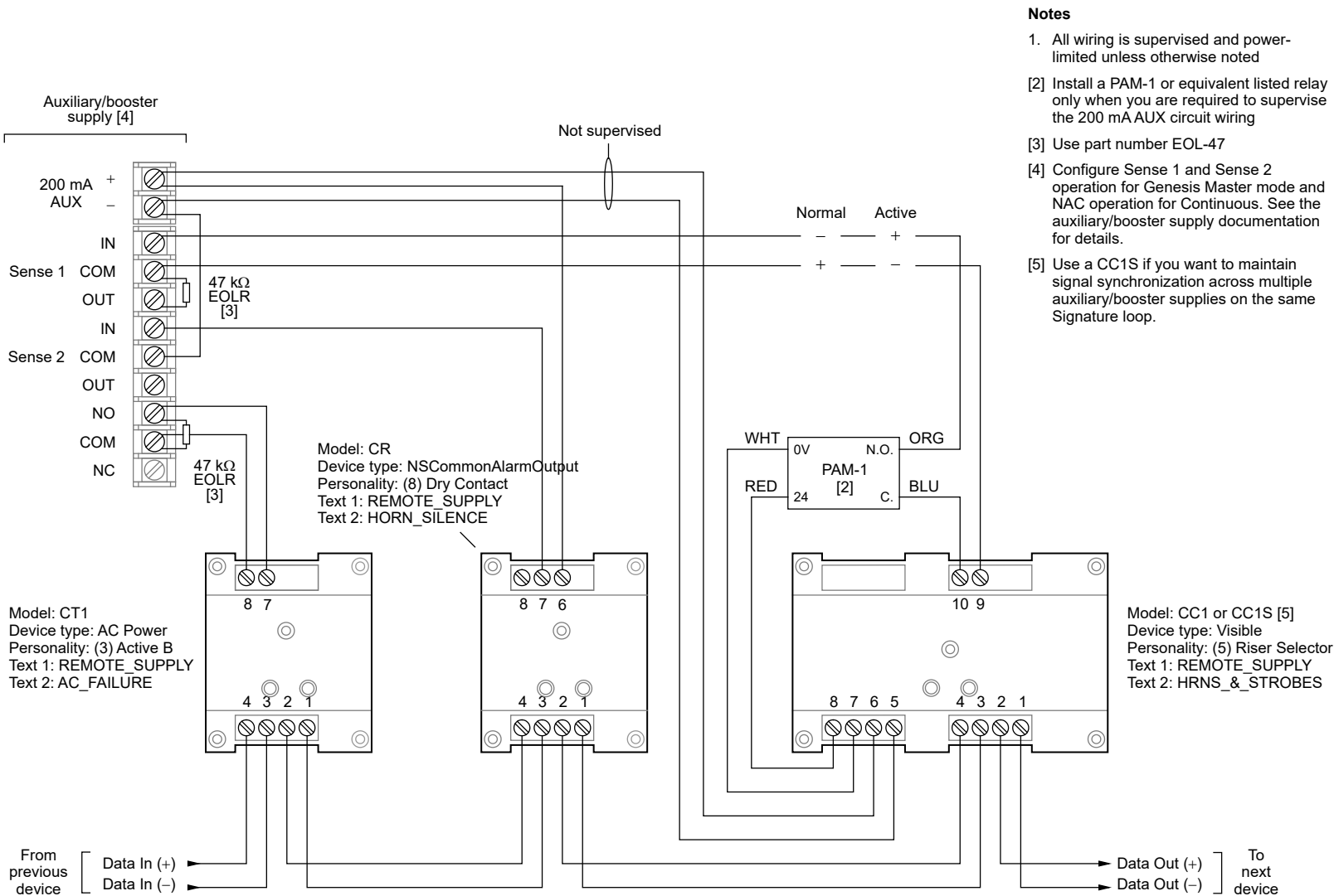
Figure 69: Using an auxiliary/booster supply to provide horn silence capability with two wires
