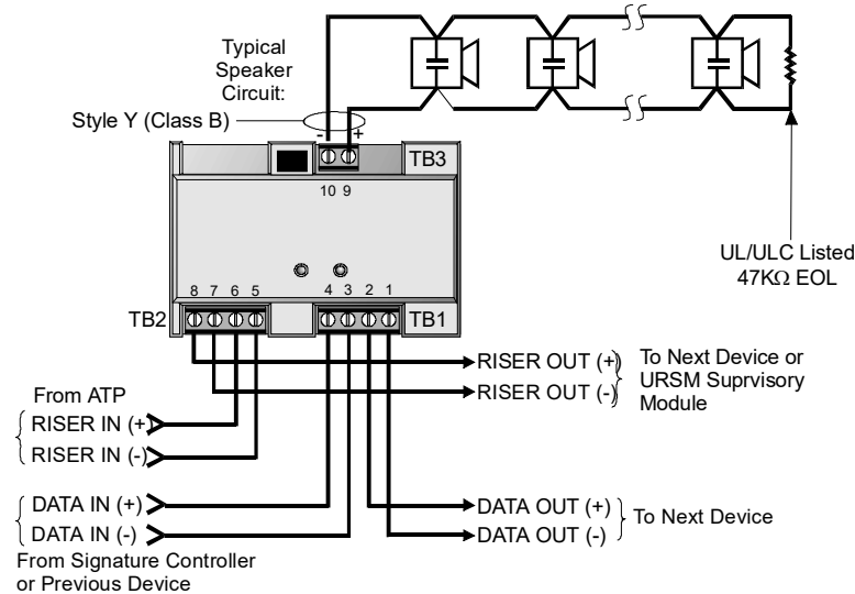
Figure 62: Single channel Class B wiring, SIGA-CC1 module
