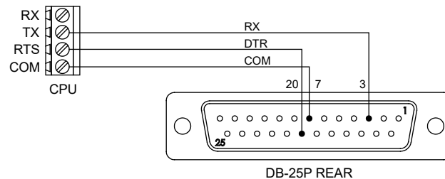
Figure 75: Wiring diagram (supervised connection)
