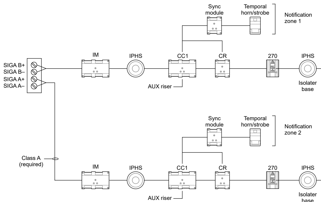
Figure 66: Signature wiring for notification circuit signal synchronization
