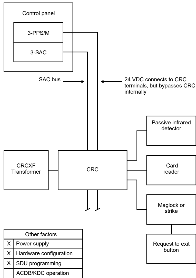
Figure 41: CRC using AC power
