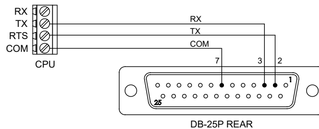
Figure 74: Wiring diagram (unsupervised connection)
