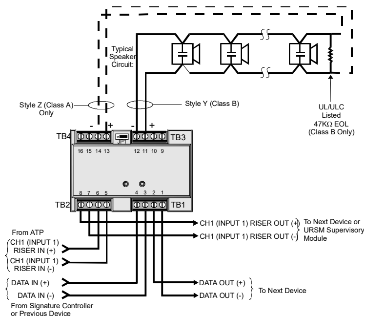
Figure 64: Single channel Class A wiring, SIGA-UM Module
