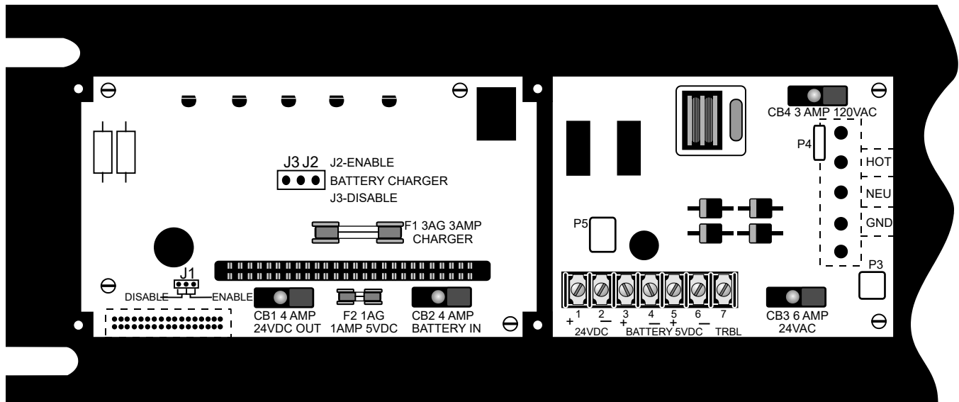
Figure 57: Power supply terminal card, with 3-ATPINT, cover removed
