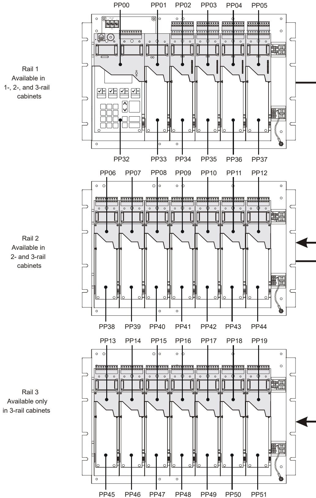
Figure 106: LRM addresses for 3-CHAS7, 3-CHAS7, 3-CHAS7 configuration
