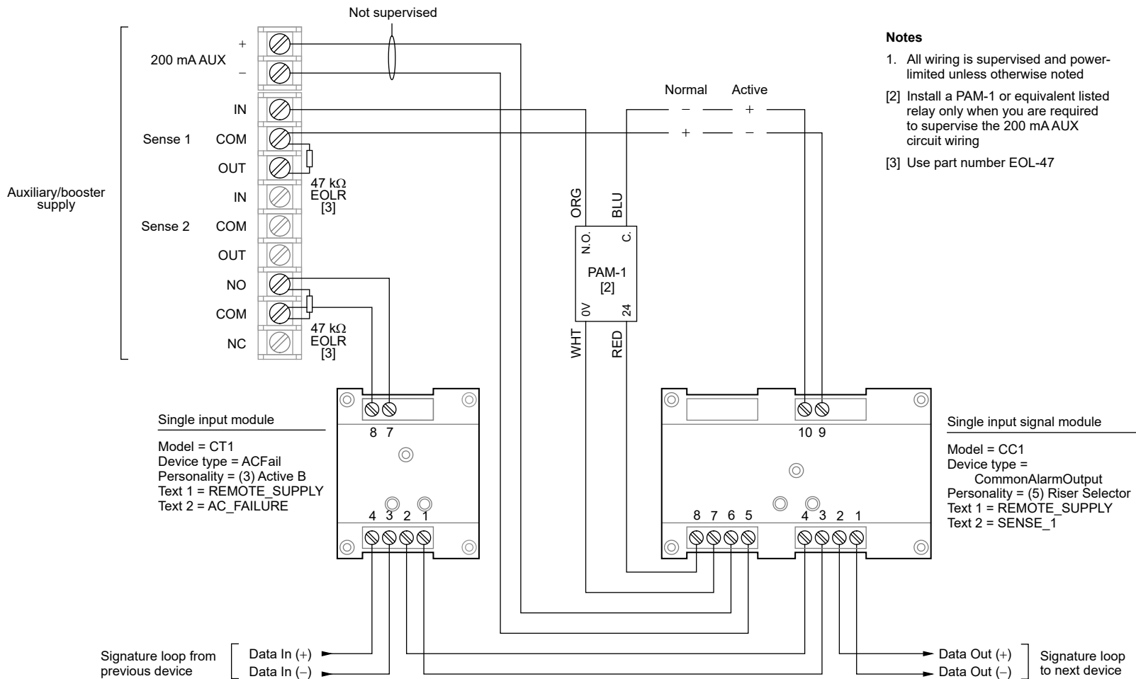
Figure 73: Typical booster power supply wiring
