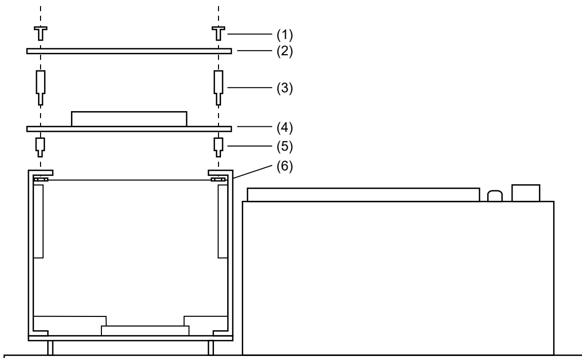
Figure 53: 3-ATPINT installation, bottom view
