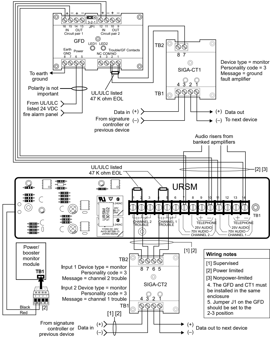
Figure 52: URSM wiring
