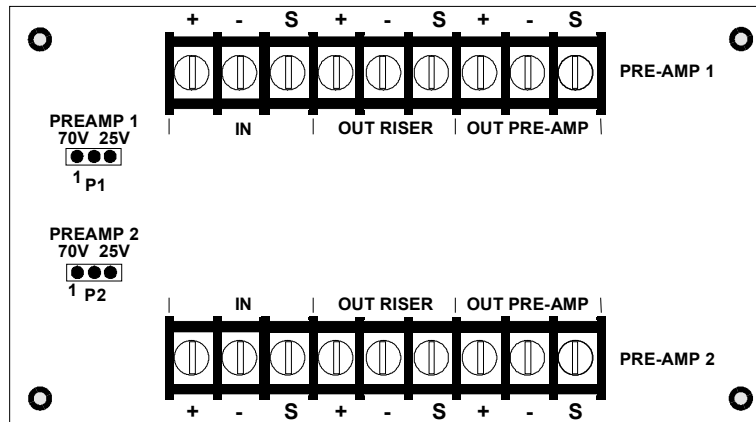
Figure 49: 3-ATPINT Interface Card
