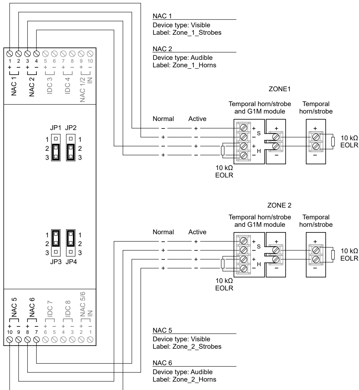
Figure 65: Typical 3-IDC8/4 card NAC wiring
