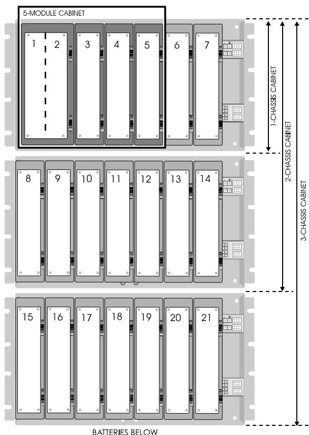
Figure 71: Local rail module slot identification
