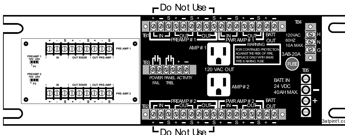
Figure 54: ATP with 3-ATPINT installed, rear view
