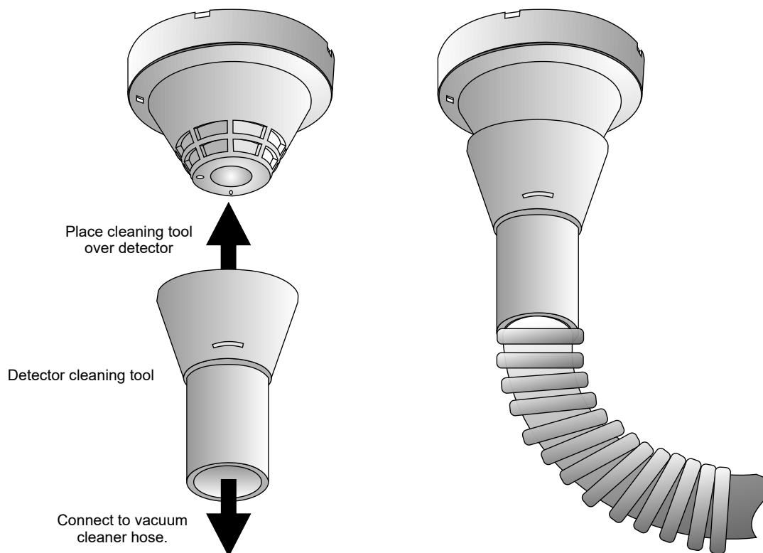
Figure 80: Detector cleaning tool
