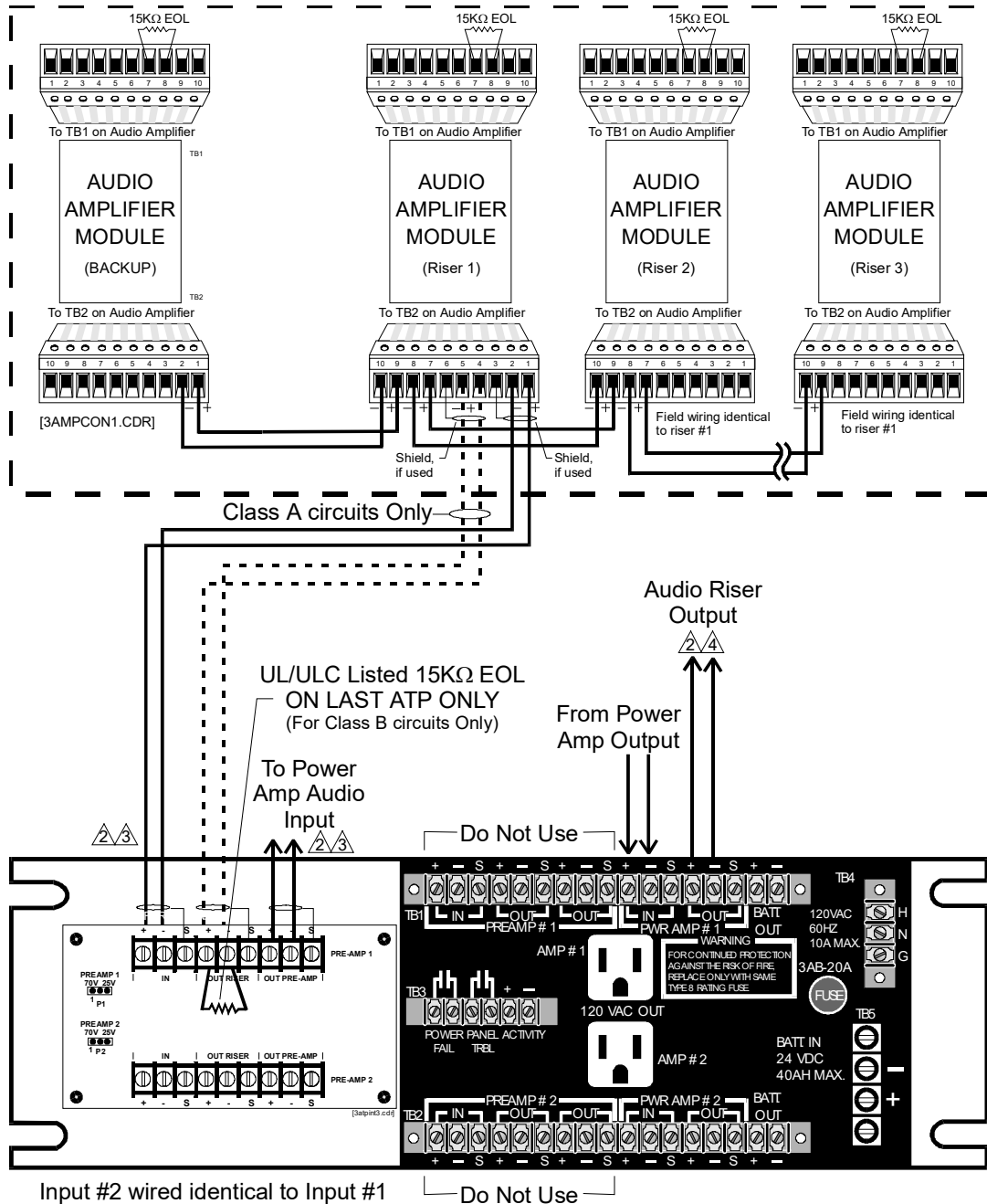
Figure 55: ATP with 3-ATPINT wiring
