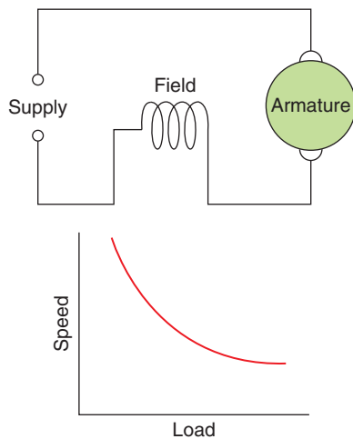
Figure 9.43 Series motor connections and characteristics.
