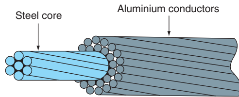
Figure 4.24 132kV overhead cable construction.
