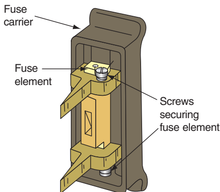
Figure 4.10 A semi-enclosed fuse.
