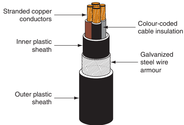
Figure 5.23 A four-core PVC/SWA cable.
