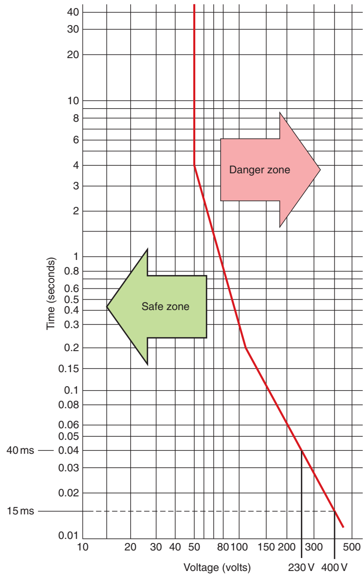
Figure 4.3 Touch voltage curve.
