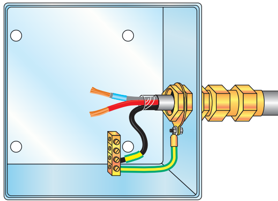
Figure 6.14 SWA cable correctly terminated in an electrical enclosure.
