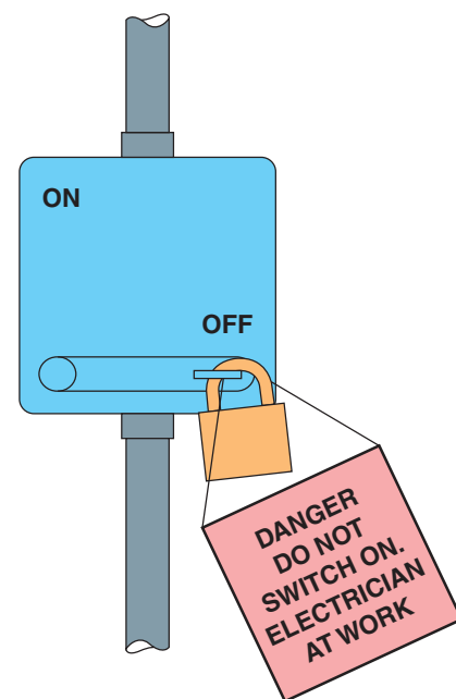
Figure 7.9 Secure isolation of a supply.
