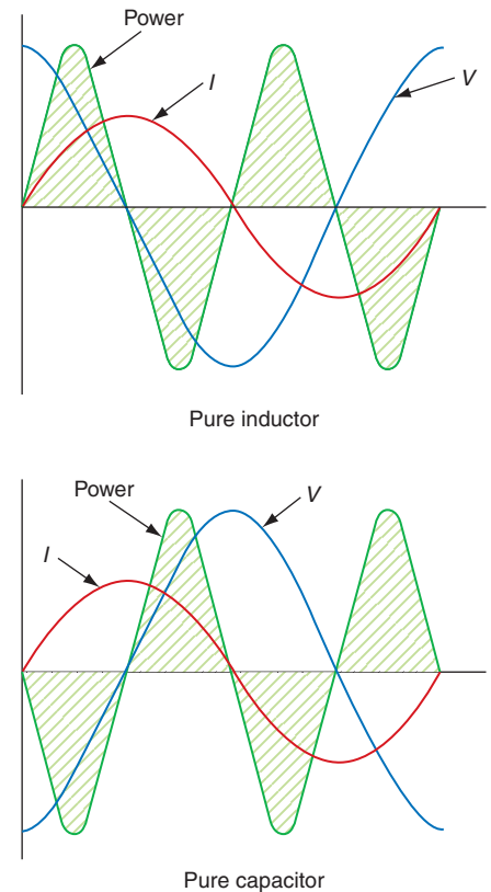
Figure 9.36 Waveform for the a.c. power in purely inductive and purely capacitive circuits.
