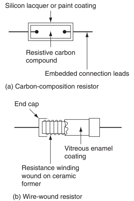
Figure 9.67 Construction of resistors.
