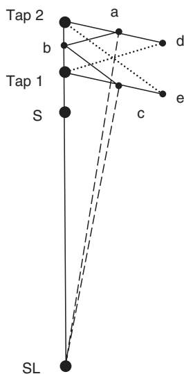
FIGURE 8.20 Voltage phasor diagrams involved in a tap change.
