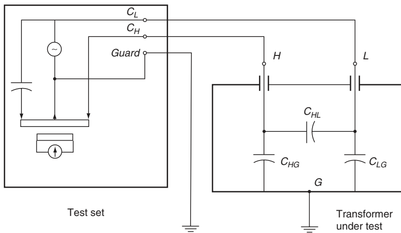
FIGURE 16.1 Measurement of capacitance and dissipation factor—high to low.
