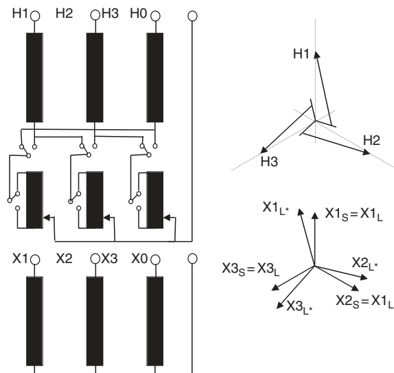
FIGURE 4.10 Regulating transformer with PST effect.
