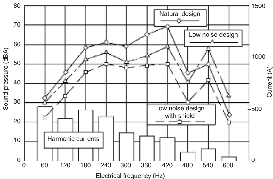
FIGURE 10.49 Design Comparison of sound-pressure levels; natural design vs. reduced noise design vs. shielded reduced noise design.
