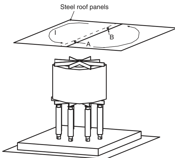
FIGURE 10.54 Example of improper joining of panels and potential local overheating.
