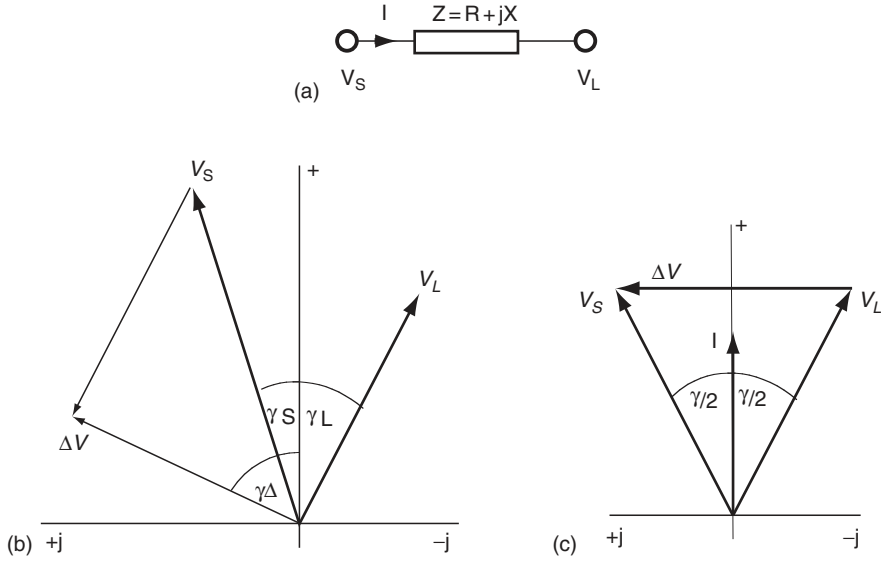
FIGURE 4.1 Power transfer.
