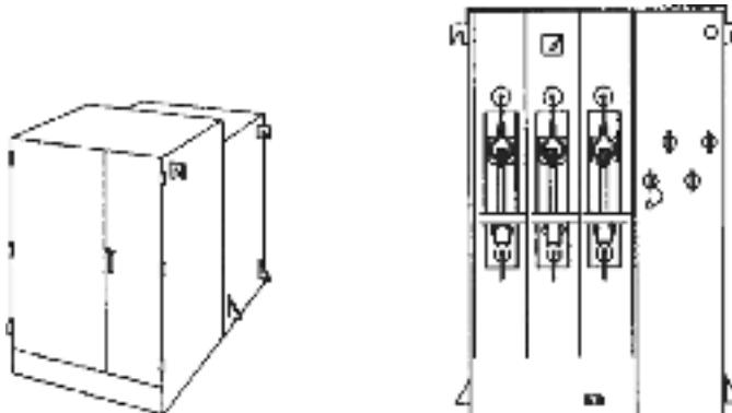
FIGURE 3.30 Loop-style live front. (By permission of Pacific Gas and Electric Company, San Francisco, CA.)
