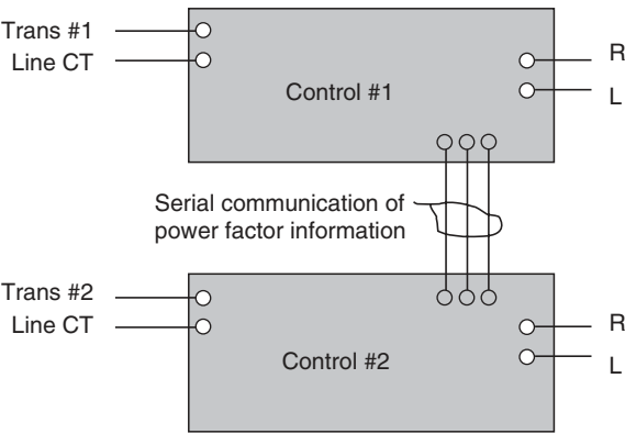
FIGURE 17.10 Control block diagram, paralleling by equal power factor, circulating-current method.
