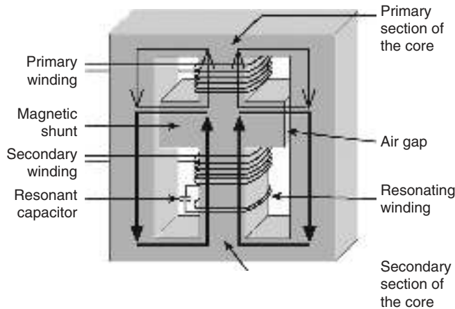
FIGURE 9.2 Components of a typical constant-voltage transformer.
