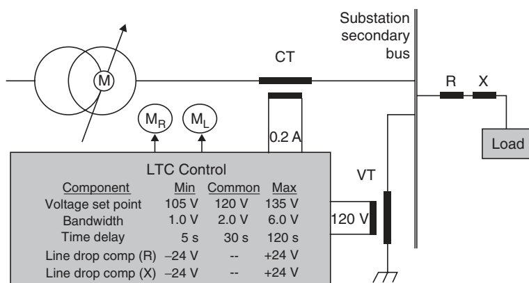
FIGURE 17.4 Control for voltage regulation at the load.
