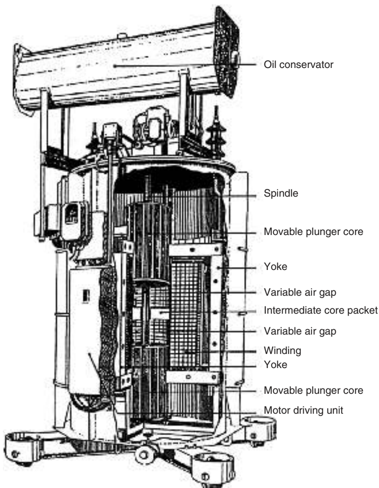
FIGURE 10.11 Arc suppression reactor.
