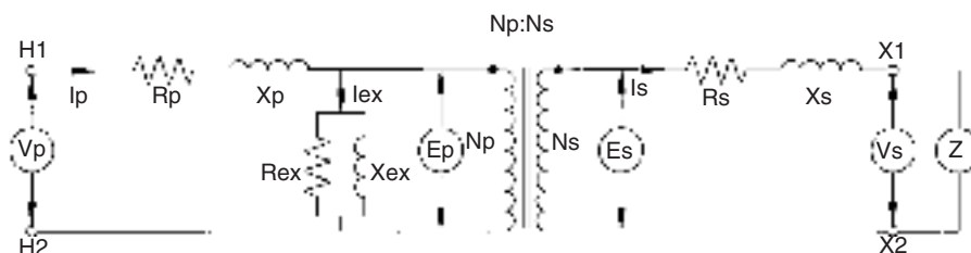
FIGURE 7.6 Equivalent transformer circuit.
