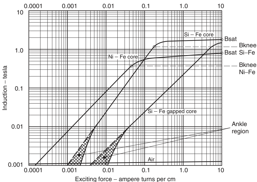
FIGURE 7.3 Typical characteristic curve.
