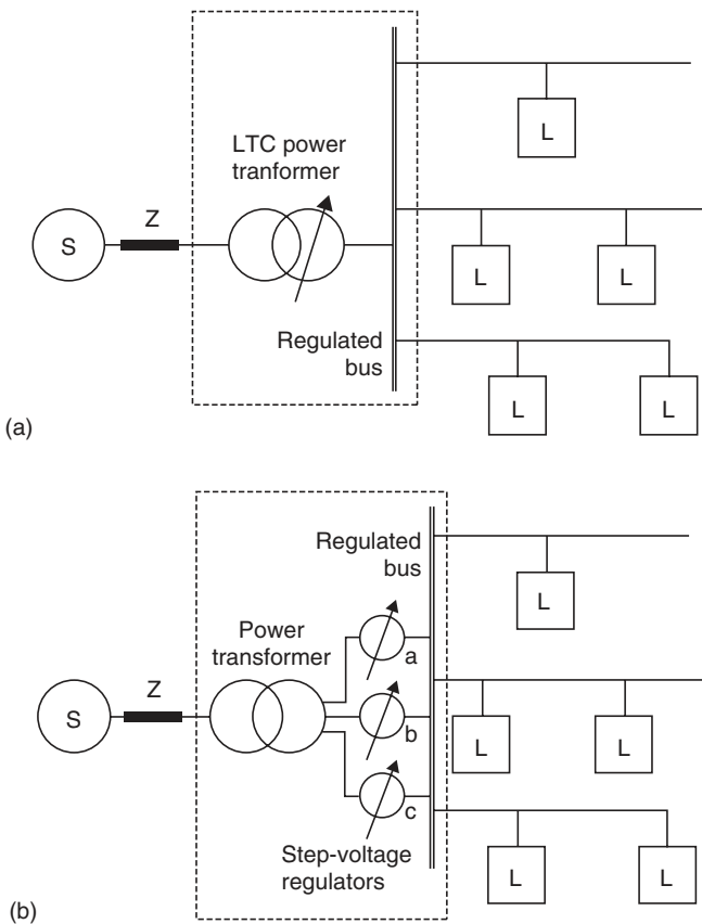
FIGURE 17.1 (a) Three-phase bus regulation with three-phase LTC transformer. (b) Independent-phase bus regulation with three single-phase step-voltage regulators.
