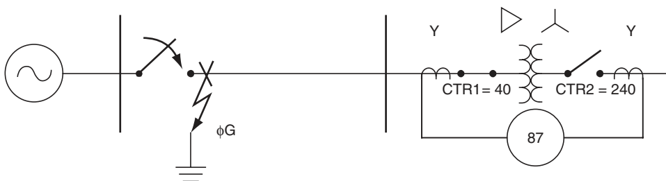
FIGURE 18.18 Transformer energization while A-phase is faulted.
