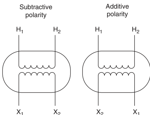
FIGURE 15.1 Single-phase transformer-terminal markings.
