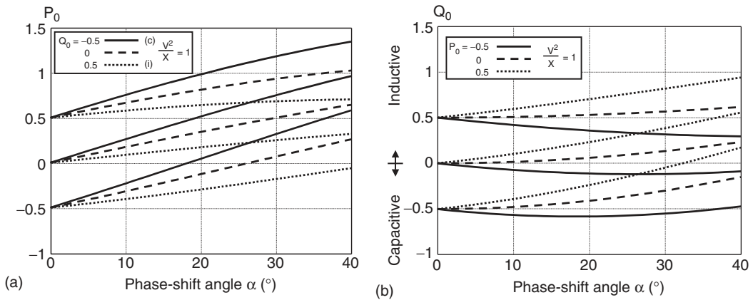
FIGURE 4.7 (a) Active power flow. (b) Reactive power flow.
