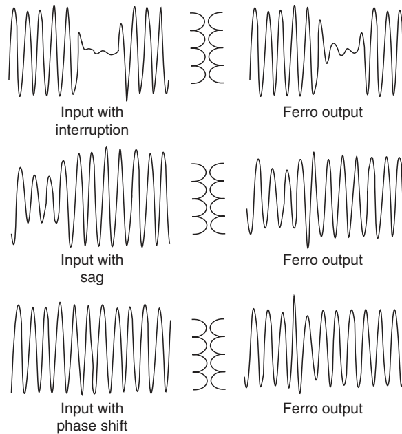
FIGURE 9.13 Output voltages (labeled ferro-output) resulting from voltage interruption, sag, and phase shift on the input.
