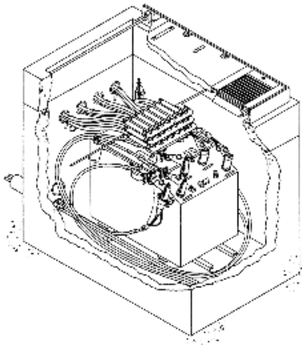
FIGURE 3.21 Four-bushing horizontal installed. (By permission of Pacific Gas and Electric Company, San Francisco, CA.)
