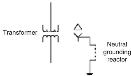
FIGURE 10.9 Typical neutral grounding reactor connection.
