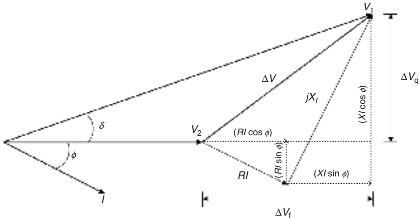
FIGURE 10.37 Power line balance phasor diagram.
