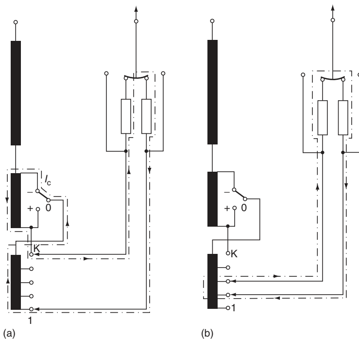
FIGURE 13.32 Effect of the leakage inductance of coarse winding/tap winding arrangement: (a) operation through mid-position; (b) operation through any tap position beside mid-position.
