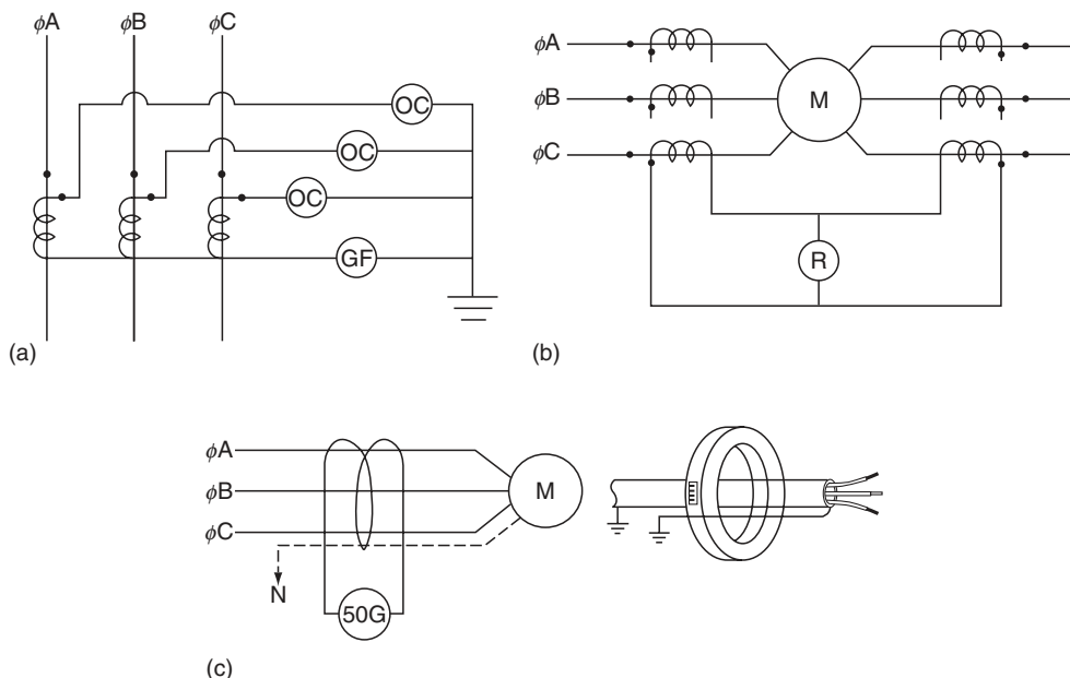
FIGURE 7.17 (a) Overcurrent and ground-fault protection scheme. (b) Differential protection scheme. (c) Zero-sequence scheme with all three-phase leads going through the window of the CT. This connection, as well as the residual connection in Figure 7.17a, will cancel out the positive- and negative-sequence currents leaving only the zero-sequence current to the 50G device. Sometimes the ground or neutral lead will be included. The diagram on the right shows sheathed cable. It is important that one ground point go back through the window to avoid the possibility of a shorted electrical turn via the ground path.
