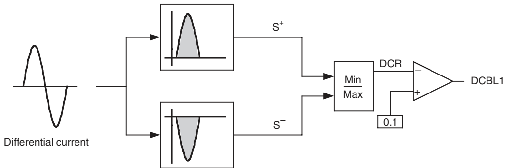
FIGURE 18.15 DC blocking logic.
