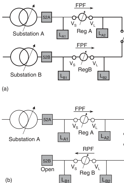
FIGURE 17.7 (a) Step-voltage regulator in routine application. (b) Step-voltage regulator in reverse power-flow application.
