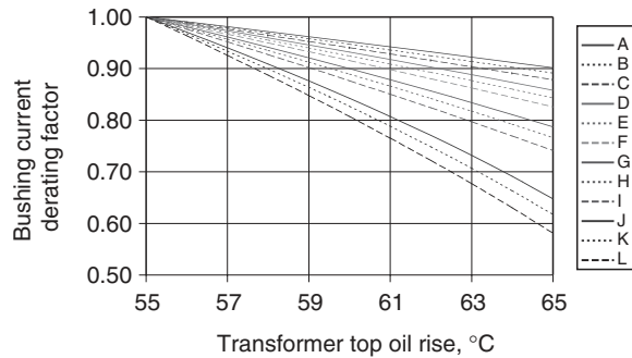
FIGURE 12.5 Bushing derating factors for transformer top-oil rises between 55 and 65°C.
