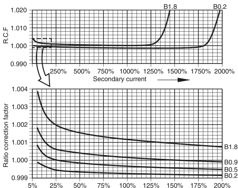
FIGURE 7.9 CT RCF characteristic curve.
