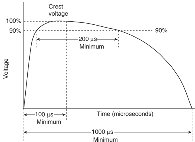
FIGURE 16.10 Standard switching-impulse wave.
