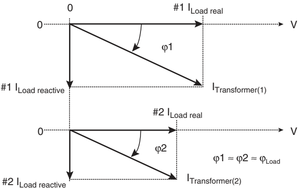
FIGURE 17.11 Phasor diagram—mismatched transformers in parallel by equal-power-factor method.
