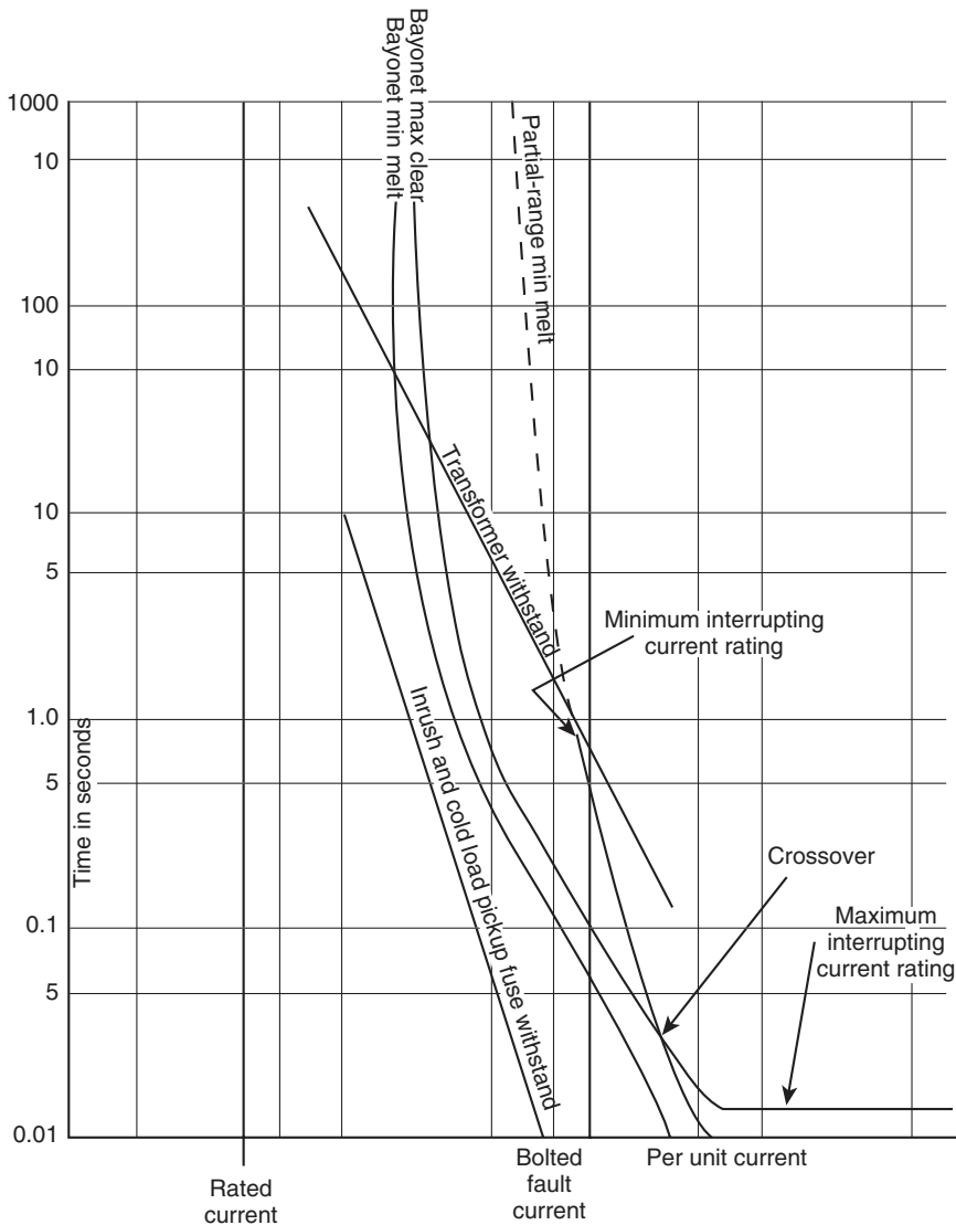
FIGURE 3.39 Time-current-curve crossover coordination. (By permission of ABB Inc., Jefferson City, MO.)
