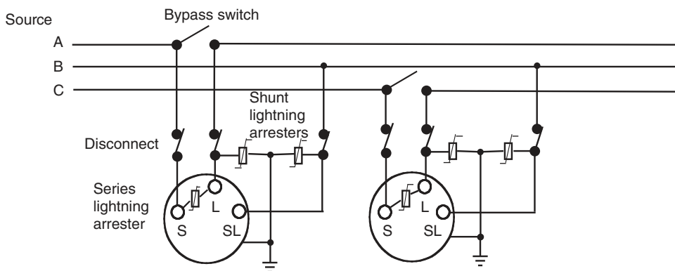
FIGURE 8.7 Connection of two voltage regulators regulating a three-phase, three-wire wye or delta circuit.
