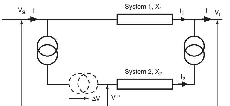
FIGURE 4.2 Parallel systems.
