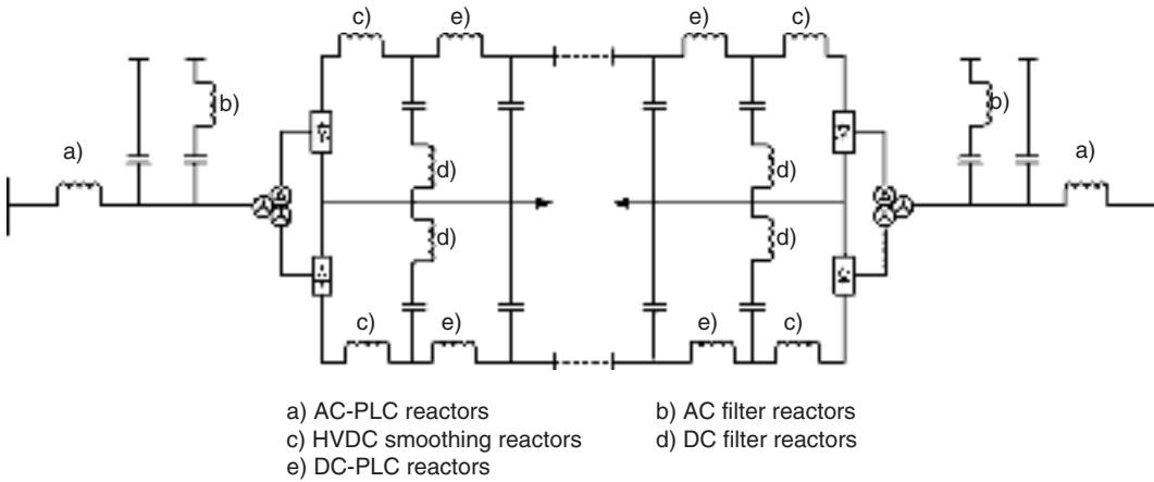
FIGURE 10.30 One line diagram of a typical HVDC bipole link illustrating reactor applications.
