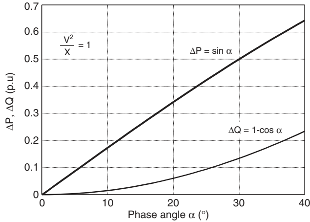
FIGURE 4.6 Additional power flow.
