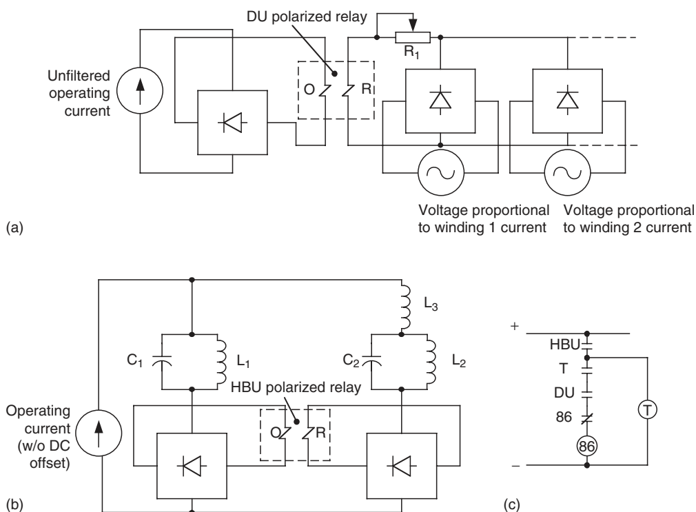
FIGURE 18.7 Transformer differential relay with second-harmonic blocking. (a) Differential unit, DU, (b) Harmonic blocking unit, HBU and (c) Simplified contact logic.
