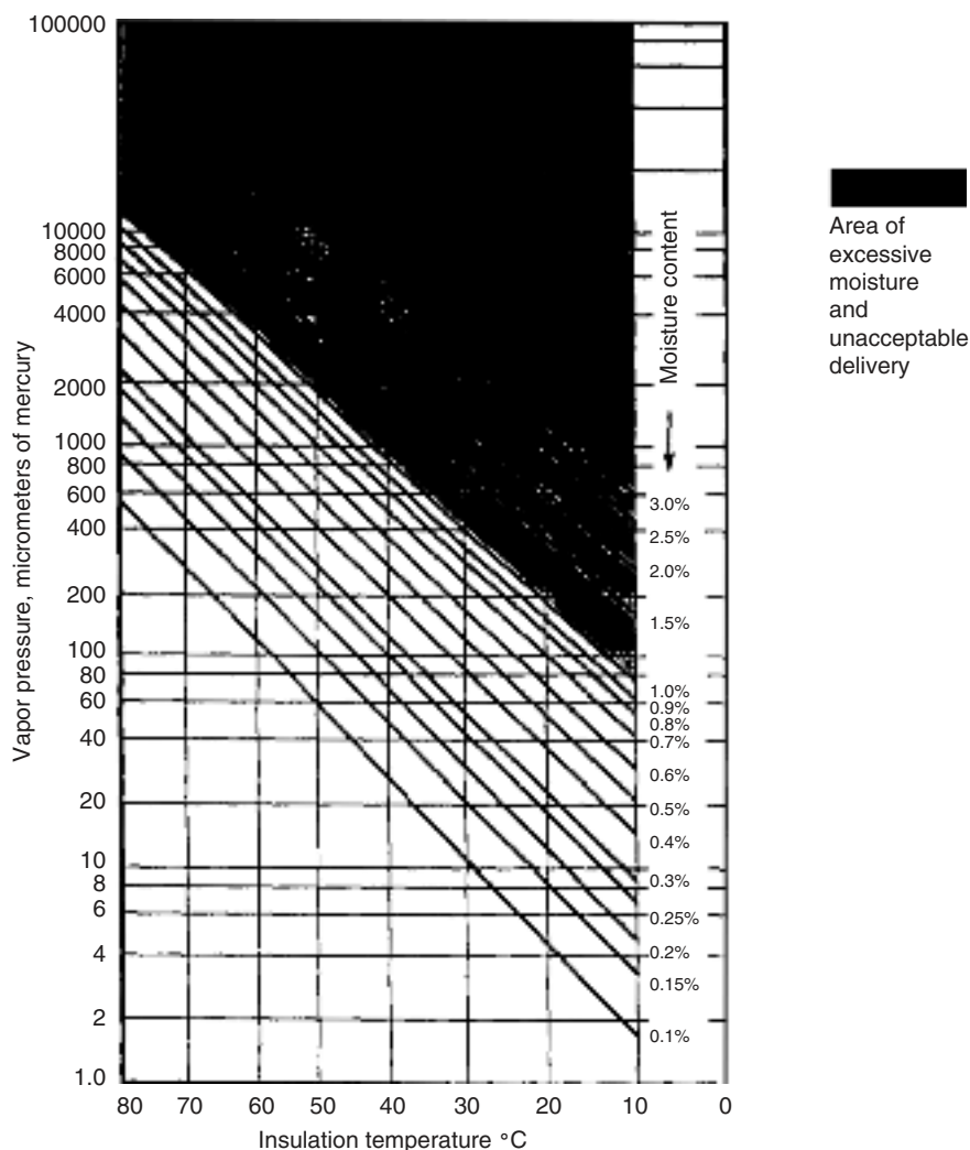
FIGURE 21.2 Moisture equilibrium chart (with moisture content in percent of dry weight of insulation). (Courtesy of Waukesha Electric Systems.)
