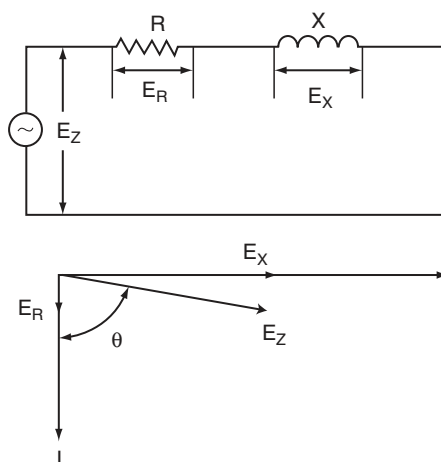
FIGURE 16.16 Equivalent circuit and phasor diagram for load-loss test.
