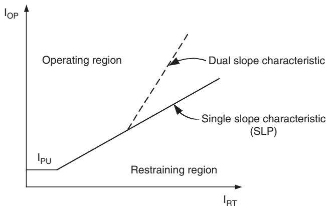
FIGURE 18.2 Differential relay with dual-slope characteristic.
