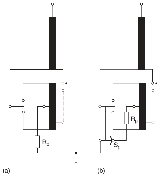
FIGURE 13.30 Methods of voltage connection (reversing change-over selector in mid-position): (a) fixed tie-in resistor R_p ; (b) with voltage switch S_p and tie-in resistor R_p .
