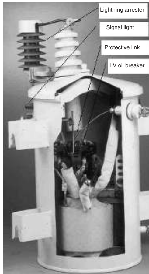
FIGURE 3.40 Cutaway showing CSP components. (By permission of ABB Inc., Jefferson City, MO.)
