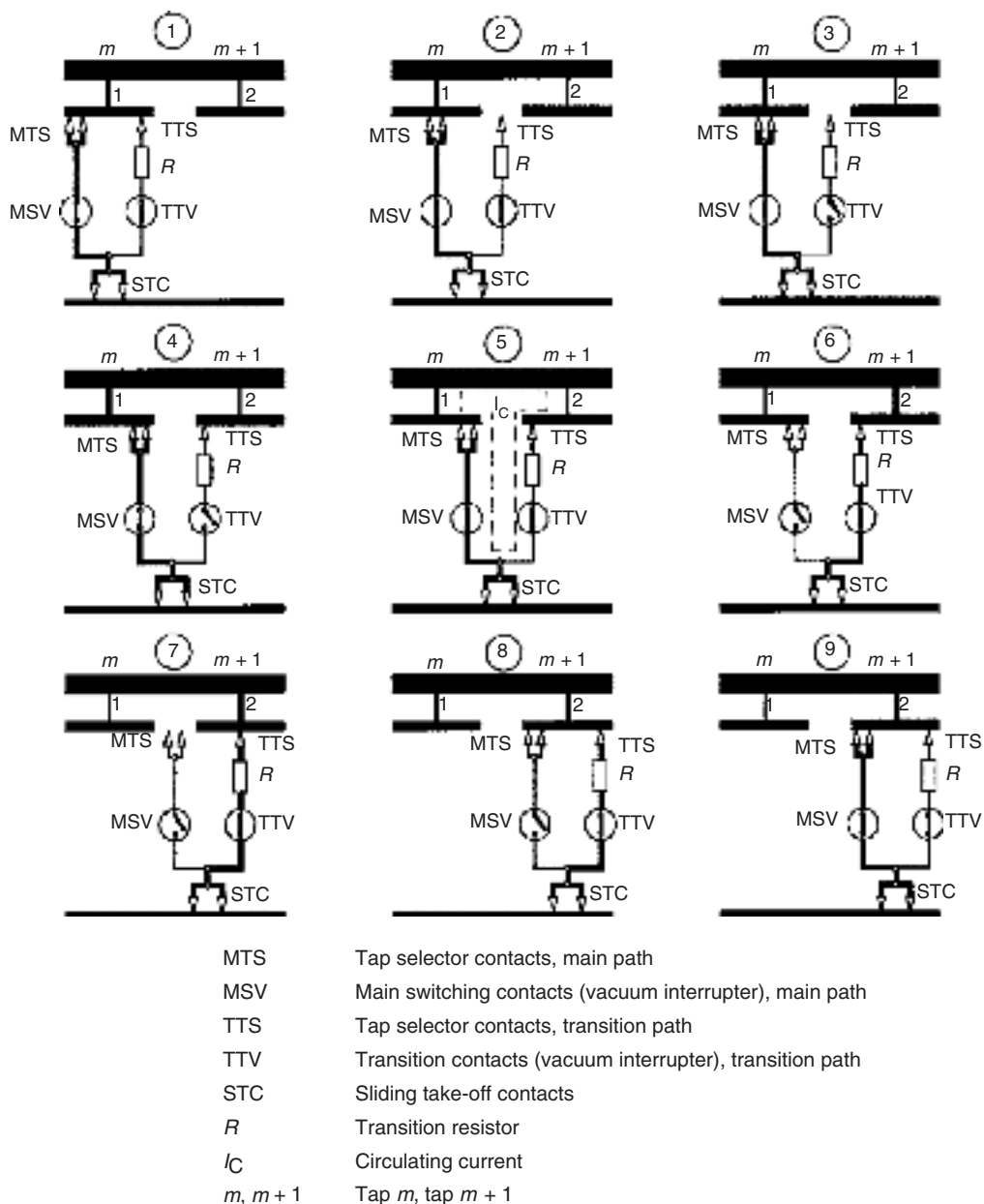
FIGURE 13.16 Switching sequence of resistor-type LTC with the same vacuum interrupters for the closing and opening side of the diverter switch.
