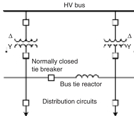
FIGURE 10.7 Typical bus tie reactor connection.
