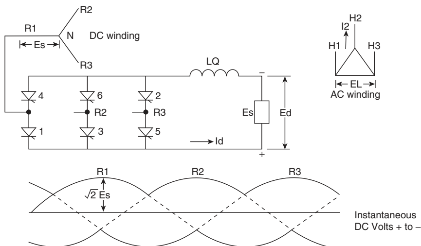
FIGURE 5.14 Three-phase bridge rectifier.
