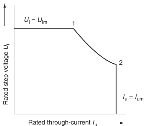
FIGURE 13.27 Rated step capacity diagram of a diverter switch: 1—upper limit point; 2—lower limit point.
