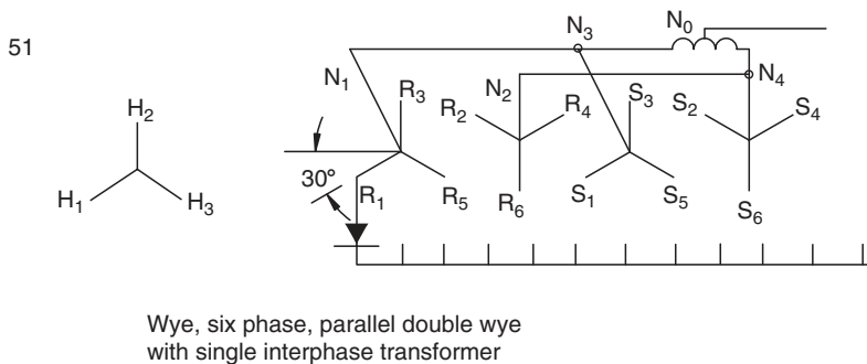
FIGURE 5.9 ANSI Circuit 51. (From ANSI/IEEE C57.18.10-1998. © IEEE 1998. With permission.)
