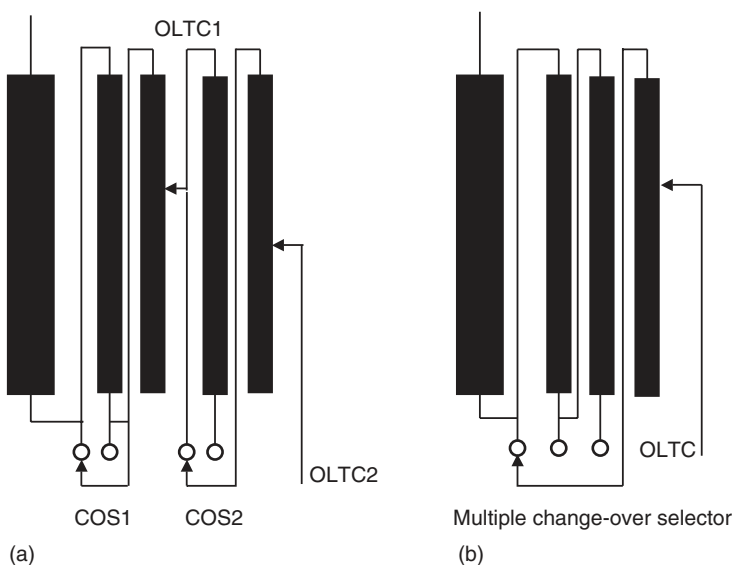
FIGURE 4.19 Use of more than one OLTC and/or multiple changeover selector.
