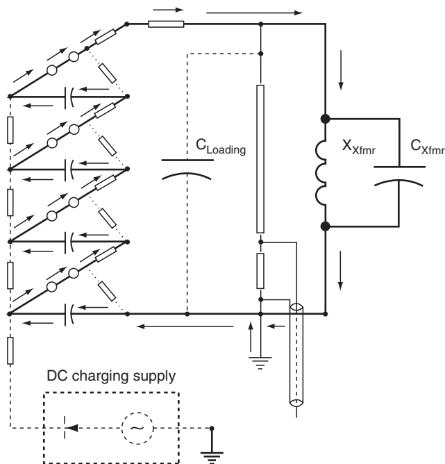
FIGURE 16.7 Discharging the capacitors of an impulse generator.
