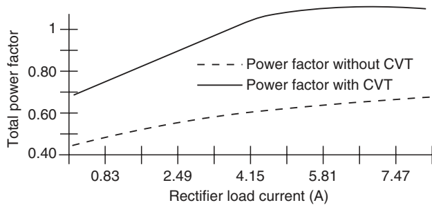
FIGURE 9.18 Power factor for a nonlinear load.
