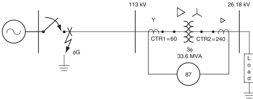
FIGURE 18.22 Transformer energization while A-phase is faulted and the transformer is loaded.
