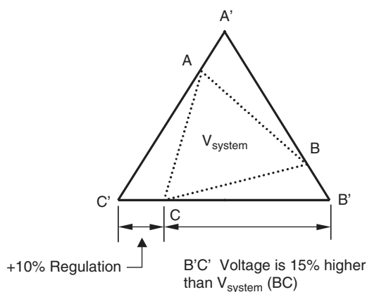
FIGURE 8.10 Phasor diagram of closed-delta-connected voltage regulators.
