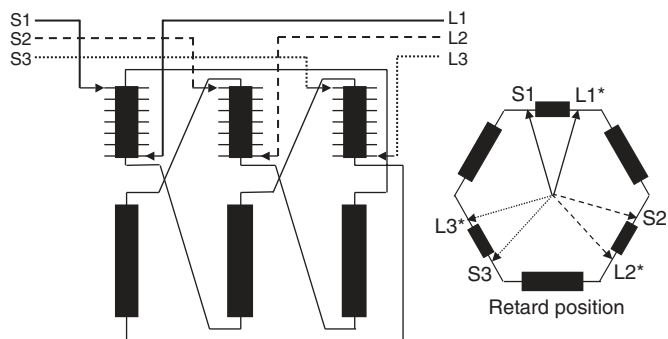
FIGURE 4.11 Delta-hexagonal PST.
