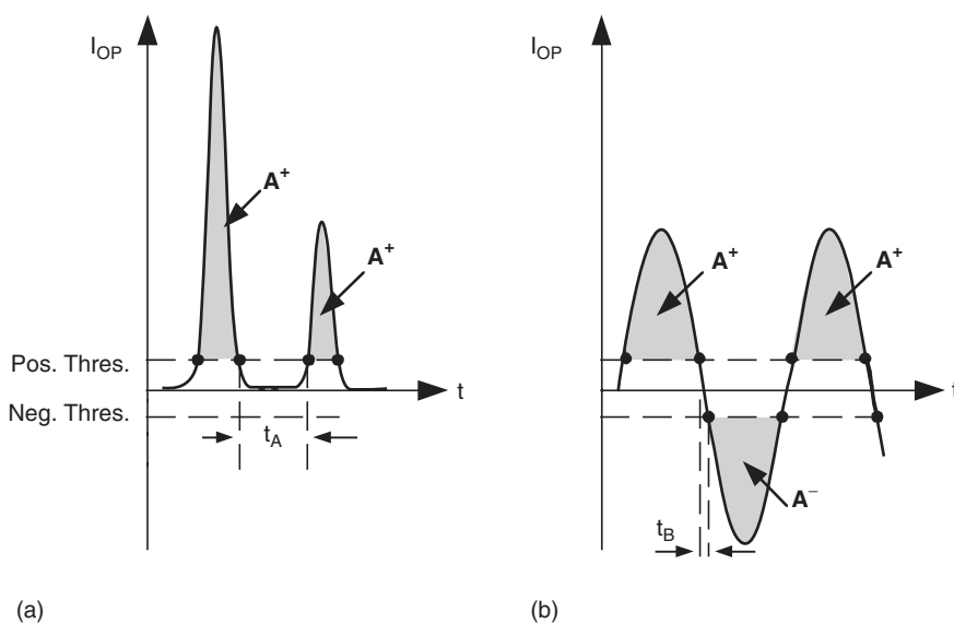
FIGURE 18.11 Differential-relay blocking based on recognizing the duration time of low-current intervals. (a) Inrush current and (b) Internal fault current.
