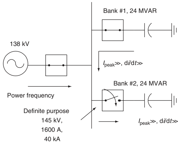
FIGURE 10.15 Back-to-back switching in a 138 kV substation.
