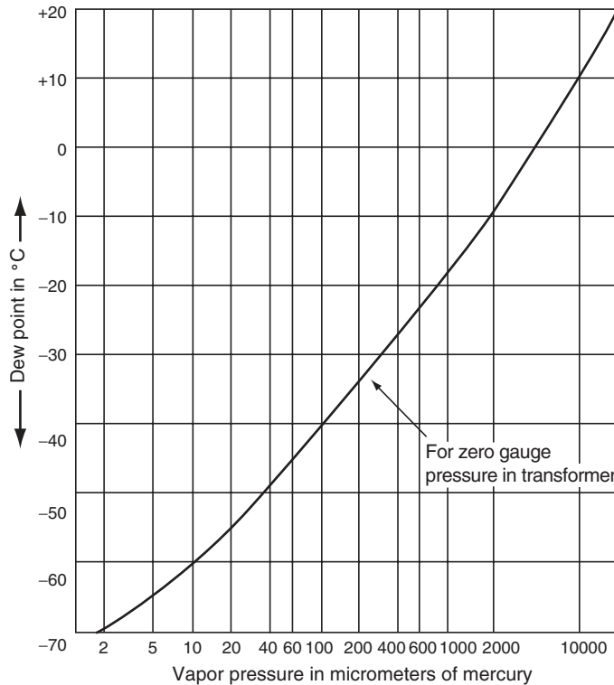
FIGURE 21.1 Conversion of dew point to vapor pressure. (Courtesy of Waukesha Electric Systems.)
