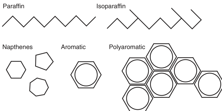
FIGURE 11.1 Carbon configurations in oil molecules.
