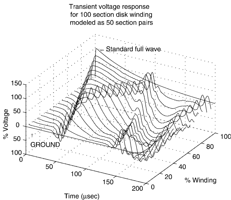
FIGURE 20.2 Voltage versus time for helical winding.
