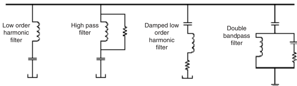
FIGURE 10.29 Typical filter reactor connections.
