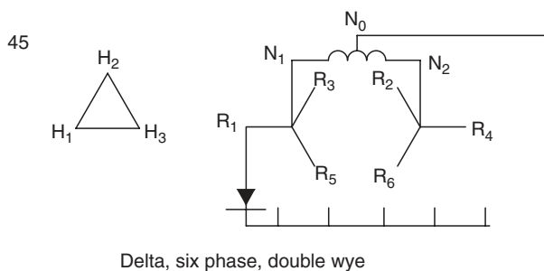
FIGURE 5.5 ANSI Circuit 45. (From ANSI/IEEE C57.18.10-1998. © IEEE 1998. With permission.)
