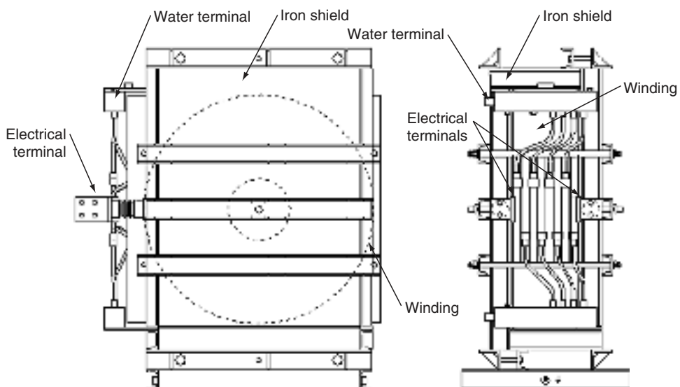
FIGURE 10.4 Dry-type iron-core reactor (water cooled).
