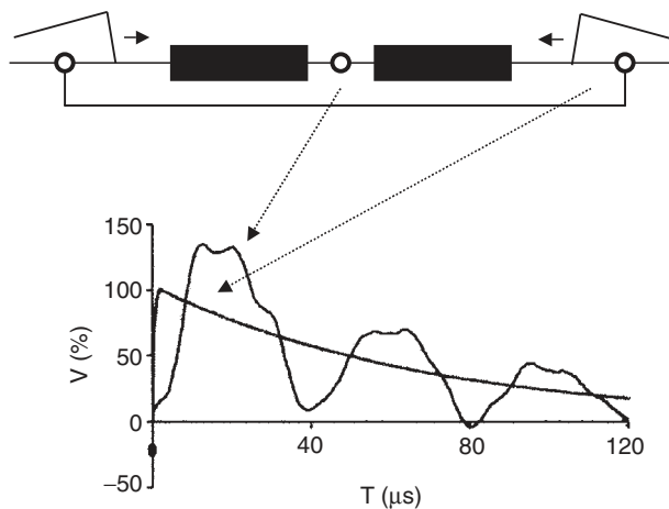
FIGURE 4.16 Lightning impulse response (bypassed PST).
