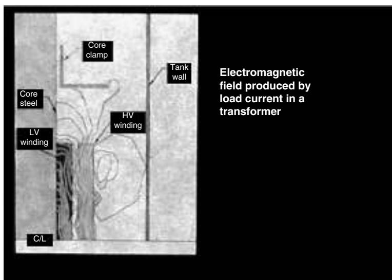
FIGURE 5.15 Transformer construction and electromagnetic leakage field.
