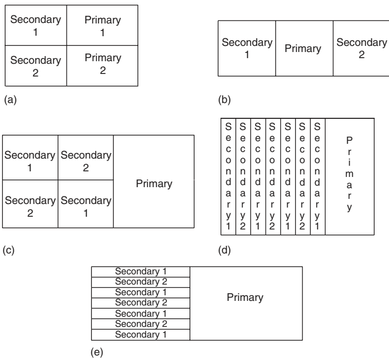
FIGURE 5.12 (a) Two-tier or stacked-coil arrangement. (b) Concentric-coil arrangement. (c) Split stacked-secondary arrangement. (d) Interleaved or bifilar secondary arrangement. (e) Interleaved helical secondary arrangement.
