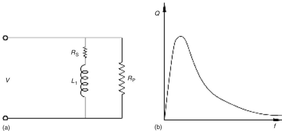
FIGURE 10.45 (a) Circuit diagram corresponding to a resistor in parallel with a fully modeled reactor, i.e., one having series resistance; (b) Q vs. frequency characteristic of a reactor with parallel resistor.
