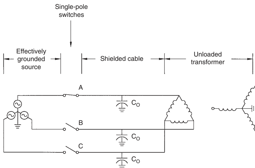
FIGURE 3.10 Typical ferroresonance situation. (From IEEE C57.105-1978, IEEE Guide for Application of Transformer Connections in Three-Phase Distribution Systems, copyright 1978 by the Institute of Electrical and Electronics Engineers, Inc. The IEEE disclaims any responsibility or liability resulting from the placement and use in the described manner. Information is reprinted with the permission of the IEEE.)
