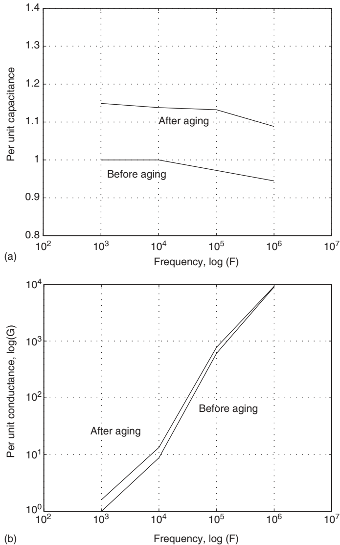
FIGURE 20.7 (a) Oil-soaked paper capacitance as a function of frequency; (b) Oil-soaked paper conductance as a function of frequency.
