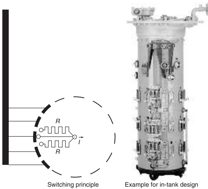
FIGURE 13.7 Design principle—selector switch (arcing tap switch). (Photo courtesy of Maschinenfabrik Reinhausen GmbH.)
