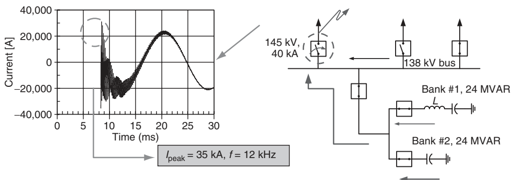
FIGURE 10.18 Circuit condition that leads to outrush current (right), outrush current (left).
