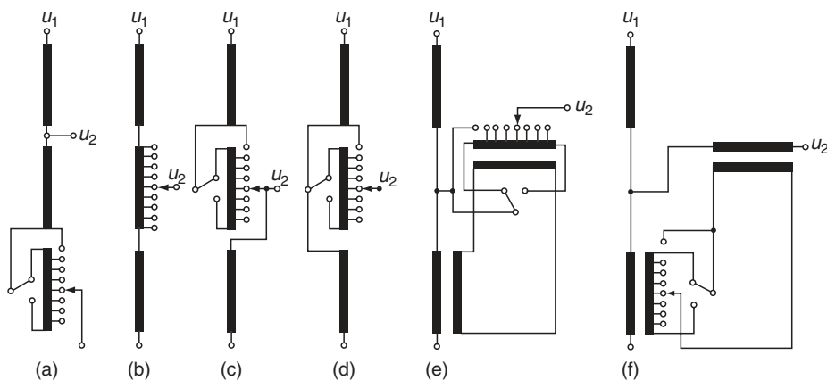
FIGURE 13.24 LTC in autotransformers.
