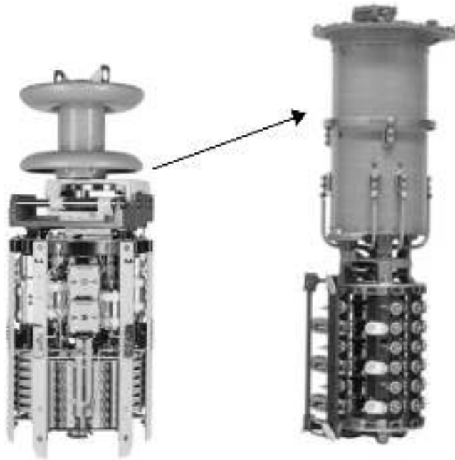
FIGURE 13.15 Resistor vacuum-type LTC with separate diverter switch and tap selector for in-tank installation in liquid filled power transformers. (Photo courtesy of Maschinenfabrik Reinhausen GmbH.)
