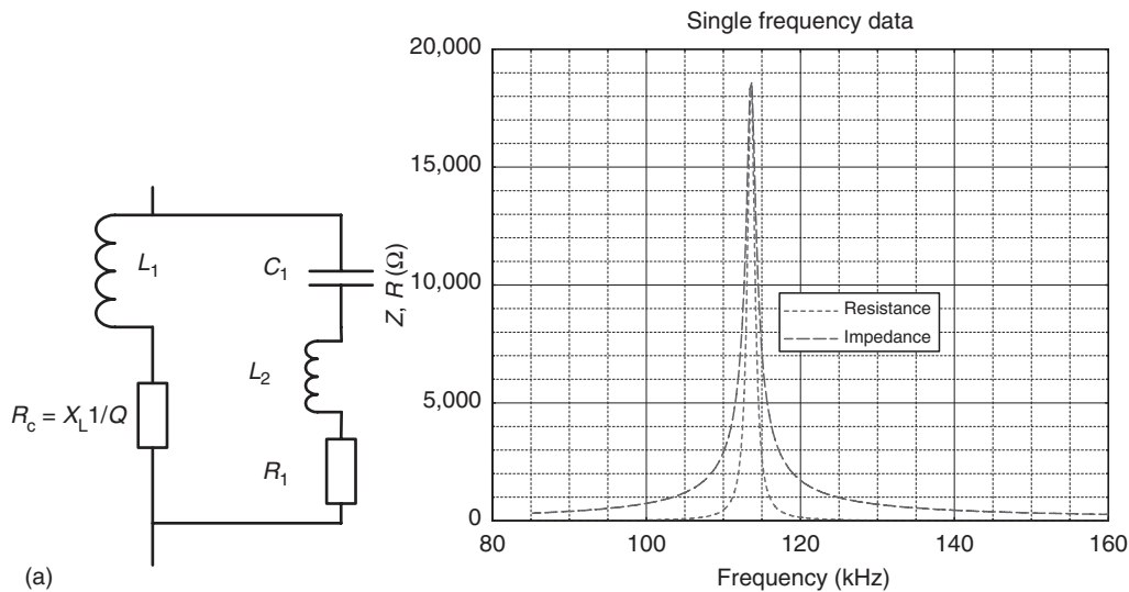
FIGURE 10.53 (a) Single frequency schematic and impedance response.
