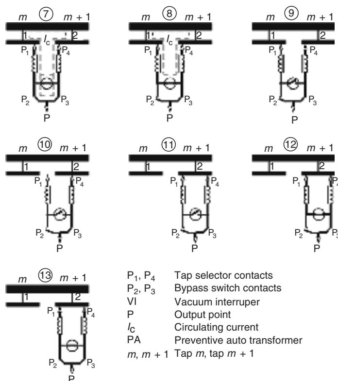
FIGURE 13.19 Switching sequence of reactor-type LTC with one vacuum interrupter per phase from bridging to nonbridging position.
