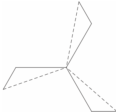
FIGURE 5.17 Zigzag wye-winding shift.
