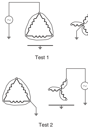
FIGURE 16.11 Applied-voltage tests on two-winding transformers.
