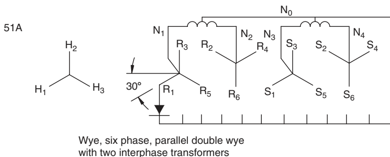
FIGURE 5.10 ANSI Circuit 51A. (From ANSI/IEEE C57.18.10–1998. © IEEE 1998. With permission.)
