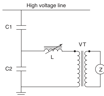
FIGURE 7.13 CCVT simplified circuit.
