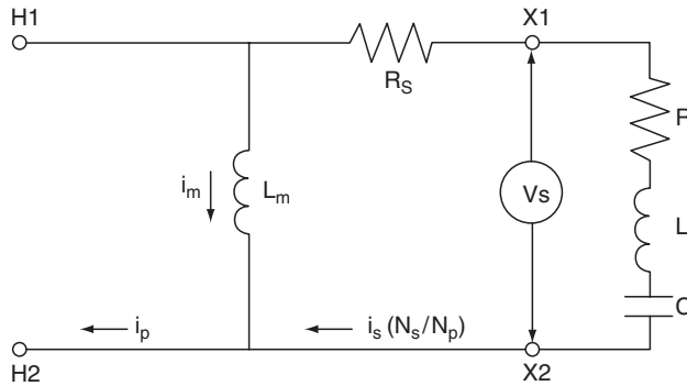
FIGURE 7.24 Linear-coupler equivalent circuit.
