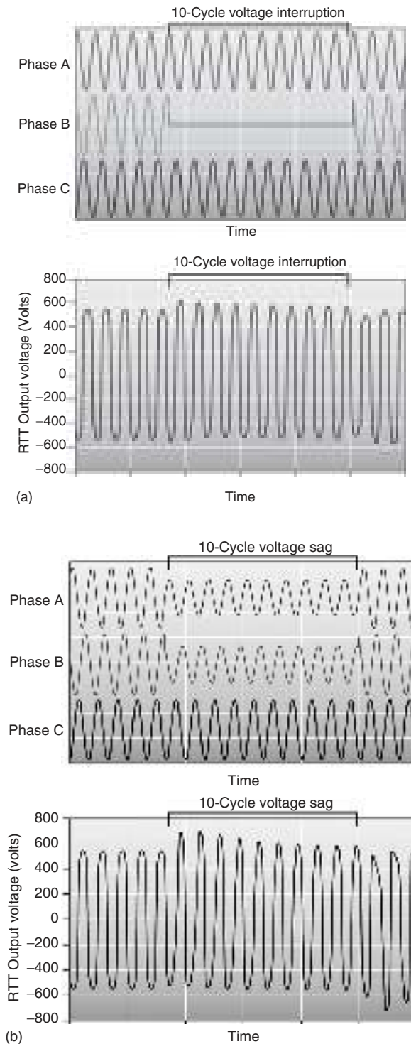
FIGURE 9.20 (a) Performance of a ride-through transformer (RTT) during a ten-cycle voltage interruption and voltage sag. Voltage regulation of an RTT during a single-phase voltage interruption (top: input; bottom: output). (b) Performance of a ride-through transformer (RTT) during a ten-cycle voltage interruption and voltage sag. Voltage regulation of an RTT during a two-phase ten-cycle voltage sag to 60% of nominal (top: input; bottom: output).
