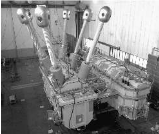
FIGURE 4.17 Two-tank PST at a test site (coolers not assembled) (650 MVA, 60 Hz, 525/525 \pm 20 \times 1.2^\circ kV). (By Courtesy of VATEch Transformatoren Weiz Austria (since 2005, Member of Siemens Group).)
