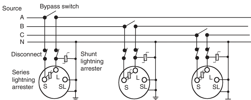
FIGURE 8.5 Connection of three regulators regulating a three-phase, four-wire, multigrounded wye circuit.
