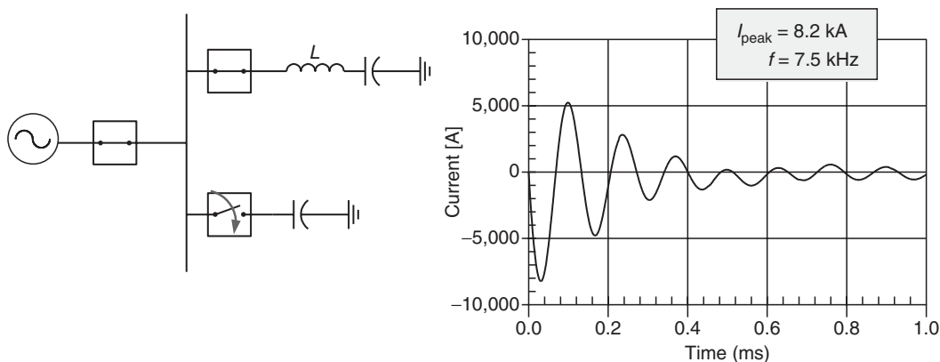
FIGURE 10.17 Back-to-back current after installation of a back-to-back capacitor reactor (right), in the circuit (left).
