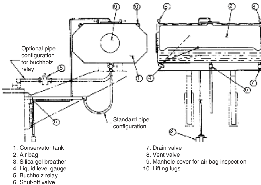
FIGURE 21.3 Outline of typical relay installation on transformer cover. (Courtesy of Waukesha Electric Systems.)
