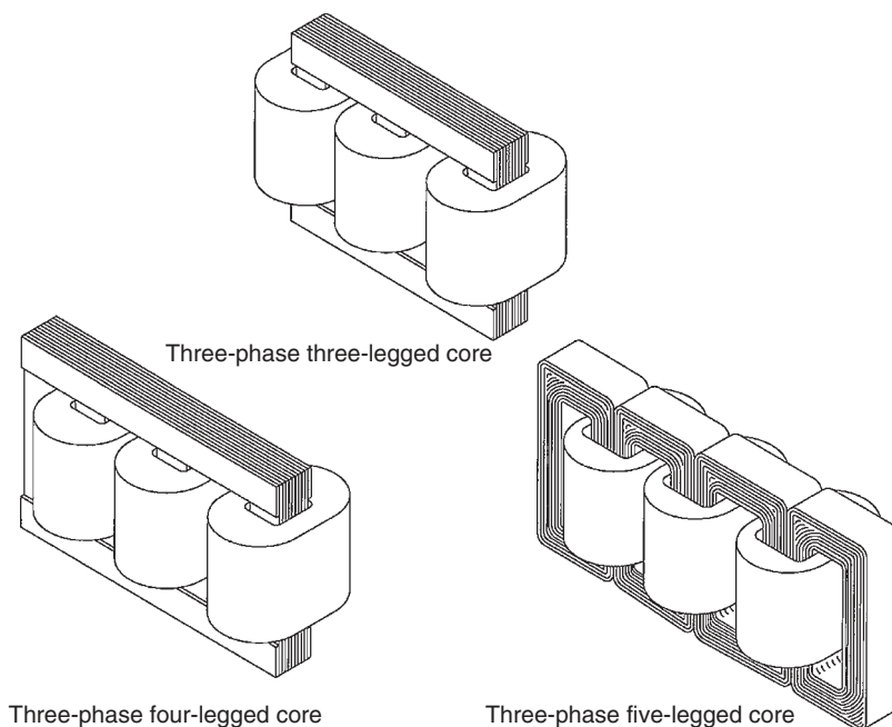
FIGURE 3.5 Three- and four-legged stacked cores and five-legged wound core. (From IEEE C57.105-1978, IEEE Guide for Application of Transformer Connections in Three-Phase Distribution Systems, copyright 1978 by the Institute of Electrical and Electronics Engineers, Inc. The IEEE disclaims any responsibility or liability resulting from the placement and use in the described manner. Information is reprinted with the permission of the IEEE.)
