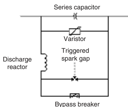
FIGURE 10.21 Typical discharge current limiting reactor connection.
