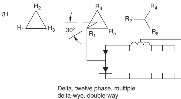
FIGURE 5.4 ANSI Circuit 31. (From ANSI/IEEE C57.18.10-1998. © IEEE 1998. With permission.)
