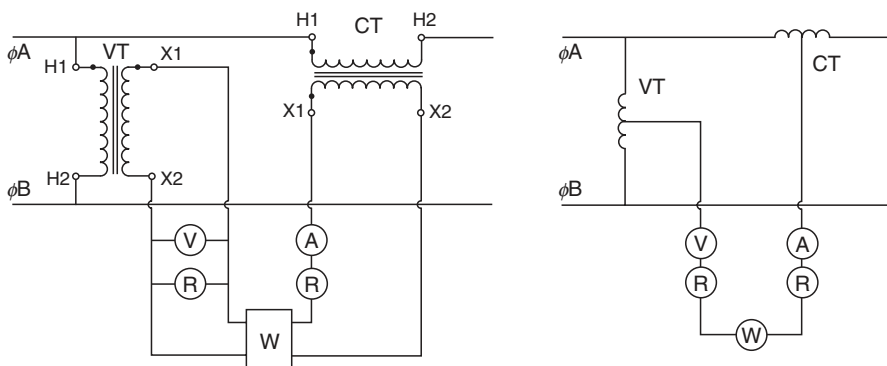
FIGURE 7.1 Typical wiring and single-line diagram.
