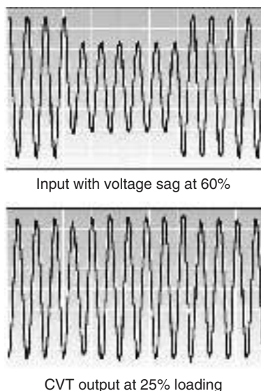
FIGURE 9.8 Voltage regulations with a constant-voltage transformer during a voltage sag to 60%.
