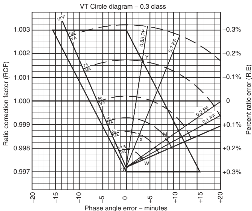
FIGURE 7.10 Voltage transformer circle diagram (fan curves).
