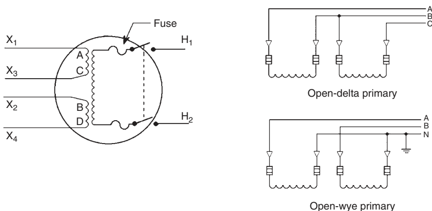
FIGURE 3.16 Two-bushing subway. (By permission of Pacific Gas and Electric Company, San Francisco, CA.)
