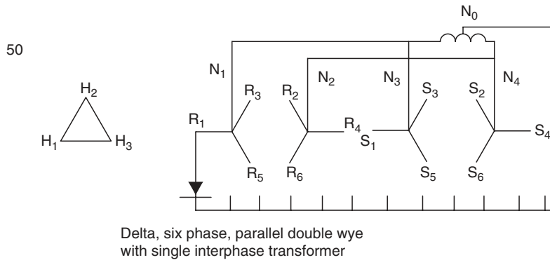
FIGURE 5.7 ANSI Circuit 50. (From ANSI/IEEE C57.18.10-1998. © IEEE 1998. With permission.)
