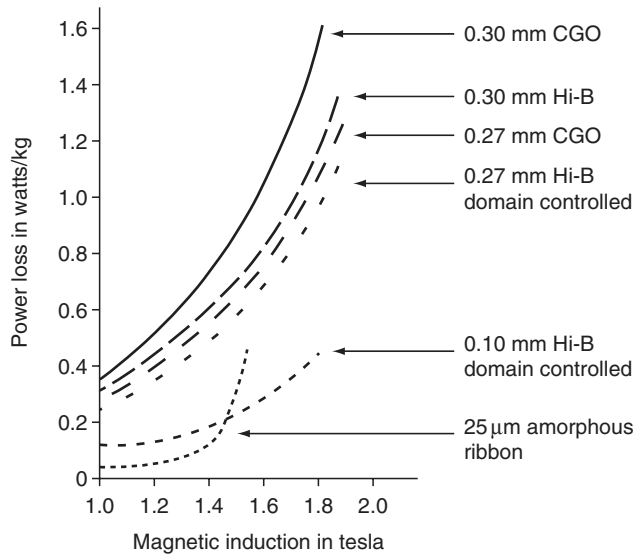
FIGURE 1.4 Loss characteristics for electrical core-steel materials over a range of magnetic induction (core flux density).
