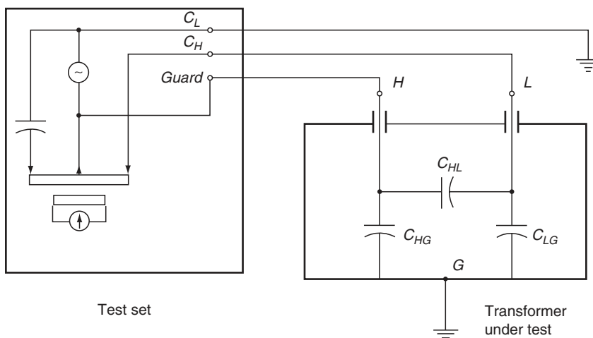
FIGURE 16.2 Measurement of capacitance and dissipation factor—low to ground.
