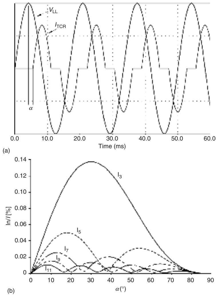
FIGURE 10.27 (a) TCR current and voltage waveforms. (b) TCR harmonic current spectra as a percentage of fundamental current.
