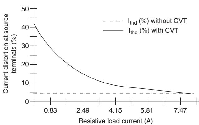
FIGURE 9.15 Line-current distortions for a linear load.
