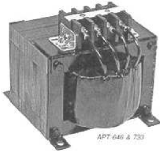
FIGURE 7.23 600-V, indoor-class auxiliary CT frame shell-type laminated “EI” core. (Photo courtesy of Kuhlman Electric Corp.)
