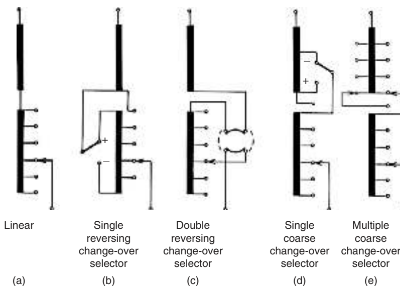
FIGURE 13.20 Basic arrangements of tap windings.
