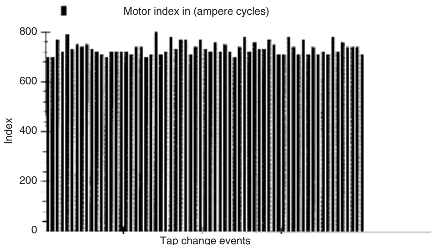
FIGURE 23.8 Sample motor-current-index curve.
