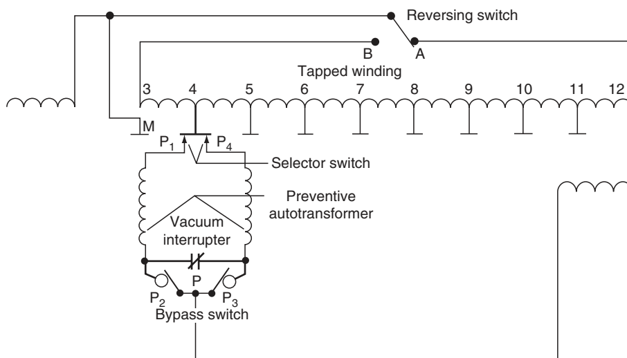
FIGURE 13.17 Reactor vacuum-type LTC—typical winding layout, LTC in position 16L.
