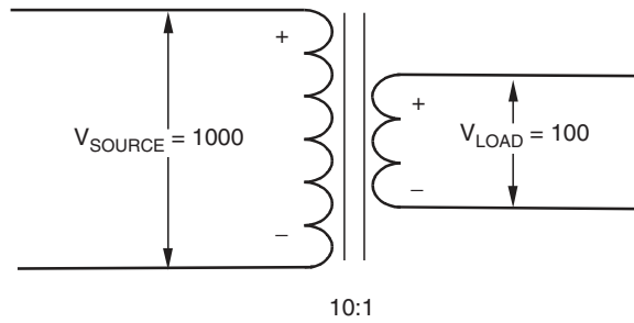
FIGURE 8.12 Transformer with 10:1 turns ratio.
