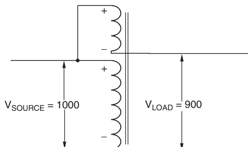
FIGURE 8.14 Step-down autotransformer.
