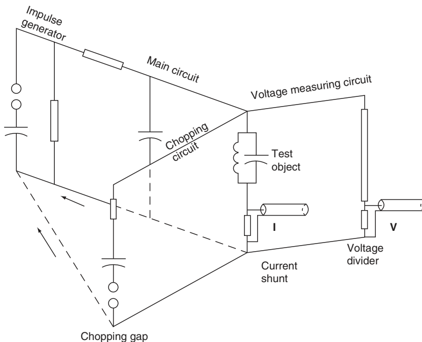
FIGURE 16.8 Impulse-test setup.
