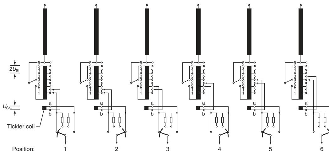
FIGURE 13.21 LTC for tap windings with tickler coil.
