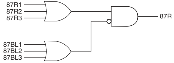
FIGURE 18.10 Common harmonic blocking method.
