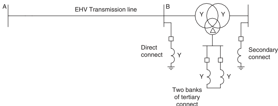
FIGURE 10.24 Typical shunt reactor connections.
