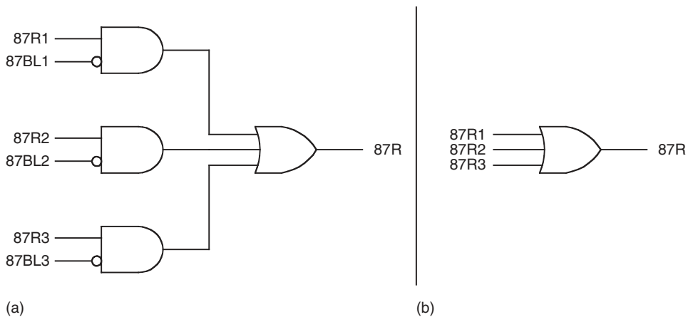
FIGURE 18.9 Three-phase differential relay with: (a) Independent harmonic blocking and (b) Independent harmonic restraint.
