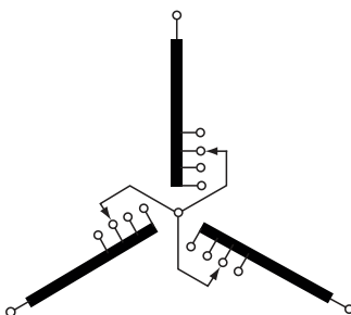
FIGURE 13.22 LTC with wye-connected windings.
