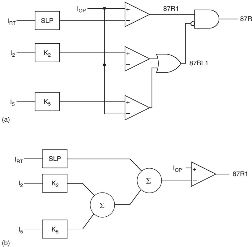
FIGURE 18.8 Two approaches to a differential element. (a) Harmonic blocking and (b) Harmonic restraint.
