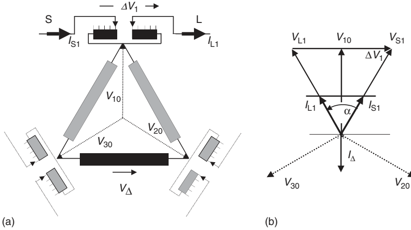
FIGURE 4.8 Single core symmetrical PST.
