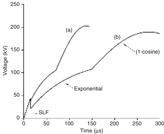
FIGURE 10.40 Typical TRV capability envelopes for 123 kV class circuit breaker at (a) 60% and (b) 100% of rated fault current.
