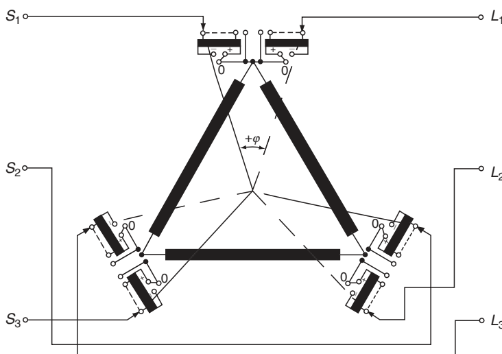
FIGURE 13.25 Phase-shifting transformer—direct circuit arrangement.
