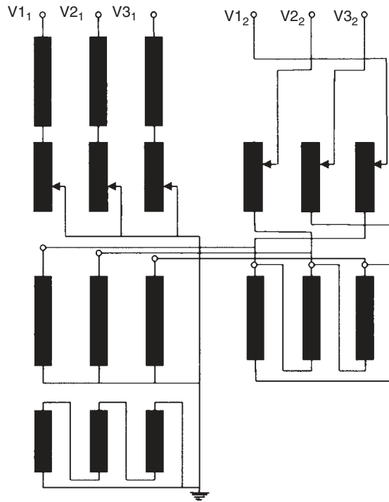
FIGURE 4.13 Quadrature booster—simplified connection diagram.
