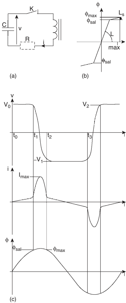
FIGURE 9.21 (a) Schematic diagram. (b) Simplified characteristic \Phi(i) . (c) Voltage V , current i and flux \Phi as a function of time.
