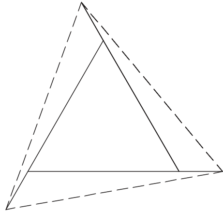
FIGURE 5.16 Extended delta-winding shift.
