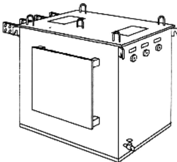
FIGURE 3.17 Three-phase vault. (By permission of Pacific Gas and Electric Company, San Francisco, CA.)
