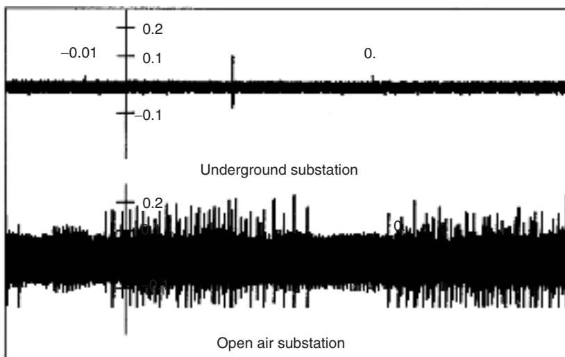
FIGURE 23.1 Electric PD measurements on transformers in underground and open-air substations. The overhead transmission lines cause a multitude of signals, making a PD measurement very insensitive. Underground stations are generally fed by cables that attenuate the high-frequency signals from the network, and PD measurements are quite sensitive. Horizontal scale in seconds, vertical scale in mV.
