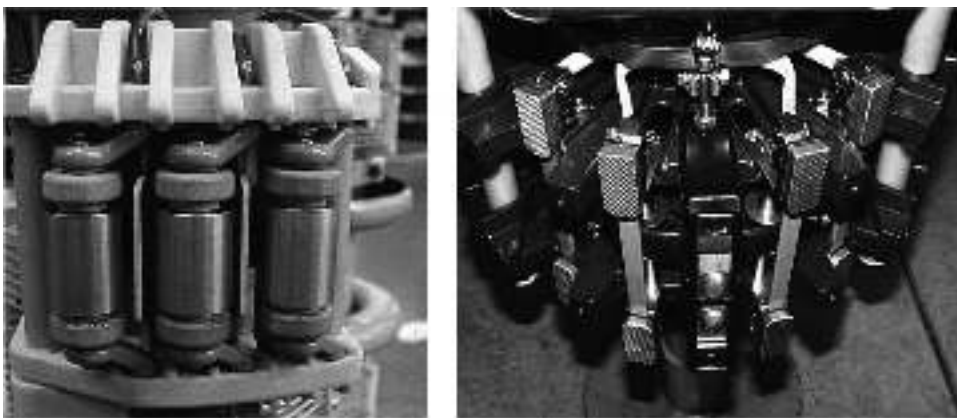
FIGURE 13.9 LTCs with tungsten-copper arcing contact system for mineral transformer oil (different scales). (Photo courtesy of Maschinenfabrik Reinhausen GmbH.)
