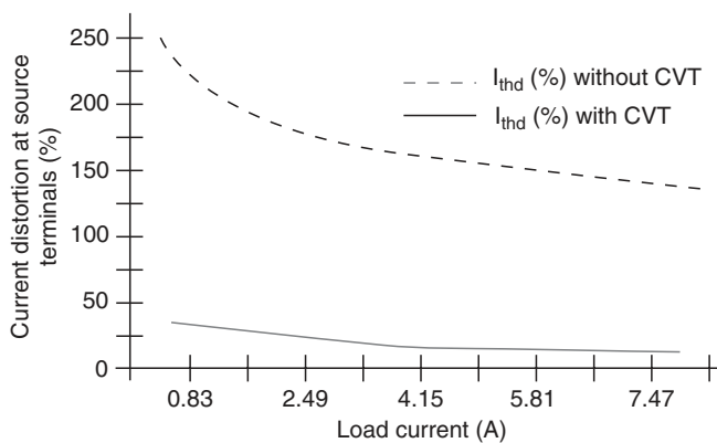
FIGURE 9.16 Line-current distortions for a nonlinear load.
