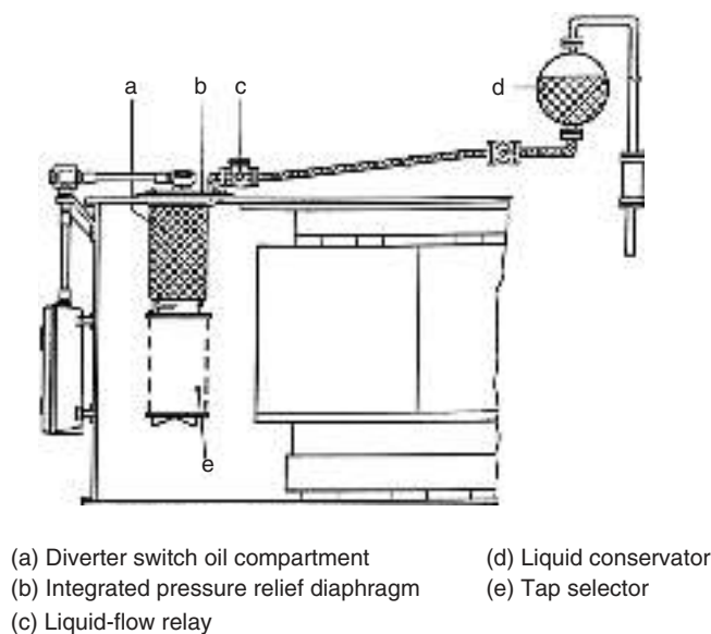
FIGURE 13.33 Arrangements of protection devices of internally mounted LTCs.
