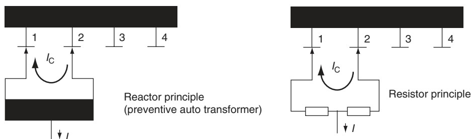
FIGURE 13.4 Basic switching principle “make (2) before break (1)” using transition impedances.
