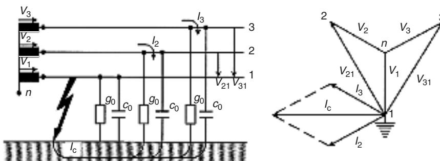
FIGURE 10.12 Single line-to-ground fault in nongrounded system.
