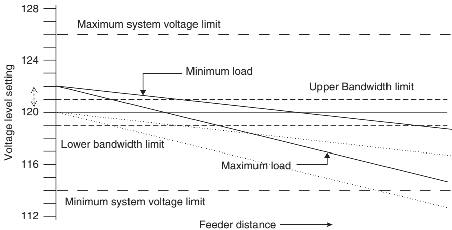
FIGURE 8.28 Voltage profile using voltage-level setting without LDC.
