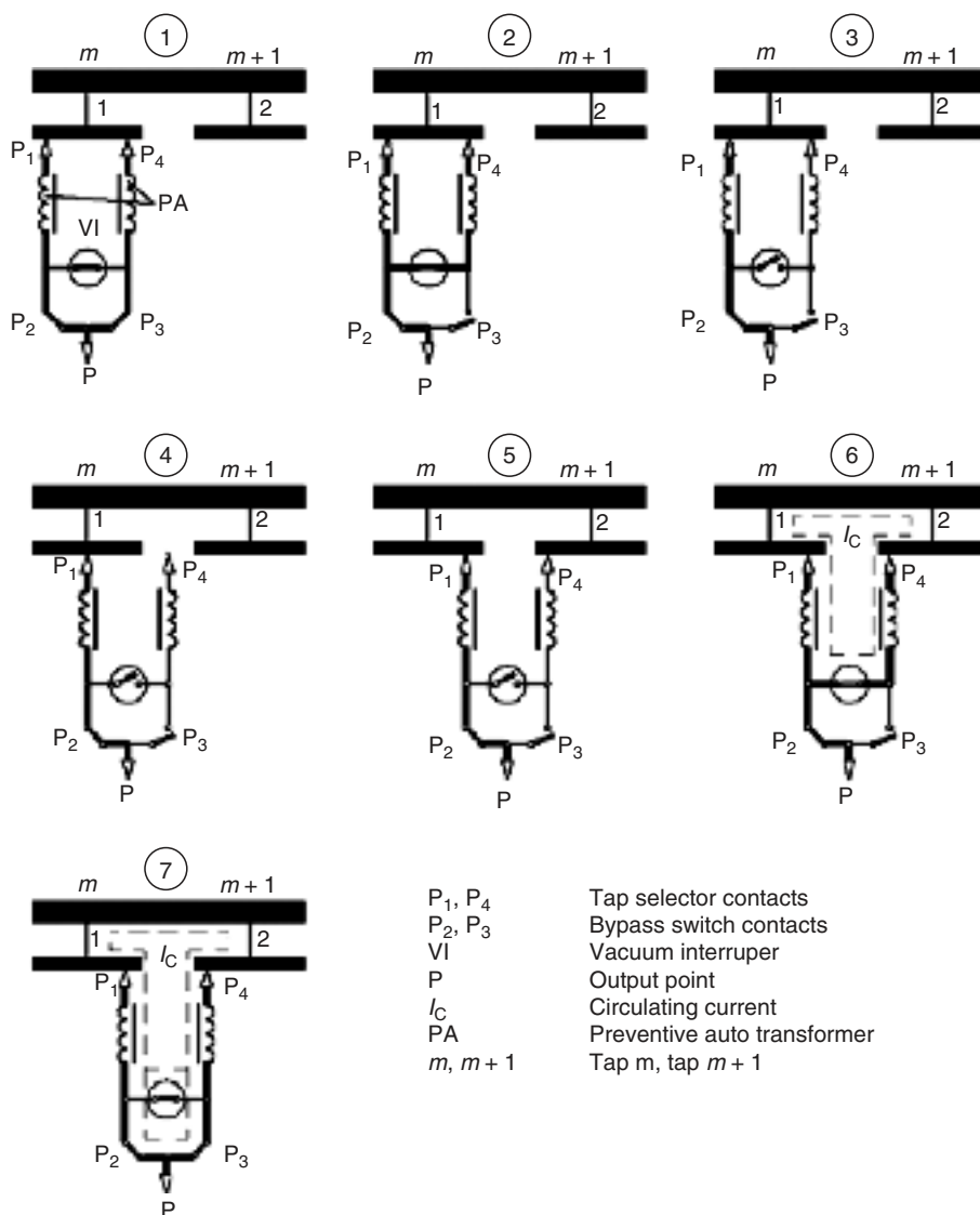
FIGURE 13.18 Switching sequence of reactor-type LTC with one vacuum interrupter per phase from nonbridging to bridging position.
