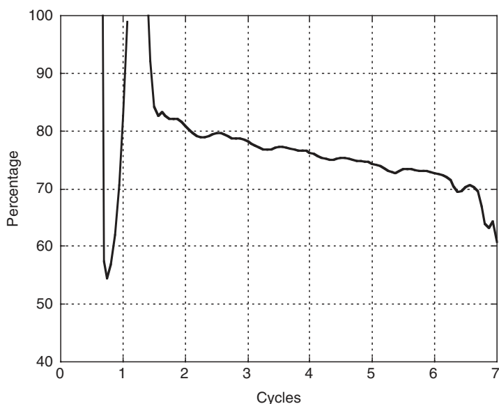
FIGURE 18.30 DC content of the differential current for Case 3.
