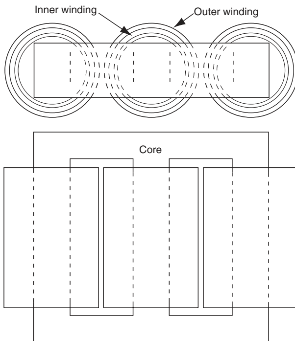
FIGURE 2.4 Schematic of three-phase core-form construction.
