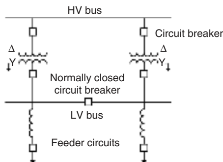
FIGURE 10.5 Typical phase reactor connection.
