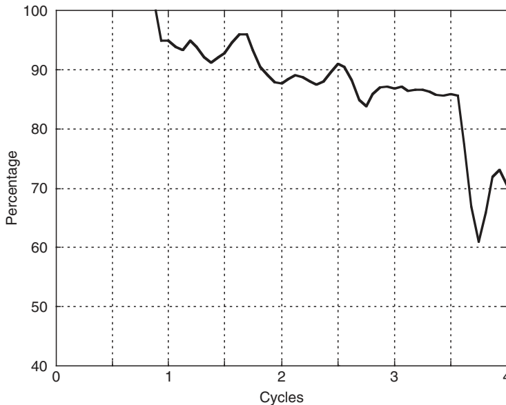
FIGURE 18.26 DC content of the differential current for Case 2.
