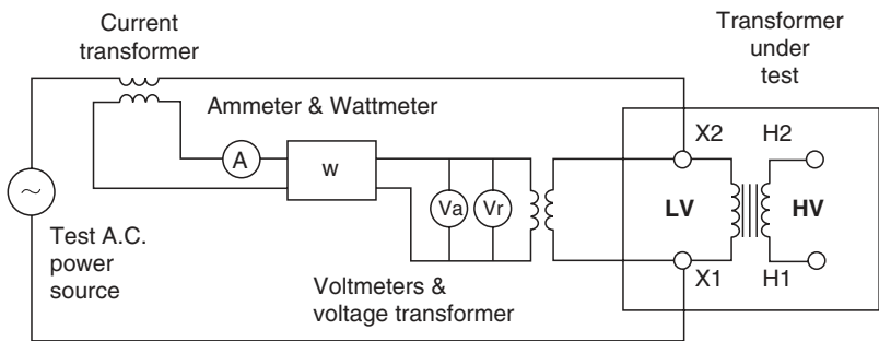
FIGURE 16.14 Test circuit for no-load-loss measurement.
