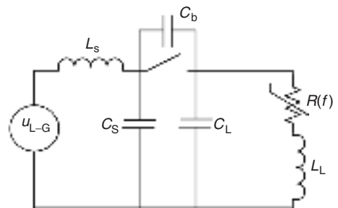
FIGURE 10.39 Single-phase equivalent circuit for a star connected and solidly grounded shunt reactor bank, where L_L is the reactor reactance (for gapped iron-core shunt reactor, manufacturer should be consulted to obtain the core saturation level at high transient frequencies and thus the resultant inductance; for air-core shunt reactors the inductance can always be considered a constant value equal to the 60 Hz rated value); C_L is the equivalent capacitance at the reactor side of the C_b ; R(f) is the reactor frequency dependent resistance; L_s is the system equivalent reactance; C_b is the equivalent capacitance across the breaker terminals; C_s is the system equivalent capacitance; and u_{L-G} = System line-to-ground voltage.
