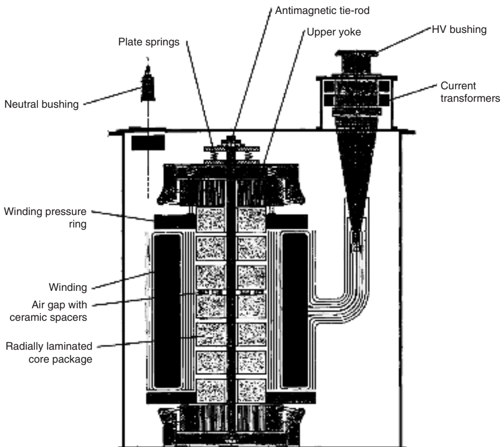
FIGURE 10.3 Gapped iron-core oil-immersed reactor.
