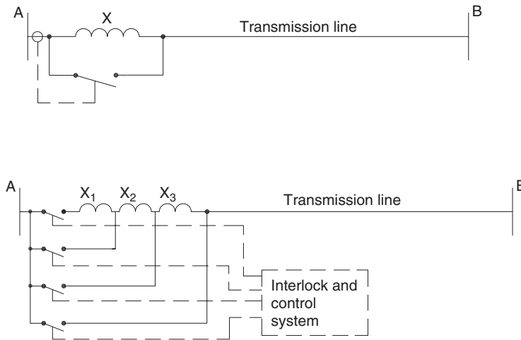
FIGURE 10.23 Switchable power control reactor (top); tapped switchable power control reactor (bottom).
