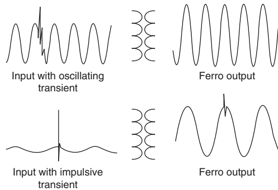
FIGURE 9.14 Output voltages resulting from oscillating and impulsive transients in the input voltages.
