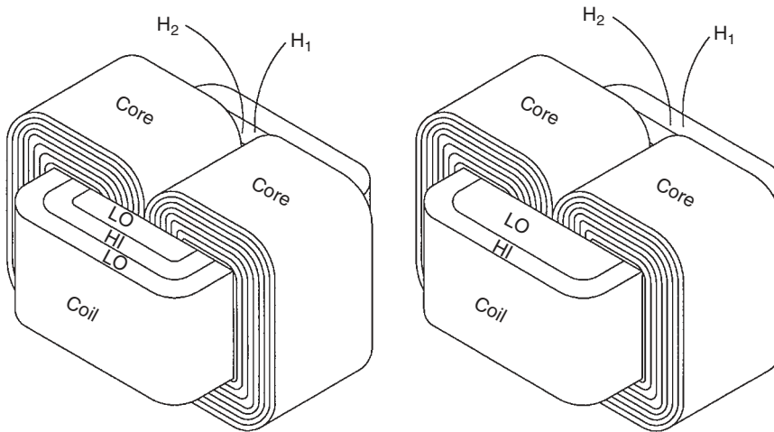
FIGURE 3.8 LO-HI-LO and LO-HI configurations. (By permission of ABB Inc., Jefferson City, MO.)
