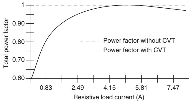
FIGURE 9.17 Power factor for a linear load.
