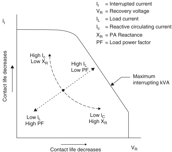
FIGURE 8.21 Tap-changer interruption envelope.
