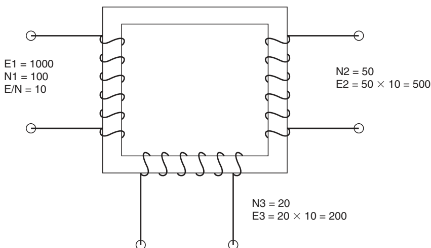
FIGURE 1.6 Steel core with windings.
