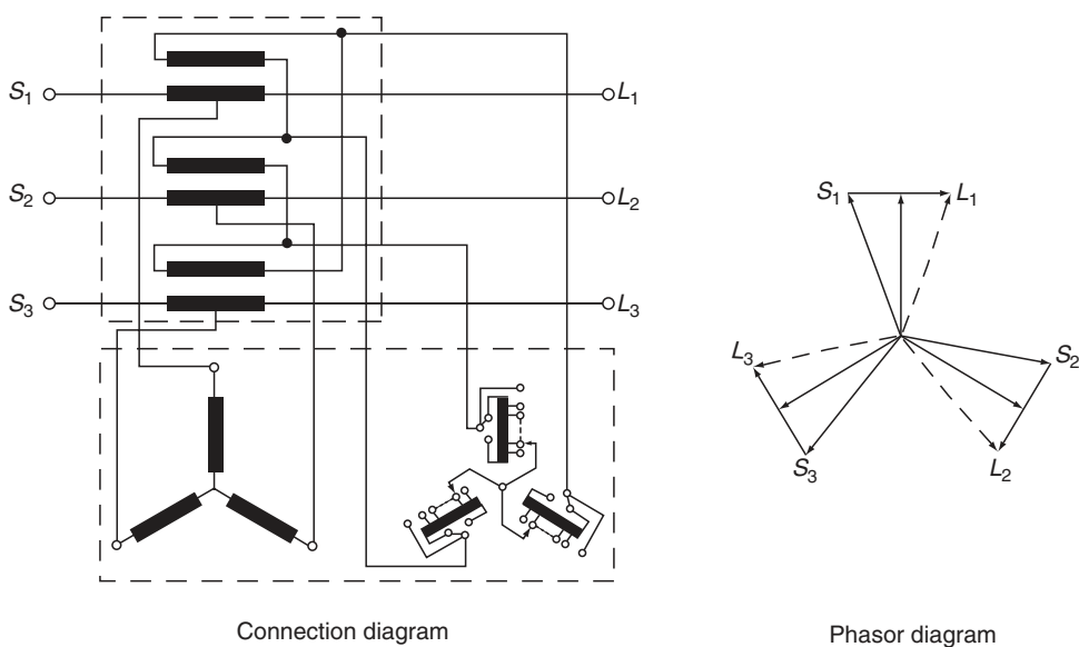
FIGURE 13.26 Phase-shifting transformer—intermediate circuit arrangement.
