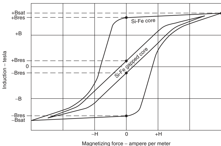
FIGURE 7.16 Typical B-H curve for Si-Fe steel.
