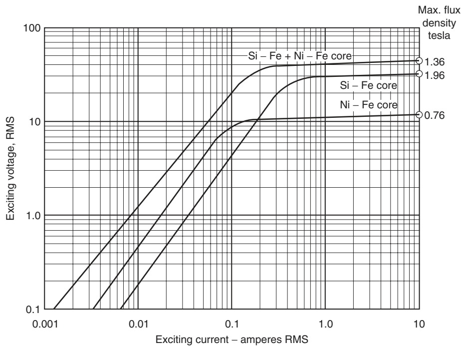
FIGURE 7.4 Typical composite core.
