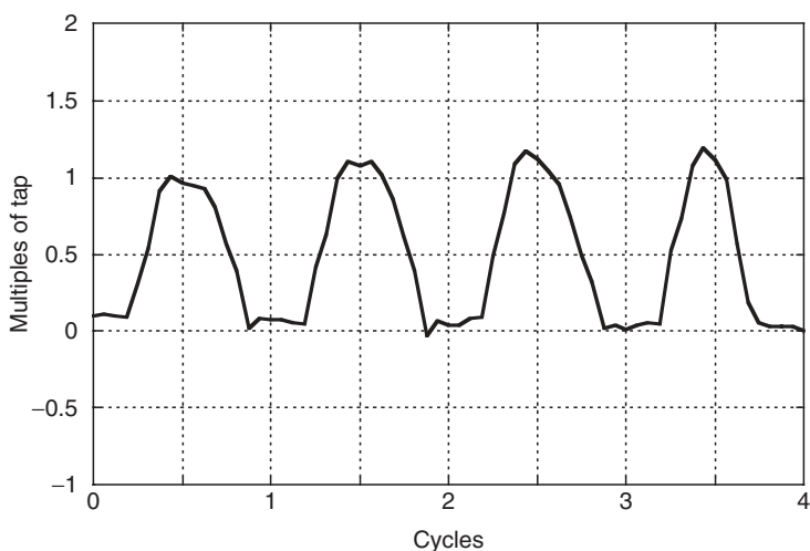
FIGURE 18.24 Differential current during transformer energization with the power transformer loaded.
