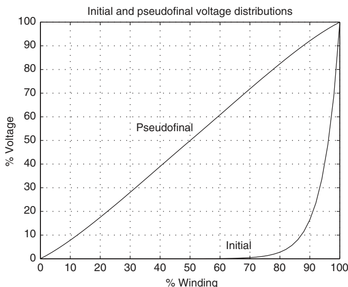
FIGURE 20.3 Initial and pseudo-final voltage distribution.
