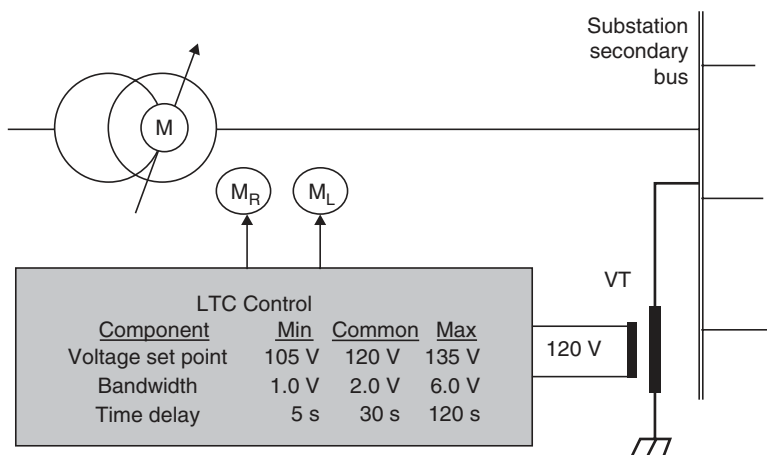
FIGURE 17.3 Control for voltage regulation of the bus.
