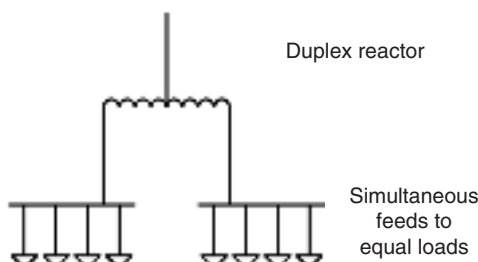
FIGURE 10.14 Typical duplex reactors connections.
