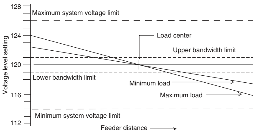
FIGURE 8.29 Voltage profile using voltage-level setting with LDC.
