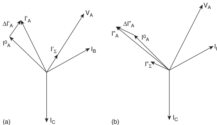
FIGURE 23.5 Analysis of bushing sum currents: (a) change in current phasor due to change in power factor of bushing A; (b) change in current phasor due to change in capacitance of bushing A.
