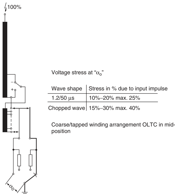
FIGURE 13.34 Voltage stress between selected and preselected tap of coarse/tapped winding arrangement, LTC in mid-position.
