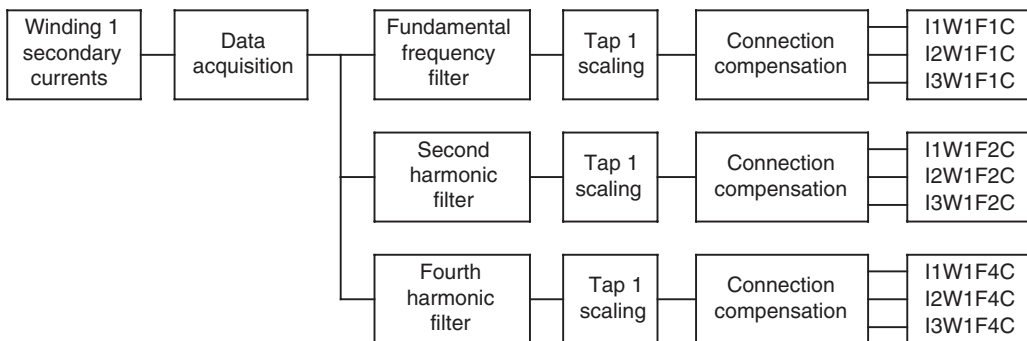
FIGURE 18.12 Data acquisition, filtering, scaling, and compensation for Winding 1 currents.
