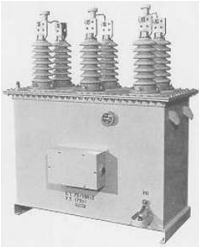
FIGURE 7.30 34.5-kV three-phase oil-filled metering unit. (Photo courtesy of Kuhlman Electric Corp.)
