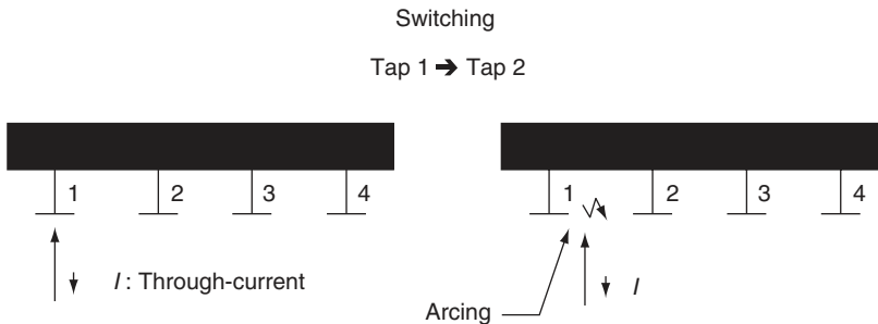
FIGURE 13.3 Loss of system load with single contact switching.
