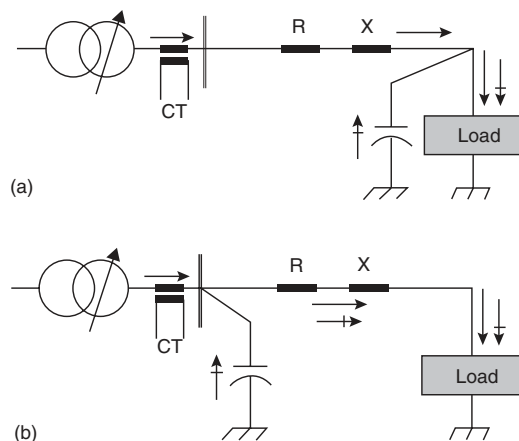
FIGURE 17.6 (a) Feeder with power-factor-correction capacitors, capacitors at the load. (b) Feeder with power-factor-correction capacitors, capacitors at the source bus.
