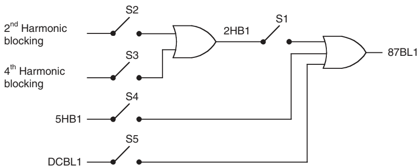
FIGURE 18.16 Differential-element blocking logic.
