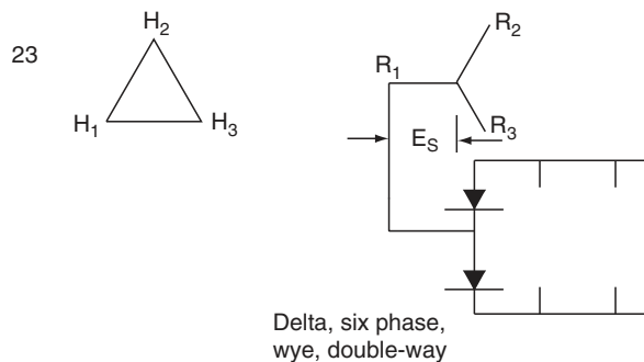
FIGURE 5.1 ANSI Circuit 23. (From ANSI/IEEE C57.18.10-1998. © IEEE 1998. With permission.)
