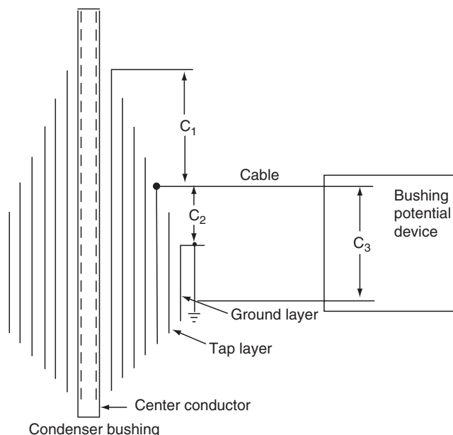
FIGURE 12.8 Bushing potential device.
