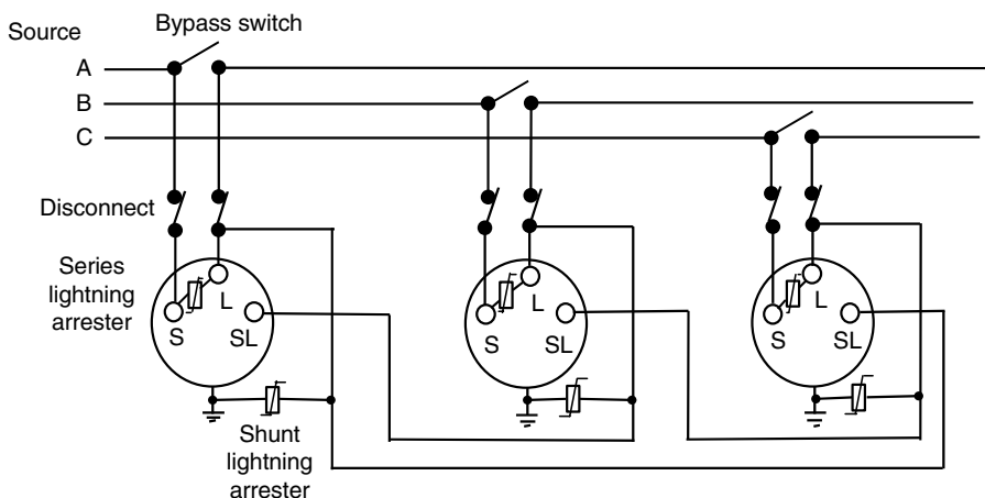
FIGURE 8.9 Connection of three voltage regulators in a three-phase, three-wire delta circuit.
