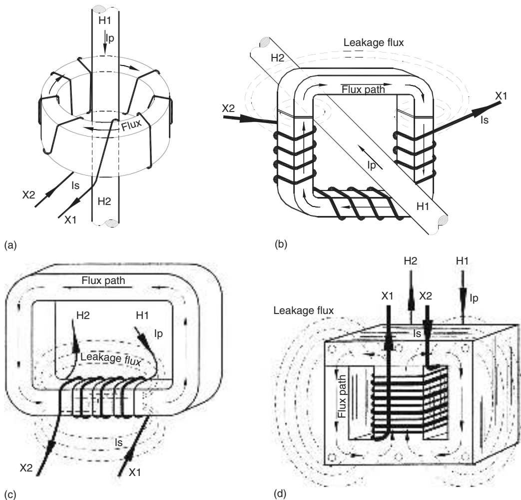
FIGURE 7.5 Typical core and winding arrangements. (a) Tape-wound toroidal core with fully distributed winding. Note the absence of leakage flux, which exists but is considered to be negligible. Sensitivity to primary-conductor position is also negligible. The primary can also consist of several turns. (b) Cut core with winding partially distributed. Leakage flux, in this case, depends on the location of the primary conductor. As the conductor moves closer to the top of the core, the leakage flux increases. (c) Distributed-gap core with winding distributed on one leg only. This type has high leakage flux but good coupling, since the primary and secondary windings occupy the same winding space. (d) Laminated "EI" core, shell-type. This type has high leakage flux, since a major portion of magnetic domains are against the direction of the flux path. The orientation is not all in the same direction, as it is with a tape-wound core.
