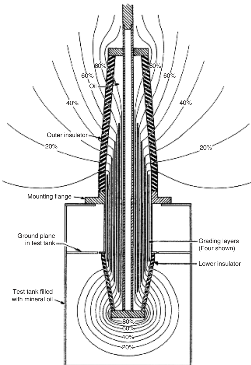
FIGURE 12.3 Exponential plot of oil-filled, capacitance-graded bushing.
