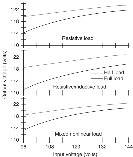
FIGURE 9.10 Output-voltage regulation with varying input ac voltage.
