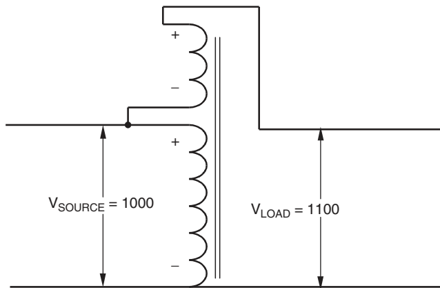
FIGURE 8.13 Step-up autotransformer.
