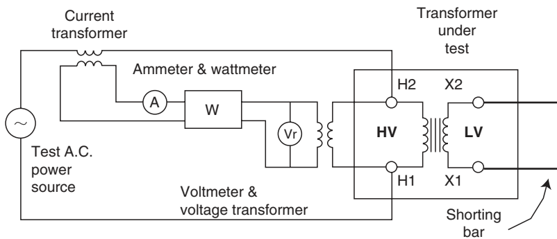
FIGURE 16.15 Test circuit for load-loss measurement.
