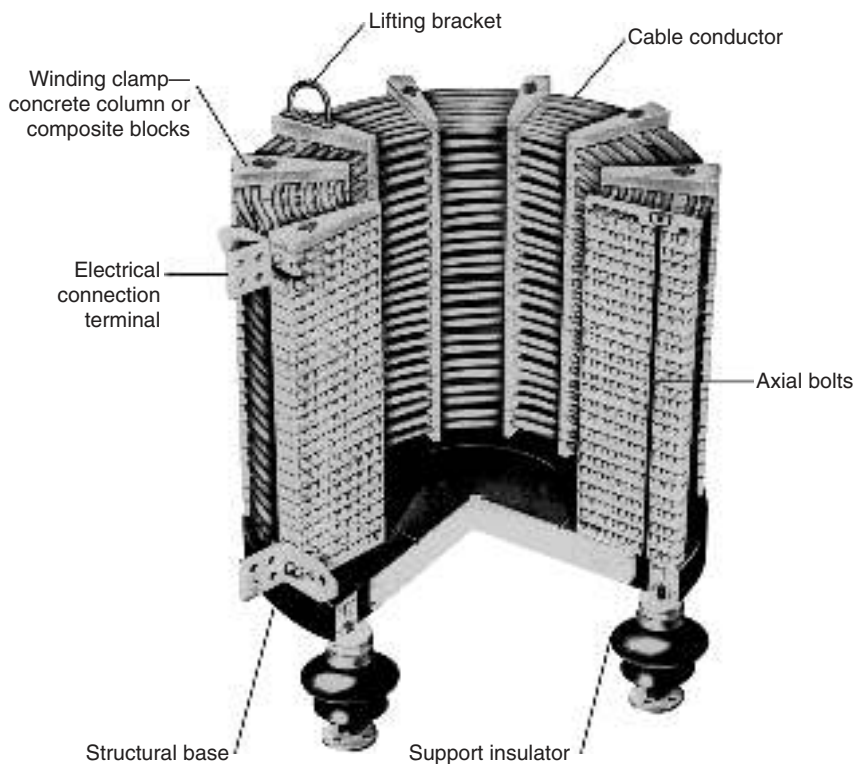
FIGURE 10.1 Open style reactor.
