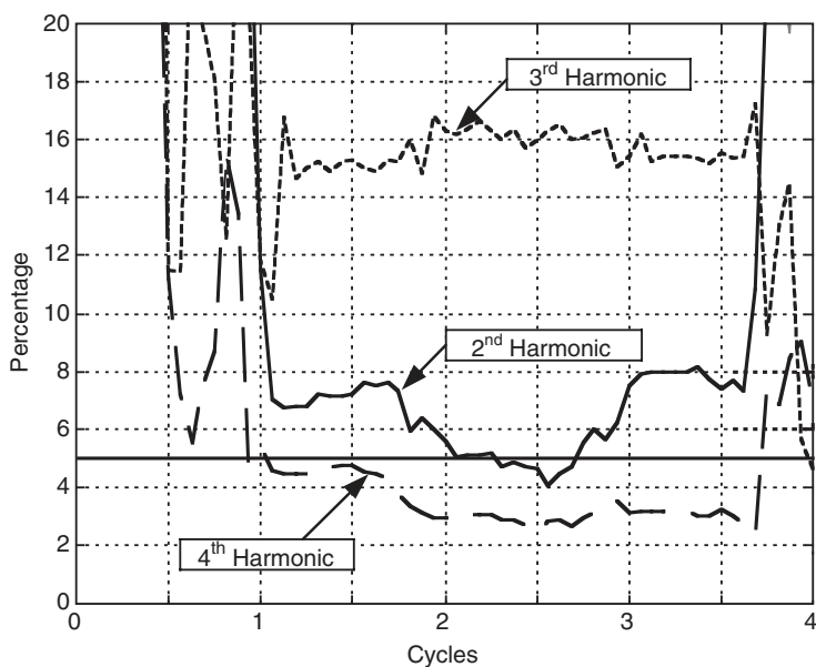
FIGURE 18.20 Second, third, and fourth harmonic as percentages of fundamental of the inrush current where the third-harmonic content is greater than the even-harmonic content.
