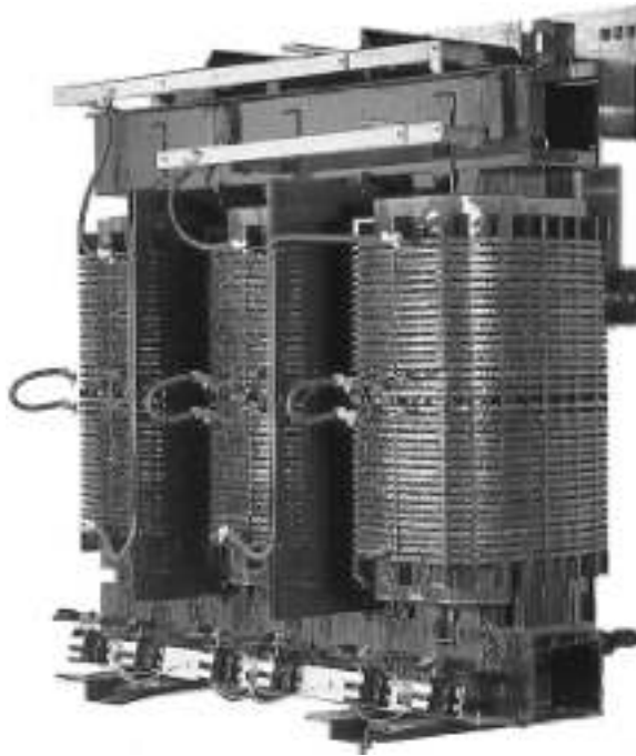
FIGURE 6.2 Three-phase 1500-kVA dry-type transformer, 15-kV-class primary, 600-V secondary. Three cooling fans can be seen on the base, below the coils. (Photo courtesy of ABB.)
