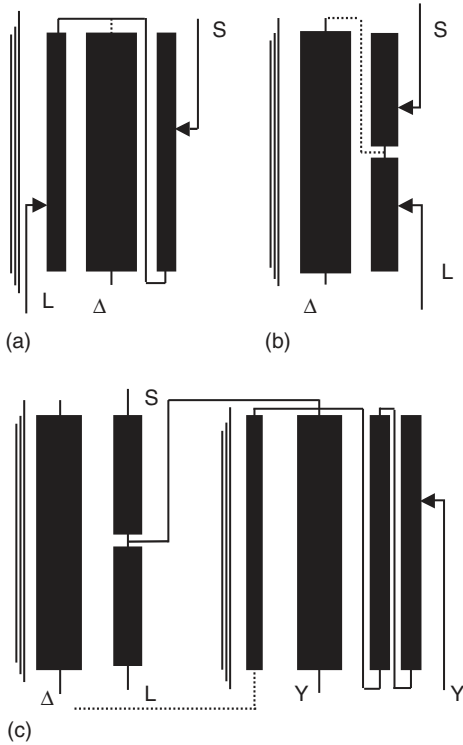
FIGURE 4.15 Winding arrangements.
