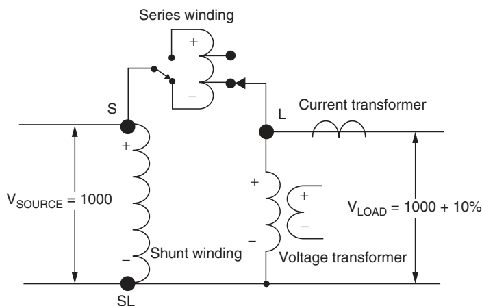
FIGURE 8.23 Voltage regulation on the load side (Type A).
