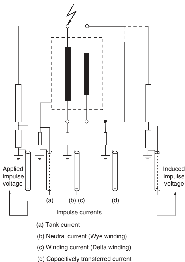
FIGURE 16.9 Impulse-current measurement locations.
