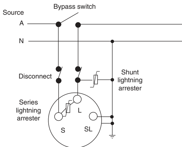
FIGURE 8.3 Voltage regulator connection in a single-phase circuit.
