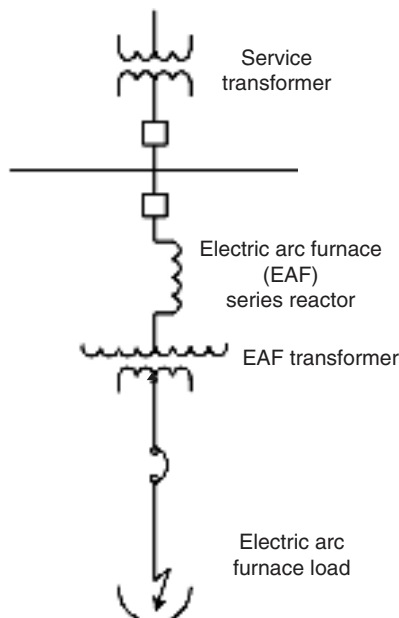
FIGURE 10.31 Typical electric arc furnace series reactor connection.
