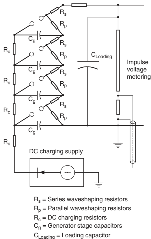
FIGURE 16.5 Marx generator with four stages.
