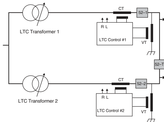
FIGURE 17.8 LTC transformers in parallel with no interconnections.
