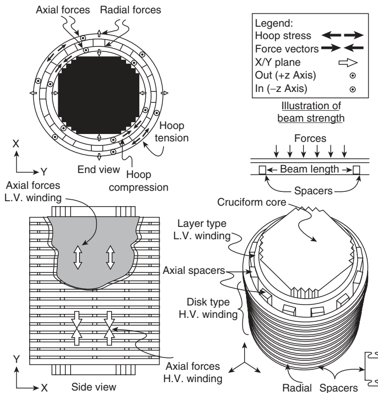
FIGURE 22.1 Concentric circular winding. (From IEEE Guide for Failure Investigation, Documentation, and Analysis for Power Transformers and Shunt Reactors, C57.125–1991. © 1991 IEEE. With permission.)
