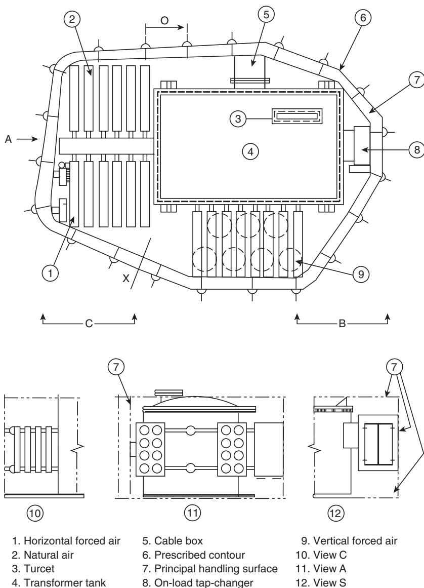
FIGURE 19.2 Typical microphone positions for sound measurement on transformers having cooling auxiliaries mounted either directly on the tank or on a separate structure spaced <3 m from the principal radiating surface of the main tank. (From IEC 60076-10. With permission.)
