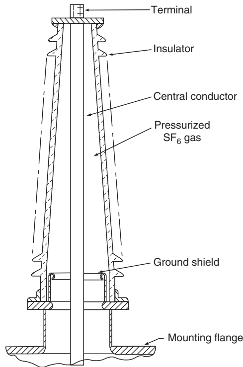
FIGURE 12.4 Pressurized SF 6 gas bushing.
