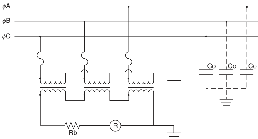
FIGURE 7.11 VTs wye-connected on ungrounded system.
