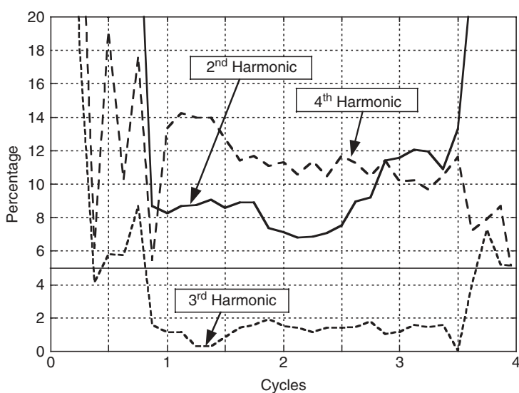
FIGURE 18.25 When the loaded transformer is energized with reduced voltage, the fourth harmonic provides information to restrain or block the differential element.
