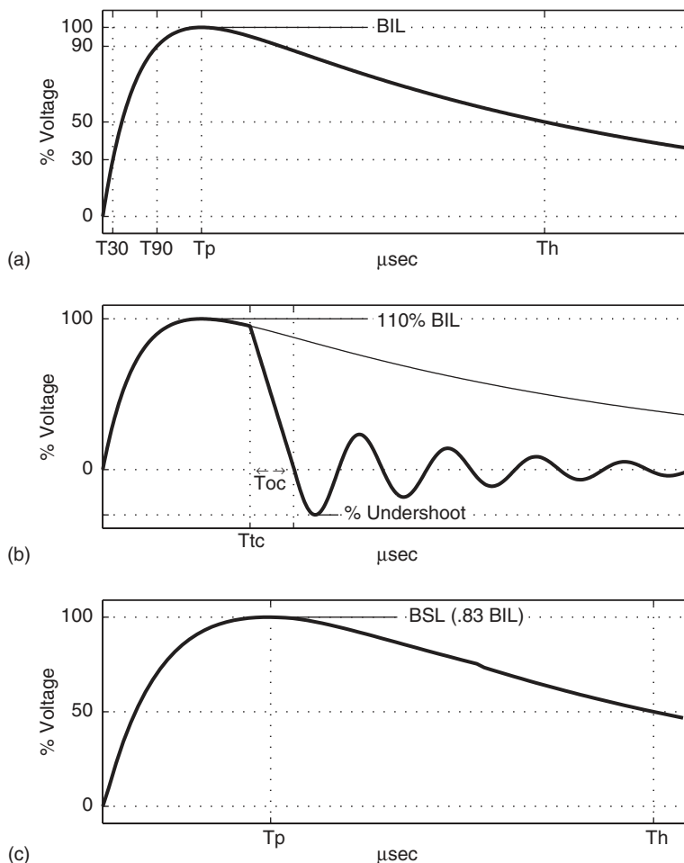
FIGURE 20.8 Standard voltage waveforms for impulse tests: (a) full, (b) chopped, and (c) switching surge.
