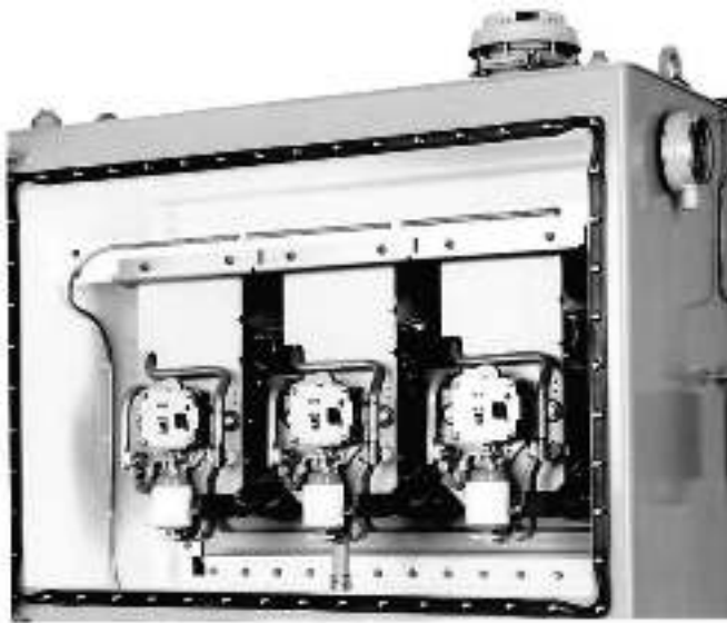
FIGURE 13.11 Reactor vacuum-type LTC with one vacuum interrupter per phase. (Photo courtesy of Maschinenfabrik Reinhausen GmbH.)
