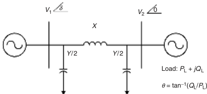
FIGURE 10.38 Transmission system \pi equivalent circuit.
