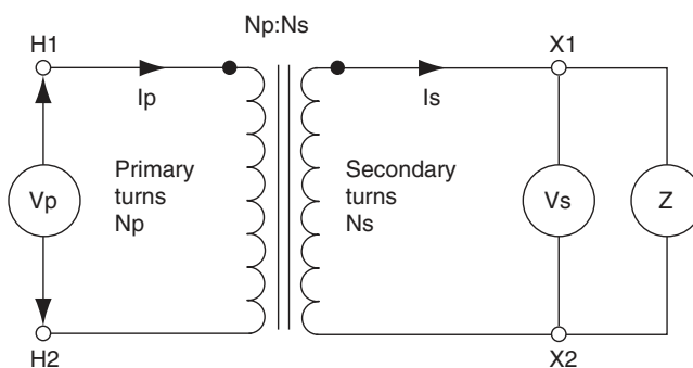
FIGURE 7.2 Ideal transformer.
