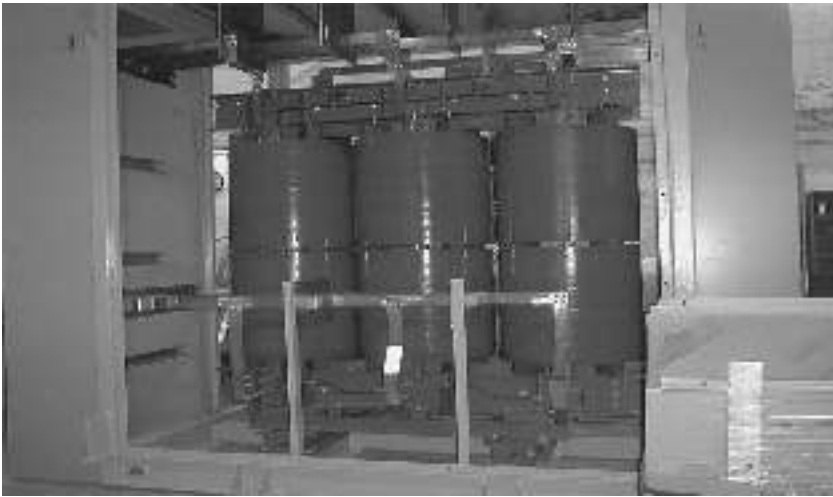
FIGURE 5.19 A 12-pulse Circuit 31 5450-kVA, 4160-V delta primary to 2080-V delta and wye secondaries, cast-coil transformer in case. (Photo courtesy of Niagara Transformer Corp.)
