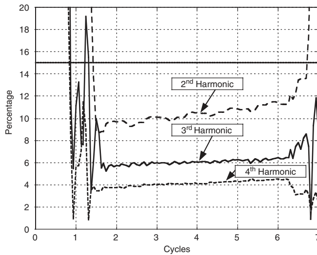
FIGURE 18.29 Second-harmonic percentage drops to approximately 9%.
