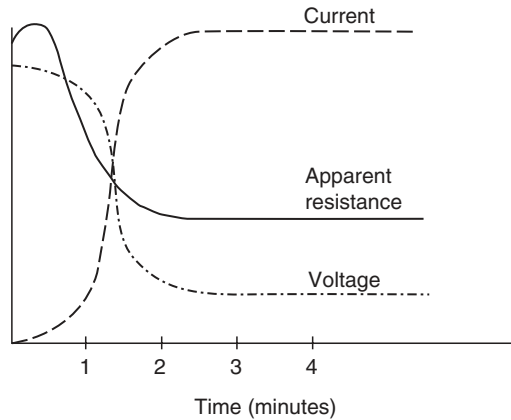
FIGURE 16.18 Trend of current, voltage, and apparent resistance with time.
