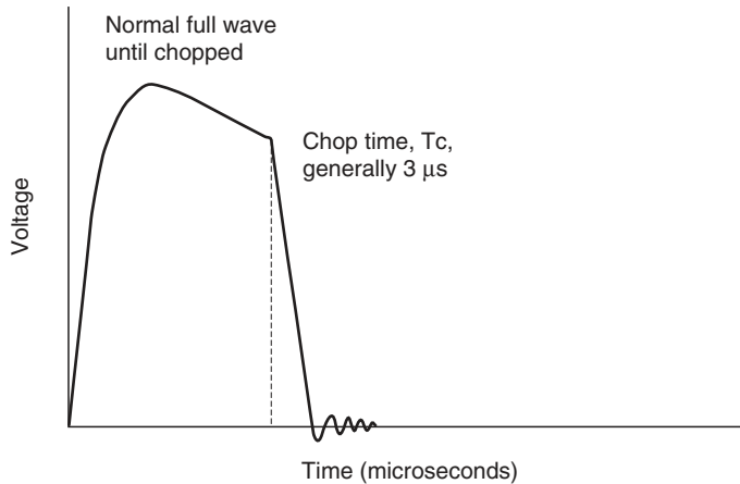
FIGURE 16.4 Standard chopped-wave lightning impulse.
