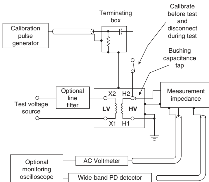
FIGURE 16.13 Test circuit for partial-discharge measurement during the induced-voltage test.
