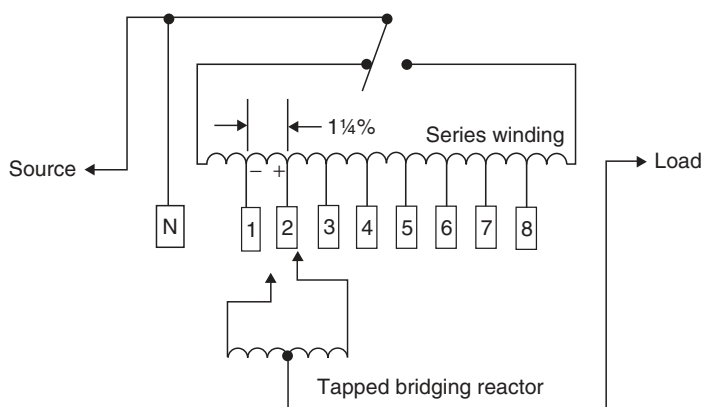
FIGURE 8.18 One movable contact on stationary contact (asymmetrical position).
