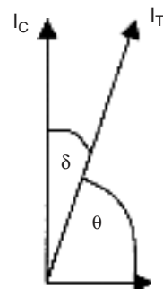
FIGURE 23.2 Power-factor graphical representation.
