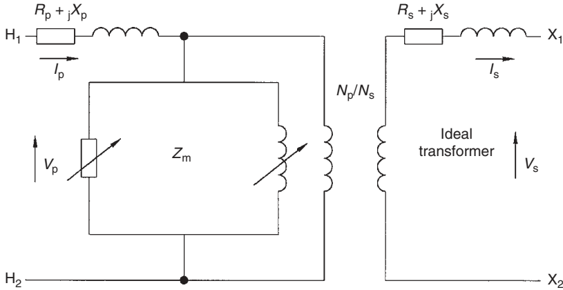
FIGURE 3.37 Complete transformer equivalent circuit. (By permission of ABB Inc., Jefferson City, MO.)
