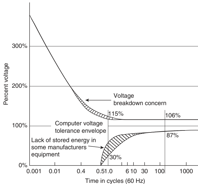
FIGURE 9.6 Voltage-tolerance envelope specified by the Computer and Business Equipment Manufacturers Association. Note: This is reproduced from IEEE Std. 446 (Orange Book).
