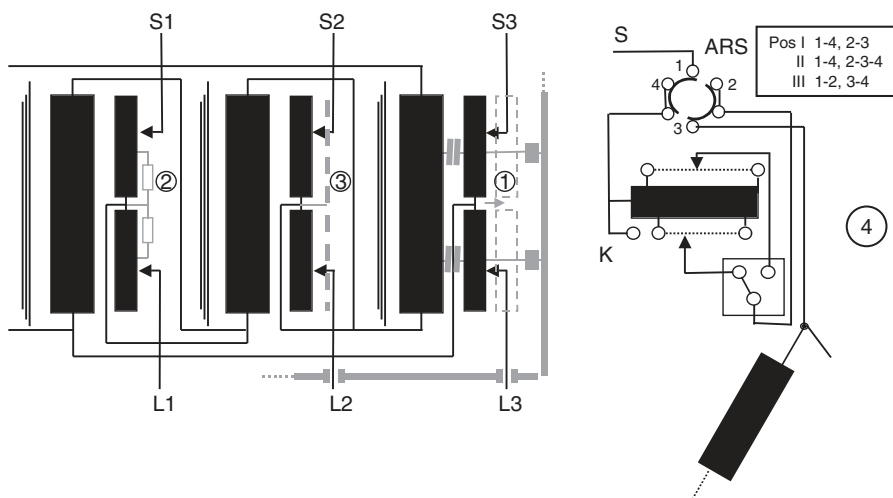
FIGURE 4.18 Control of the tap-winding potential during changeover selector operation.
