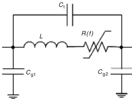
FIGURE 10.41 Reactor model for TRV studies where C_{g1} and C_{g2} are the stray capacitance of reactor terminals to ground; C_t , terminal to terminal stray capacitance; L , reactor inductance; R(f) , reactor frequency dependent resistance.
