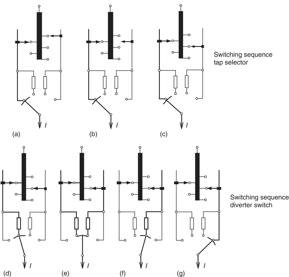
FIGURE 13.6 Switching sequence of tap selector—diverter switch (arcing switch).
