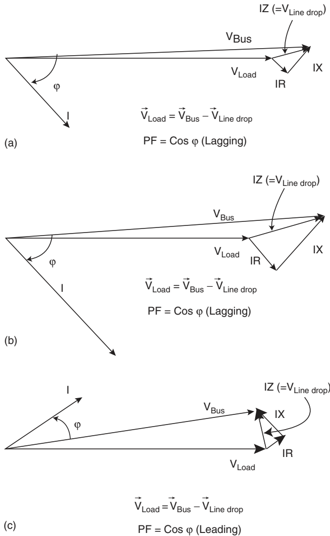
FIGURE 17.5 (a) Load phasor diagram, normal load, lagging power factor. (b) Load phasor diagram, heavy load, lagging power factor. (c) Load phasor diagram, normal load, leading power factor.
