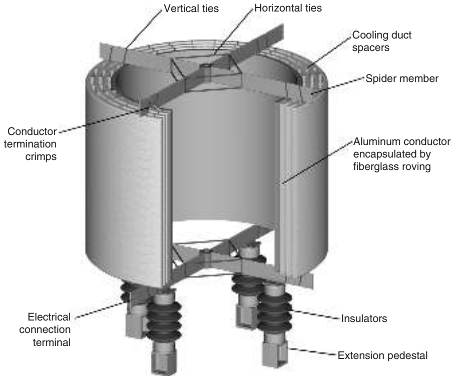
FIGURE 10.2 Modern fully encapsulated reactor.
