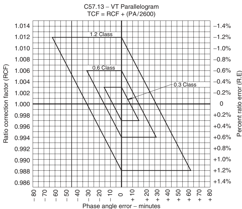
FIGURE 7.7 Accuracy coordinates for VTs.
