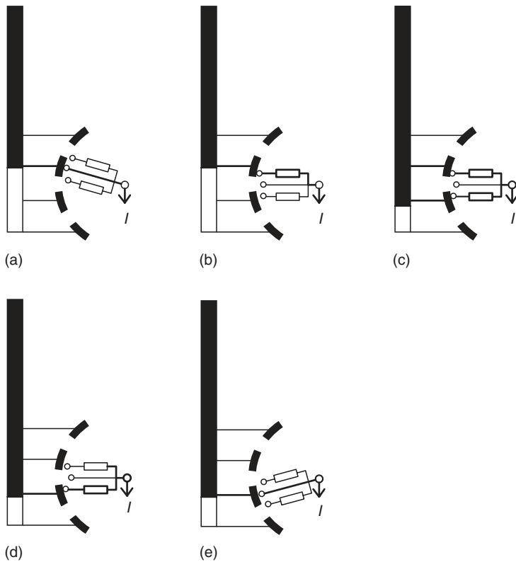
FIGURE 13.8 Switching sequence of selector switch (arcing tap switch.)
