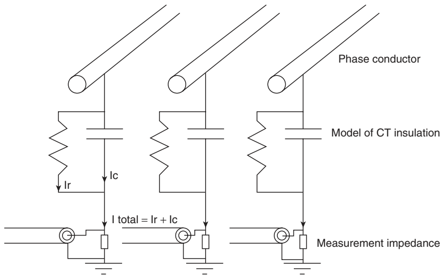
FIGURE 23.3 Schematic representation of relative tan delta measurements.
