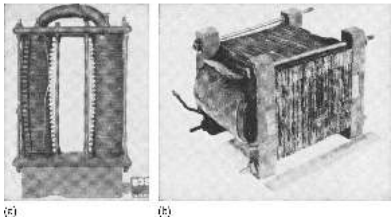
FIGURE 3.1 (a) Gaulard and Gibbs transformer; (b) William Stanley’s early transformer. (By permission of ABB Inc., Raleigh, NC.)
