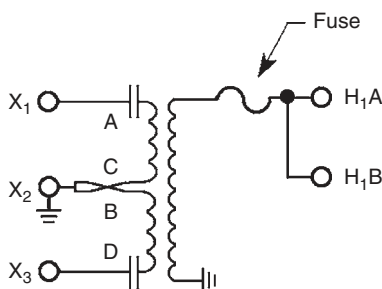
FIGURE 3.19 Two-primary bushing. (By permission of Pacific Gas and Electric Company, San Francisco, CA.)
