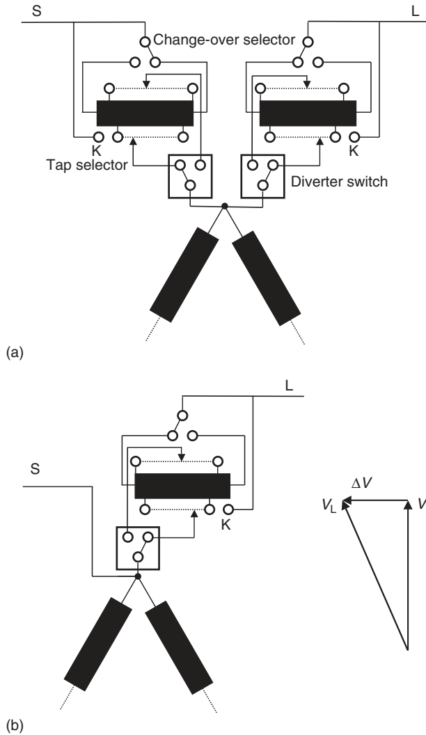
FIGURE 4.9 (a) Single-core symmetrical PST (b) Single-core unsymmetrical PST.
