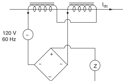
FIGURE 7.25 Standard two-element connection.
