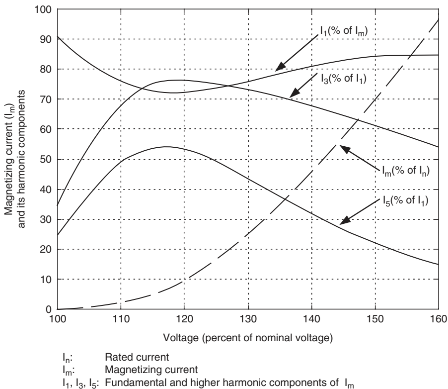
FIGURE 18.4 Harmonic content of transformer exciting current as a function of the applied voltage. (From Cooper Power Systems, Electric Power System Harmonics: Design Guide , Cooper Power Systems, Bulletin 87011, Franksville, WI, 1990. With permission.)
