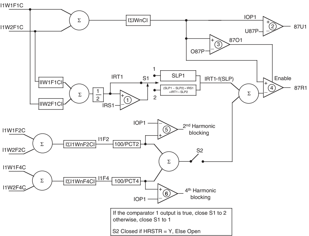
FIGURE 18.13 Even-harmonic restraint, 87R1, and unrestraint, 87U1, differential elements.
