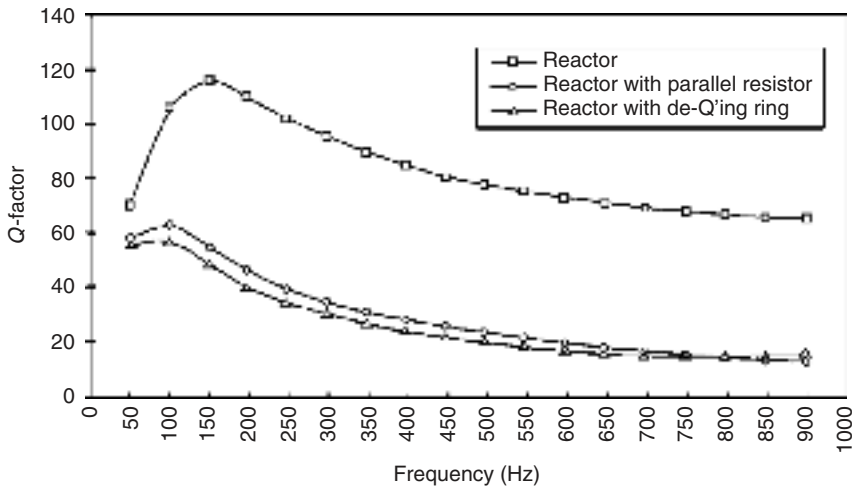
FIGURE 10.47 Graph of Q vs. frequency for natural Q-filter reactor, a filter reactor plus parallel resistor, and a filter reactor with a de-Q'ing ring system.
