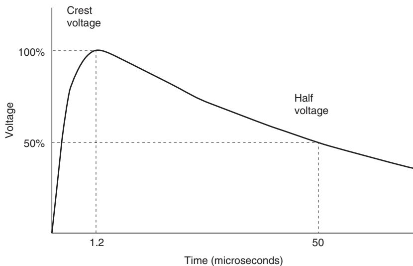
FIGURE 16.3 Standard full-wave lightning impulse.
