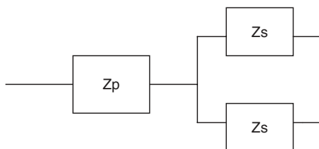
FIGURE 5.13 Impedance diagram of a three-winding transformer.
