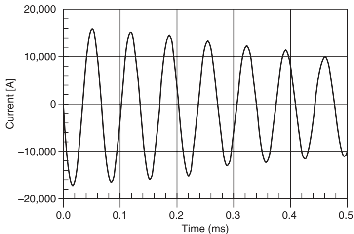
FIGURE 10.16 Back-to-back current in the first pole to close of bank number 2 circuit breaker.
