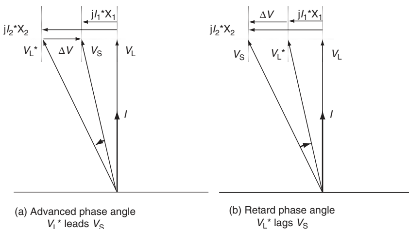
FIGURE 4.3 No-load voltage diagram of parallel systems.
