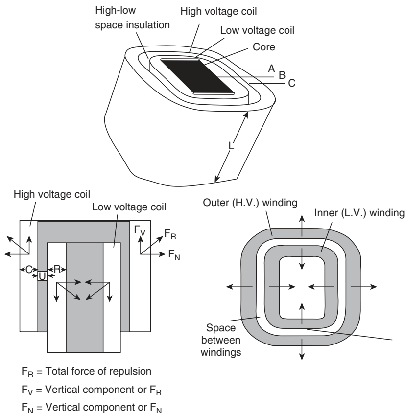
FIGURE 22.2 Rectangular winding. (From IEEE Guide for Failure Investigation, Documentation, and Analysis for Power Transformers and Shunt Reactors, C57.125–1991. © 1991 IEEE. With permission.)
