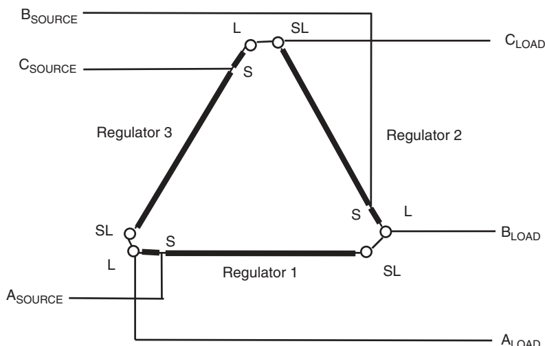
FIGURE 8.11 Power connection of closed-delta-connected voltage regulators.
