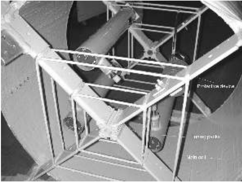
FIGURE 10.52 Internal view of line trap showing tuning device and protective device.
