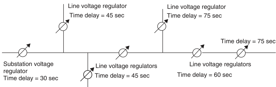
FIGURE 8.27 Cascading single-phase voltage regulators.
