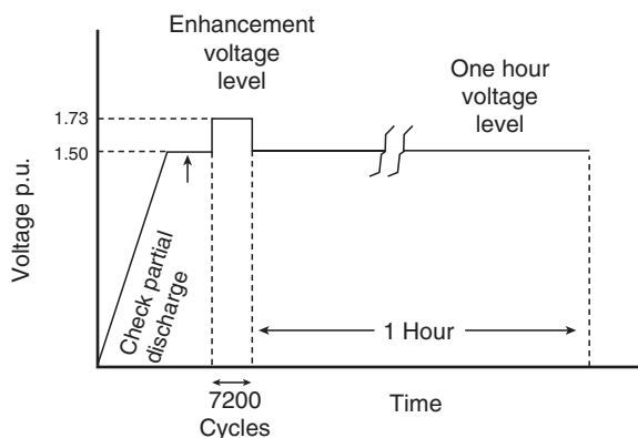
FIGURE 16.12 Induced-voltage test for Class II power transformers.
