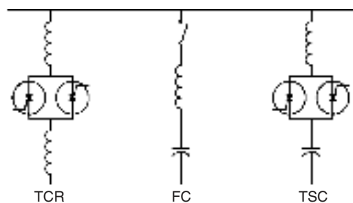
FIGURE 10.26 Static VAR compensator.
