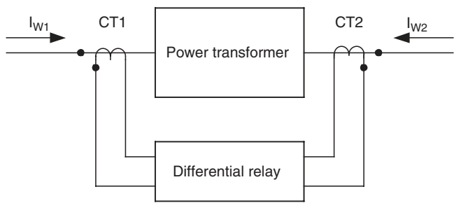
FIGURE 18.1 Typical differential-relay connection diagram.
