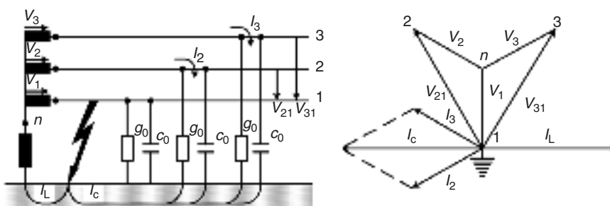
FIGURE 10.13 Single line-to-ground fault in resonant-grounded system.
