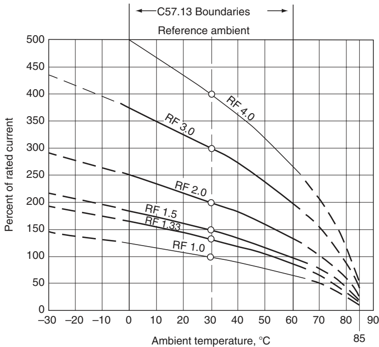
FIGURE 7.15 CT derating chart.
