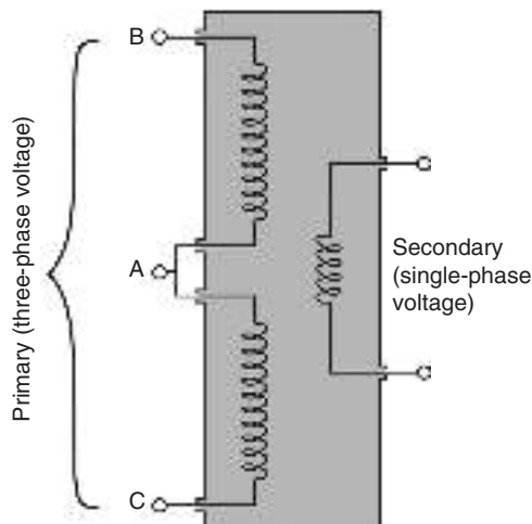
FIGURE 9.19 Schematic of a ride-through transformer.
