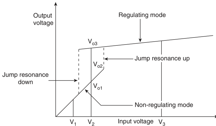
FIGURE 9.5 Output voltage vs. input voltage for constant-voltage transformer with jump resonance.
