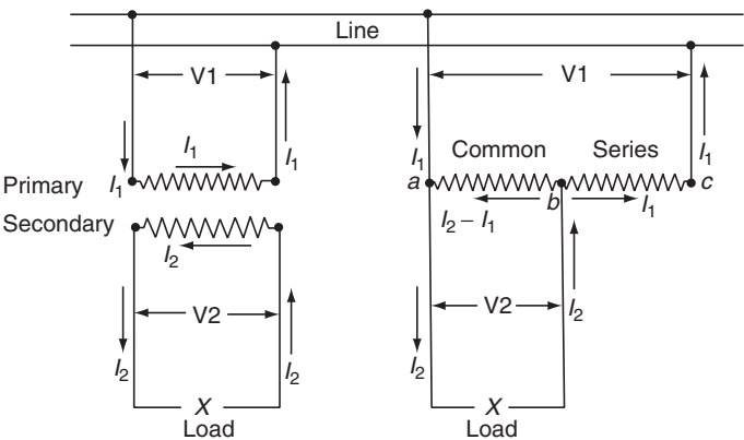
FIGURE 15.3 Current flow in double-wound transformer and autotransformer.
