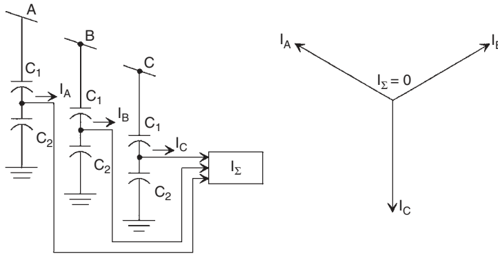
FIGURE 23.4 Bushing sum-current measurements.
