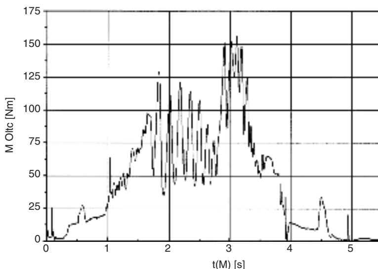
FIGURE 23.6 Sample torque curve.
