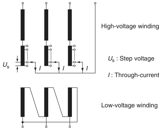
FIGURE 13.2 Principle winding arrangement of a regulating transformer in wye connection.
