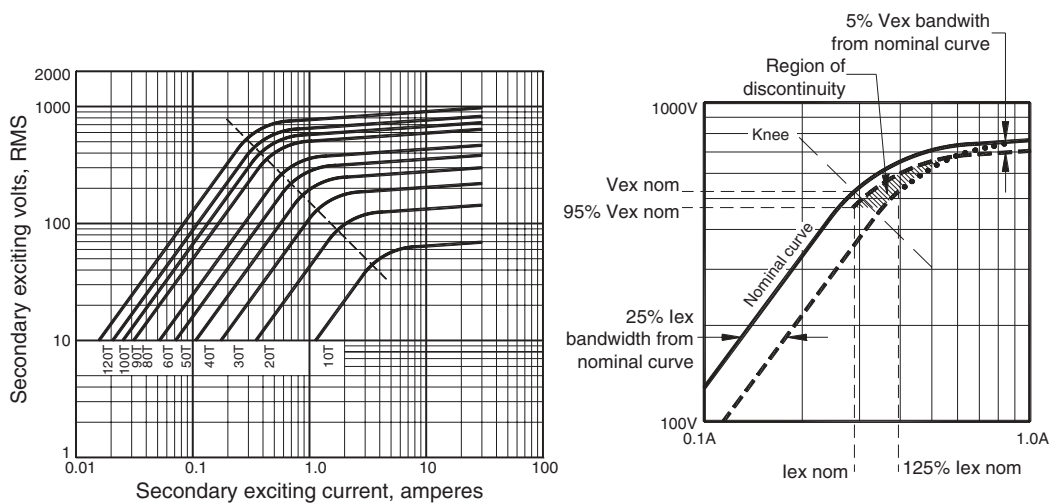
FIGURE 7.14 (Left) Saturation curve for a multiratio CT; (right) Saturation curve discontinuity of tolerances.
