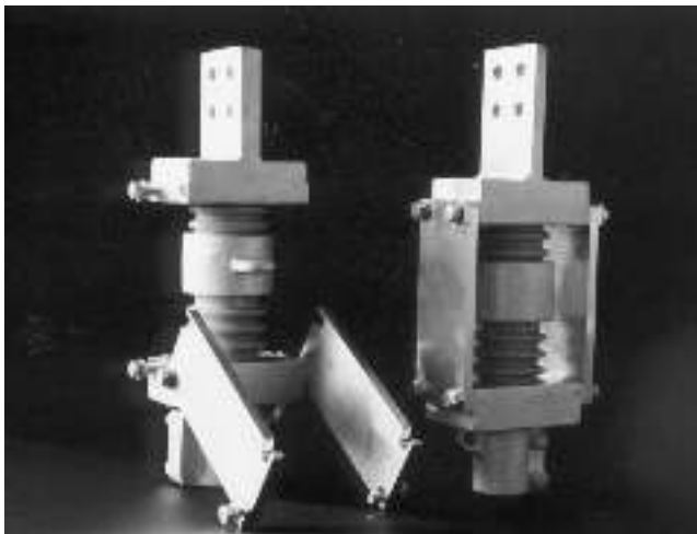
FIGURE 12.9 Lapp test terminal. (Photo courtesy of Lapp Insulator Company, Leroy, NY.)
