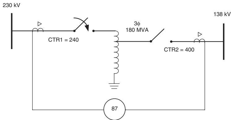
FIGURE 18.27 Transformer energization during commissioning.
