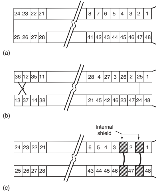
FIGURE 20.6 Common disk winding section pairs: (a) continuous; (b) interleaved; and (c) internally shielded.
