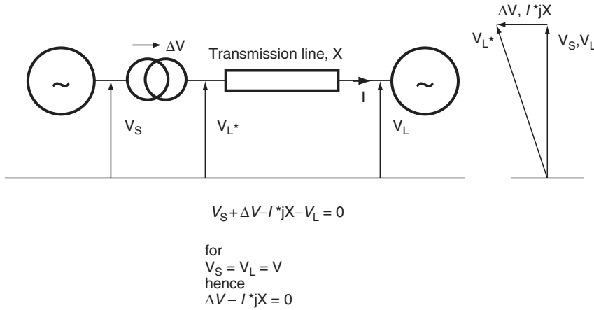
FIGURE 4.4 Connection of two systems.
