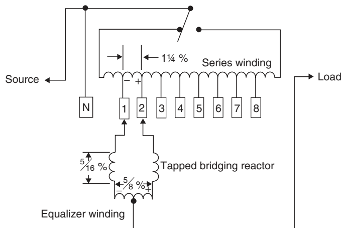
FIGURE 8.22 Equalizer winding incorporated into the main coil of a regulator.
