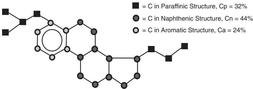
FIGURE 11.2 Typical oil molecule.
