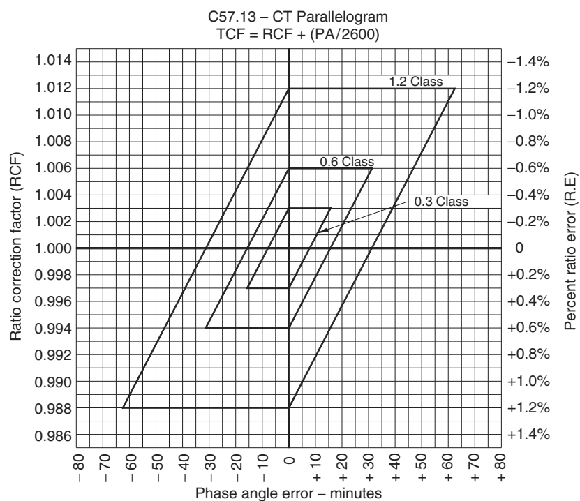
FIGURE 7.8 Accuracy coordinates for CTs.
