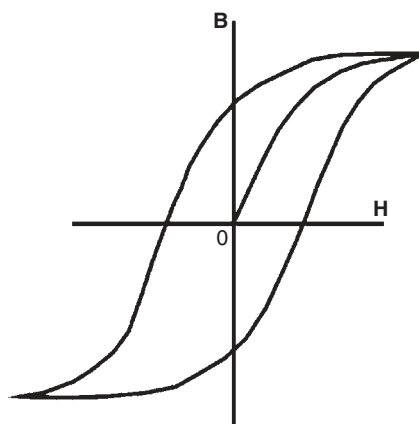
FIGURE 1.7 Hysteresis loop.
