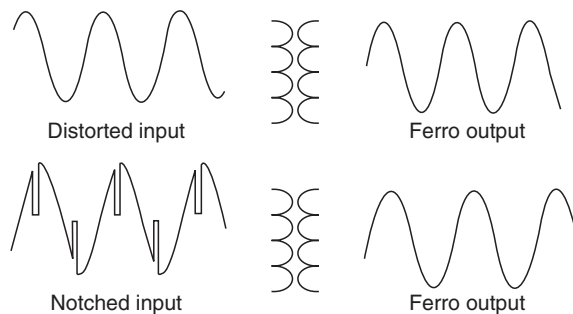
FIGURE 9.12 Output voltages resulting from distorted and notched input voltages at full load.
