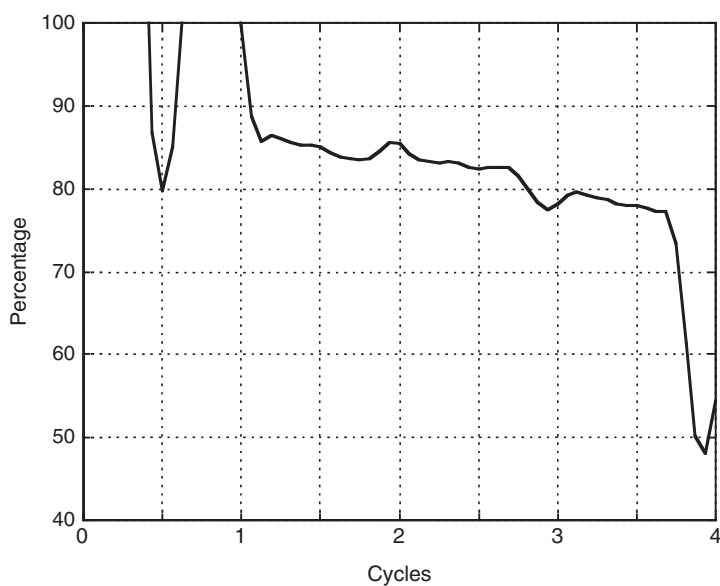
FIGURE 18.21 DC component as percentage of the rms value of fundamental during inrush conditions.
