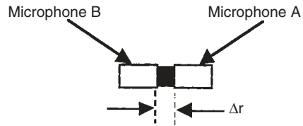
FIGURE 19.1 Measurement of pressure gradient using two closely spaced microphones.
