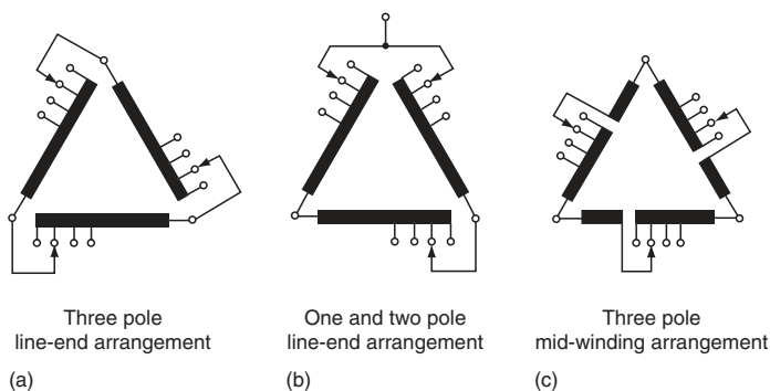
FIGURE 13.23 LTC with delta-connected windings.
