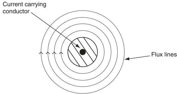
FIGURE 1.1 Magnetic field around conductor.
