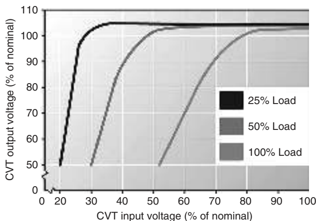
FIGURE 9.9 Typical performance of a constant-voltage transformer (CVT) as a function of load; as the CVT load increases, the ability of the CVT to regulate its output voltage decreases.
