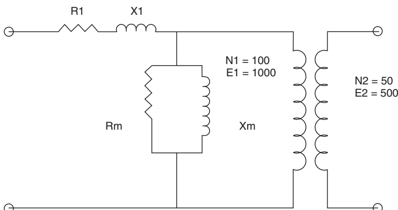
FIGURE 1.5 Equivalent circuit.
