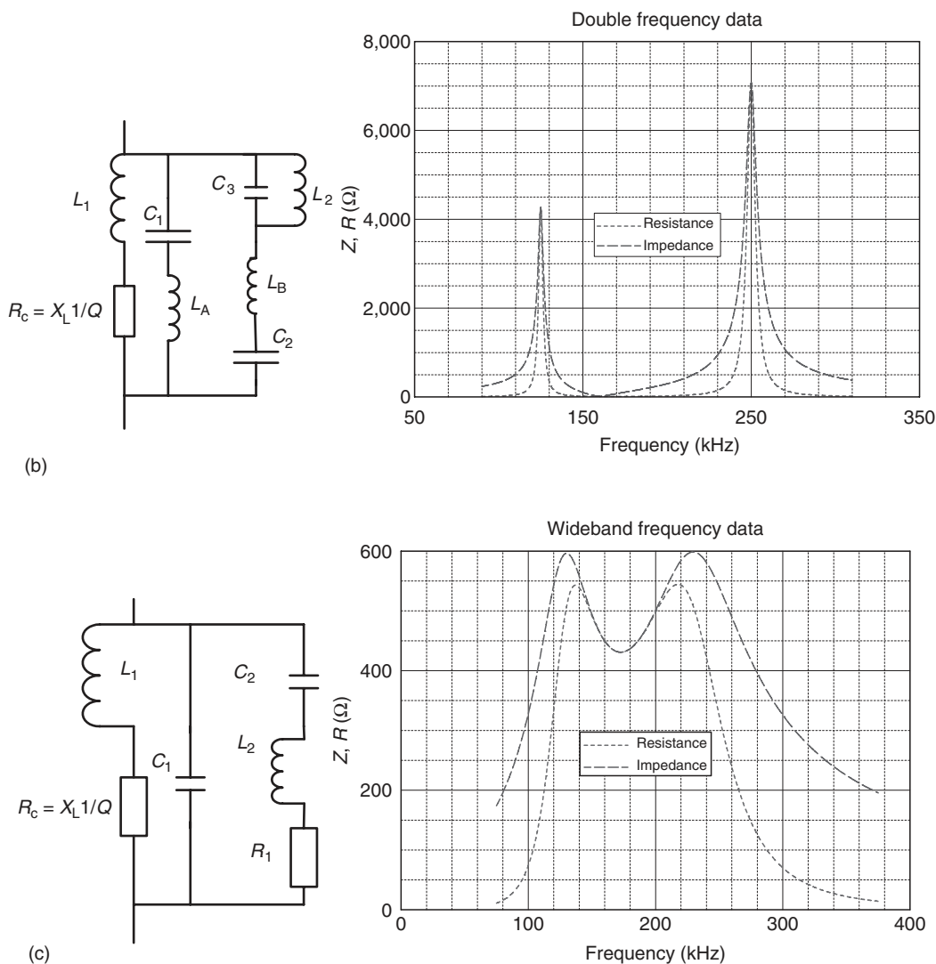
FIGURE 10.53 (continued) (b) Double frequency schematic and impedance response; (c) wideband frequency schematic and impedance response.
