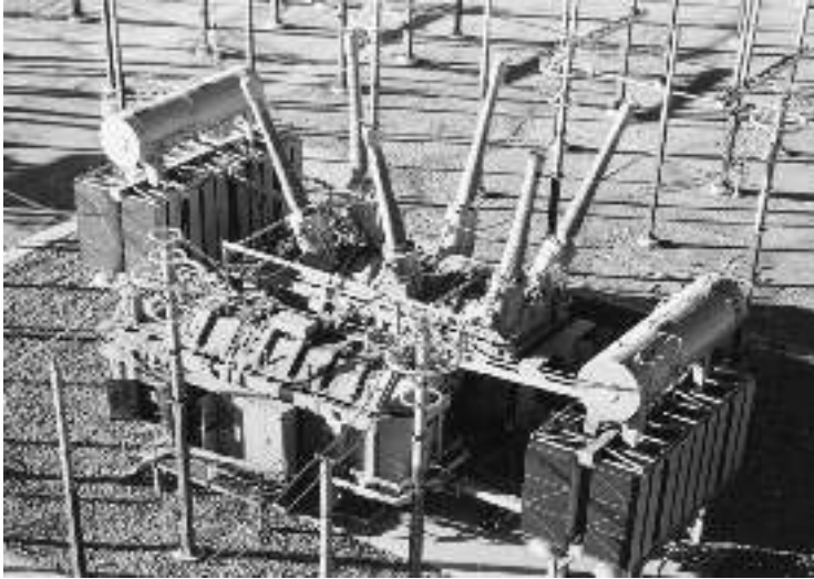
FIGURE 4.20 Two-tank PST with three coarse- and one fine-tap winding at field site (650 MVA, 60 Hz, 525/525 \pm 12 \times 1.2^\circ kV). (By Courtesy of VATEch Transformatoren Weiz Austria (since 2005, Member of Siemens Group).)
