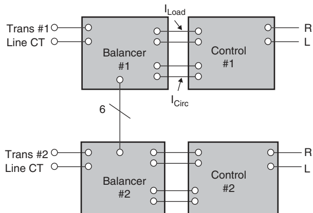
FIGURE 17.9 Control block diagram, paralleling by usual circulating-current method.
