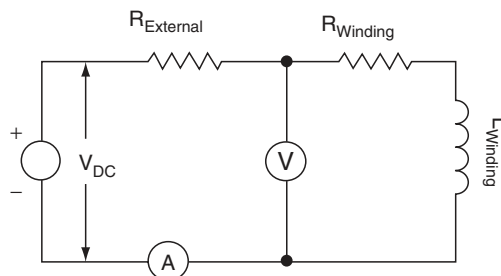
FIGURE 16.17 Circuit for measuring winding resistance.
