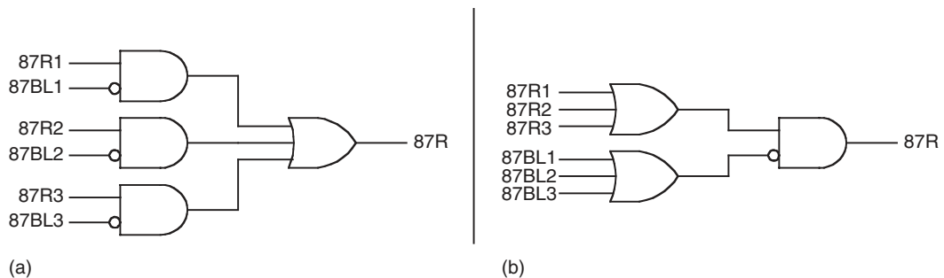
FIGURE 18.17 Differential-relay blocking logic. (a) IHBL = Y and (b) IHBL = N.
