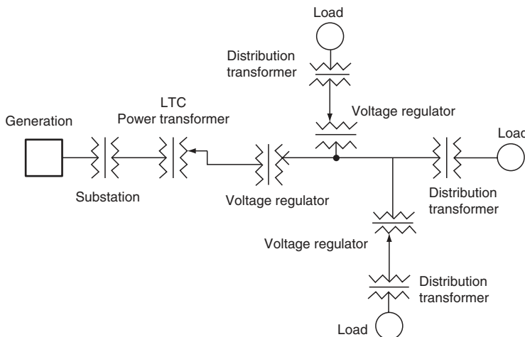
FIGURE 8.2 Power system.
