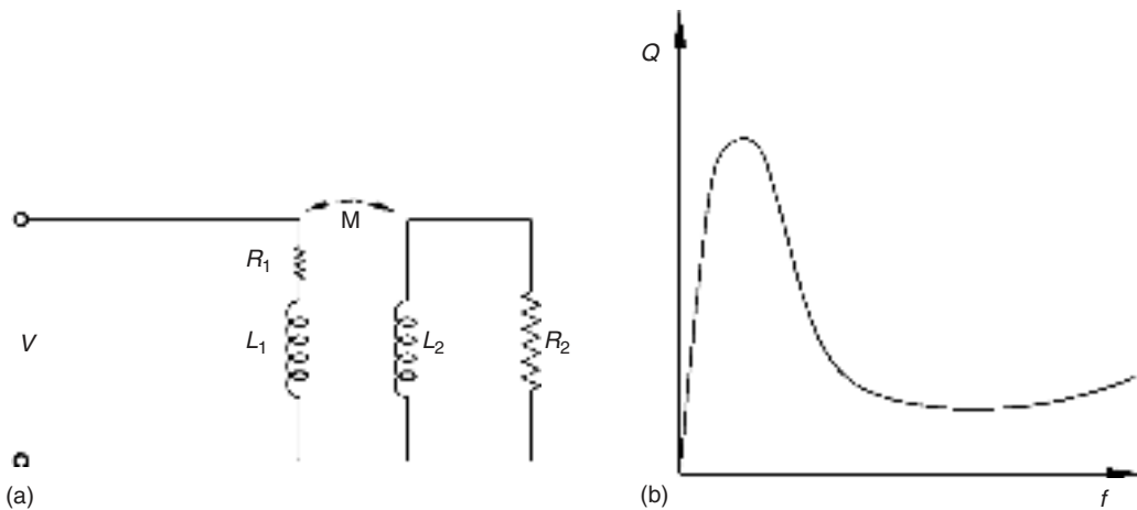
FIGURE 10.46 (a) Circuit diagram for a reactor with a de-Q'ing ring; (b) Typical graph of Q vs. frequency for a reactor plus de-Q'ing rings.
