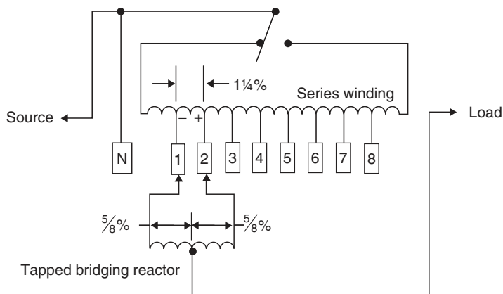
FIGURE 8.19 Two movable contacts on adjacent stationary contacts (bridging position).
