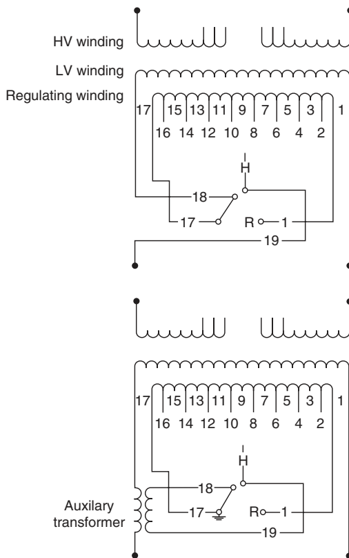
FIGURE 2.19 Schematic and connection chart for transformer with a load tap changer supplied on a 13.2-kV low voltage.
