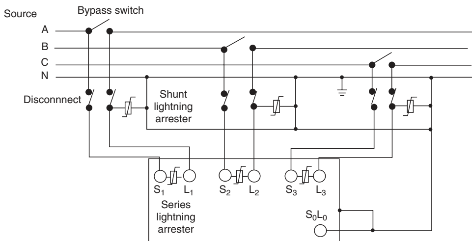
FIGURE 8.26 Connection of three-phase regulator regulating a three-phase, four-wire, multigrounded wye circuit.
