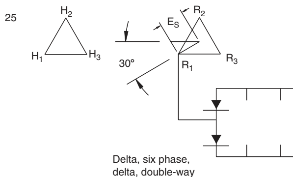
FIGURE 5.2 ANSI Circuit 25. (From ANSI/IEEE C57.18.10-1998. © IEEE 1998. With permission.)
