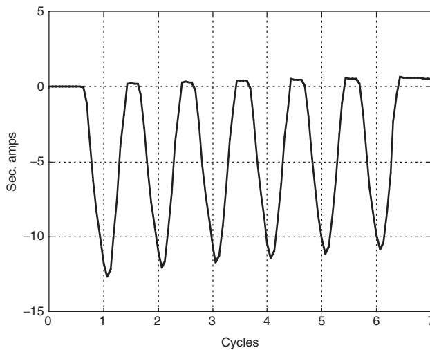
FIGURE 18.28 Inrush current with low-current intervals lasting less than one-quarter cycle.
