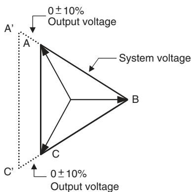
FIGURE 8.8 Phasor diagram of two voltage regulators regulating a three-phase circuit.
