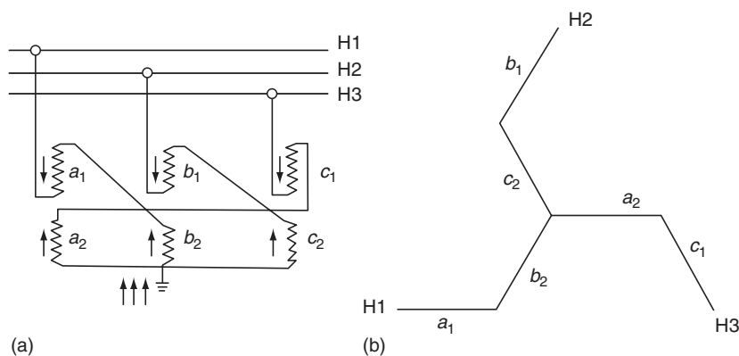
FIGURE 15.4 Interconnected star-grounding transformer: (a) current distribution in the coils for a line-to-ground fault and (b) normal operating voltages in the coils.
