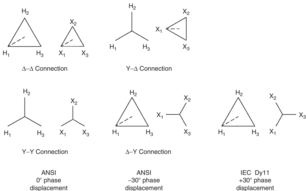
FIGURE 3.12 Three-phase angular displacement. (From IEEE C57.105-1978. The IEEE disclaims any responsibility or liability resulting from the placement and use in the described manner. Information is reprinted with the permission of the IEEE.)
