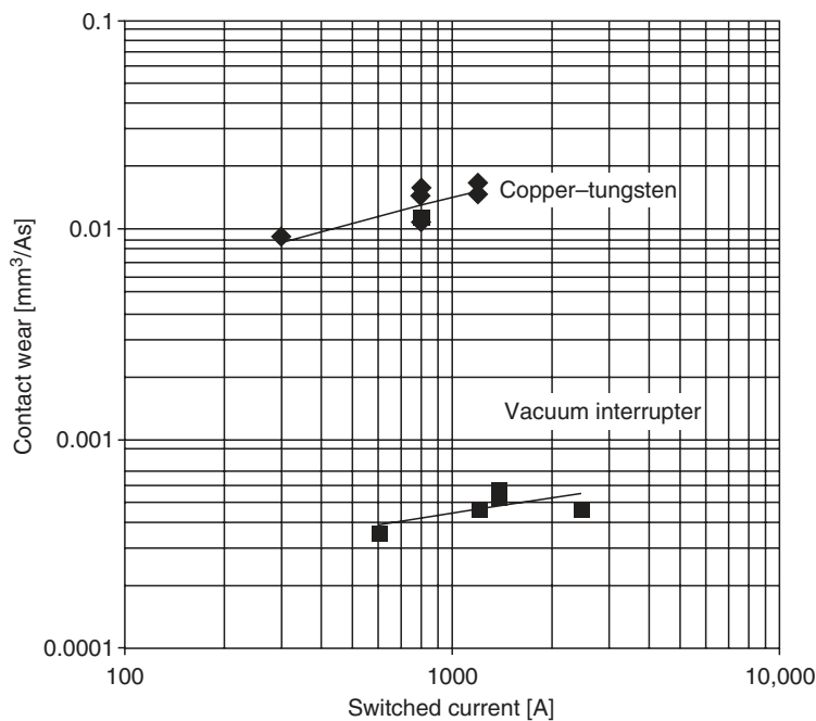
FIGURE 13.12 Comparison of the rates of contact wear of conventional copper–tungsten contacts and vacuum interrupters.
