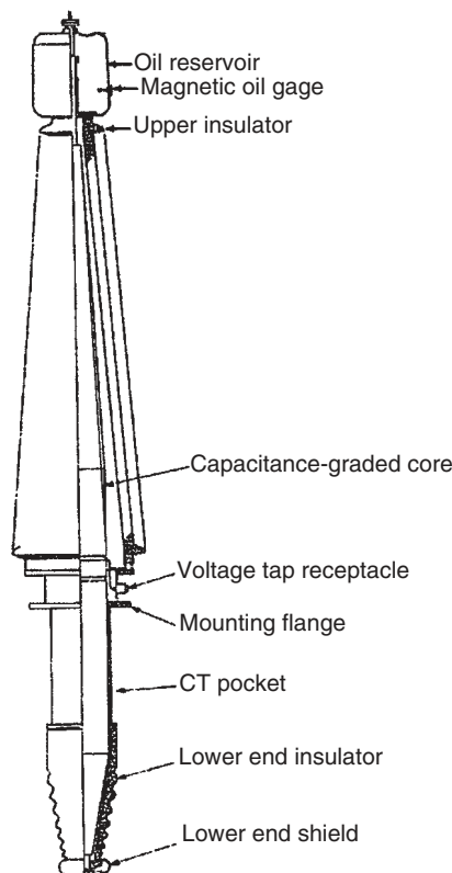
FIGURE 12.2 Oil-filled, capacitance-graded bushing.
