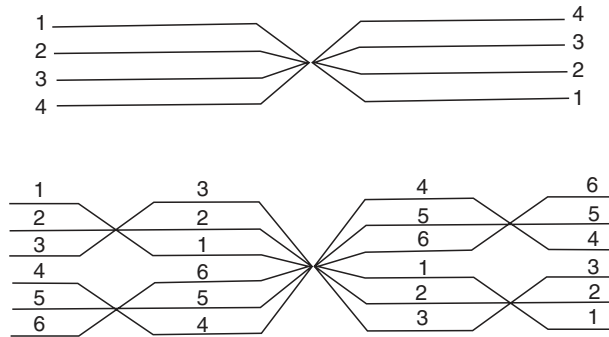
(a) Forms of transposition
