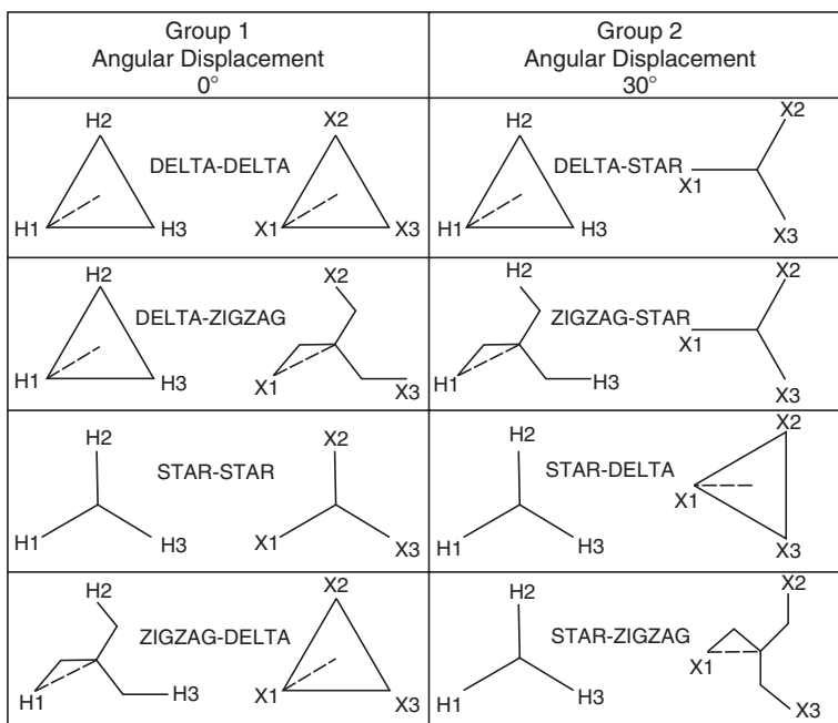
FIGURE 15.2 Standard angular displacement for three-phase transformers.
