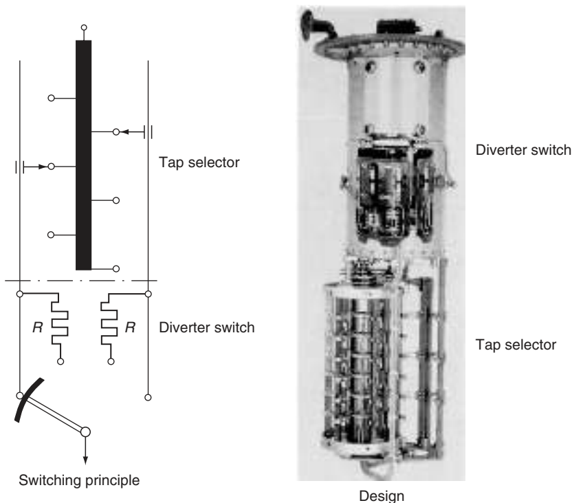
FIGURE 13.5 Design principle—diverter switch (arcing switch) with tap selector. (Photo courtesy of Maschinenfabrik Reinhausen GmbH.)
