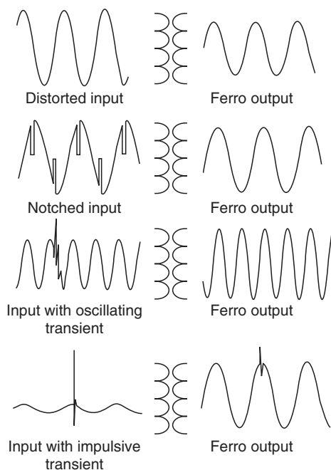
FIGURE 9.7 Filtering ability of a constant-voltage transformer.
