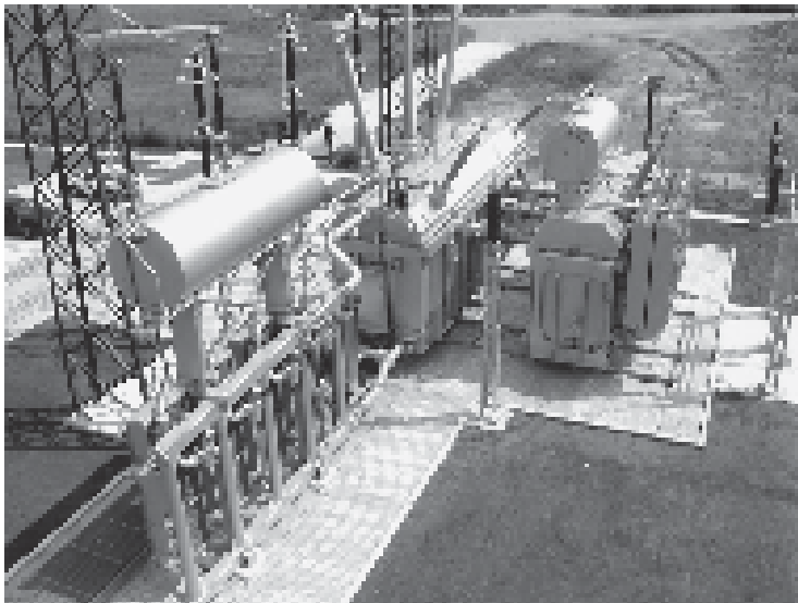
FIGURE 4.14 Quadrature booster set (300 MVA, 50 Hz, 400 \pm 12 \cdot 1.25\% / 115 \pm 12 \cdot 1.45^\circ kV). (By Courtesy of EVN Energieversorgung Niederösterreich Austria and Siemens AG, Germany.)
