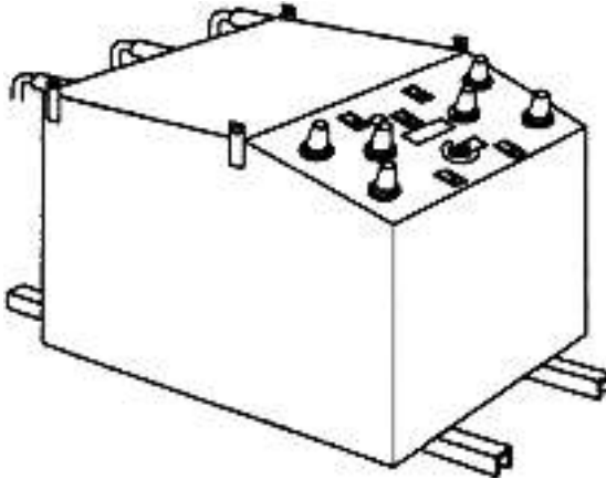
FIGURE 3.23 Six-bushing horizontal. (By permission of Pacific Gas and Electric Company, San Francisco, CA.)
