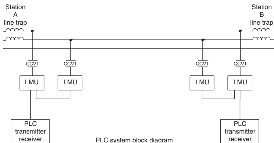
FIGURE 10.51 Block diagram of typical PLC system; Interphase Coupling.
