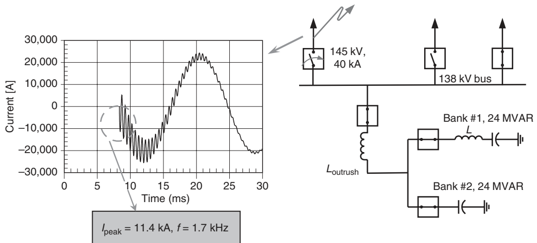
FIGURE 10.19 Location of the outrush reactor in the circuit (right) and outrush current after reactor installation (left).
