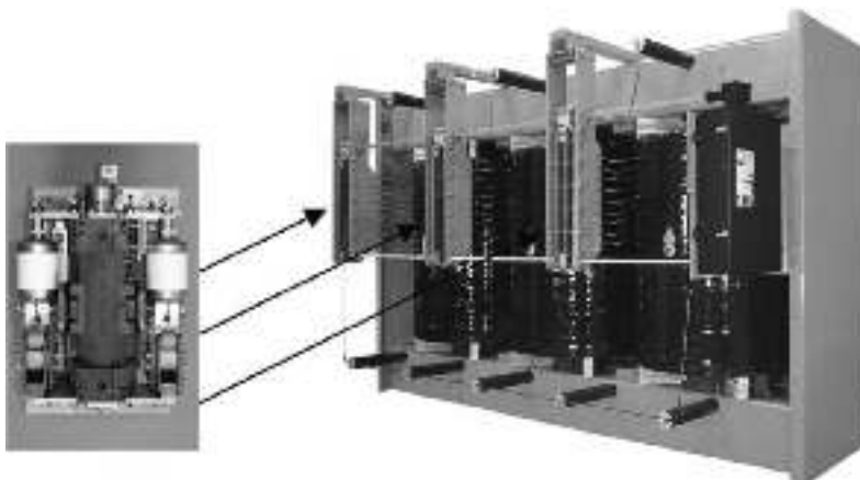
FIGURE 13.13 Resistor vacuum-type LTC for dry-type transformers. (Photo courtesy of Maschinenfabrik Reinhausen GmbH.)
