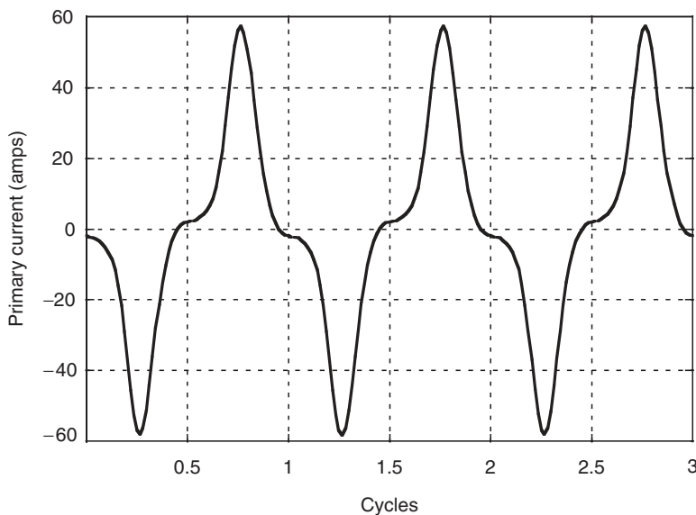
FIGURE 18.3 Exciting current of an overexcited transformer; overvoltage of 150% applied to a 5-KVA, 230/115-V single-phase transformer.
