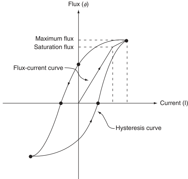
FIGURE 9.3 Flux-current curve with hysteresis curve.
