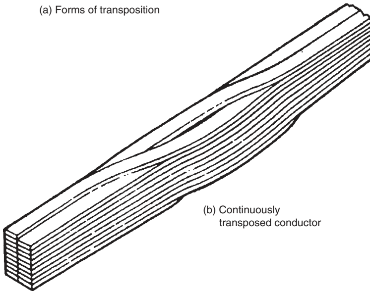
FIGURE 1.10 Continuously transposed conductor cable.
