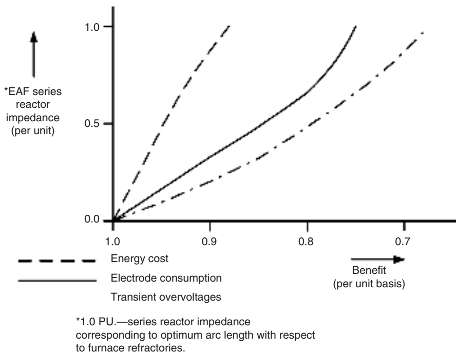
FIGURE 10.32 EAF series reactor benefits.
