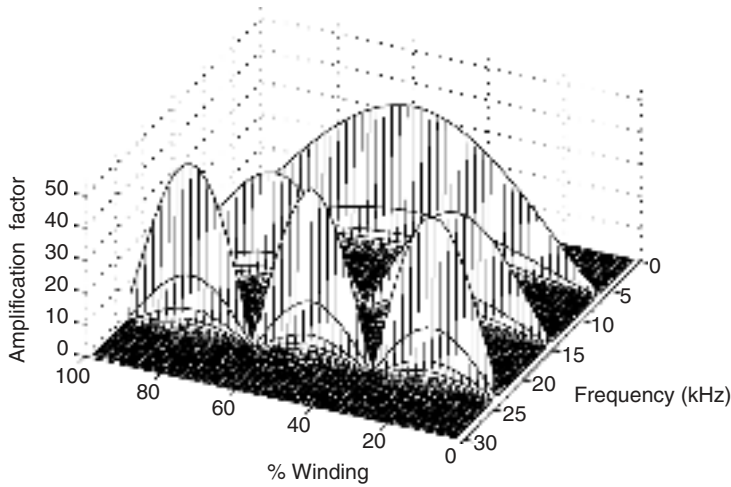
FIGURE 20.5 Amplification factor at 5 from 0 to 30 kHz.
