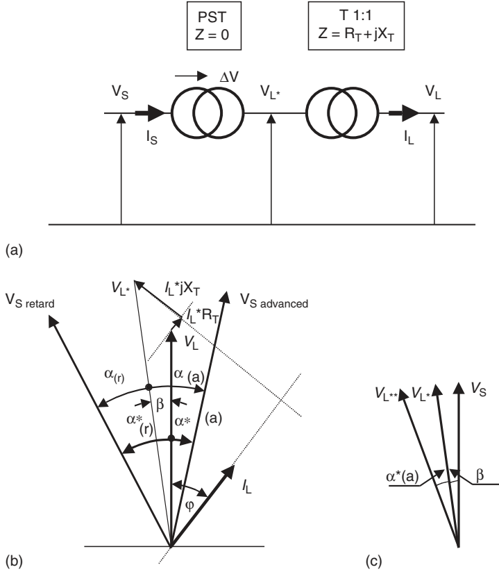
FIGURE 4.5 On-load diagram of a PST.
