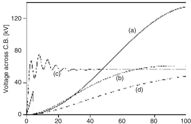
FIGURE 10.42 Results of a TRV study for a subtransmission substation: (a) Breaker TRV capability, (b) system TRV when no reactor installed, (c) system TRV when a current limiting reactor installed, and (d) system TRV with capacitor across reactor terminals.
