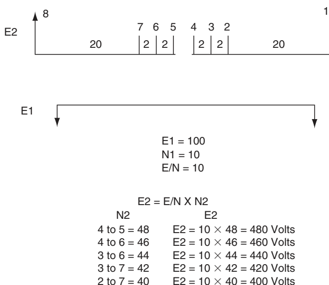
FIGURE 1.9 Illustration of how taps added in the windings can compensate for voltage drops.
