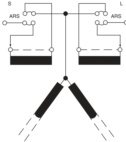
FIGURE 13.31 Phase-shifting transformer—change-over operation by means of an advance-retard switch (ARS).
