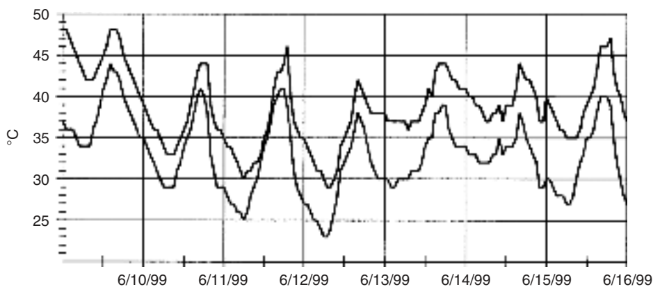
FIGURE 23.9 Sample differential-temperature measurement. The top trace is the main-tank top-oil temperature, and the bottom trace is the LTC compartment temperature.
