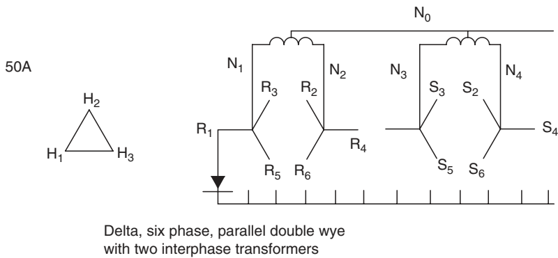
FIGURE 5.8 ANSI Circuit 50A. (From ANSI/IEEE C57.18.10-1998. © IEEE 1998. With permission.)
