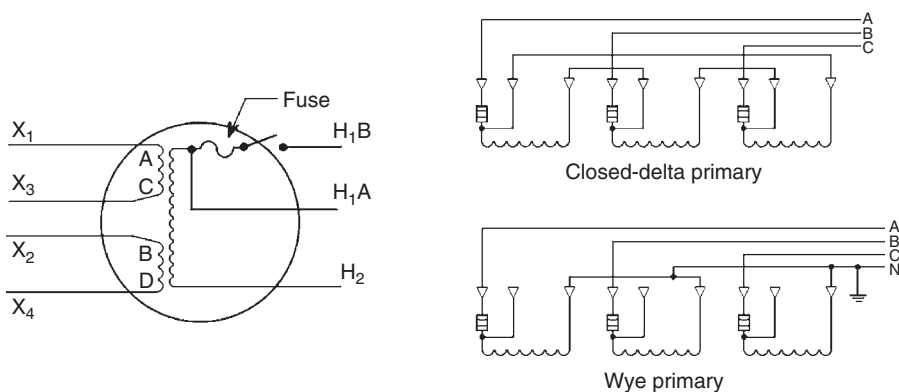
FIGURE 3.15 Three-bushing subway. (By permission of Pacific Gas and Electric Company, San Francisco, CA.)
