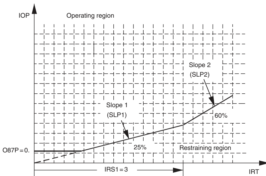
FIGURE 18.14 Percentage restraint differential characteristic.
