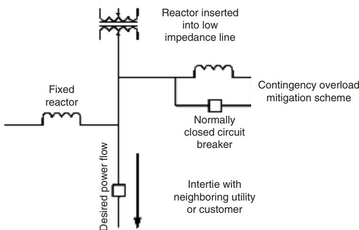
FIGURE 10.22 Typical high voltage power flow control reactor connections.
