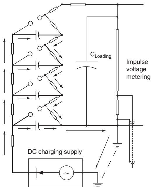
FIGURE 16.6 Charging the capacitors of an impulse generator.
