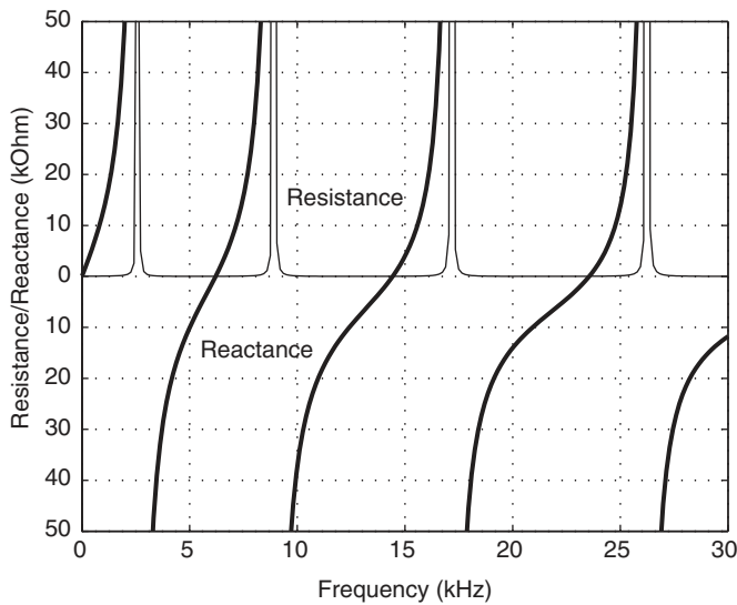
FIGURE 20.4 Terminal impedance for a helical winding.
