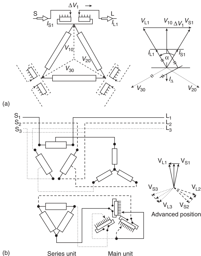
FIGURE 15.5 Two main type of PSTs: (a) single core; (b) dual core.
