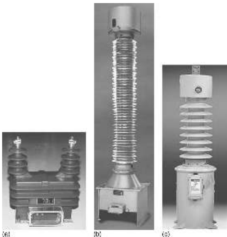
FIGURE 7.12 (a) 15-kV dual-bushing outdoor VT, (b) 242-kV single-bushing VT, (c) 69-kV single-bushing VT. (Photos courtesy of Kuhlman Electric Corp.)
