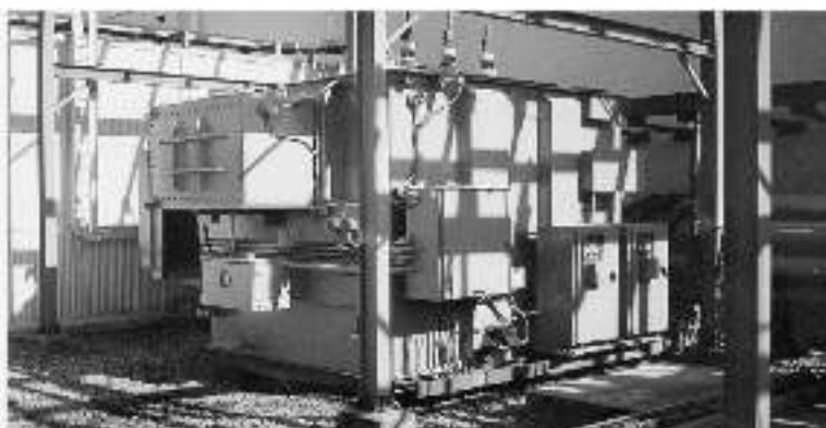
FIGURE 5.23 A 37,500-kVA OFAF regulating autotransformer with LTC and saturable core reactors and dc power supplies. The high voltage is dual voltage for 13,800-V wye and 23,000-V wye. The LTC and saturable-core reactors permit the secondary voltage to range from 14,850-V wye down to 7,150-V wye. The LTC makes coarse taps, while the saturable-core reactors provide infinite variability between taps. This transformer powers downstream to an electrochemical service diode rectifier. The transformer weighs over 170,000 lb, as it includes the main transformer, a series transformer, a preventive autotransformer, and saturable core reactors. The dc power supplies provide control to the saturable-core reactors. (Photo courtesy of Niagara Transformer Corp.)
