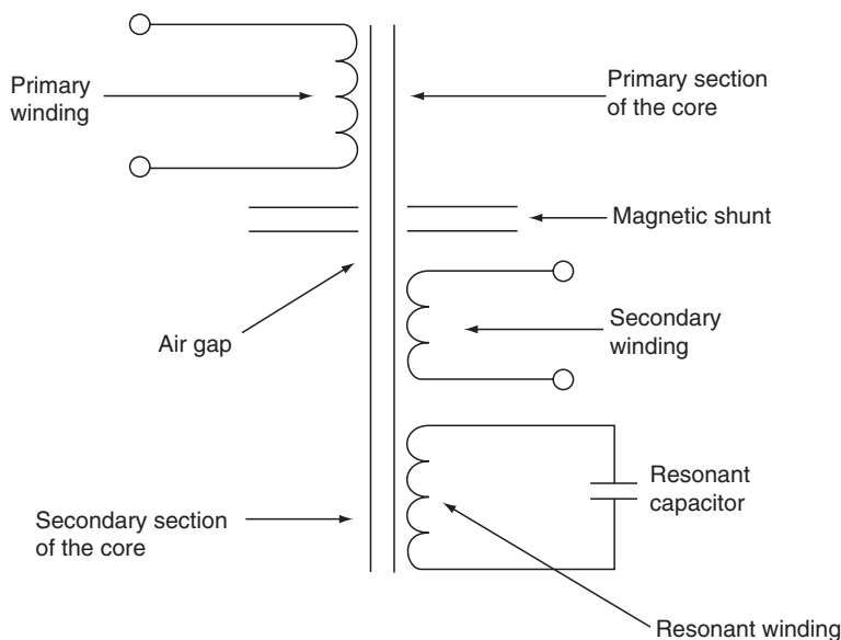
FIGURE 9.4 Schematic of a constant-voltage transformer.
