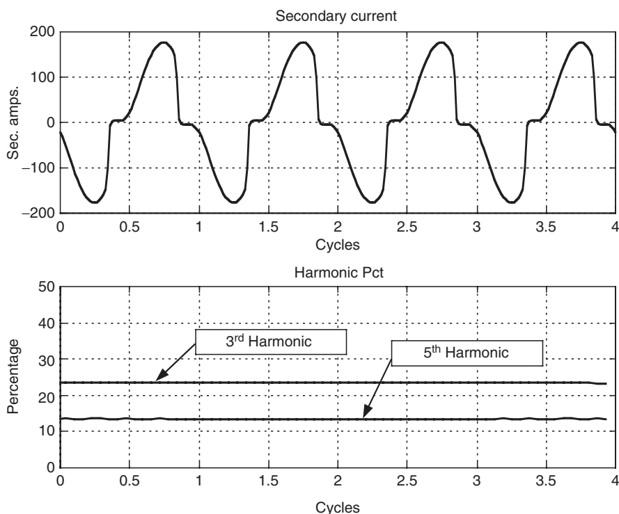
FIGURE 18.5 Typical secondary current for symmetrical CT saturation and its harmonic content.
