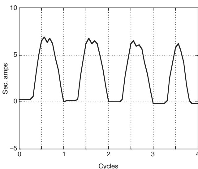
FIGURE 18.19 Element 1 high-side winding current, I_{AB} , recorded while energizing the transformer with an A-phase external fault.
