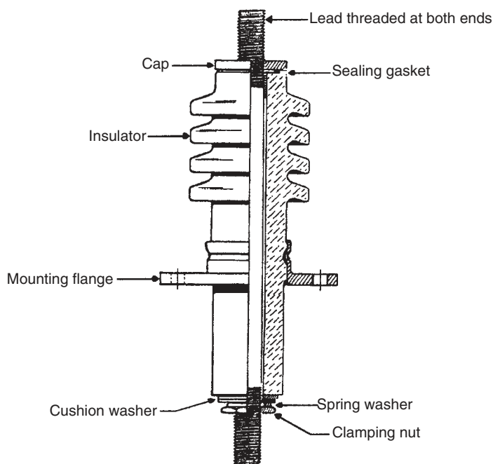
FIGURE 12.1 Solid-type bushing.
