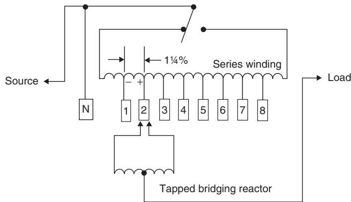
FIGURE 8.17 Two movable contacts on the same stationary contact (symmetrical position).
