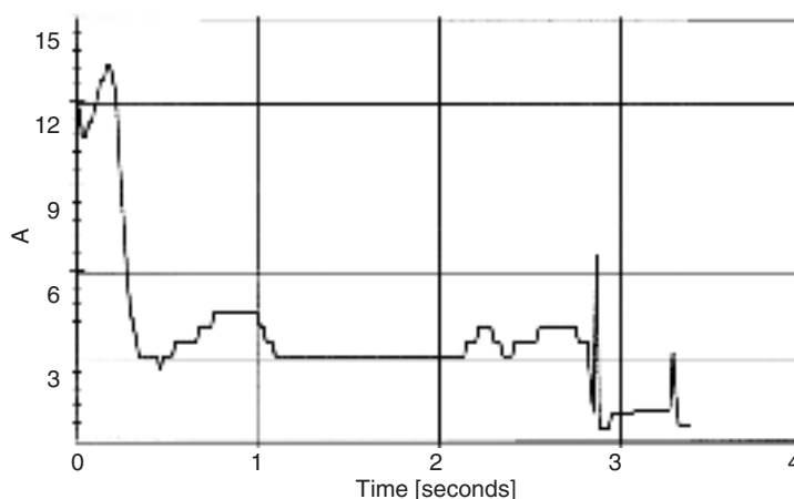
FIGURE 23.7 Load-tap-changer motor current during a tap-changing event.
