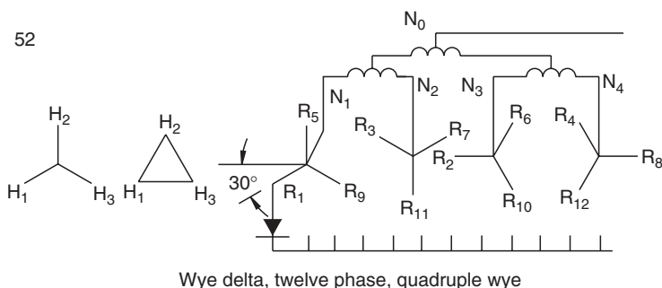
FIGURE 5.11 ANSI Circuit 52. (From ANSI/IEEE C57.18.10–1998. © IEEE 1998. With permission.)
