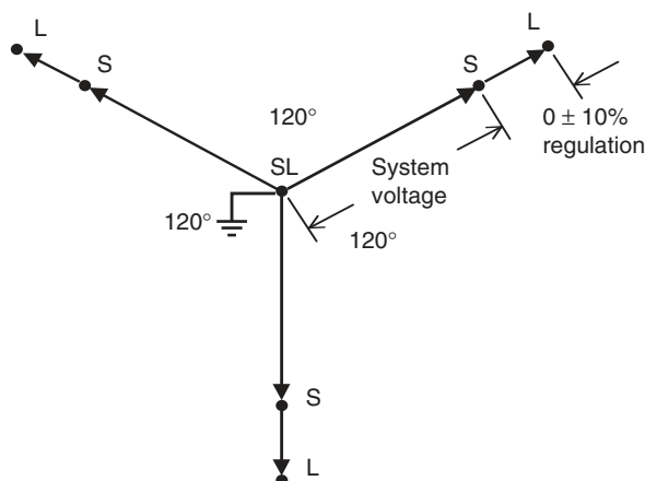
FIGURE 8.6 Phasor diagram of three regulators regulating a three-phase, four-wire, multigrounded wye circuit.
