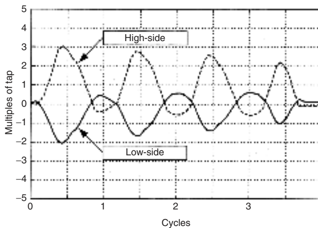
FIGURE 18.23 Element 1 inrush currents from the high- and low-side transformer windings after relay scaling.
