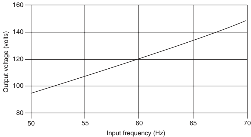
FIGURE 9.11 Output-voltage amplitude resulting from variations in frequency of the ac input voltage.
