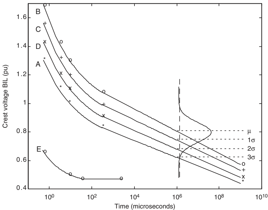
FIGURE 20.9 Voltage-time curve for insulation coordination.
