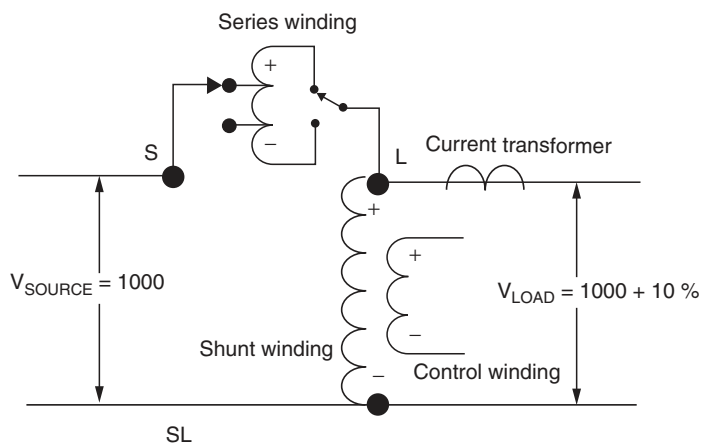
FIGURE 8.24 Voltage regulation on the source side (Type B).
