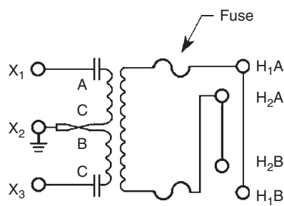
FIGURE 3.20 Four-primary bushing. (By permission of Pacific Gas and Electric Company, San Francisco, CA.)
