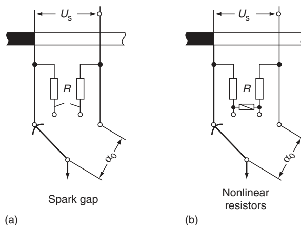
FIGURE 13.35 Overvoltage protection devices arranged within the diverter switch (arcing switch).
