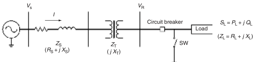
FIGURE 10.33 Radial system.
