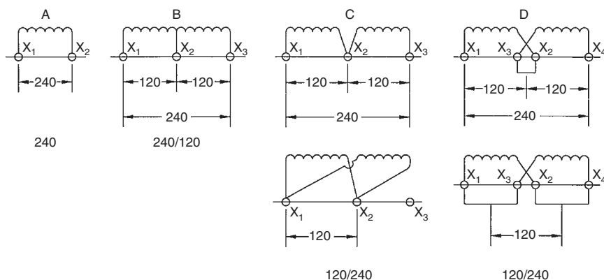
FIGURE 3.9 Single-phase secondary connections. (By permission of ABB Inc., Jefferson City, MO.)
