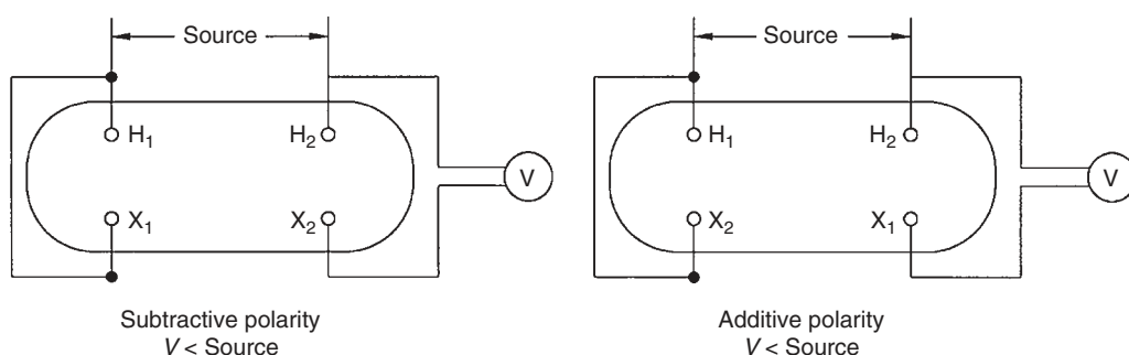
FIGURE 3.11 Single-phase polarity. (From IEEE C57.12.90-1999. The IEEE disclaims any responsibility or liability resulting from the placement and use in the described manner. Information is reprinted with the permission of the IEEE.)
