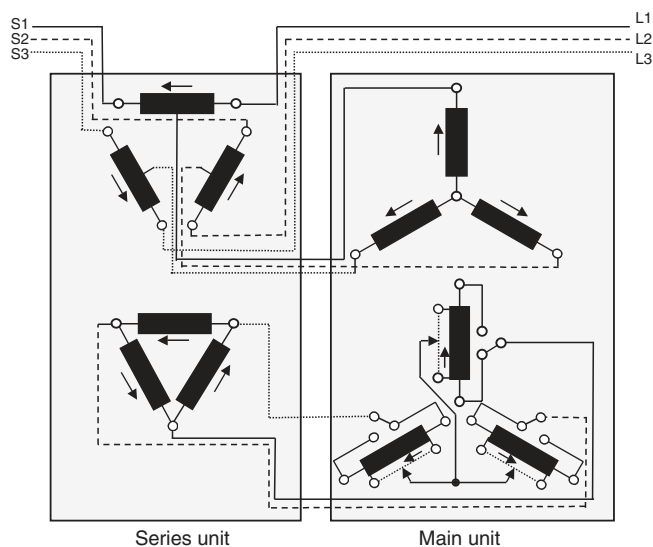
FIGURE 4.12 Two-core PST.
