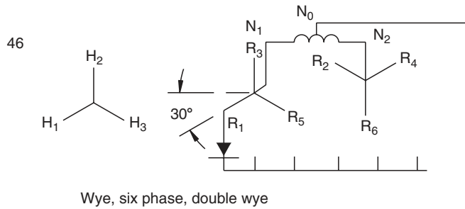
FIGURE 5.6 ANSI Circuit 46. (From ANSI/IEEE C57.18.10-1998. © IEEE 1998. With permission.)
