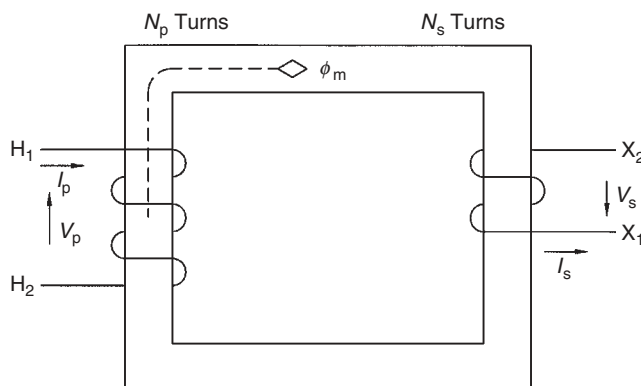
FIGURE 3.36 Two-winding transformer schematic. (By permission of ABB Inc., Jefferson City, MO.)
