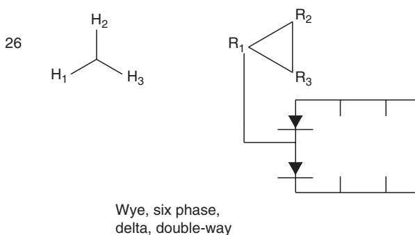
FIGURE 5.3 ANSI Circuit 26. (From ANSI/IEEE C57.18.10-1998. © IEEE 1998. With permission.)
