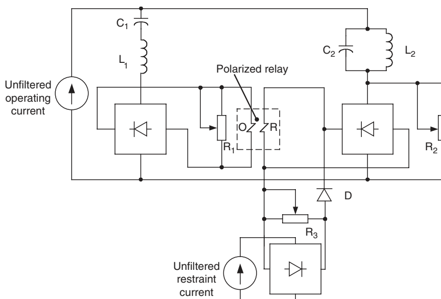
FIGURE 18.6 Transformer differential relay with harmonic restraint.
