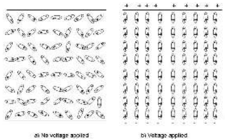
Fig. 3.17: Polarisation of a dielectric.
