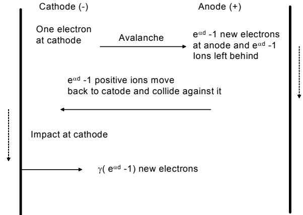
Fig. 3.3: Secondary ionization due to cathode collision
