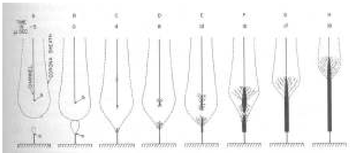
Fig. 5.9: Leader approaching ground
