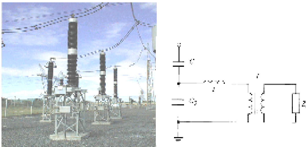
Fig. 1.22 :A high voltage Capacitive Voltage Transformer(CVT)
