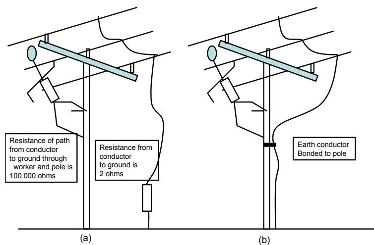
Fig. 6.6: Unsafe (a) and safe (b) earthing practices for work on a line.
