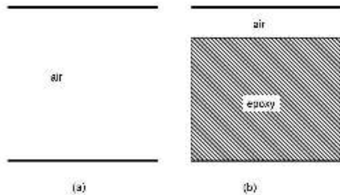
Fig. 3.25: Series dielectrics
