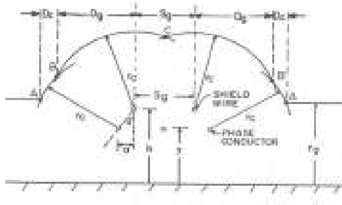
Fig. 5.17: The geometrical model for line lightning protection.
