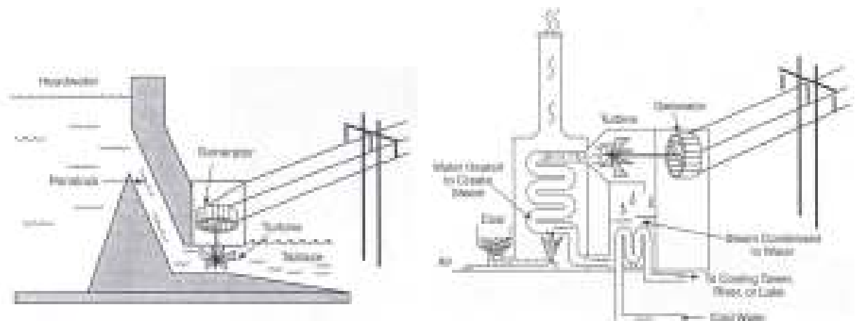
Fig. 1.3: Schematic diagrams, showing the operation of a hydro-electric power station (left) and a coal-fired power station (right)
