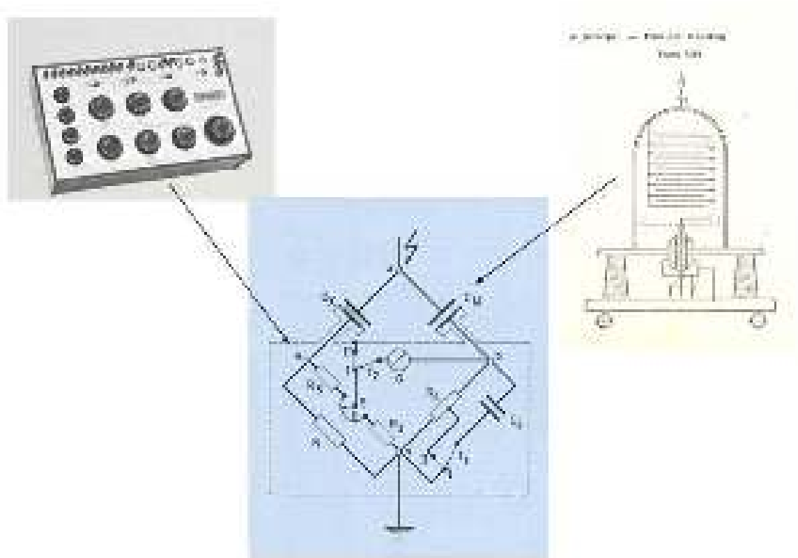
Fig. 4.20: Typical Schering Bridge set-up (Tettex)
