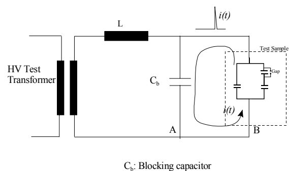
Fig. 4.23: Discharge detector circuit
