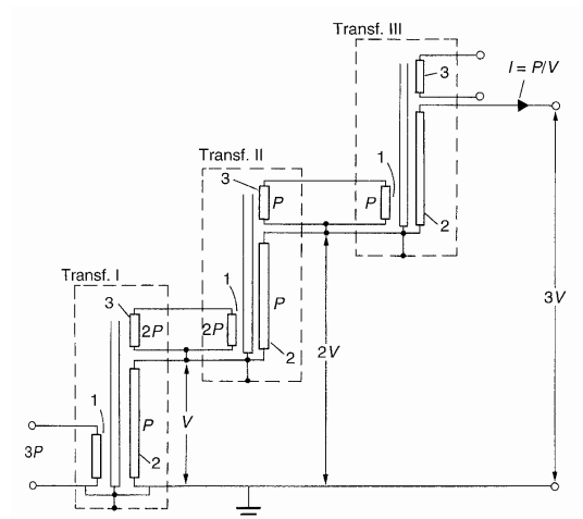
Fig. 4.3: Cascade connected test transformers
