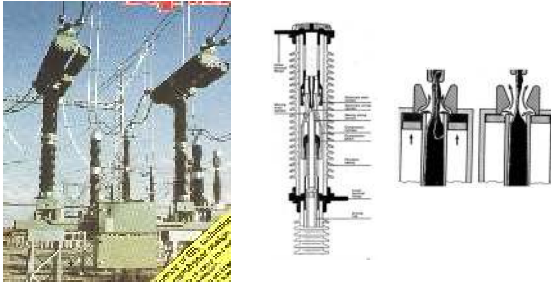
Fig. 1.28: SF6 Circuit Breakers
