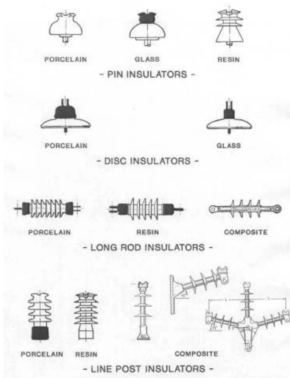
Fig. 1.12: Insulator types
