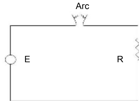
Fig. 3.12: Circuit for interruption of an arc.
