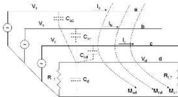
Fig. 6.4: Electromagnetic induction
