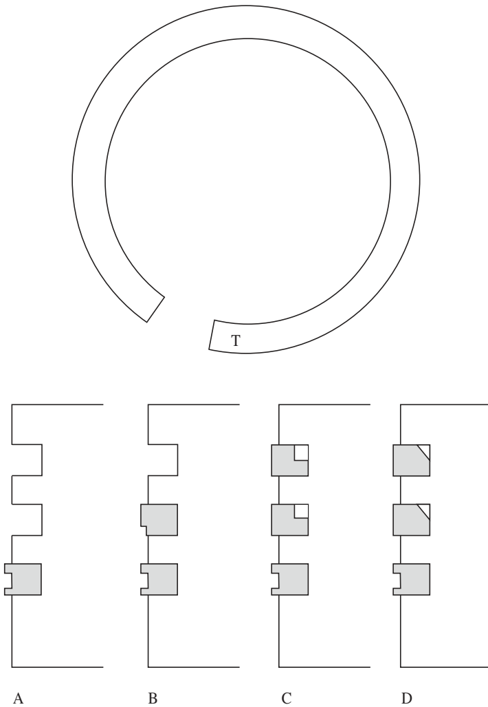
FIG. 7-21 Four-cycle pistons have three rings—an oil ring at the bottom (A). Some use a scraper ring (B), but the upper two rings on most pistons are compression rings (C, D). Scraper and compression rings must be installed in the correct orientation with the marked side up toward the piston crown.
