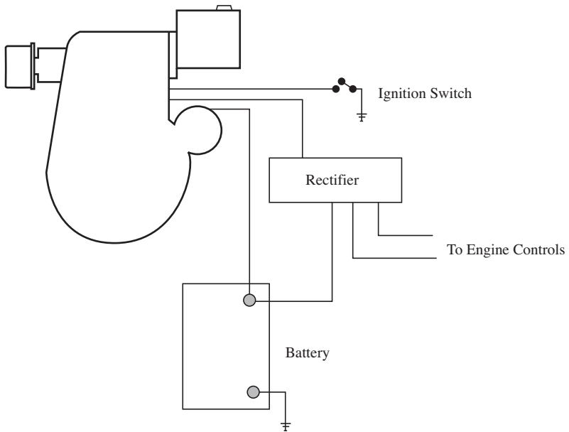
FIG. 4-3 The flywheel alternator on smaller gensets supplies power for battery charging and engine controls.
