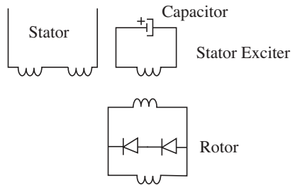
Brushless Generator
