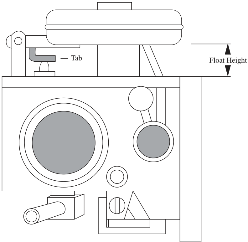
FIG. 6-10 Float height is most often measured from the toe of the float to the carburetor body.
