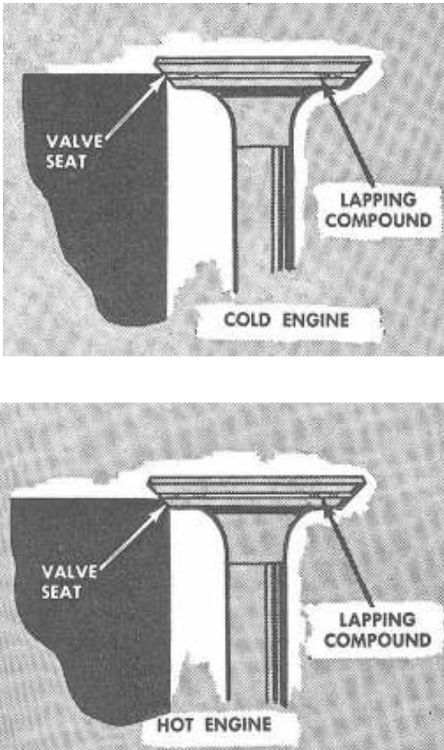
FIG. 7-15 Lapping valves concaves the valve face because valve steel is much softer than Stellite and similar seat materials. When the engine warms and the seat moves as a result of thermal expansion, the valve leaks. Thermal expansion also can upset valve seating on new or low-hour engines.
