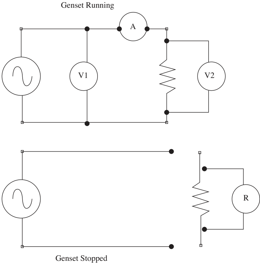
FIG. 3-10 An ammeter ( A ) connects in series, a voltmeter in parallel. Meter V1 reads the voltage across the entire circuit; V2 reads the voltage drop across the load. Resistance measurements ( R ) are made with the power shut off and the component under test disconnected.
