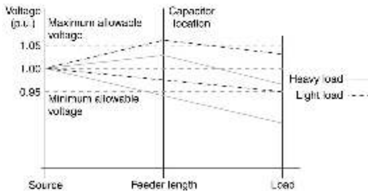
Figure 4.10 Capacitor effect on voltage
