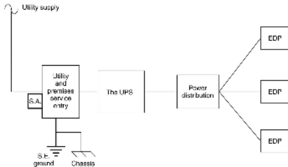
Figure 6.17 Positioning of a lightning arrester
