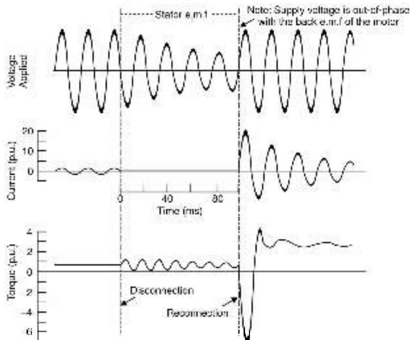
Figure 4.13 Transient torque
