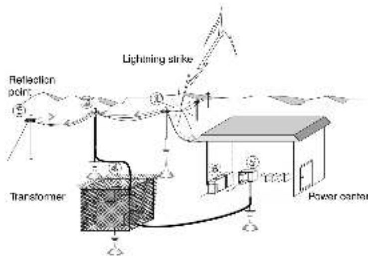
Figure 6.16 Lightning strike to an overhead distribution line
