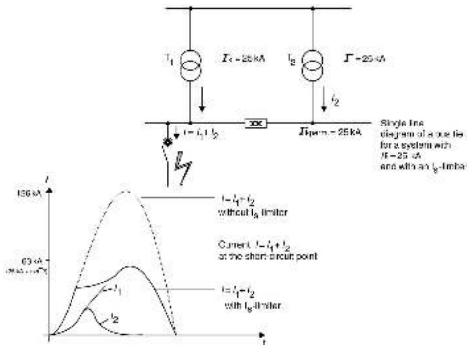
Figure 2.12 Practical use of I_g -limiter
