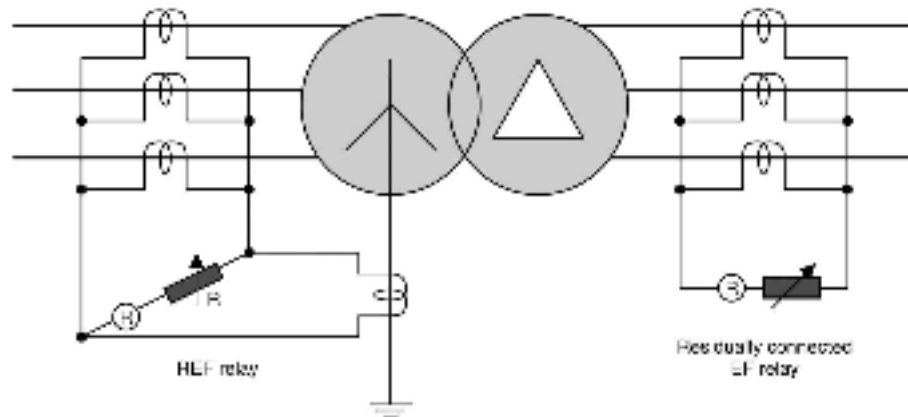
Figure 5.51 A restricted earth fault system
