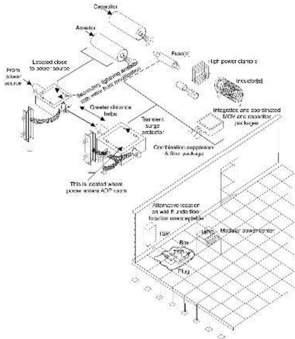
Figure 6.18 Supplementary surge protection elements
