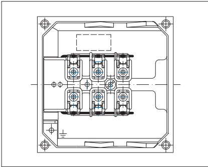
Terminal Box in aluminum motors, sizes 90-100
