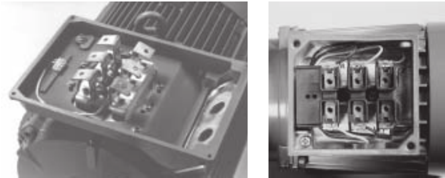
Terminal box of a cast iron motor and of an aluminum motor.
