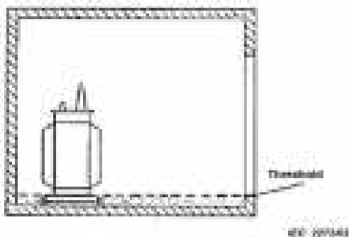
Figure 10 – Sump with integrated common catchment tank
