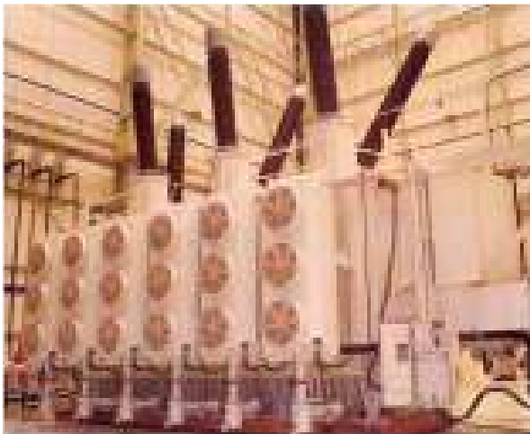
450 MVA auto-connected system intertie transformer
