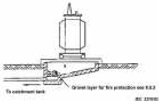
Figure 9 – Sump with separated catchment tank
