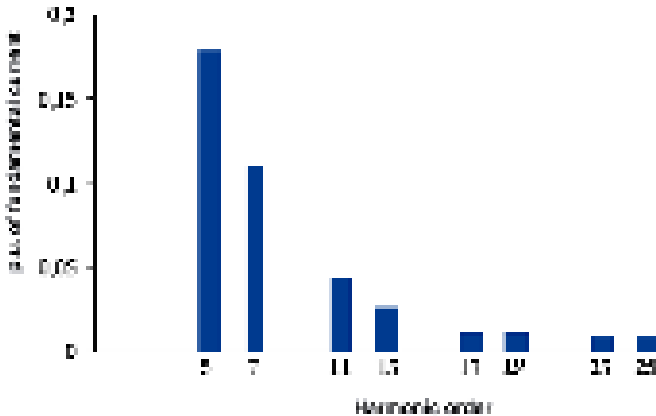
Example on harmonic current spectrum in p.u. of the fundamental frequency current in a 6-pulse connection
