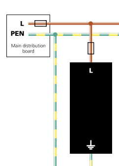
TN-C earthing system
