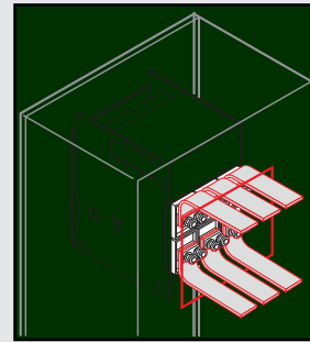
Flat rear terminals
