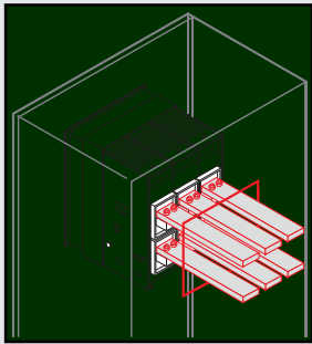
Horizontal rear terminals
