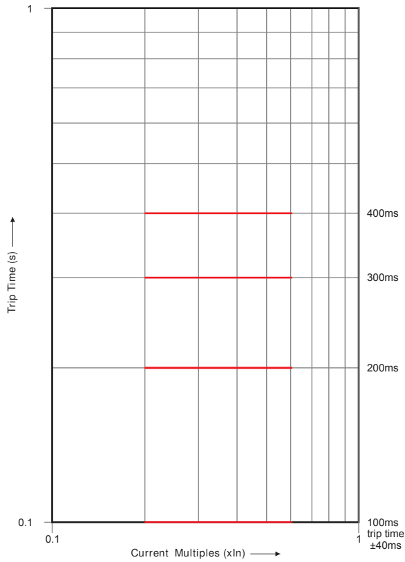
Earth Fault I t OFF (SR18G, SR18G/SR18Gi with display)
