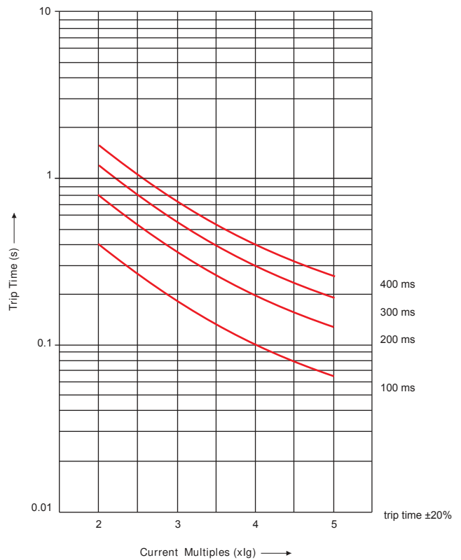
Earth Fault I t 2 t ON (SR18G, SR18G/SR18Gi with display)
