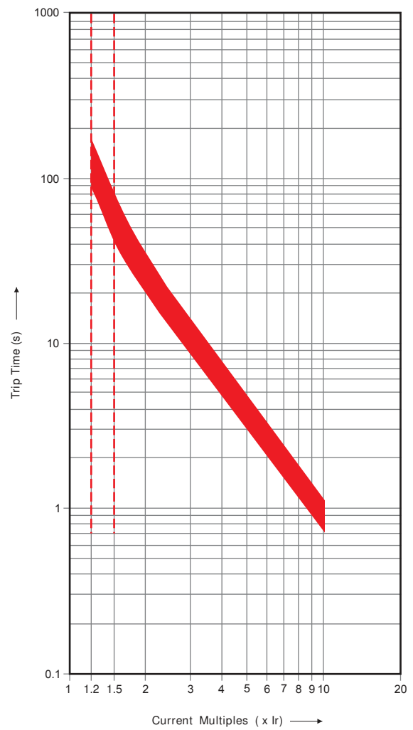
Overload (SR18)
