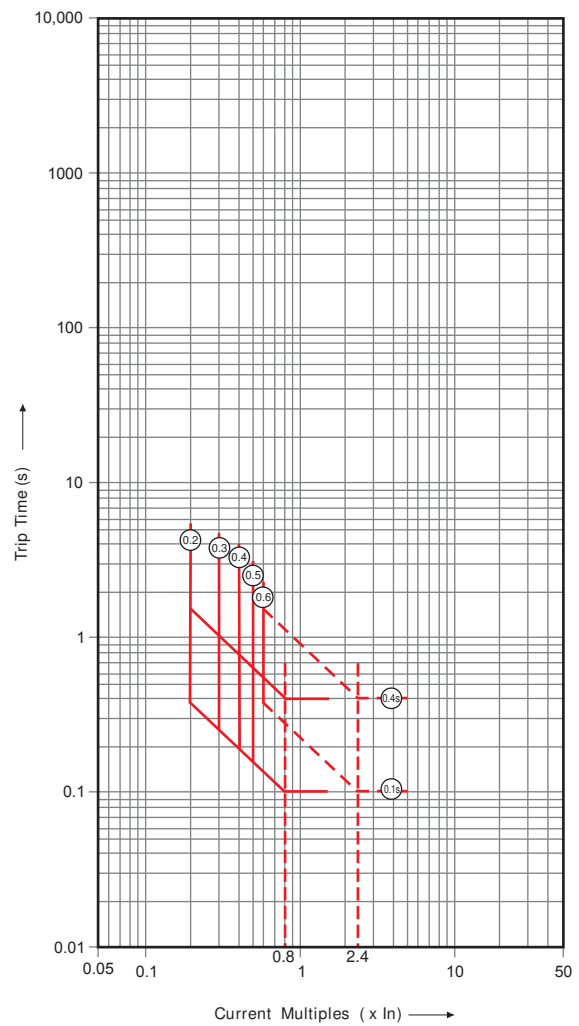
Earth Fault - I t ON (SR71)
