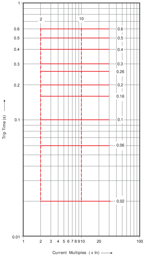
Short-Circuit (SR18)
