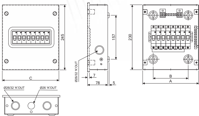
IP30 Single Door
