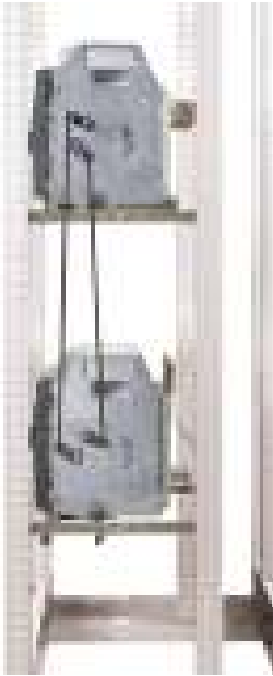
Interlocking of two MasterPact NT or NW circuit breakers using connecting rods.
