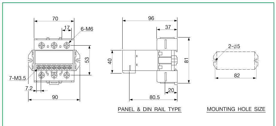
PANEL & DIN RAIL TYPE EOCR-DZT (Terminal Type)
