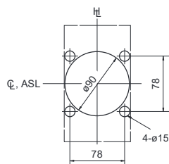
i Panel cutout dimensions
