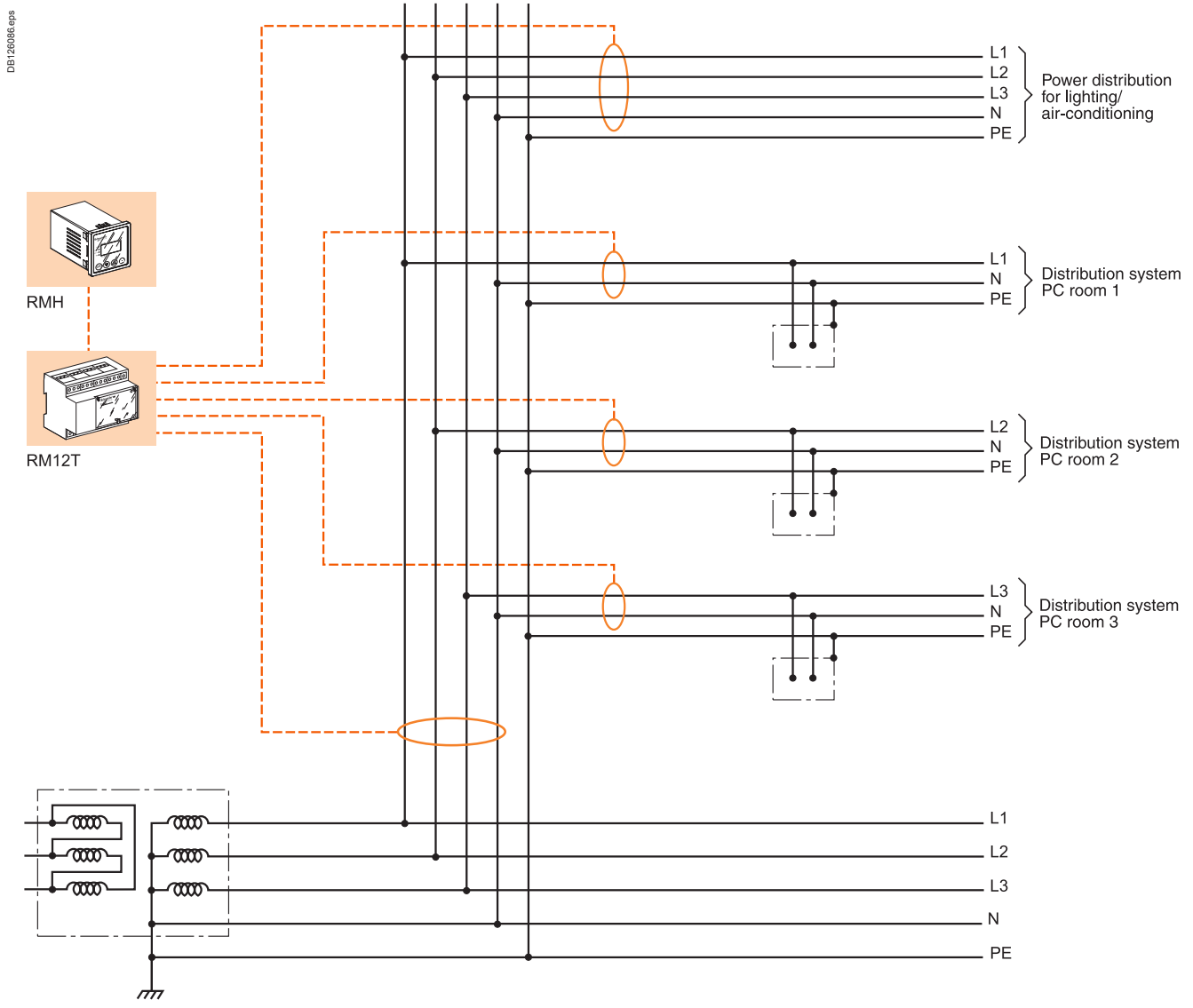
PC network.
