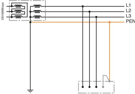
TN-C diagram.
