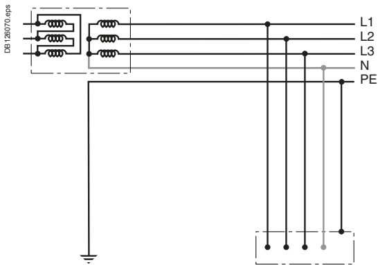
IT system.
