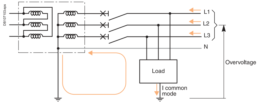
Example of a common-mode disturbance.
