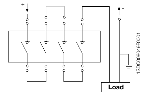
H) 4 poles in series (1000 Vdc)
