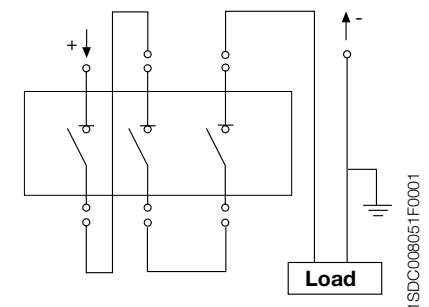
I) 3 poles in series (750 Vdc)
