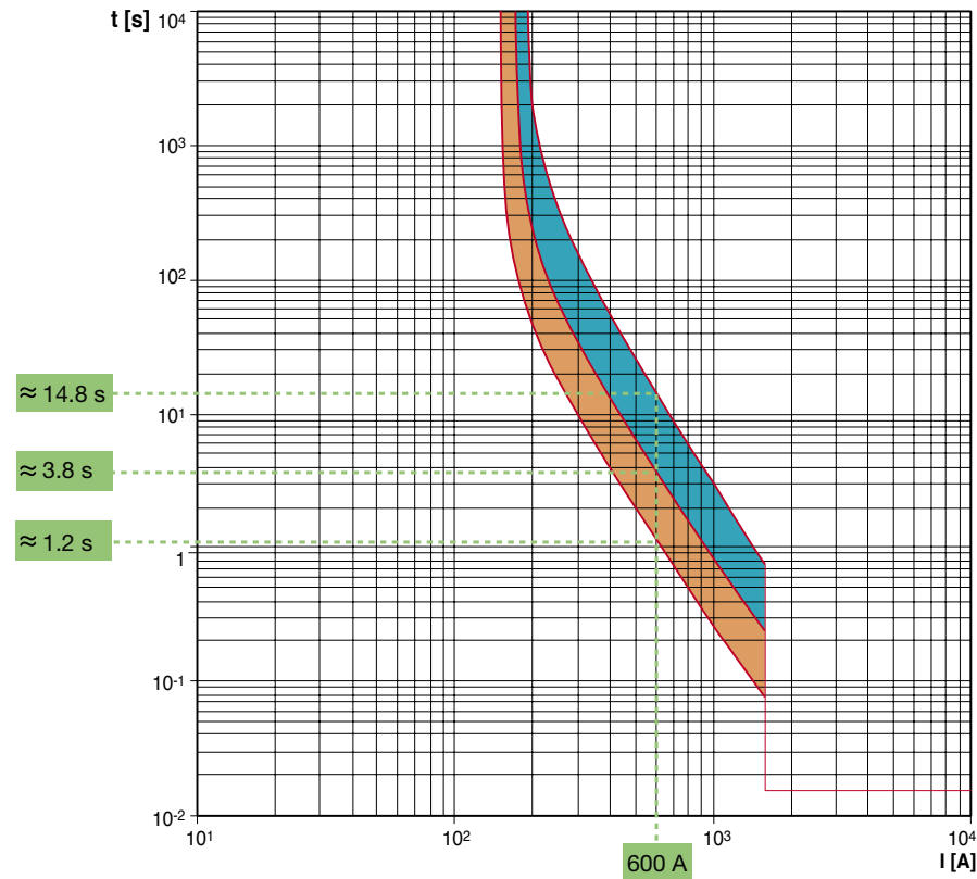
T1 160 - In 160 Time-current curves
