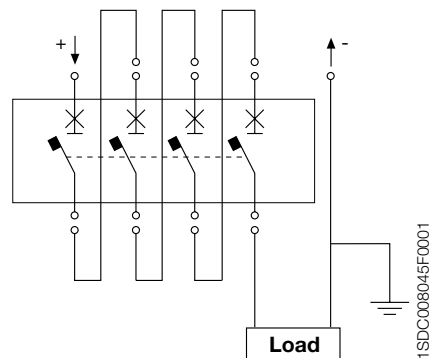
C) 4 poles in series (1000 Vdc)
