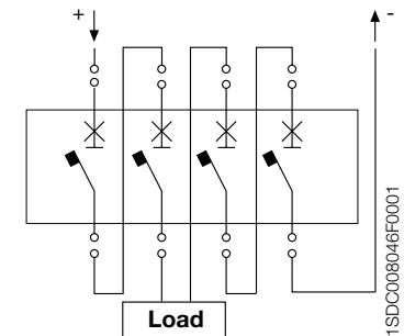
D) 2+2 poles in series (1000 Vdc)
