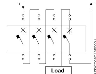
A) 3+1 poles in series (1000 Vdc)
