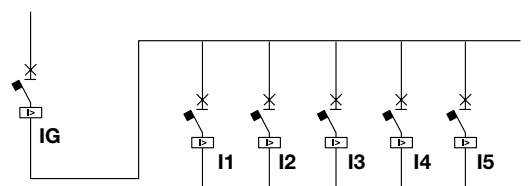
Circuit diagram
