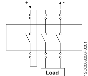
G) 2+1 poles in series (750 Vdc)
