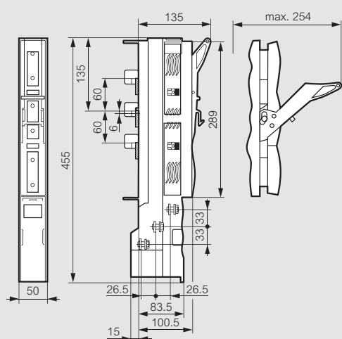
■ SPX-V 00 on 60 mm collector rail
