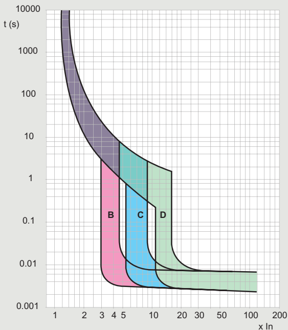
Main tripping curves for DX circuit breakers
