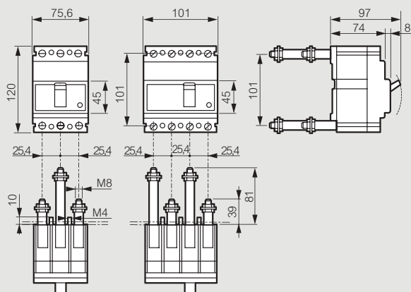
■ Fixed version, rear terminals
