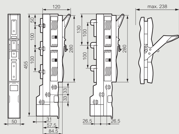
■ SPX-V 00 on 100 mm collector rail
