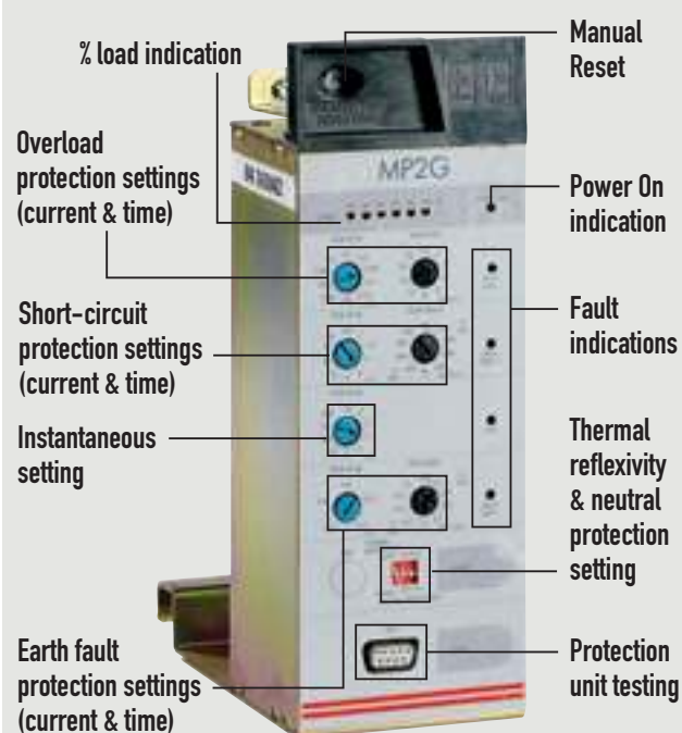
MP 2G electronic protection unit
