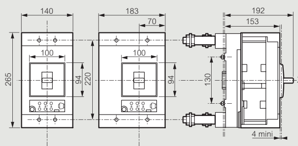
■ Plug-in version, rear terminals
