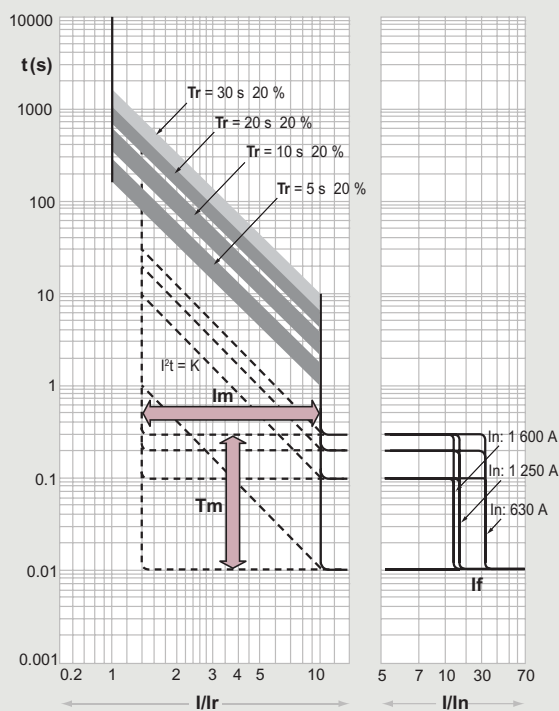
DPX-H 1600 circuit breaker with electronic release
