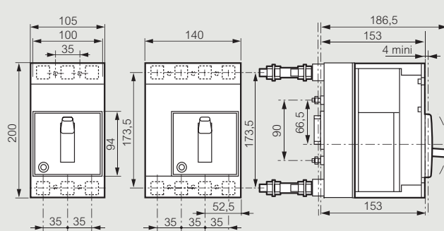
■ Plug-in version, rear terminals
