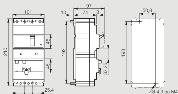
■ Fixed version, front terminals with earth leakage module mounted side by side
