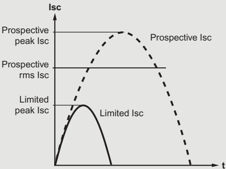
Limitation of the prospective short-circuit current
