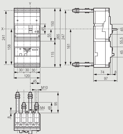
■ Fixed version, rear terminals with earth leakage module mounted side by side
