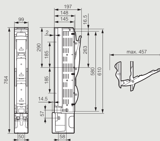
■ SPX-V 1/2/3 on 185 mm collector rail
