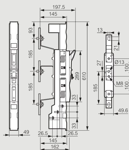
■ SPX-V 00 on 185 mm collector rail using a collector rail adaptor
