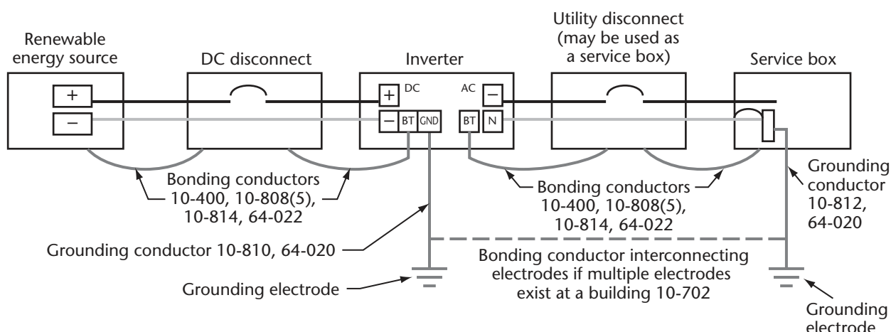
Rule 64-020(2)(b) Grounding electrode requirements
