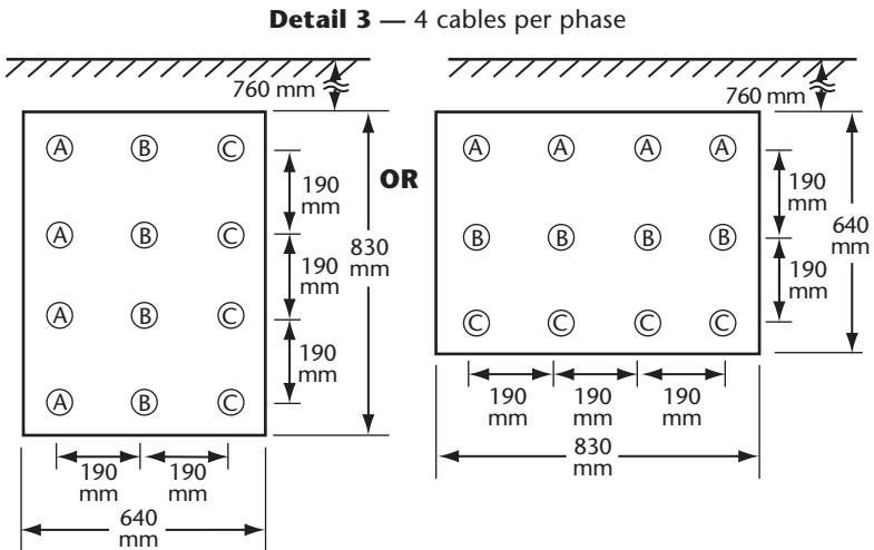
Diagram B4-2 Installation configurations — Conduit
