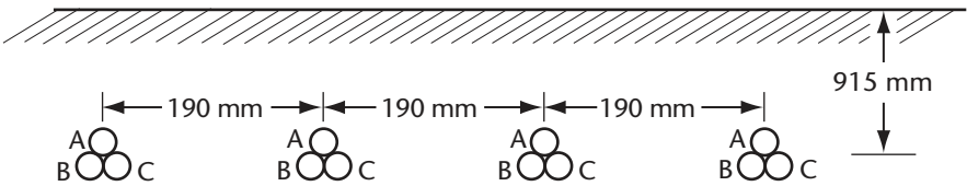
Detail 4 4 cables per phase
