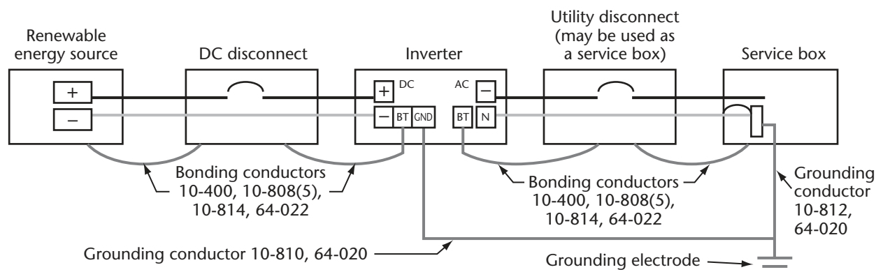
Rule 64-020(2)(a) Grounding electrode requirements
