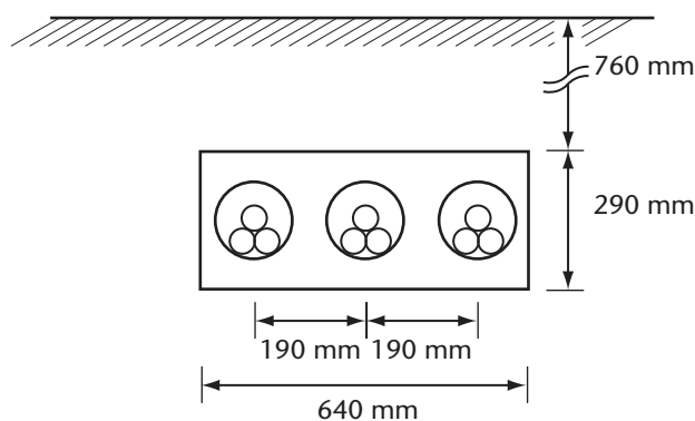
Detail 3 — 3 cables per phase
