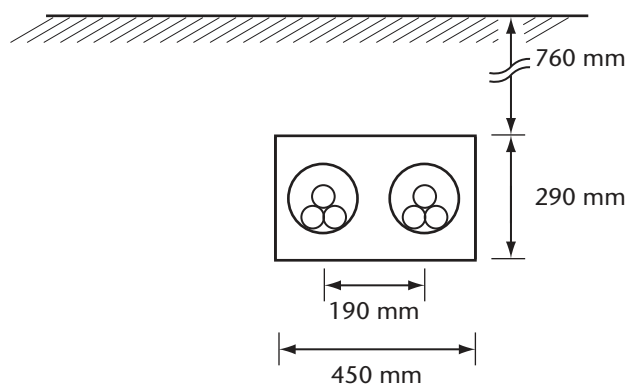
Detail 2 — 2 cables per phase
