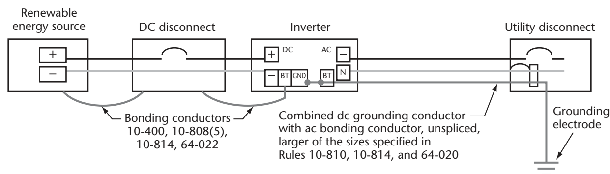
Rule 64-020(2)(c) Grounding electrode requirements
