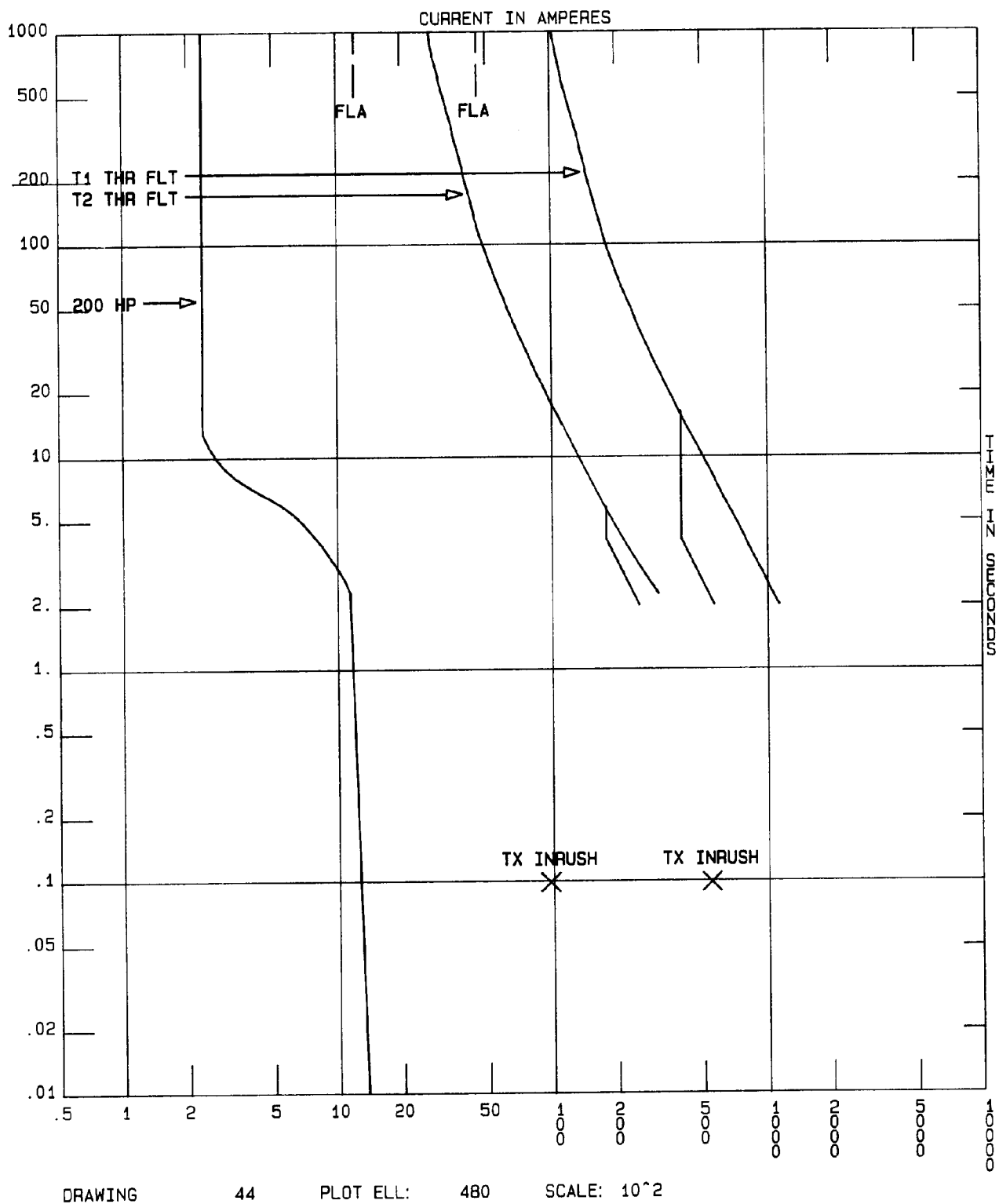
Figure 4-4. Key protection points.
