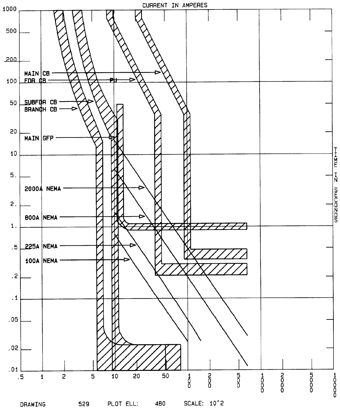
Figure 5-29. Improved ground-fault protection and coordination.
