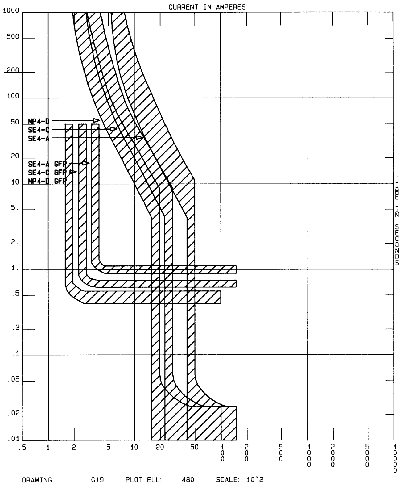
Figure G-19. Ground-fault protection at main, feeder, and branch (selective, time-coordinated).
