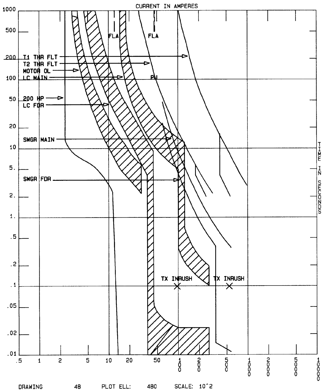
Figure 4-8. Switchgear main protection.
