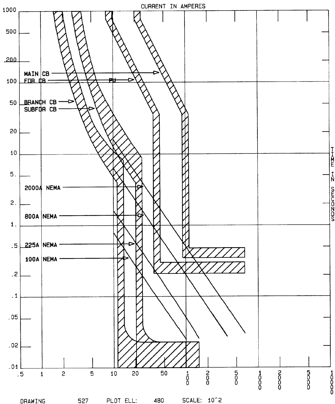
Figure 5-27. Standard overcurrent protection.
