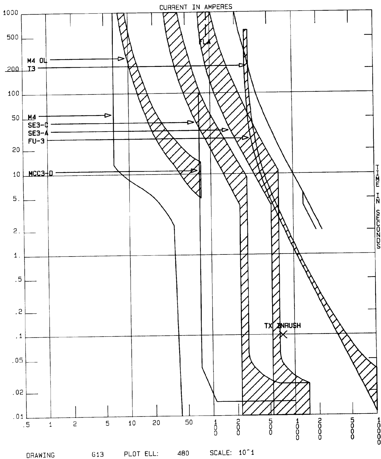
Figure G-13. Composite time-current curves for Example 2.
