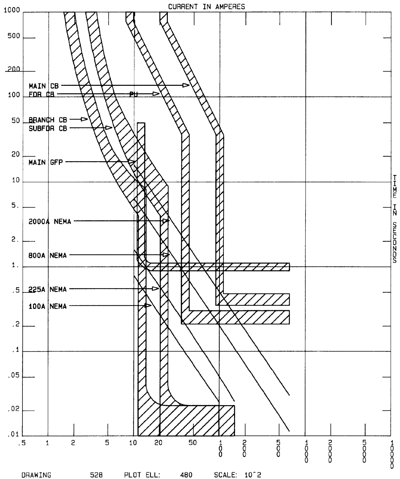
Figure 5-28. Main-only ground-fault protection.
