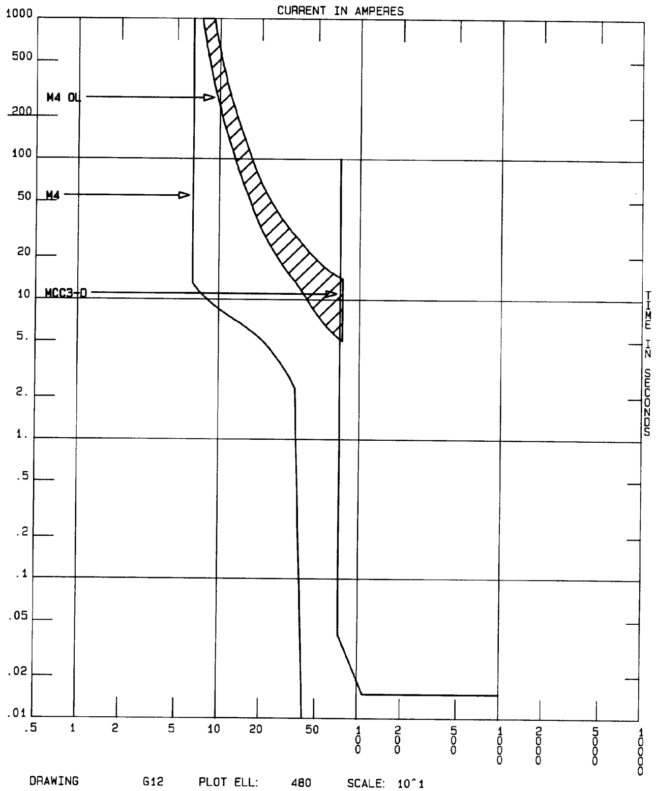
Figure G-12. M4 starting, overload, and MCP short-circuit protection curves.
