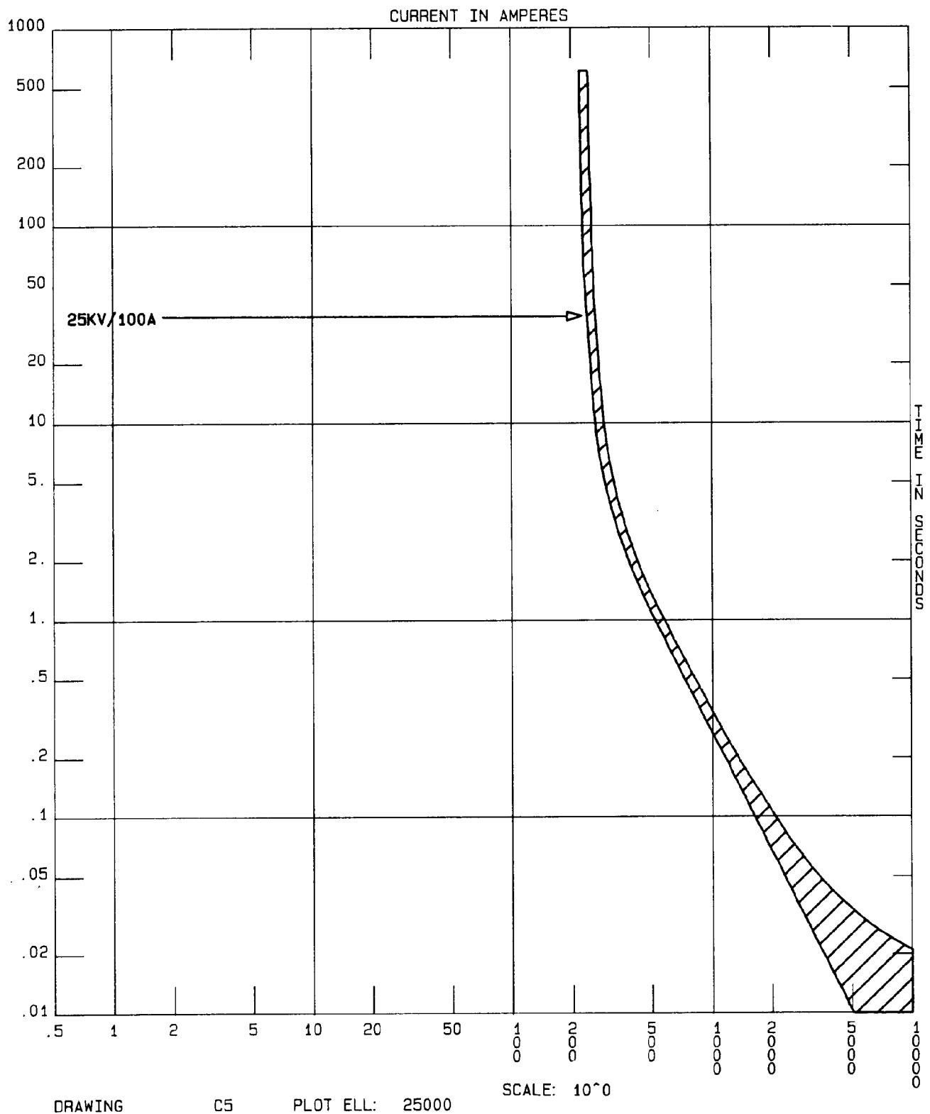
Figure C-5. Time-current characteristic curve for typical medium voltage fuse.
