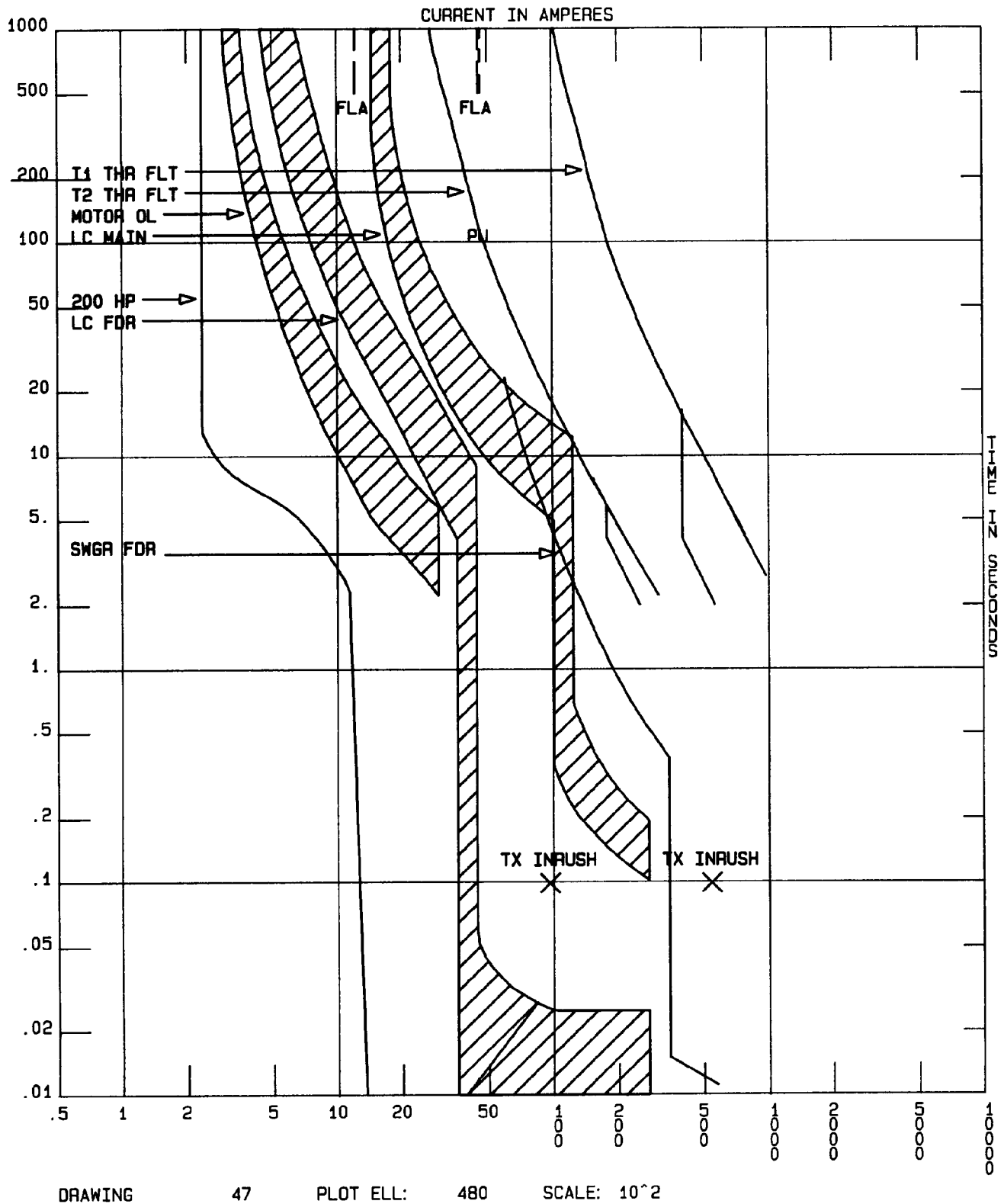
Figure 4-7. Switchgear feeder protection.
