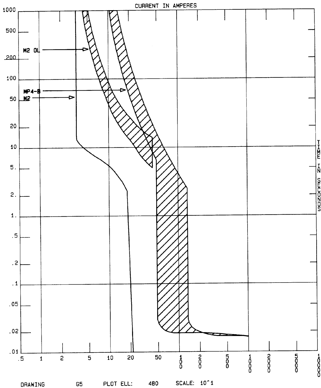
Figure G-5. M2 starting, overload, and CB short-circuit protection curves.
