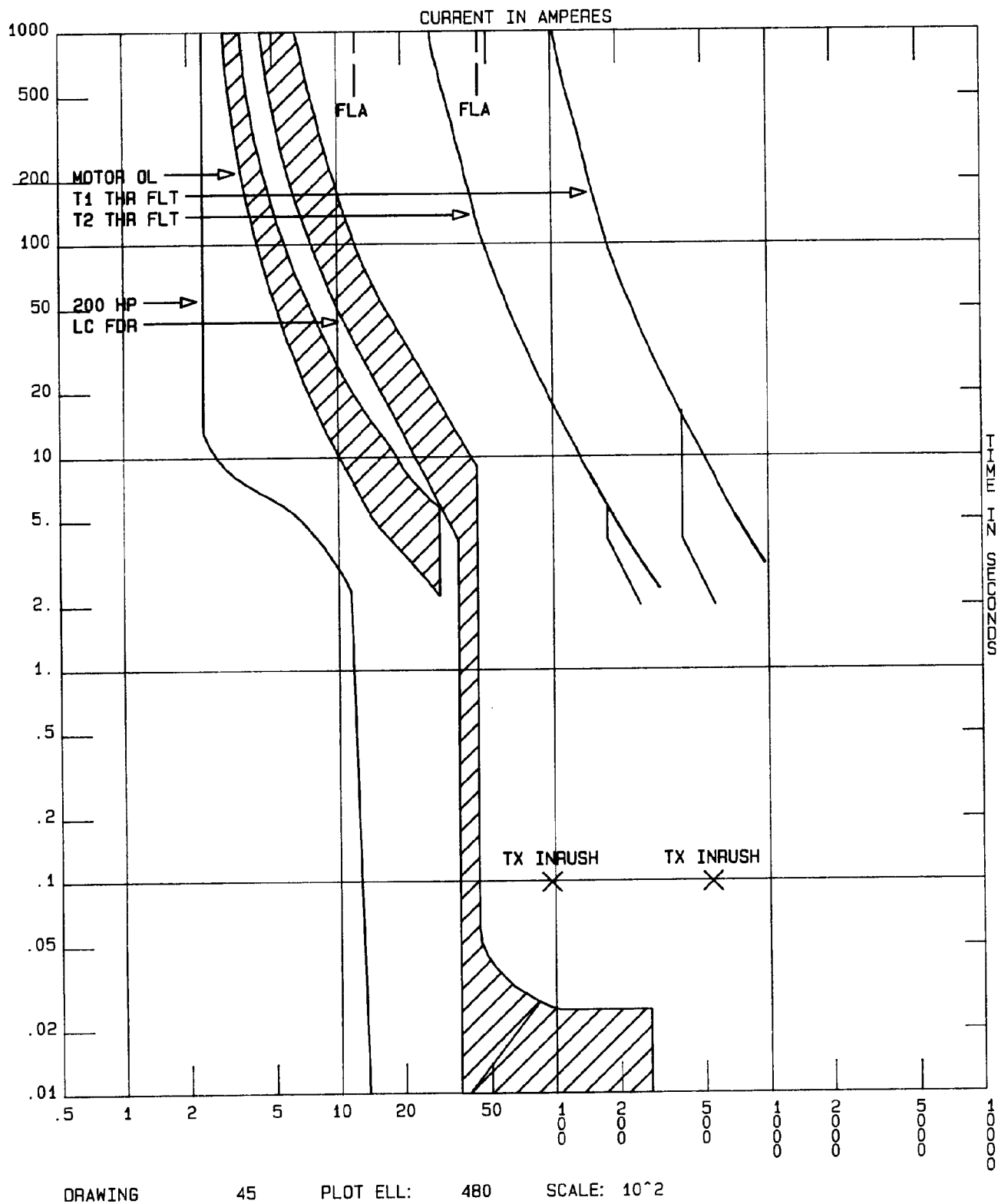
Figure 4-5. LC feeder protection.
