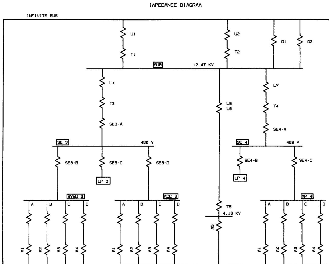
Figure G-20. Impedance diagram.
