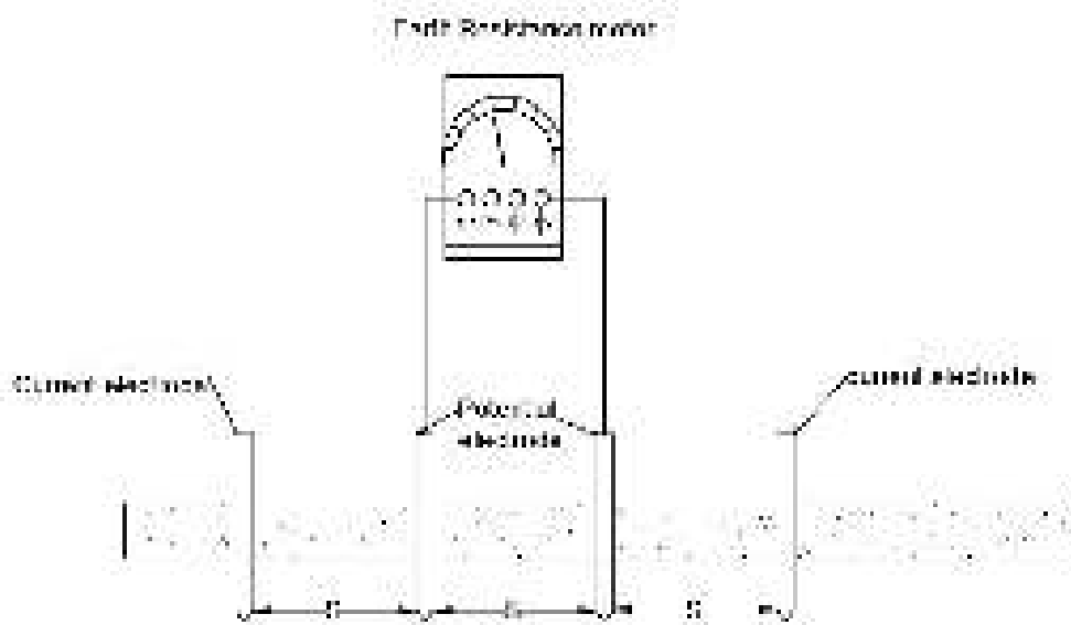
Figure 24. Connection for correction of potential electrode resistance
