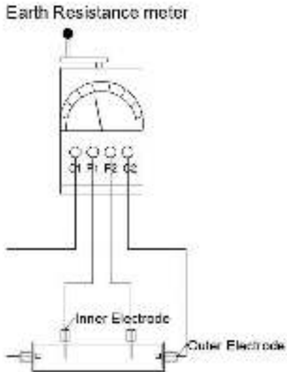
Figure 16. Measurement using four probe earth resistance meter
