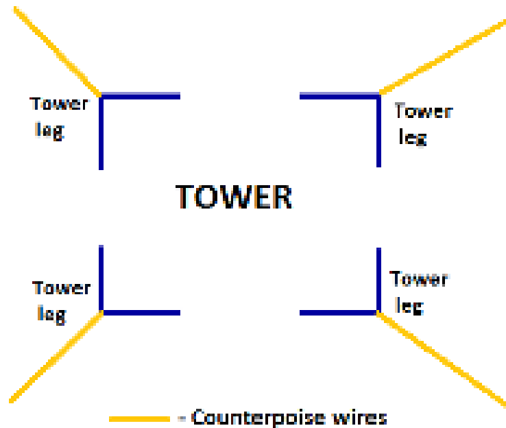
Figure 33. Counterpoise earthing
