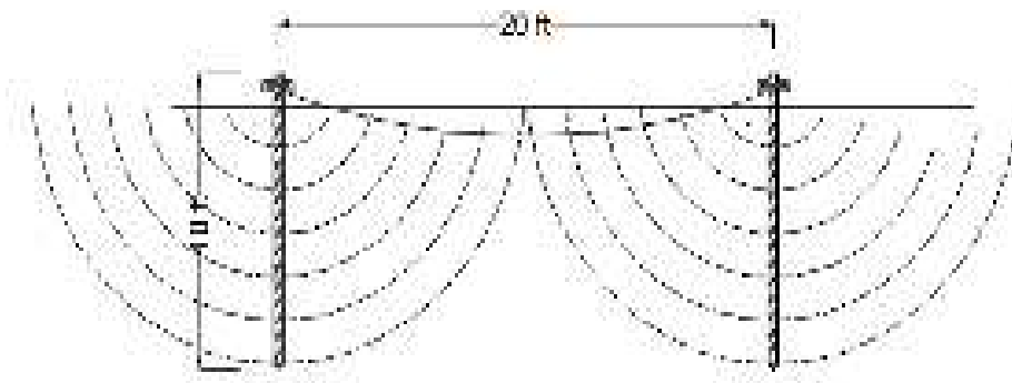
Figure 10. Proper spacing between earth electrodes
