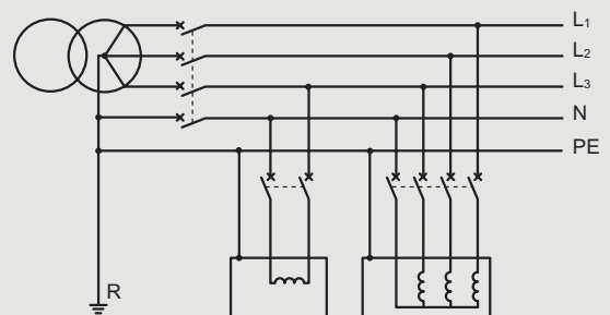
TN-S system
