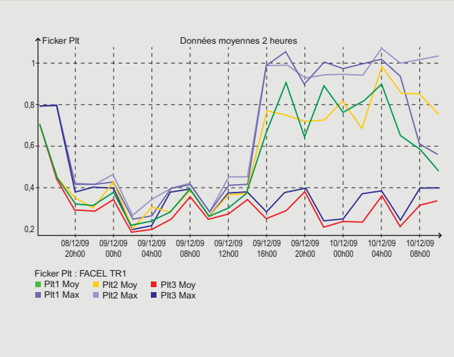
Example of recording showing flicker severity variations
