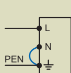
Single phase receiver
