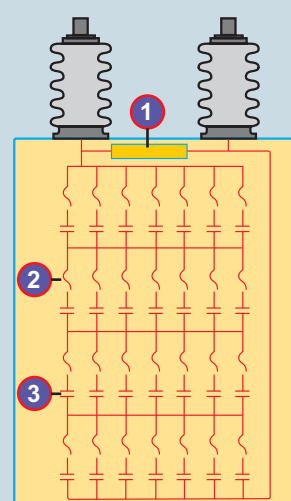
Internal view of an "all-film" HV capacitor with internal fuses
