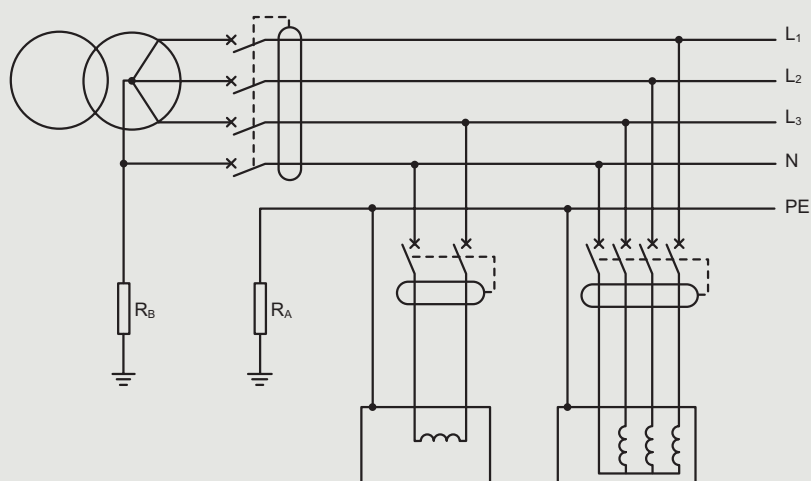
TT system
