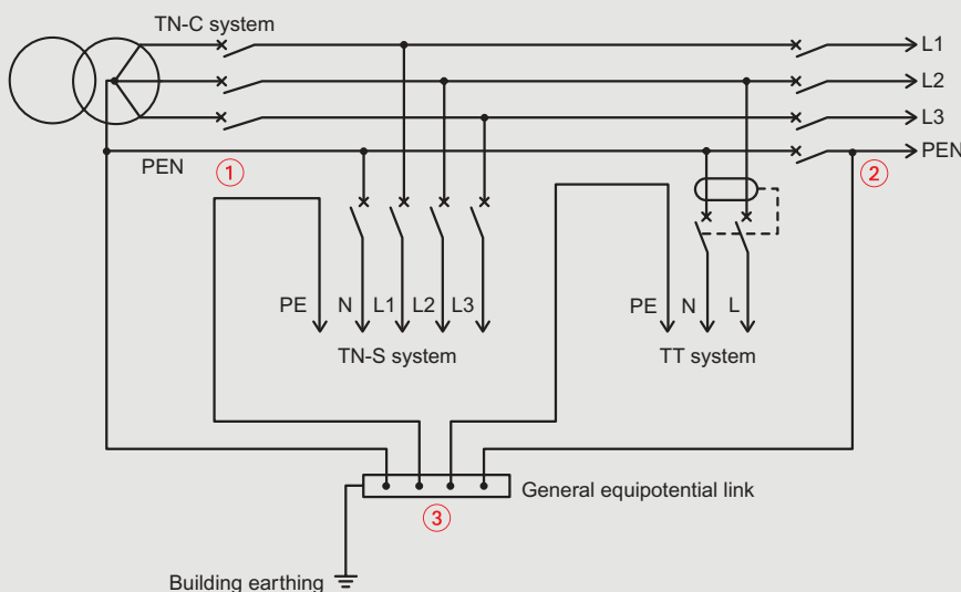
Schematic diagram of the power supply in the same building or in two buildings close to one another
