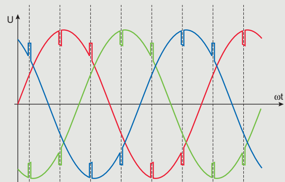
Illustration of undervoltages and overvoltages or "commutation notches"
