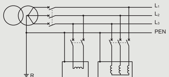
TN-C system
