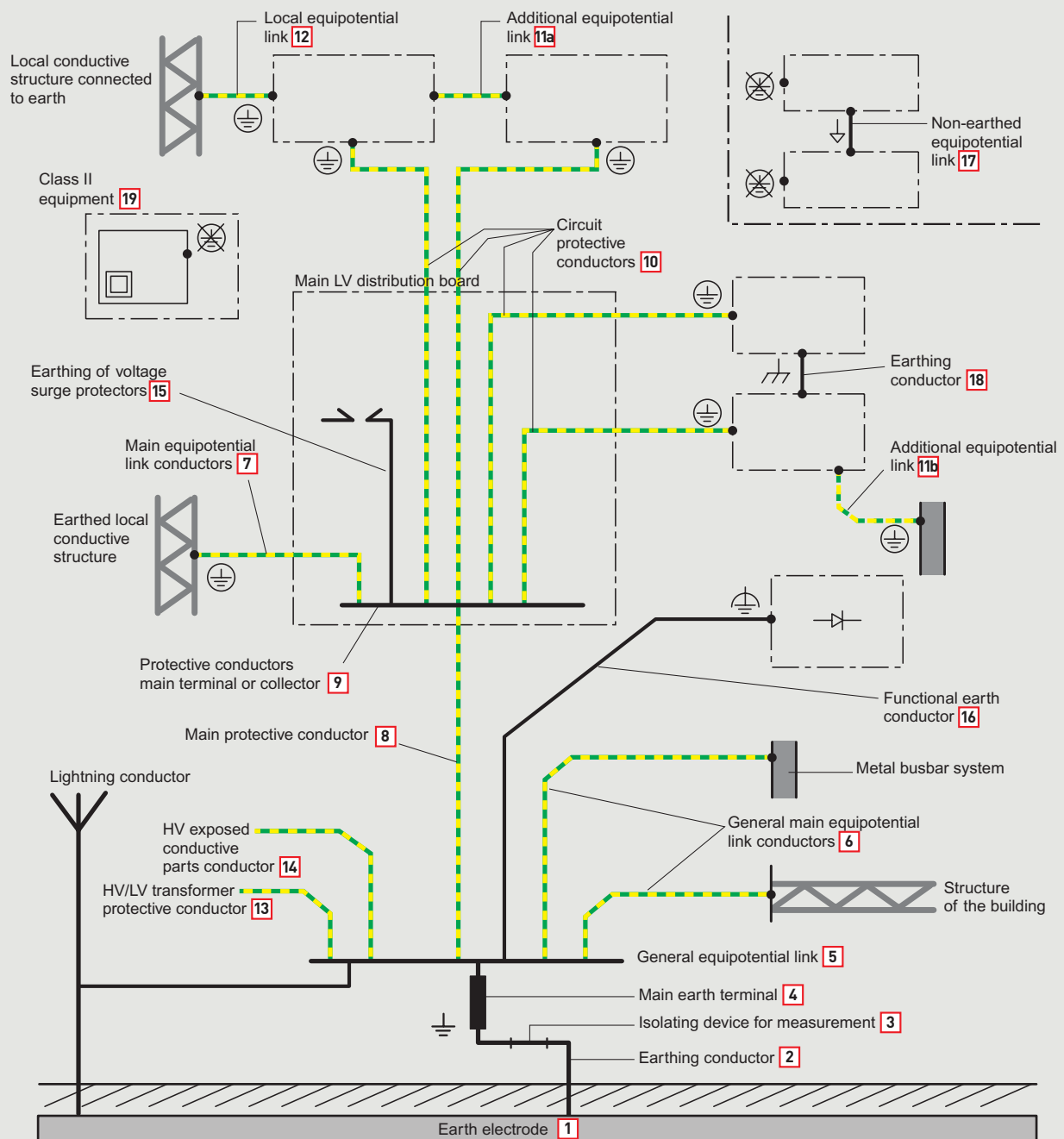
Diagram of the protection system (see definitions on the following pages)
