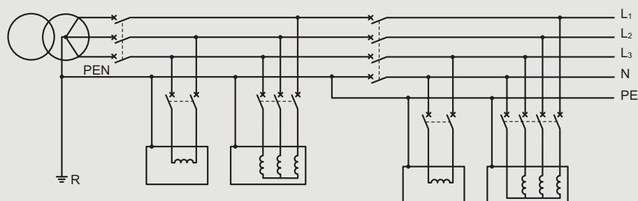
TN-C-S system
