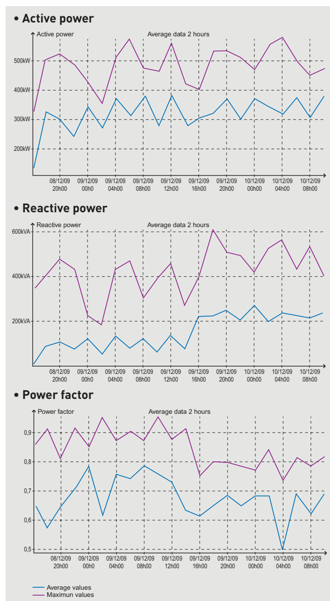
^ Examples of readings taken with Winalp 2400
