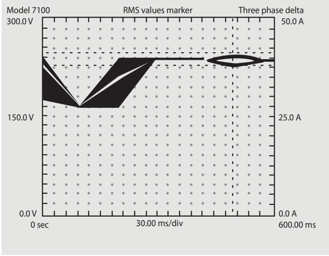
Example of recording of a voltage dip
