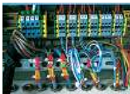
^ Connecting protective conductors by means of Viking green/yellow terminal blocks: the rail is used as collector
