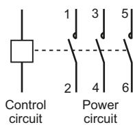
Fig. H7 Symbol for a monostable remote control switch (contactor, relay)
