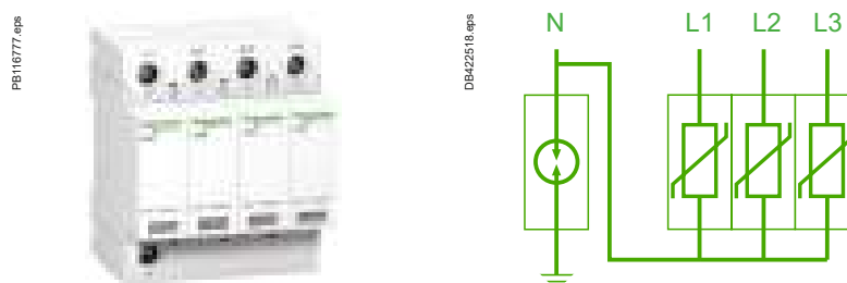
Fig. J52 The Schneider Electric brand iPRD SPD incorporates a gas discharge tube between neutral and earth and varistors between phase and neutral
