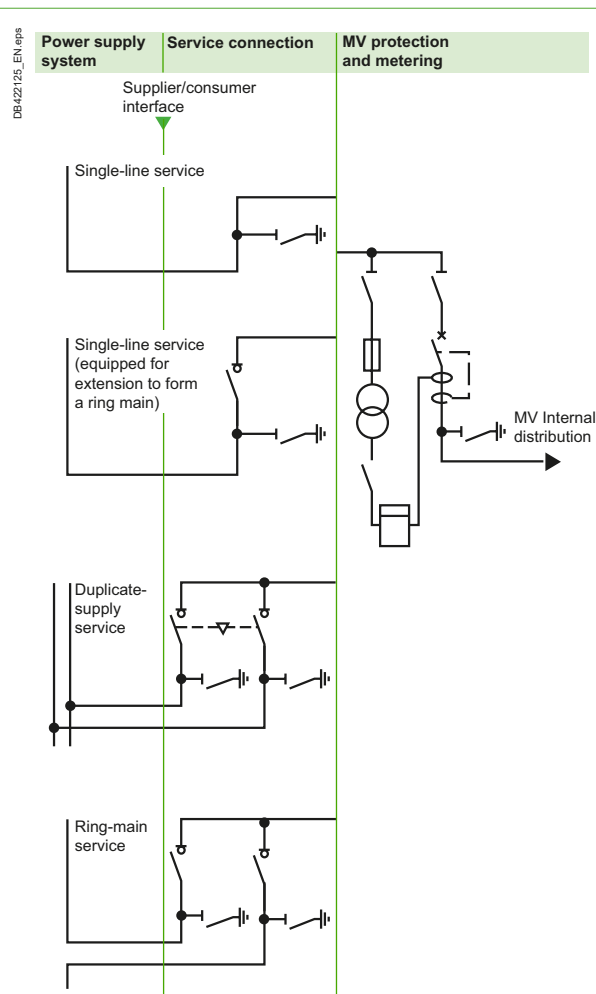
Fig. D9 MV connection with MV metering
