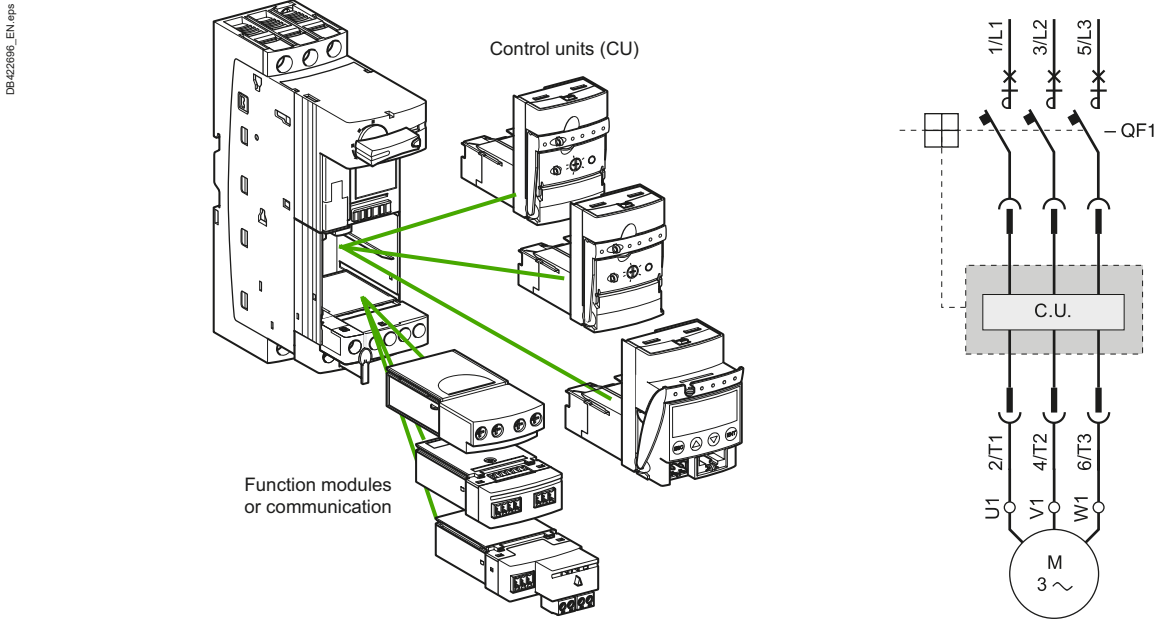
Fig. N86 Example of a CPS modularity (TeSys U starter controller by Schneider Electric)
