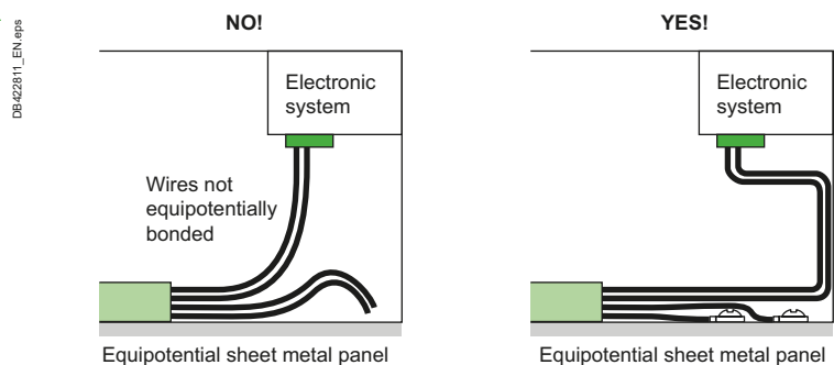
Fig. R45 Free wires must be equipotentially bonded
