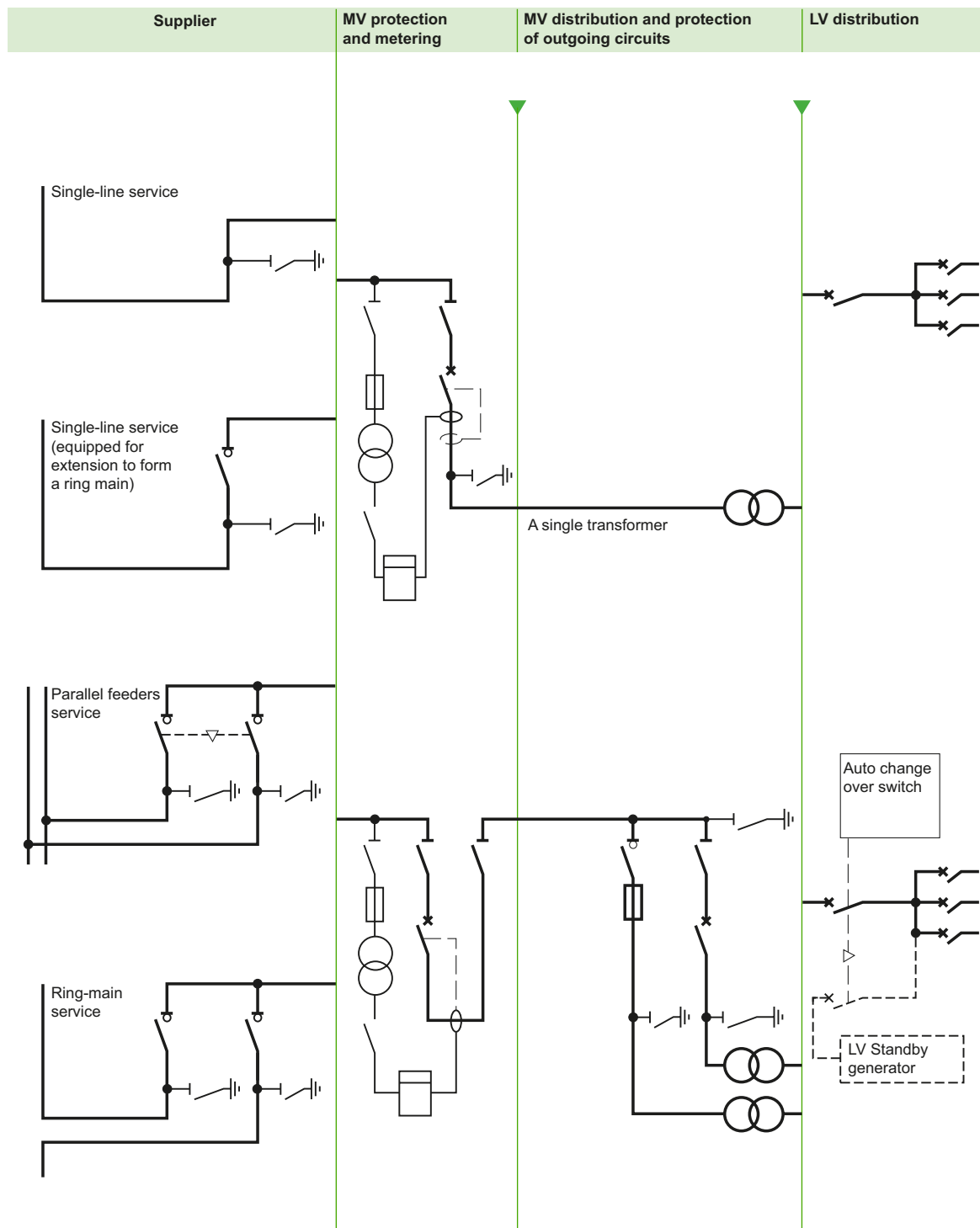
Fig. B34 Consumer substation with MV metering
