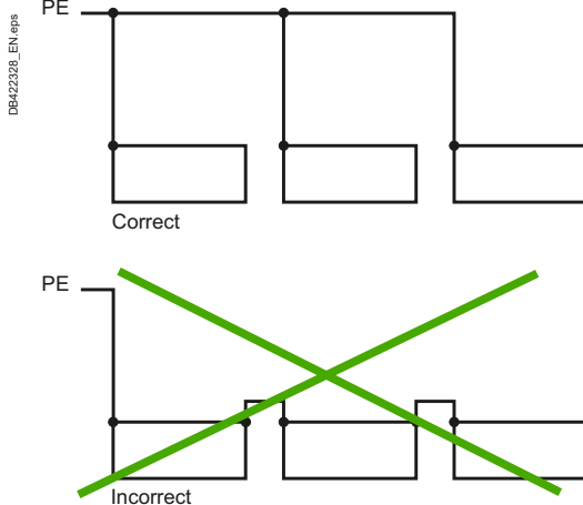
Fig. G55 A poor connection in a series arrangement will leave all downstream appliances unprotected
