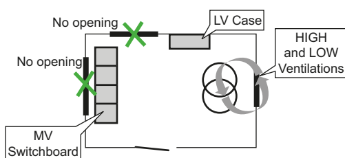
Fig. B44 Ventilation opening locations
