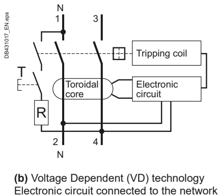
Fig. F47 The 2 technologies of RCDs
