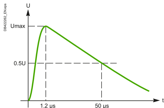
Fig. F54 Standardized 1.2/50 µs voltage transient wave
