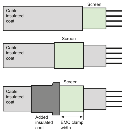
Fig. R18 Recommended screen preparation
