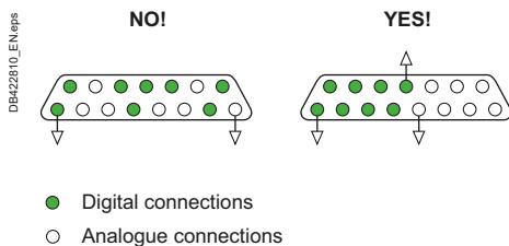
Fig. R44 Segregation applies to connectors as well!
