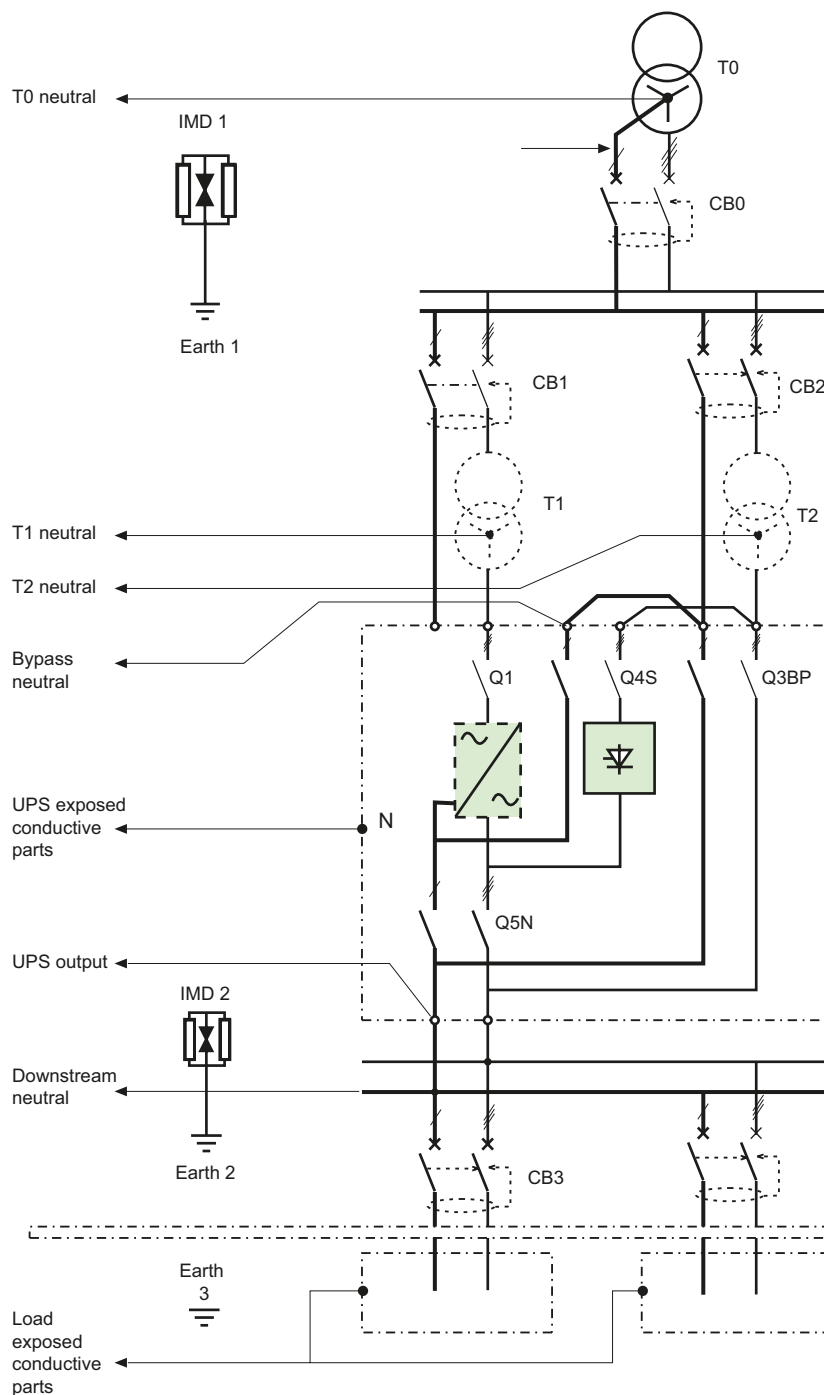
Fig. N24 The essential points that must be connected in system earthing arrangements
