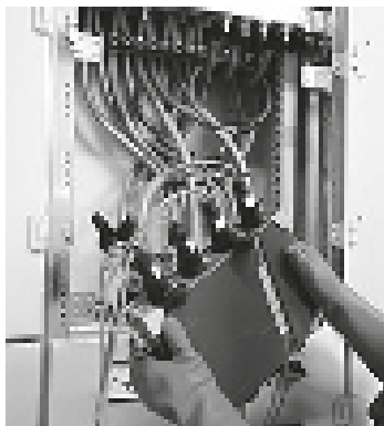
Fig. M11 Implementation of a digital Power Quality recorder within a cabinet
