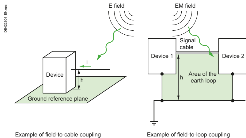
Fig. R38 Examples of radiated coupling
