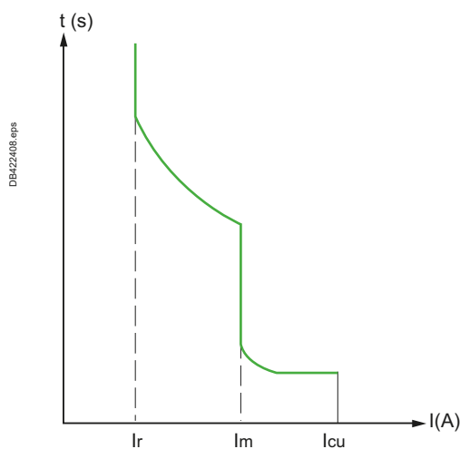
Fig. H29 Tripping curve of a thermal-magnetic circuit breaker
