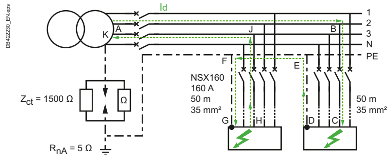
Fig. F37 Circuit breaker tripping on double fault situation when exposed-conductive-parts are connected to a common protective conductor
