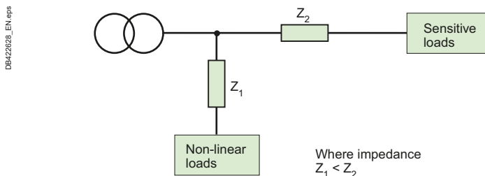
Fig. M24 Non-linear loads positioned as far upstream as possible (recommended layout)
