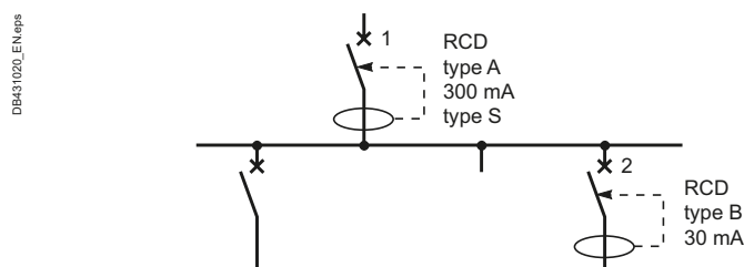
Fig. F65 Coordination between RCD type A and RCD type B
