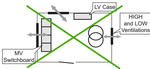
Fig. B43 Example of HV/LV prefabricated substation tested with 1250 kVA liquid filled transformer
