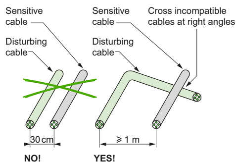
Fig. R40 Wiring recommendations for cables carrying different types of signals
