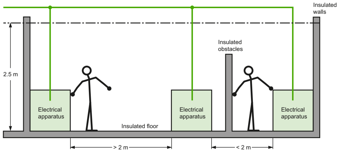
Fig. F70 Protection by out-of arm's reach arrangements and the interposition of non-conducting obstacles
