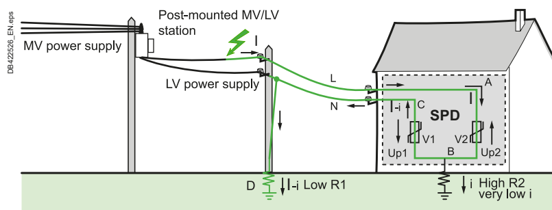
Fig. J61 Common protection only
