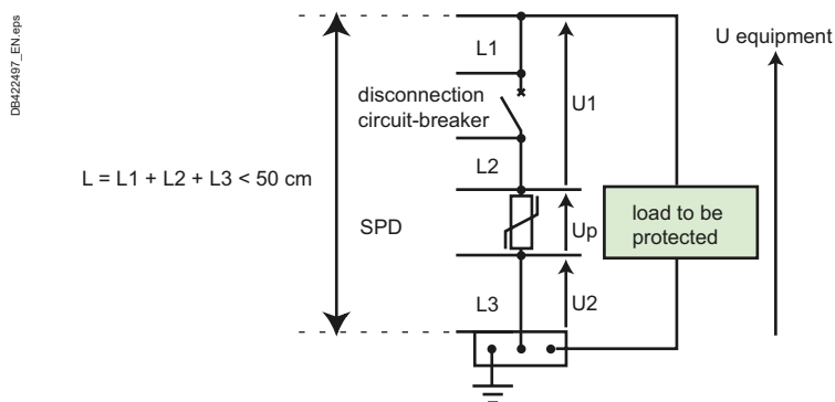
Fig. J38 Connections of a SPD L < 50 cm
