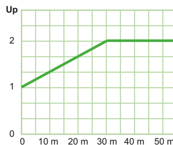
Fig. J60 Maximum voltage at the extremity of the cable according to its length to a front of incident voltage = 4kV/us
