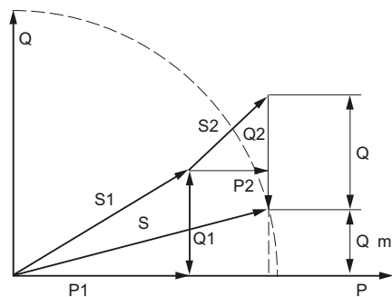
Fig. L19 Compensation Q allows the installation-load extension S2 to be added, without the need to replace the existing transformer, the output of which is limited to S
