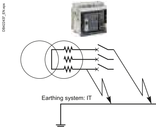
Fig. H42 Double earth fault situation
