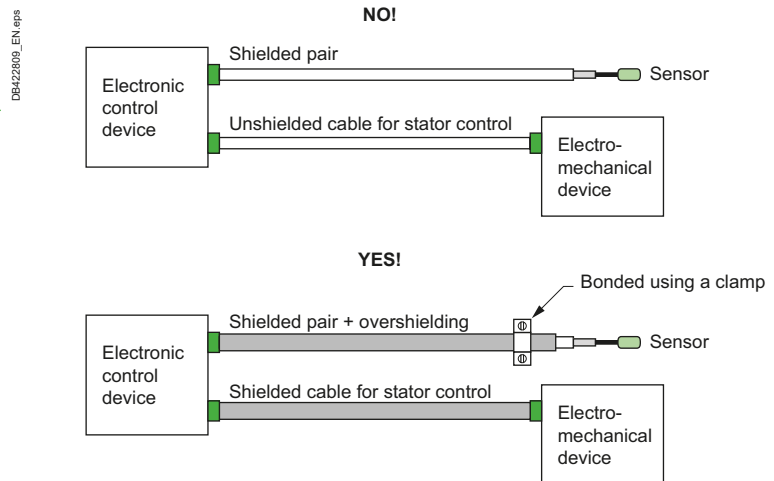
Fig. R43 Shielding and overshielding for disturbing and/or sensitive cables
