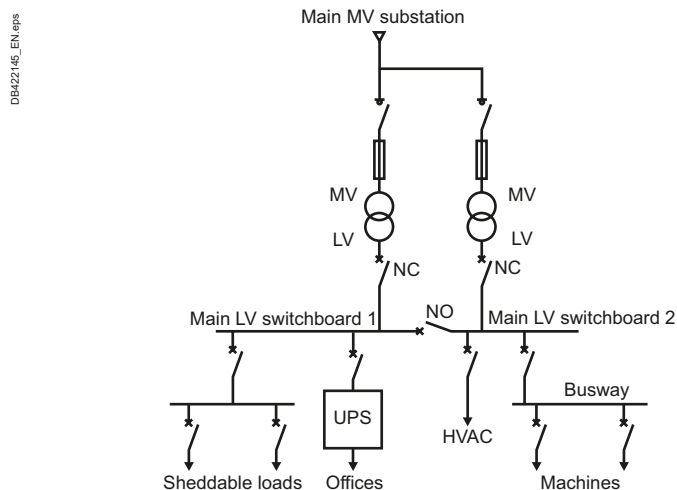
Fig. D32 Detailed single-line diagram (1 substation based on fig.D22)
