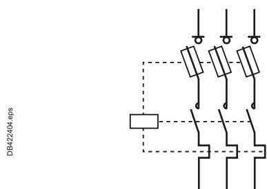
Fig. H18 Symbol for a fuse-switch disconnector + disconnector
