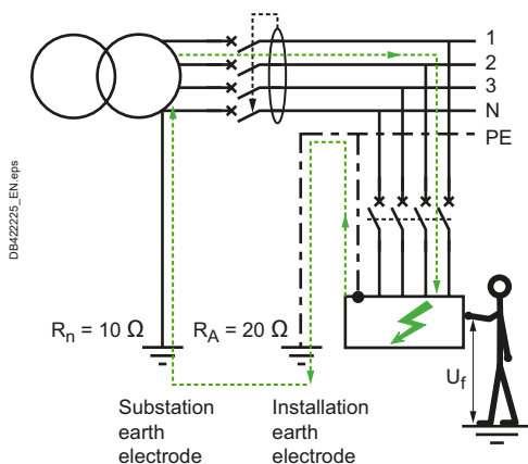
Fig. F11 Automatic disconnection of supply for TT system
