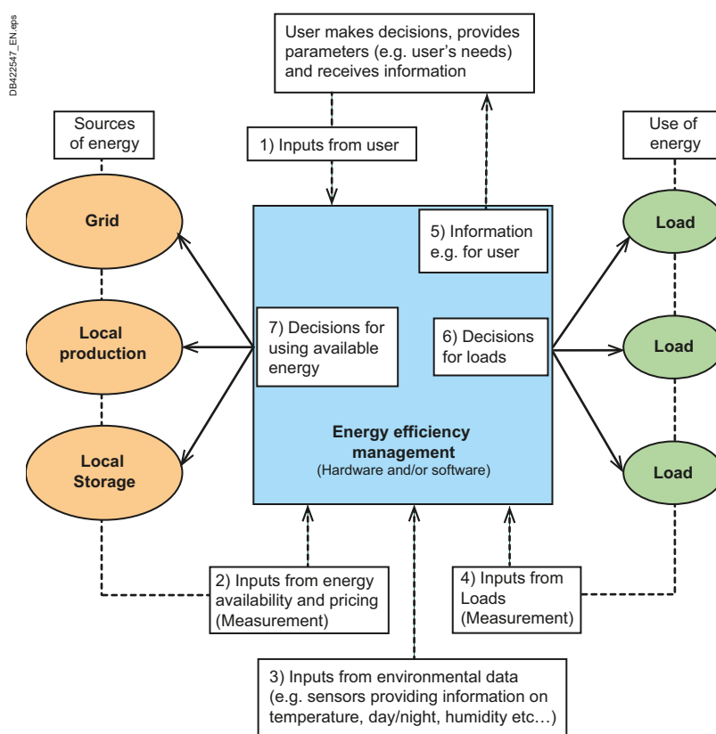
Fig. K9 Energy Efficiency and load management system
