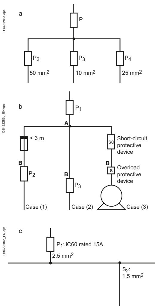
Fig. G7 Location of protective devices
