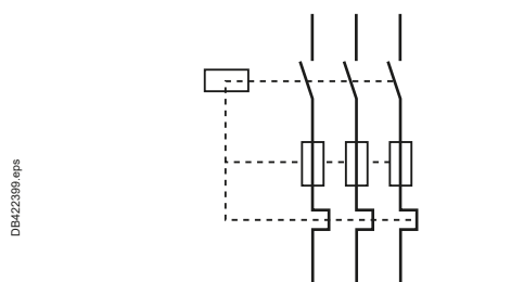
Fig. H14 Symbol for an automatic tripping switch-fuse
