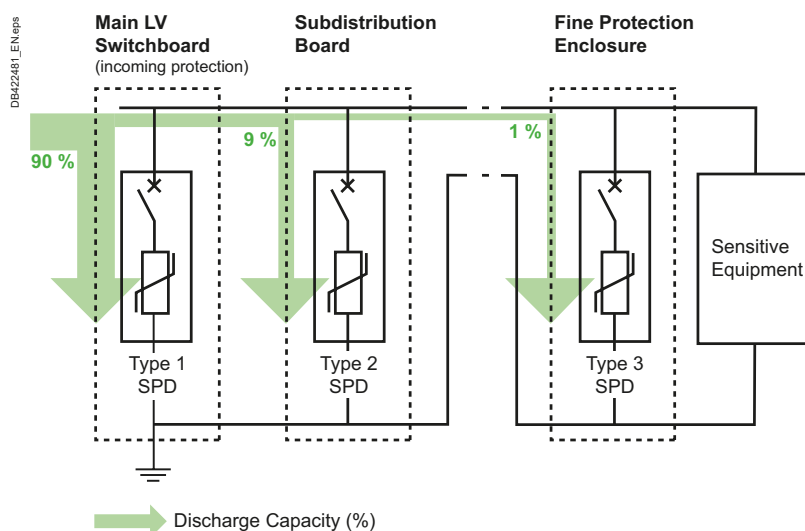
Fig. J22 Fine protection architecture
