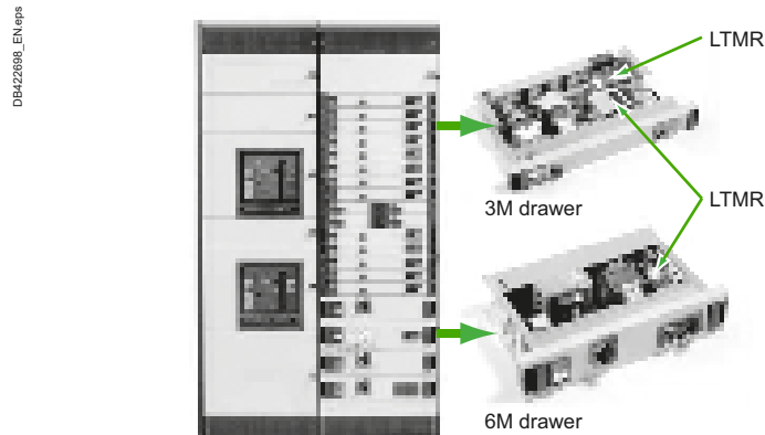
Fig. N89 Example of iPMCC: Okken switchboard and drawers by Schneider Electric
