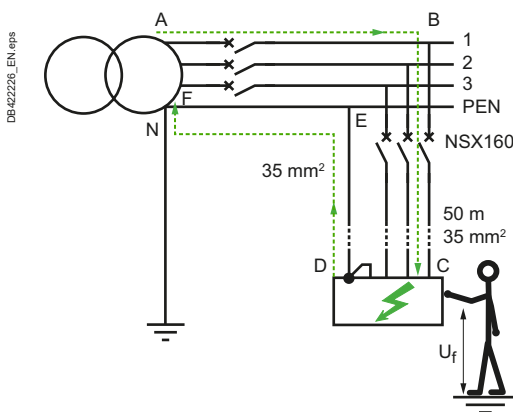
Fig. F18 Automatic disconnection in TN system
