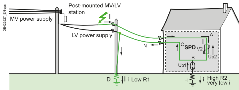
Fig. J62 Common and differential protection
