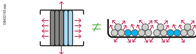
Fig. E58 Double-neutral installation for cable solution is not directly applicable for busway solution, due to their very different thermal dissipation behaviour.
