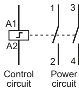
Fig. H6 Symbol for a bistable remote control switch (impulse relay)
