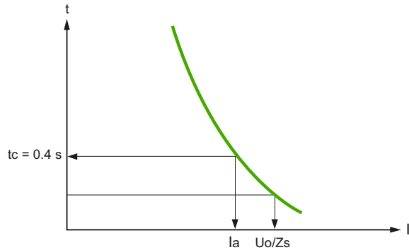
Fig. F21 Disconnection by fuses for a TN system
