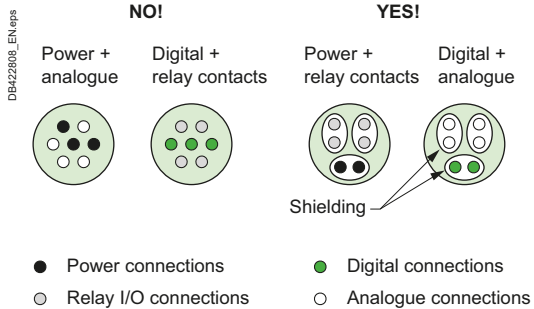
Fig. R42 Incompatible signals = different cables
