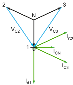
Fig. F34 Vector representation of voltages and currents in case of fault between phase 1 and earth
