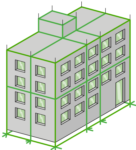
Fig. J14 Meshed cage (Faraday cage)
