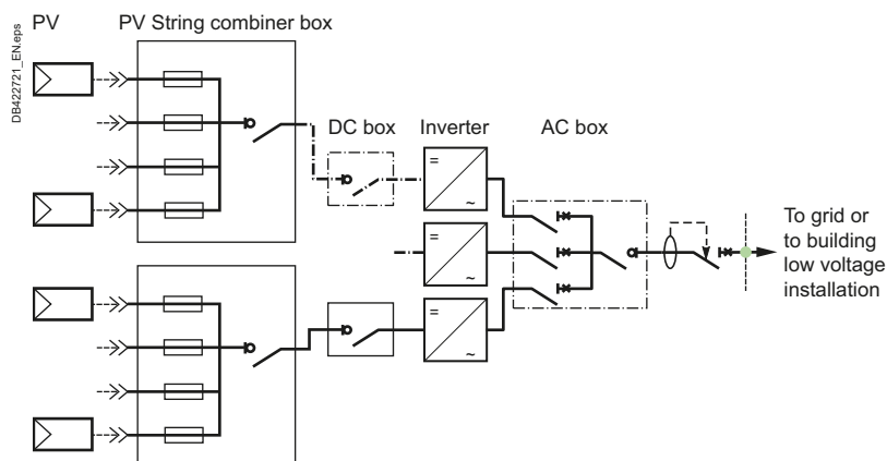
Fig. P19 Diagram showing a multi-string photovoltaic array with several single-phase inverters connected in a three-phase arrangement
