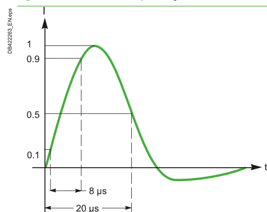
Fig. F55 Standardized current-impulse wave 8/20 µs
