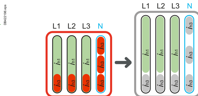
Fig. E61 The most effective solution = reduce the current density in ALL conductors, by selecting proper busway rating (single-neutral)
