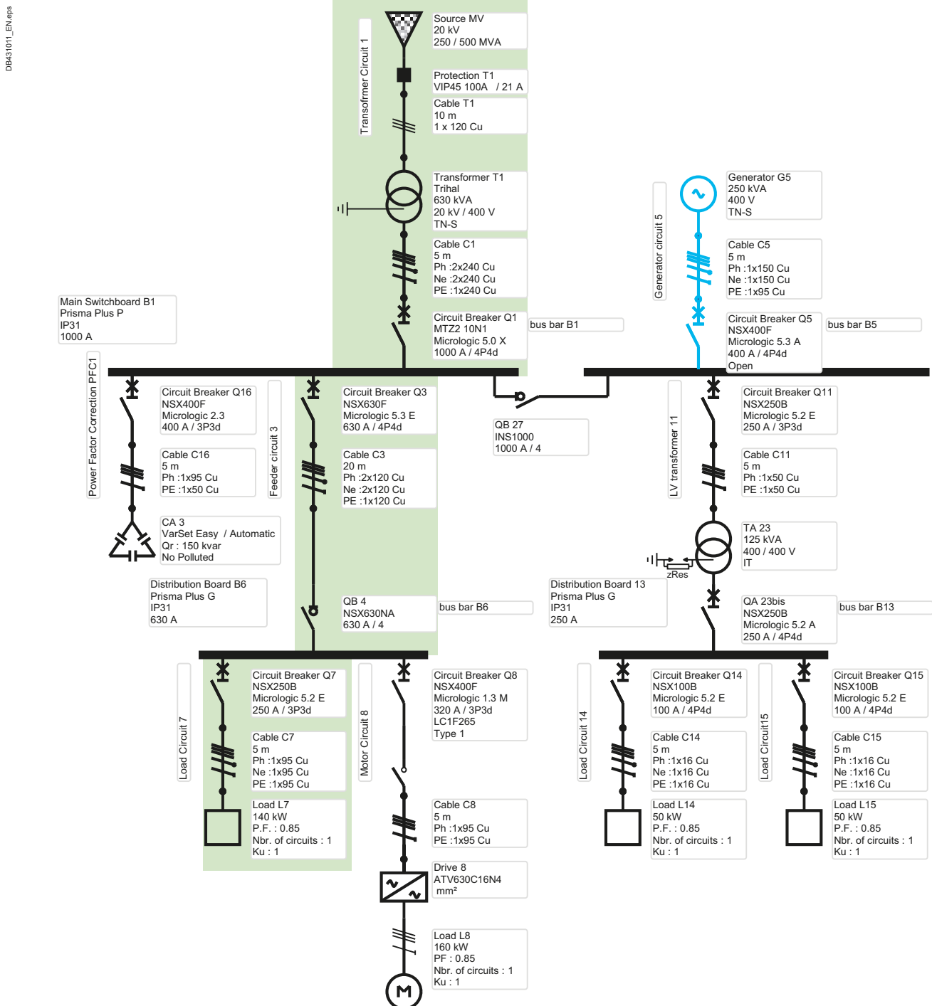
Fig. G69 Example of single-line diagram
