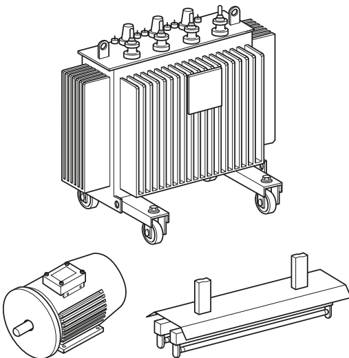
Fig. L6 Power consuming items that also require reactive energy
