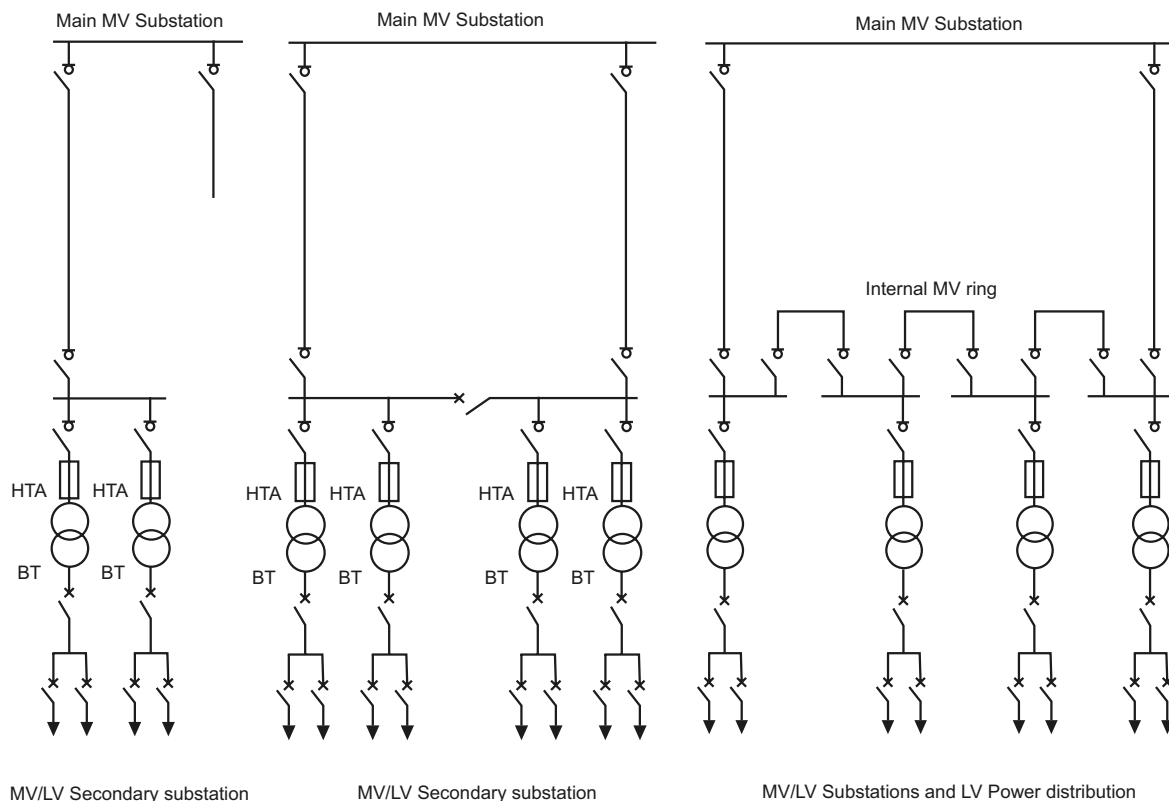
Fig. D11 Single feeder, Dual feeder, Open ring
