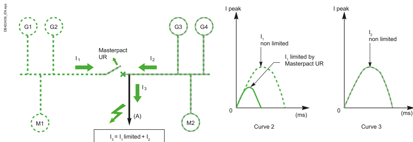
Fig. H60 Diagram of the network with Masterpact UR added as tie breaker
