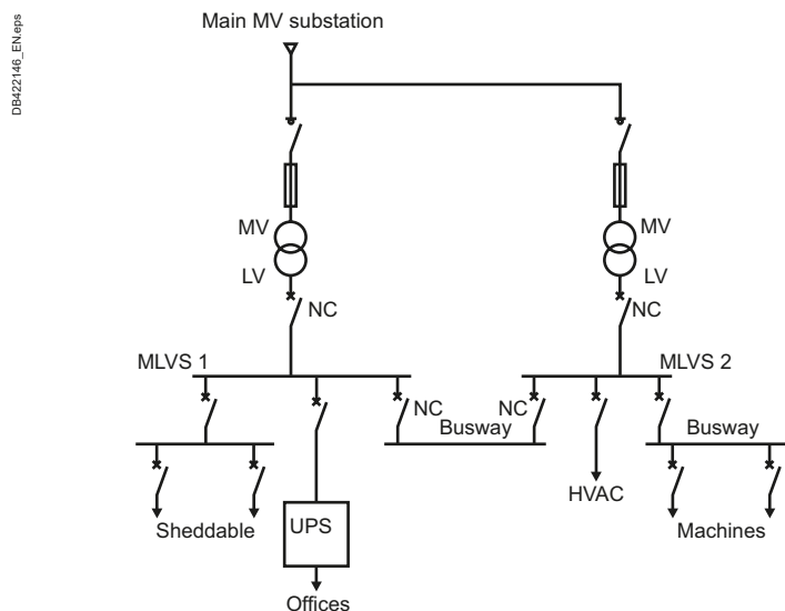
Fig. D33 Detailed single-line diagram (2 substation based on fig.D24)
