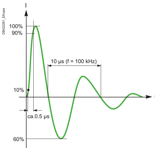
Fig. F53 Standardized 0.5 μs/100 KHz current transient wave
