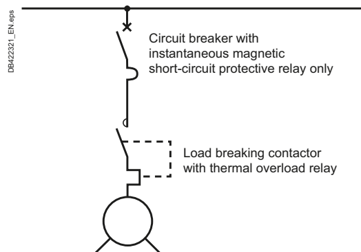
Fig. G44 Circuit protected by circuit breaker without thermal overload relay
