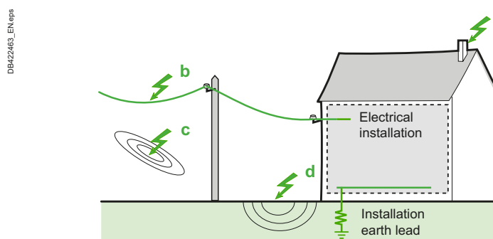
Fig. J5 Various types of lightning impact
