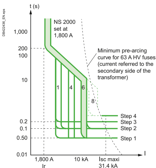
Fig. H57 Curves of MV fuses and LV circuit breaker
