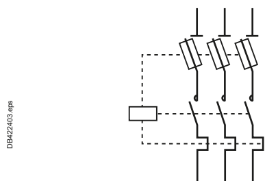
Fig. H17 Symbol for a fuse disconnecter + disconnector
