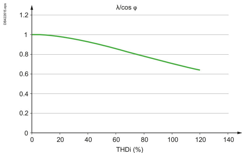
Fig. M6 Variation of \lambda/\cos\varphi as a function of \text{THD}_i , for \text{THD}_u \sim 0
