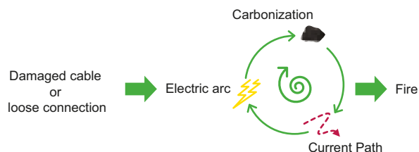
Fig. F82 Arc fault generation
