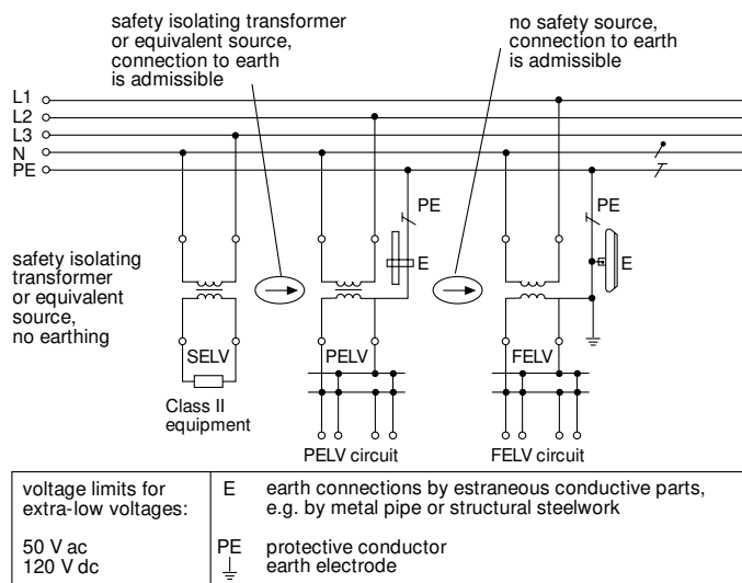
Figure 1: SELV, PELV, FELV systems
