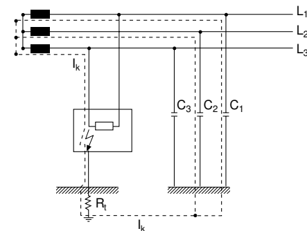
Figure 3: Earth fault in IT systems
