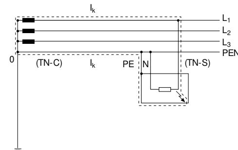
Figure 2: Earth fault in TN systems
