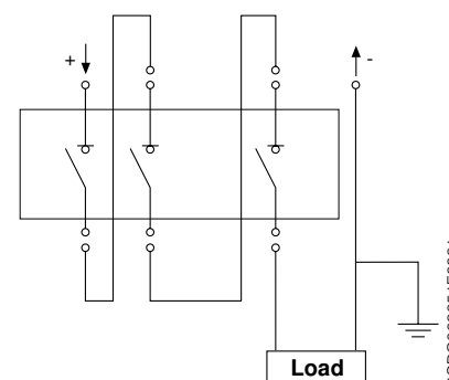
I) 3 poles in series (750 Vdc)
