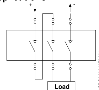
G) 2+1 poles in series (750 Vdc)
