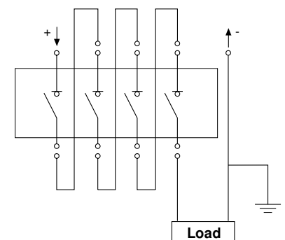
H) 4 poles in series (1000 Vdc)
