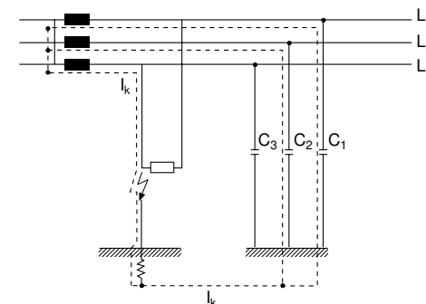
Figure 3: Earth fault in IT system
