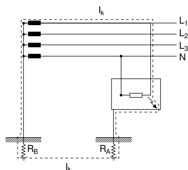
Figure 1: Earth fault in TT systems
