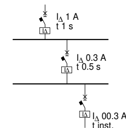
Figure 3: Vertical discrimination between RCDs
