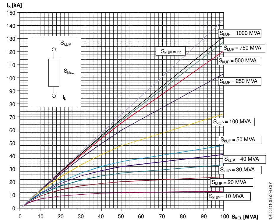
Figure 1: Chart for the calculation of the three phase short-circuit current at 400 V
