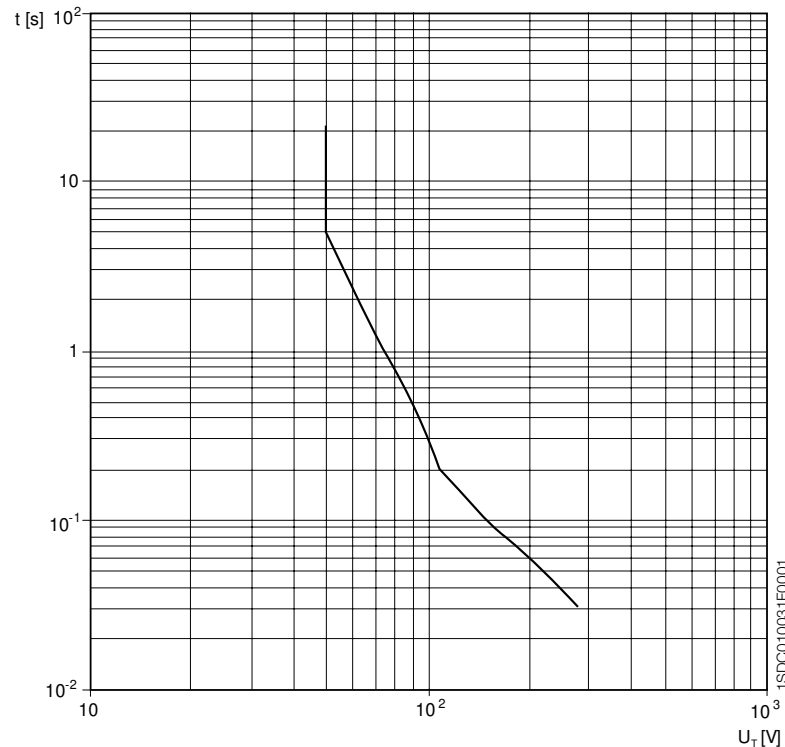
Figure 2: Safety curve
