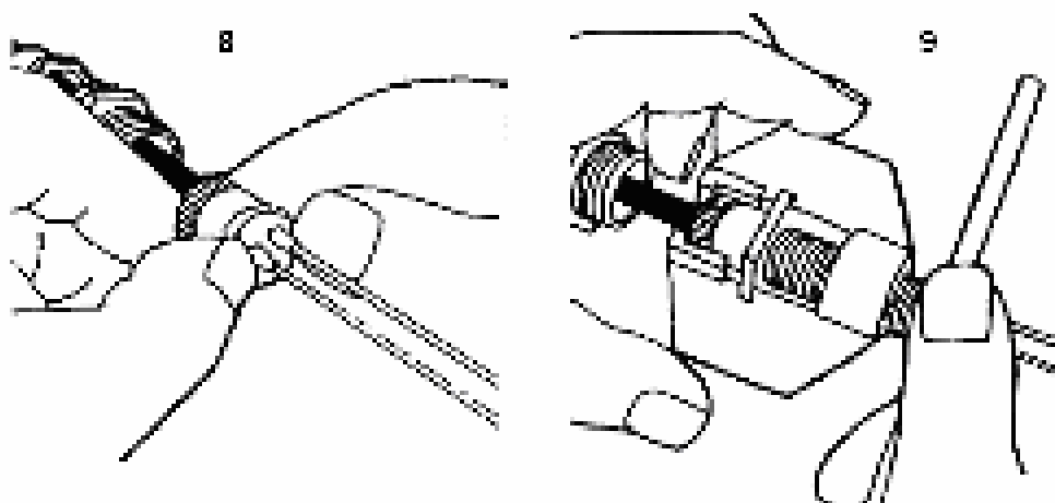
Figure 45: Fitting the gland and seal steps 8, 9
