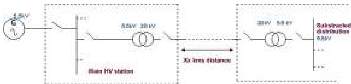
Figure 66: HV connections
