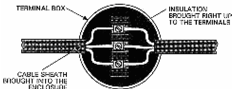
Figure 154: Terminal Connections
