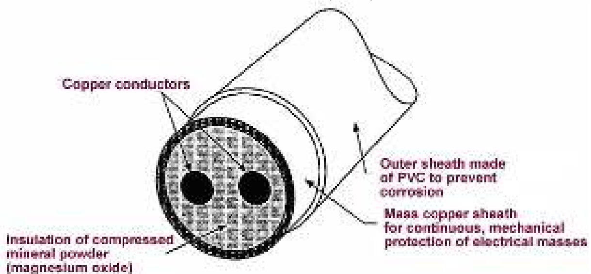
Figure 15: Construction of a mineral insulated cable
