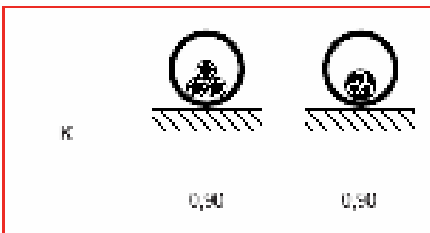
Figure 64: Cables laid in spaced pipes – free air single layer
