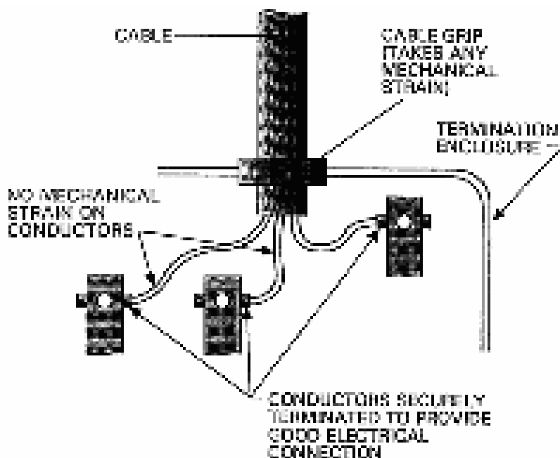
Figure 152: Cable Termination.
