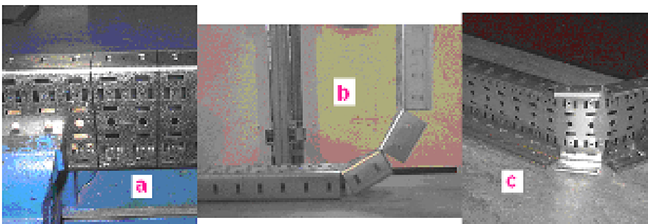
Figure 95: Construct a 90° external bend
