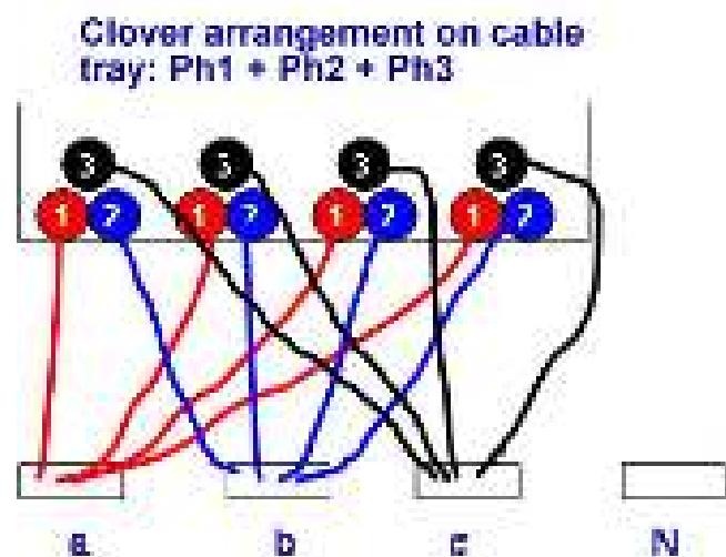
Figure 225: Clover-lead distribution of cables
