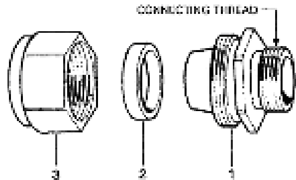
Figure 200: 16-20 BWL Gland
