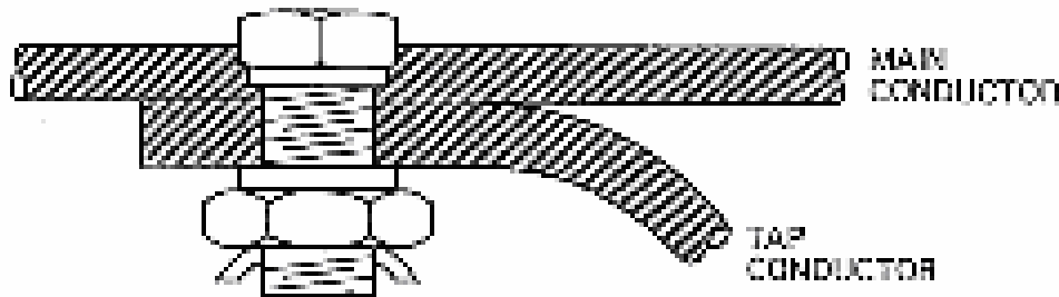
Figure 174: Split-Bolt Connector
