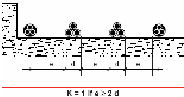
Figure 54: Cables laid spaced in free air – unperforated tray
