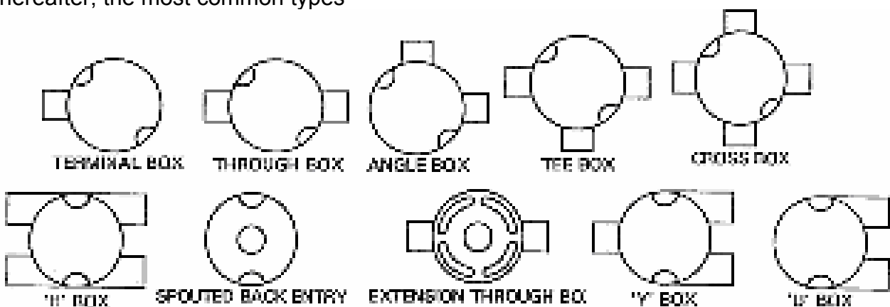
Figure 102: Different Types of Circular Conduit Boxes
