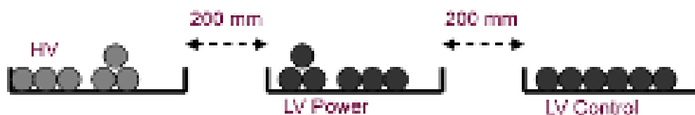
Figure 72: Horizontal distances between cable trays
