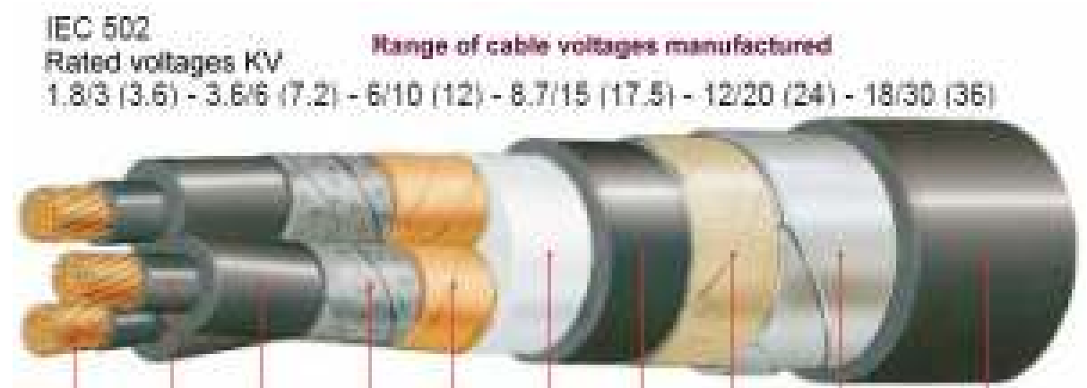
Figure 70: Three-pole cable with radial field/armoured
