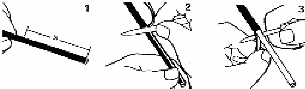
Figure 35: Removing PVC Outer-sheath
