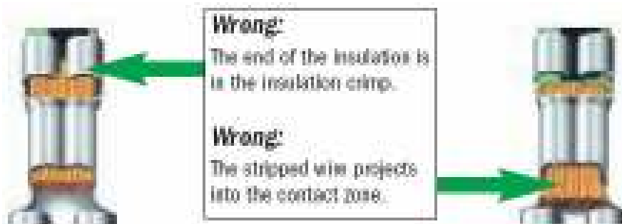
Figure 188: Wrong positions of wire on lugs
