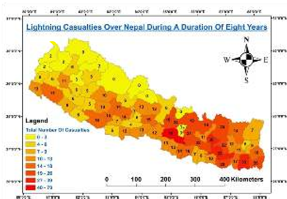
Fig 7: Spatial distribution of lightning fatalities over the 77 districts of Nepal.
