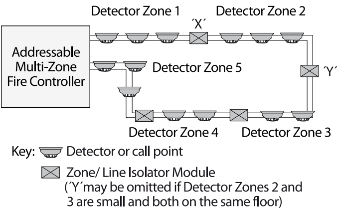
fig 3. Addressable Loop System Circuit
