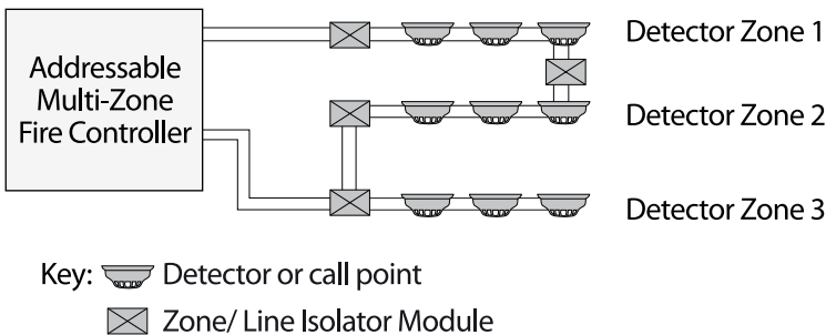
fig 4. Addressable Loop System Circuit with Spurs
