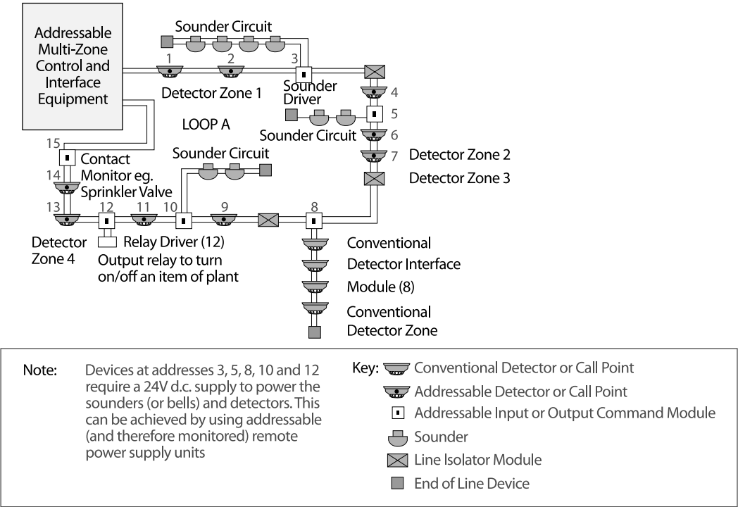
fig 5. Addressable Loop System Circuit with Conventional Spur and Addressable Output Modules
