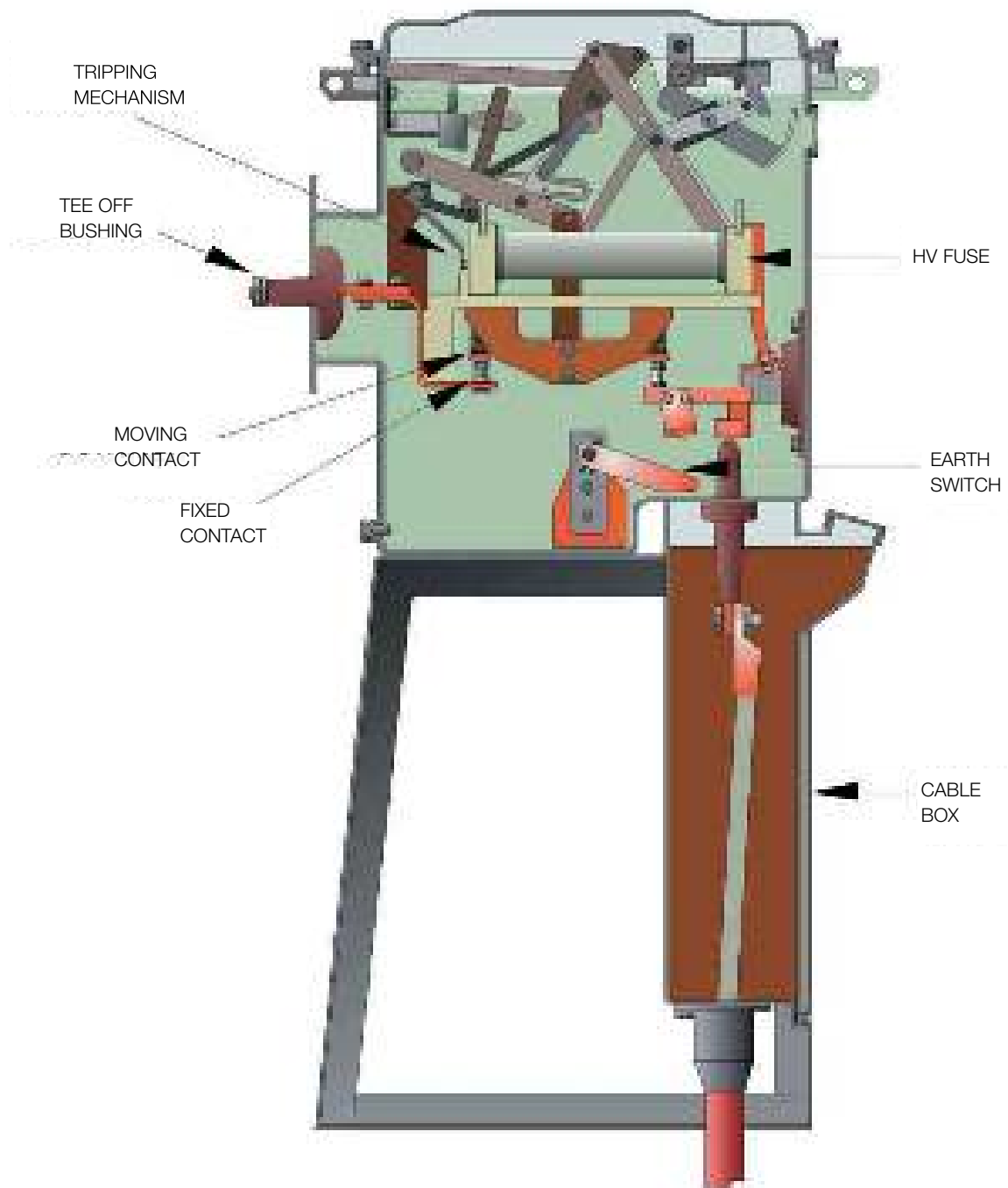
Figure 10 Typical arrangement of an 11 kV oil fuse switch
