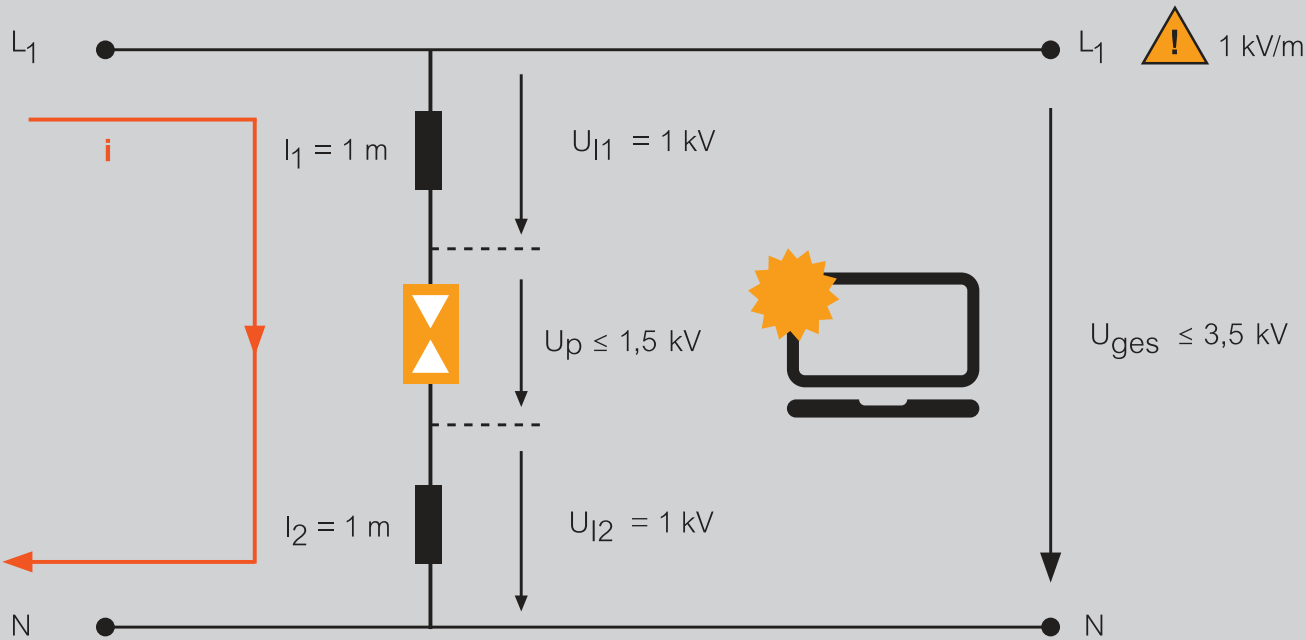
Voltage drop on the supply line when surge current is applied ( i = lightning current, U_{total} = surge voltage at protection device)
