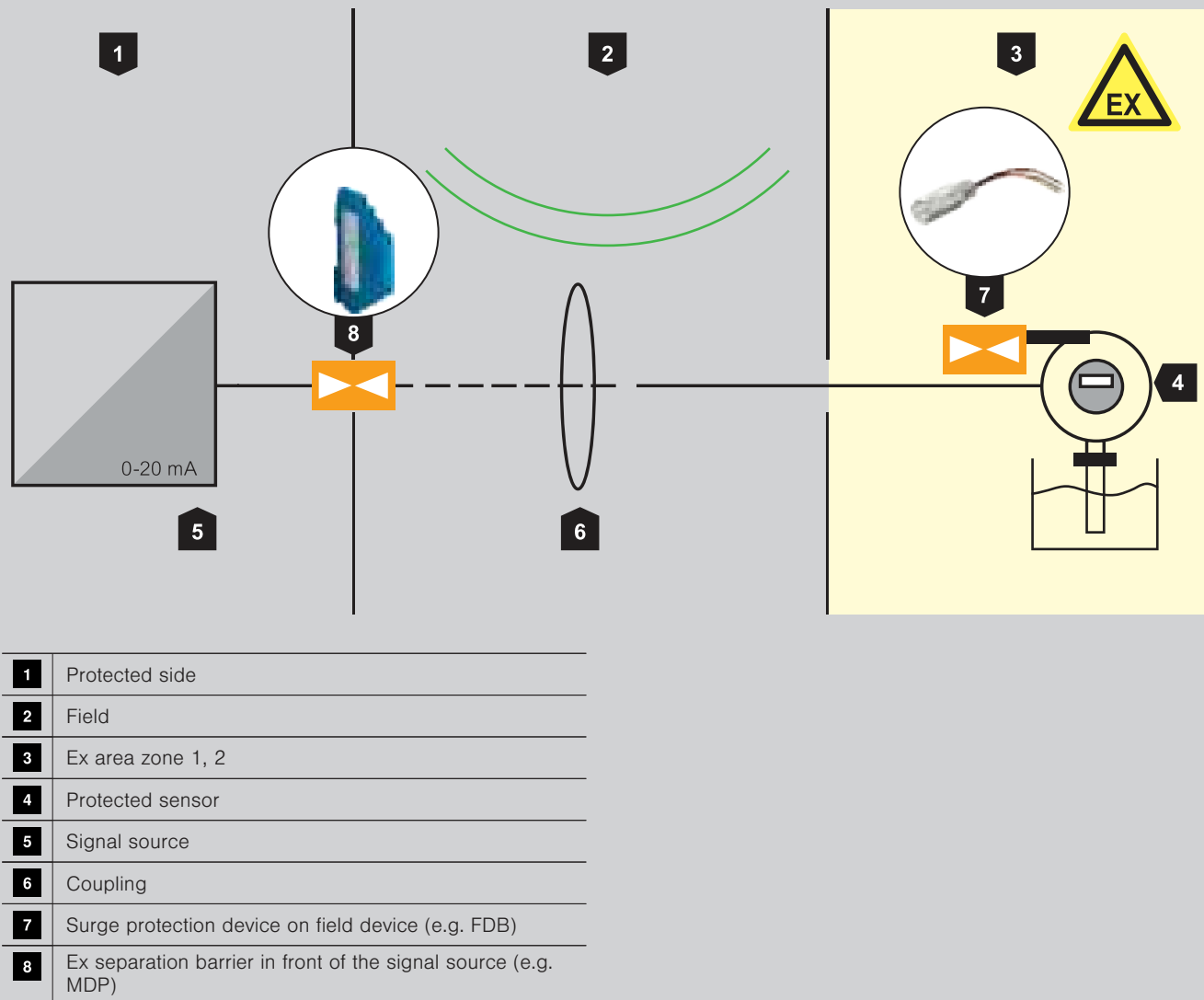
Application example – protection of a measurement/control signal line in an ex area
