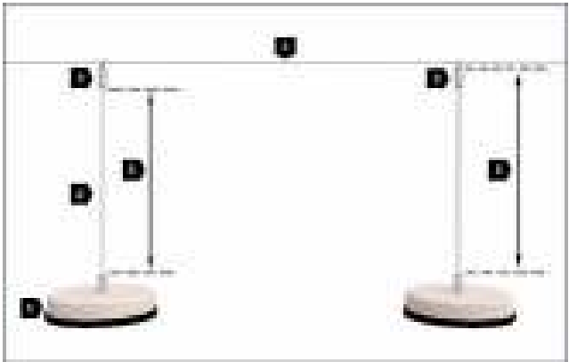
Insulated external lightning protection system with insulators
