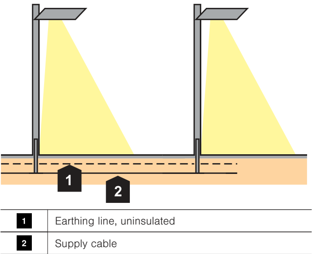
Cable routing
