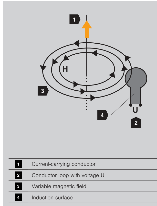
Induction in a conductor loop
