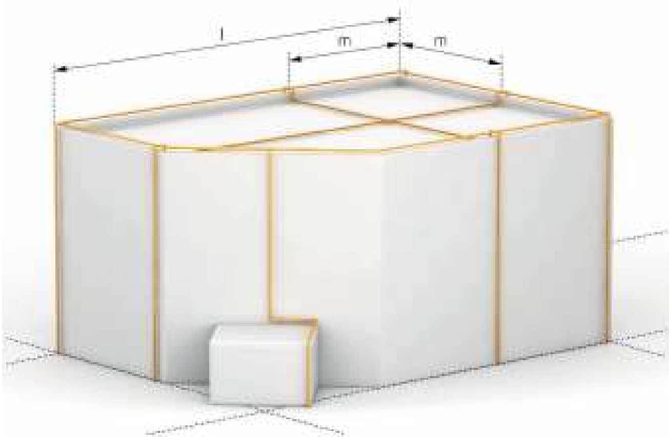
Grid system on a flat roof
