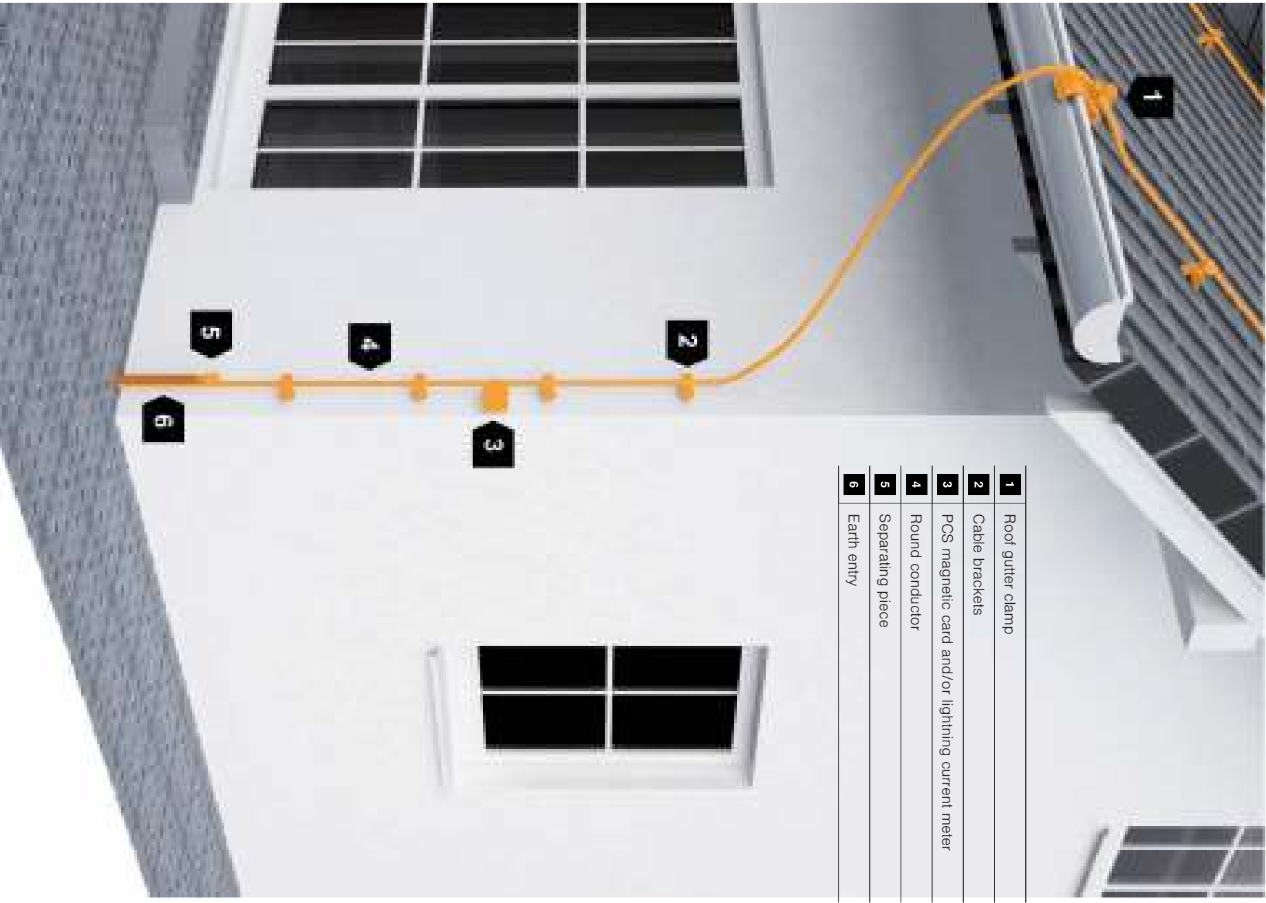
Installation principle, down-conductor unit
