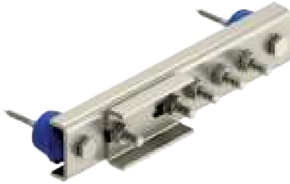
PAS equipotential busbar for potentially explosive areas
