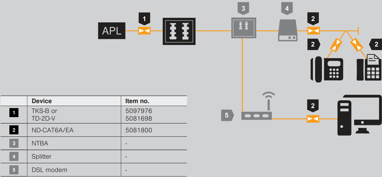
Protection of an ISDN + DSL connection with TeleDefender
