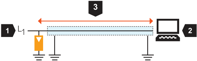
Maximum cable length between SPD and terminal
