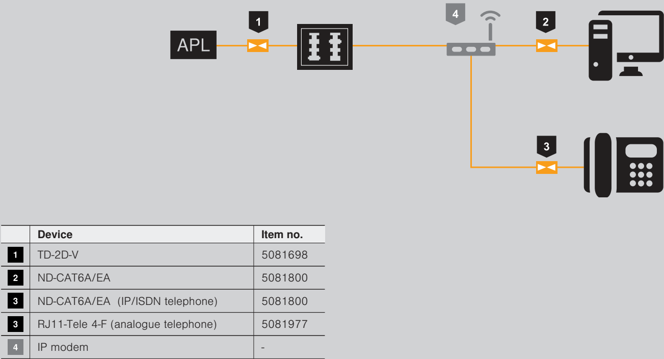
Protection of an IP connection
