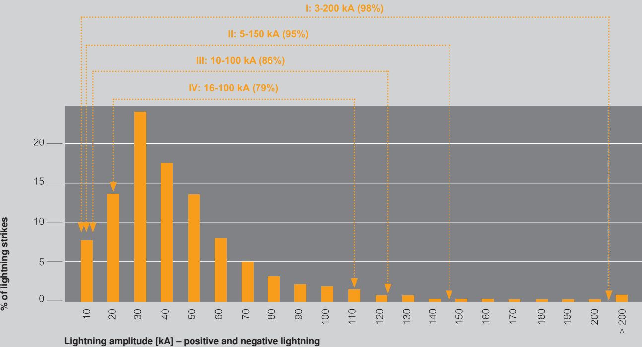
Lightning current parameters according to the risk level (LPL) in accordance with DIN VDE 0185-305-1
