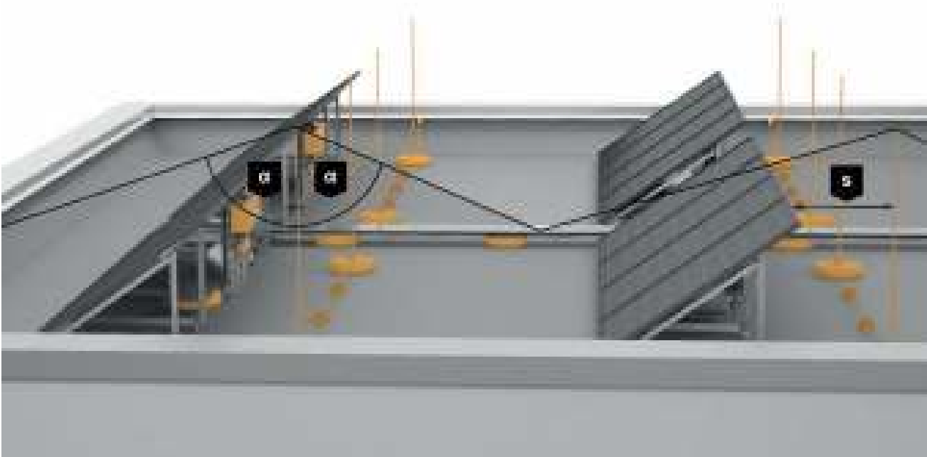
Protective angle and separation distance of air-termination rods in a photovoltaic system
