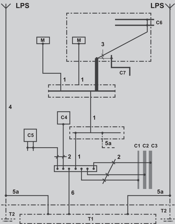
Equipotential bonding system in a building
