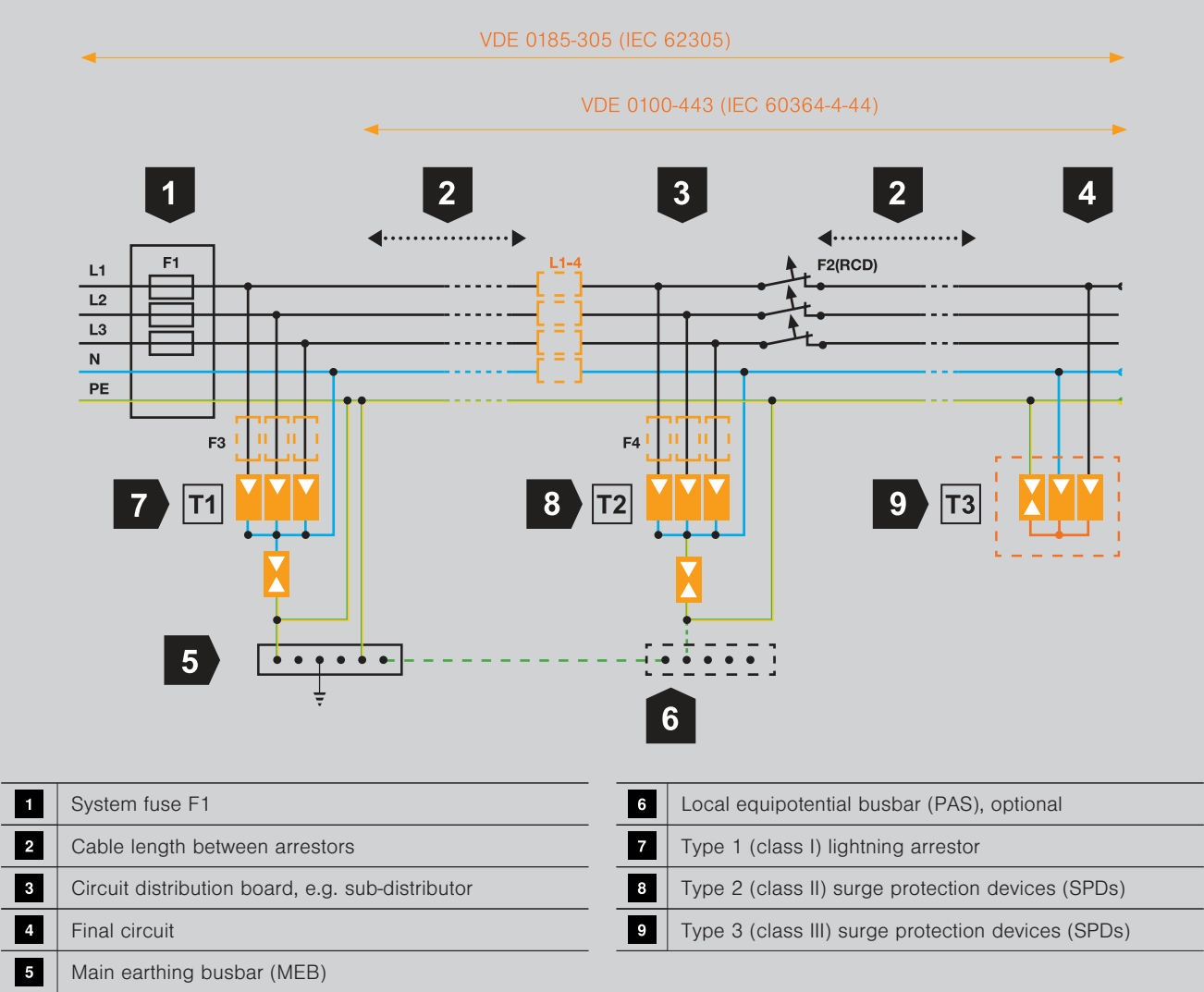
5-wire networks, TN-S and TT network system
