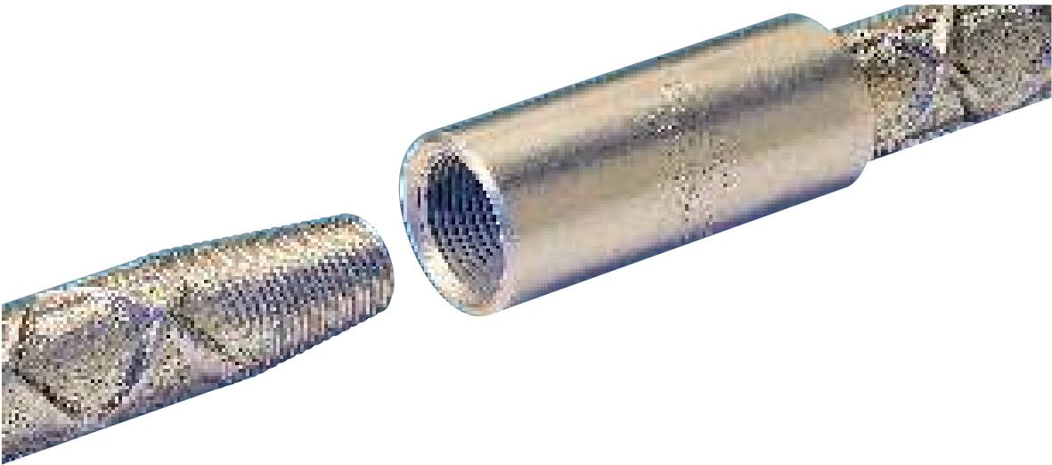
Figure 22. nVent LENTON termination of rebar provides good electrical connection.
