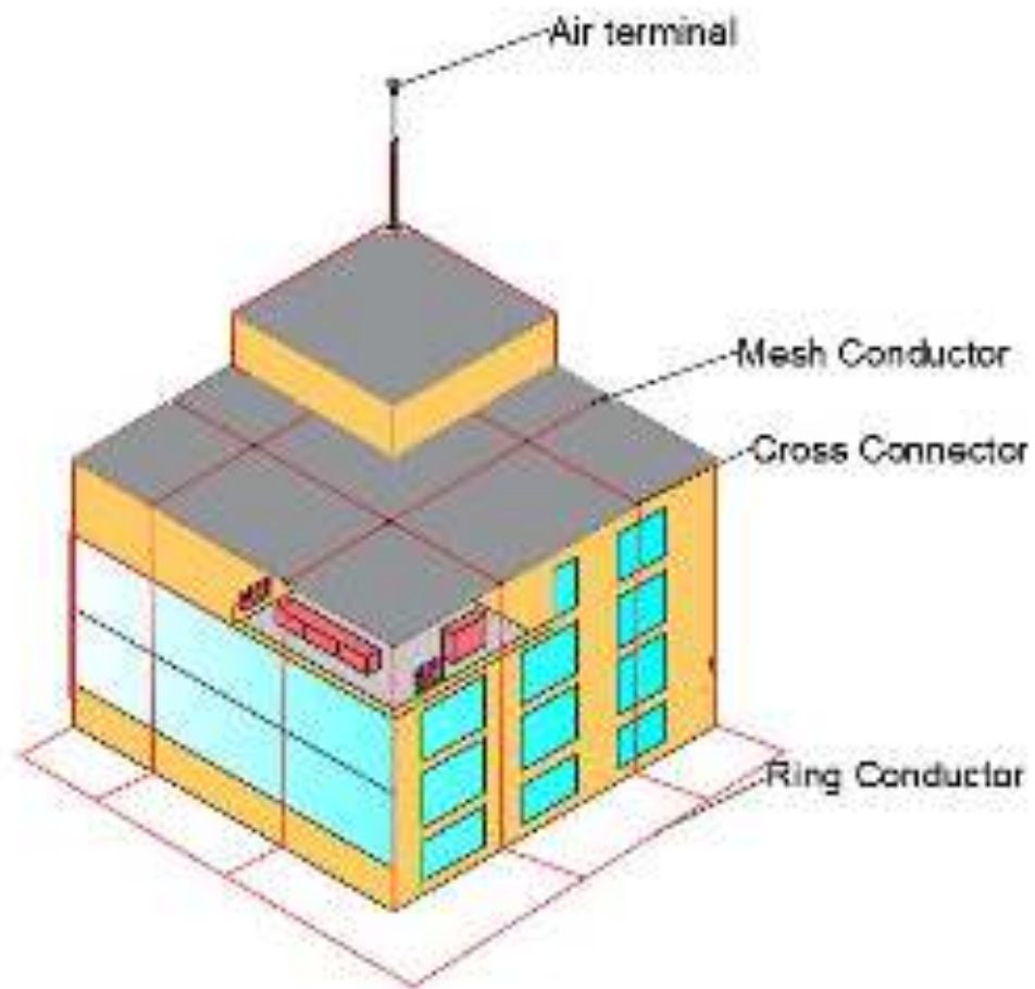
Figure 8. LPD Design
