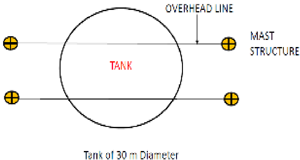
Figure 42. Storage tank protection - Overhead lines
