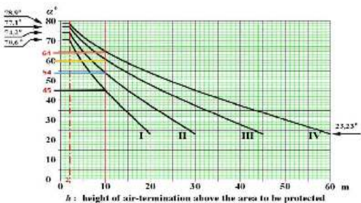
Figure 10. PAM Graph
