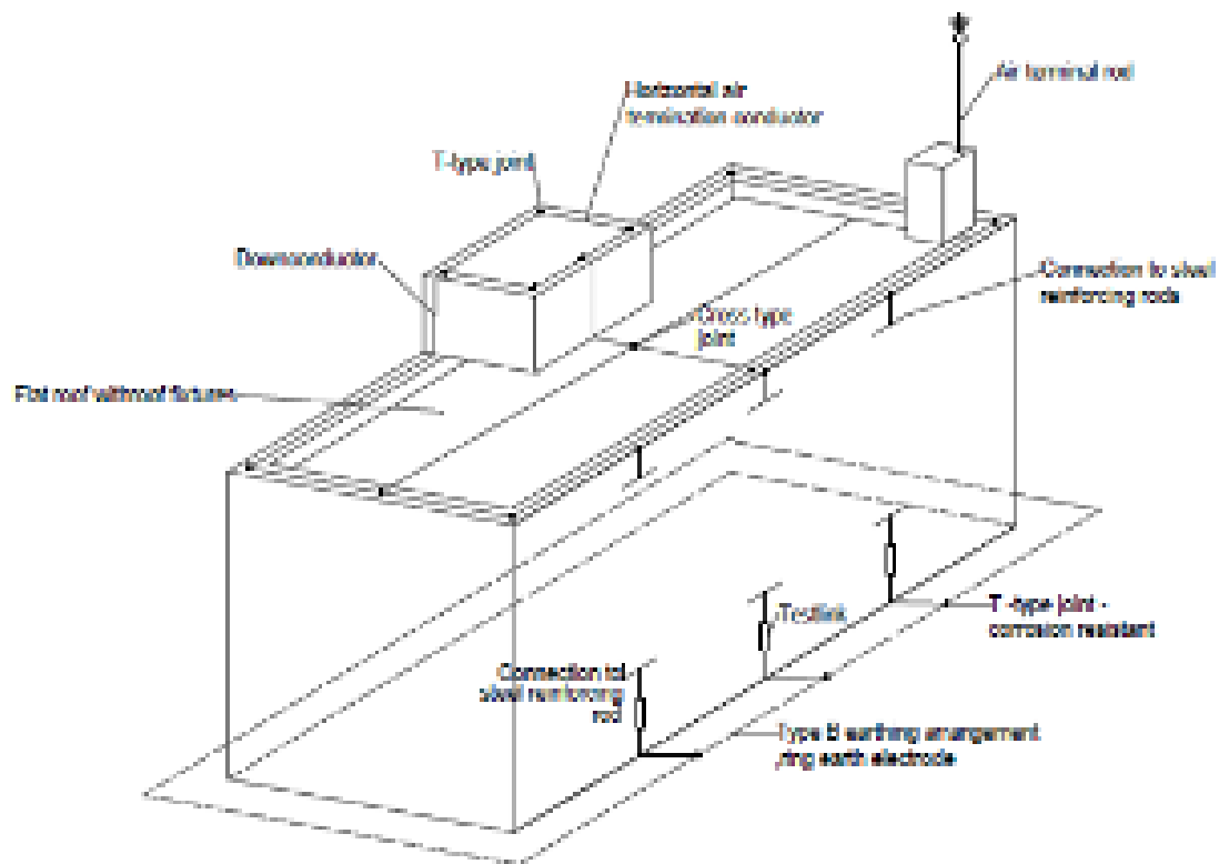
Figure 22. Natural components as LPS components
