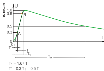
Figure 6: Full lightning impulse
