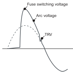
Voltage across the fuse
