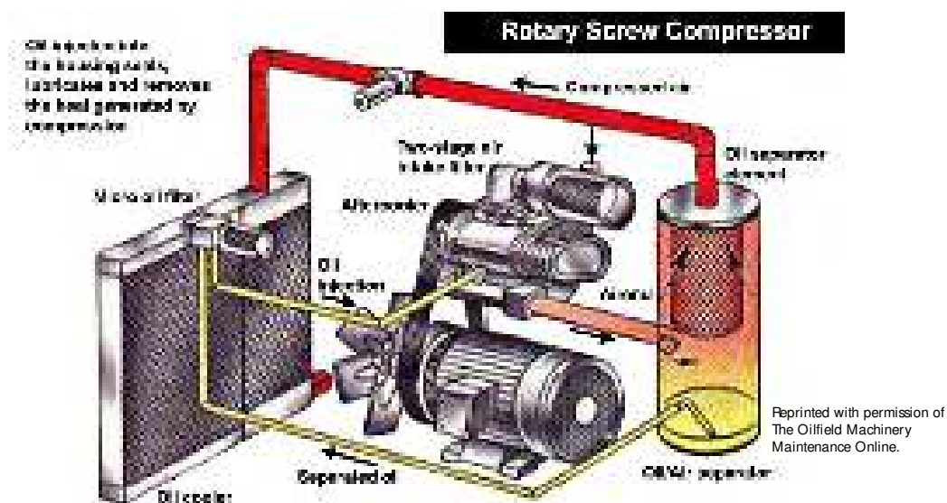
Figure 7.10.1. Rotary screw compressor.
