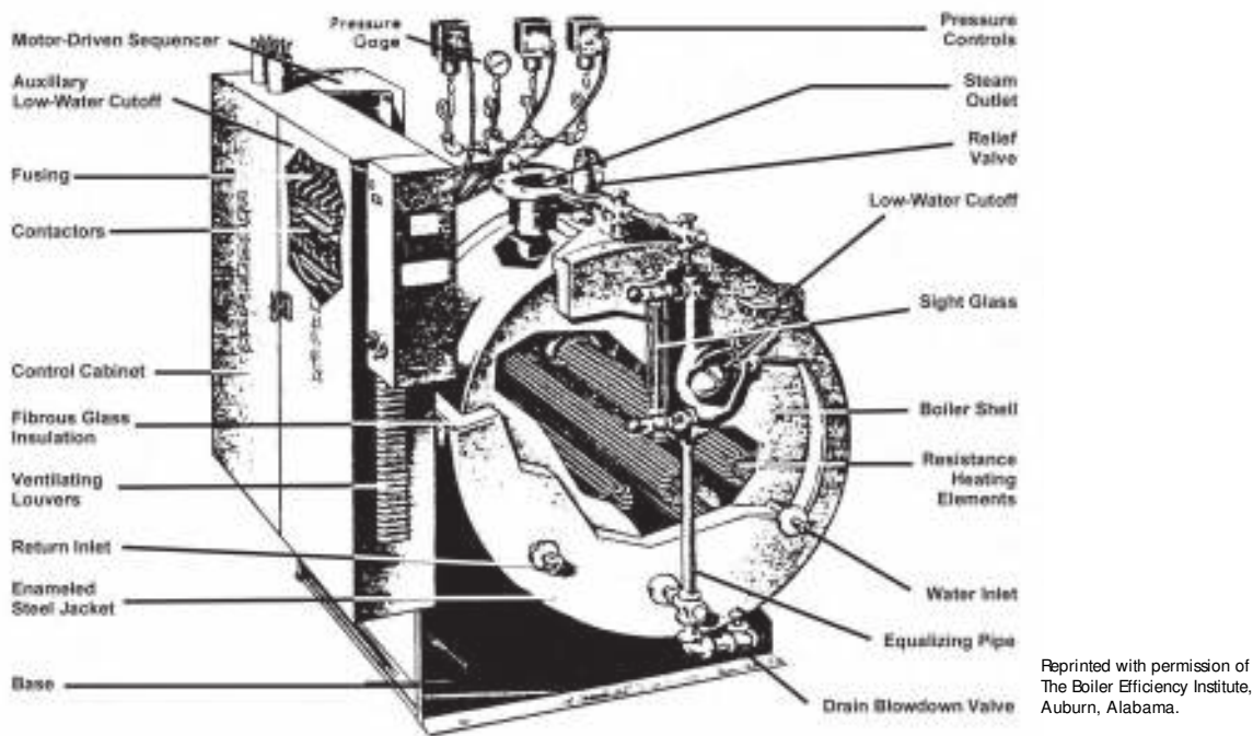
Figure 7.2.3. Electric boiler.
