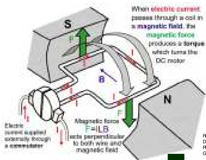
Figure 7.9.1. DC motor.
