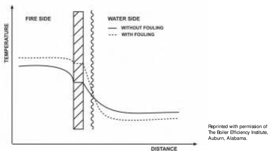
Figure 7.2.5. Effect of fouling on water side.
