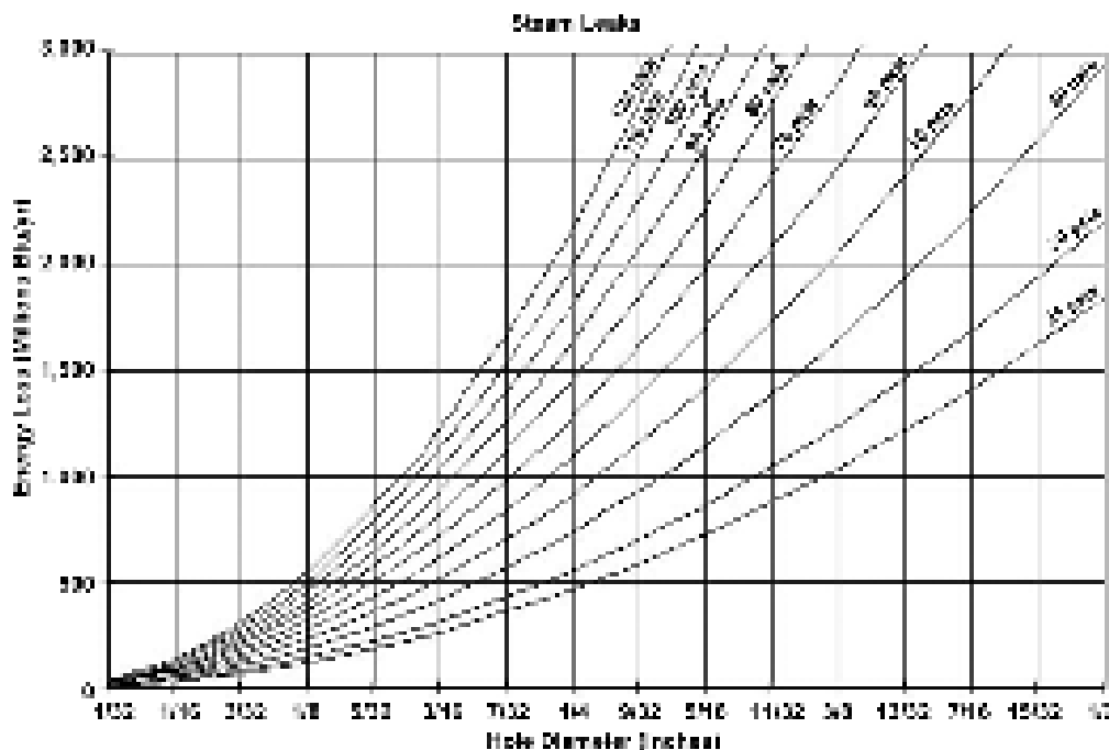
Figure 7.3.6. Energy loss from leaking steam traps.
