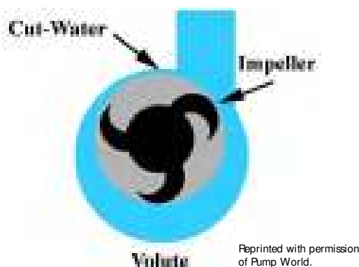
Figure 7.7.4. Centrifugal pump.
