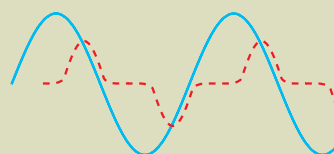
Example 4: Current and voltage out of phase and current non-sinusoidal PF \neq \cos \varphi and PF < 1
