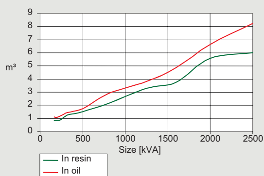
Transformer volume (L x H x D)
