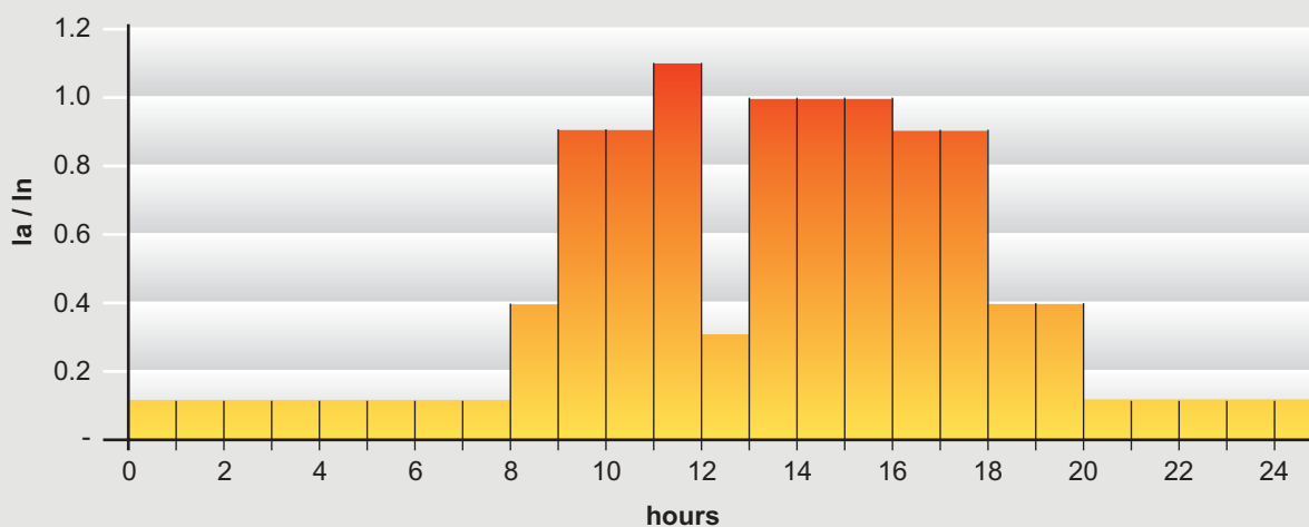
Load diagram over the working days of a small industrial factory | Ia: current effectively absorbed by the transformer In: transformer rated current | G (working days): 220
