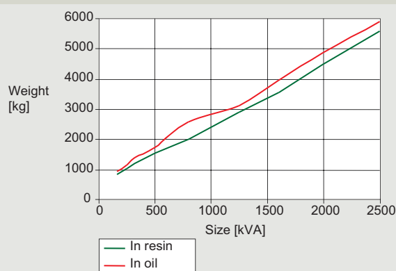
Transformer weight
