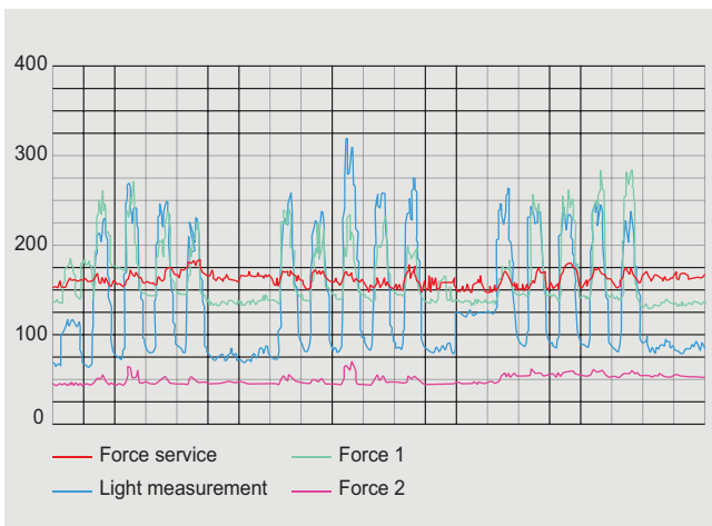
^ Example of measured load curves (kW av. / ¼h)
