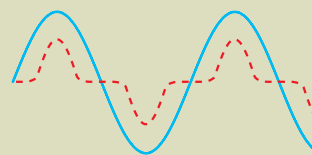
Example 3: Current and voltage in phase but current non-sinusoidal PF \neq \cos \varphi and PF < 1
