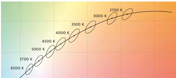
MacAdam ellipses along the Planck curve for white light
