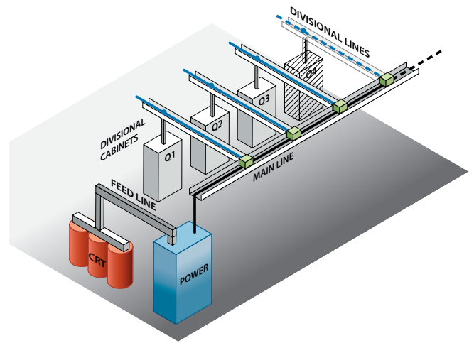
^ "Cable" solution: addition of a new distribution board to a junction box provided for this purpose
