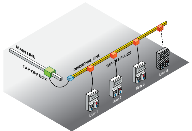
^ "Prefabricated busbar system" solution: addition of a new workstation by direct connection with the busbar system
