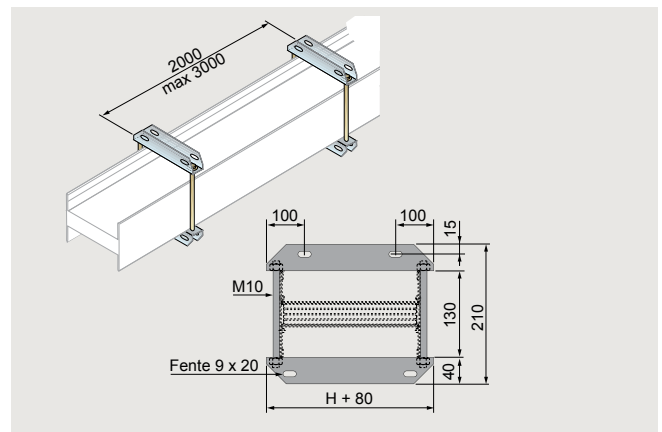
Fixing flange for flat sections
