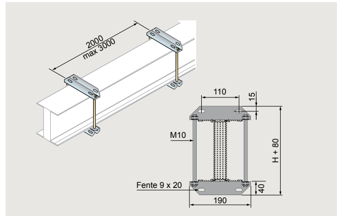
Fixing flange for angled sections
