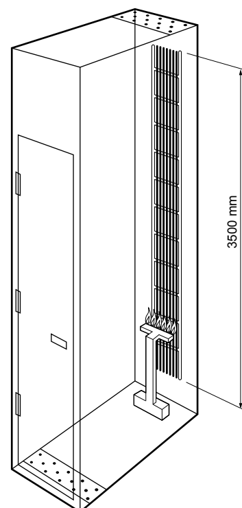
Fire resistance test device for cables in vertical layers
