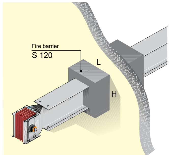
Class S12 fire barrier for Legrand SCP busbars
