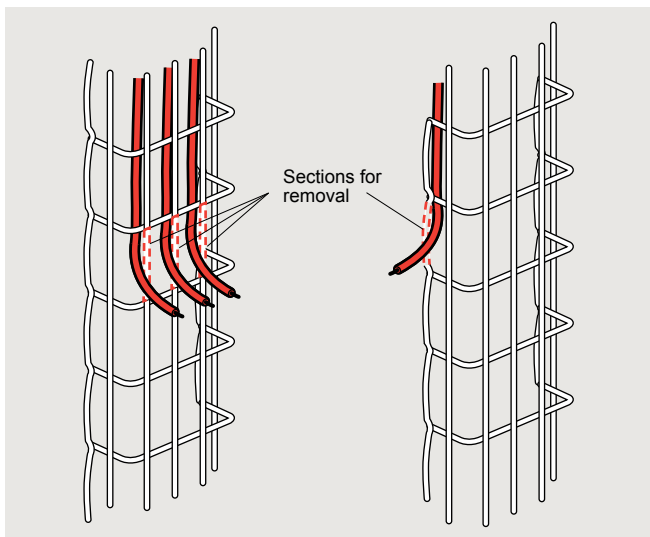
Cutting wire cable tray in order to prevent magnetic fields likely to cause heating.
