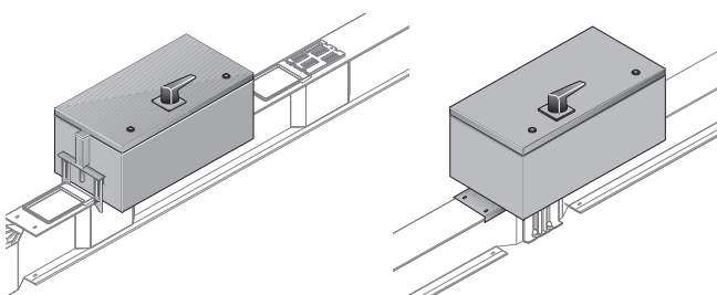
Plug-in box: mounting on a tap-off outlet
