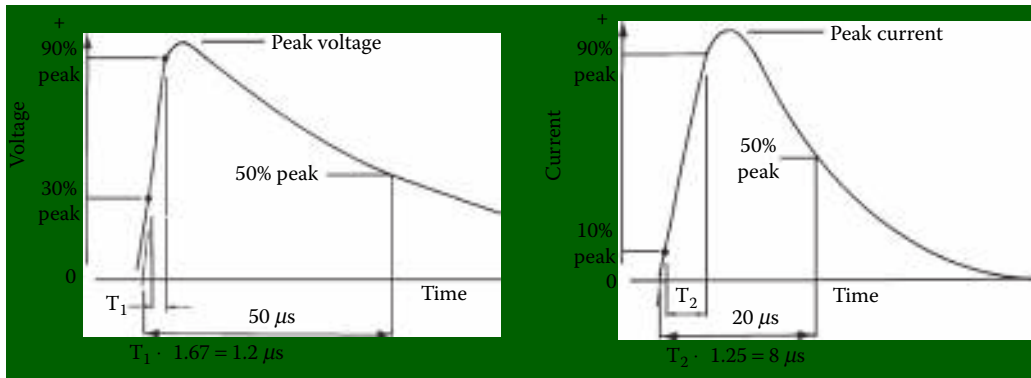
Figure 10.4 The unidirectional waveshape for outdoor-type transient overvoltage test analysis based on ANSI Standard C62.1: (a) open-circuit waveform, (b) discharge current waveform.
