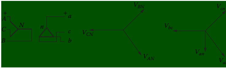
Figure 4.20 Y-Δ transformer with the primary side leading the secondary side by 30^\circ . (From [7]. Used with permission.)
