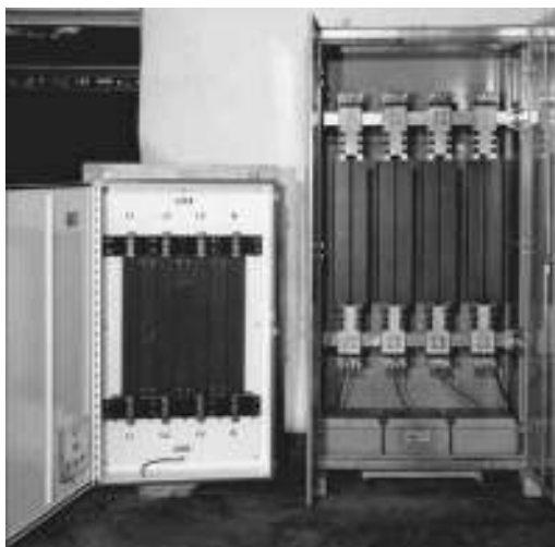
Figure 14.18 Interior view of a high-capacity hybrid power conditioner. (Courtesy of Control Concepts.)
