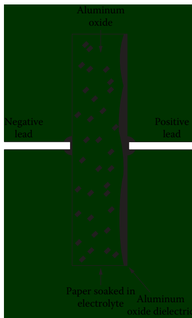
Figure 5.8 Failure mechanism of a leaky aluminum electrolytic capacitor. As the device ages, the aluminum oxide dissolves into the electrolyte, causing the capacitor to become leaky at high voltages
