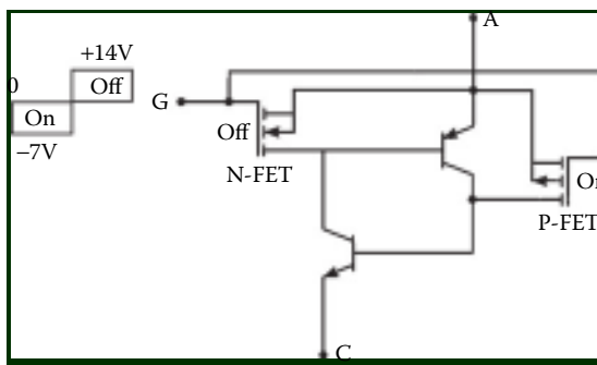
Figure 8.16 The equivalent circuit of the MCT device. (After [1] and [2].)
