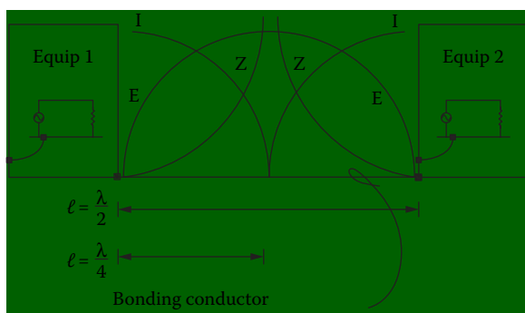
Figure 20.39 Standing waves on a bonding conductor resulting from the antenna effect. (From [2]. Used with permission.)
