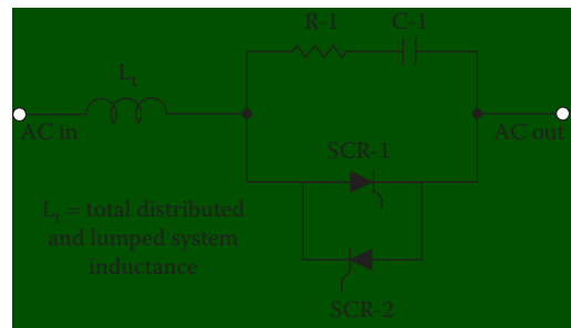
Figure 6.15 The basic RC snubber network commonly used to protect thyristors from fast-rise-time transients.
