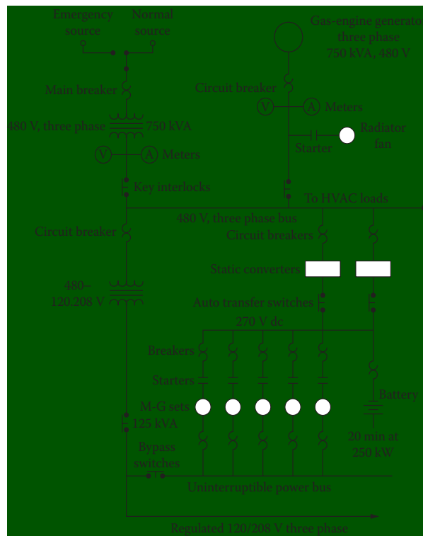
Figure 21.8 Simplified installation diagram of a high-reliability power system incorporating dual utility feeds, a standby gas-engine generator, and five battery-backed dc m-g sets. (After [1].)
