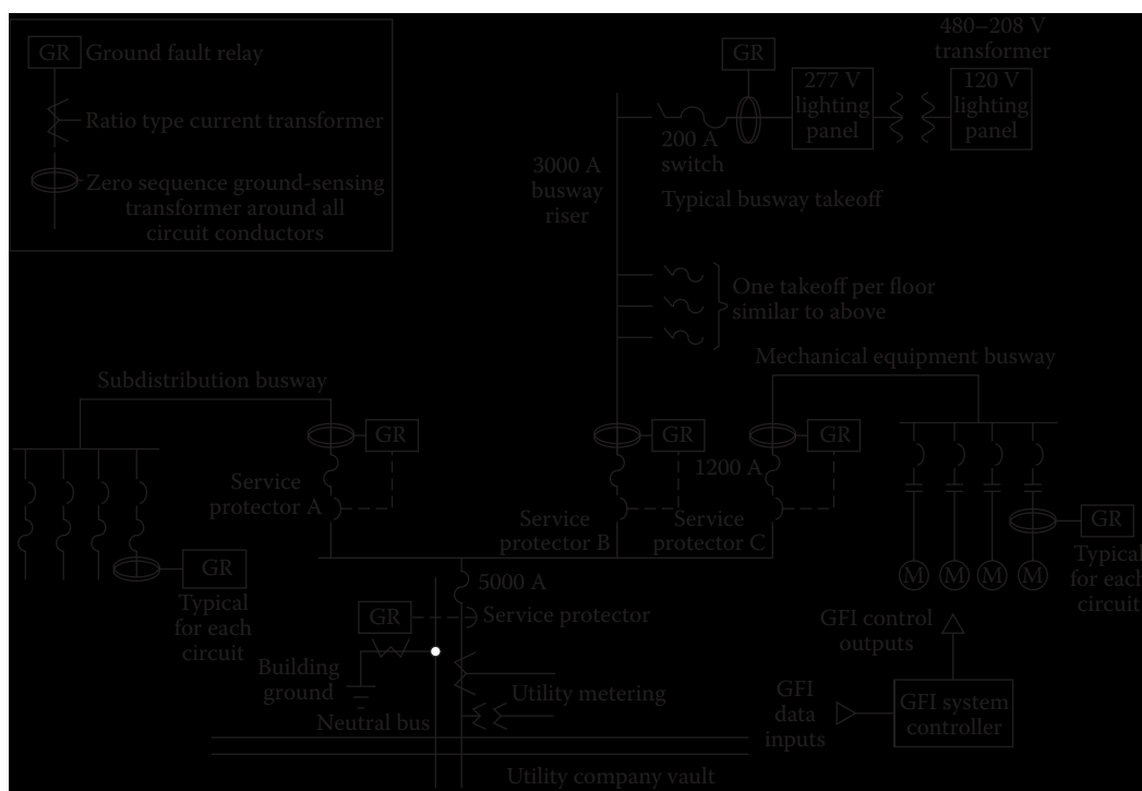
Figure 24.6 Ground-fault protection system for a large, multistory building.
