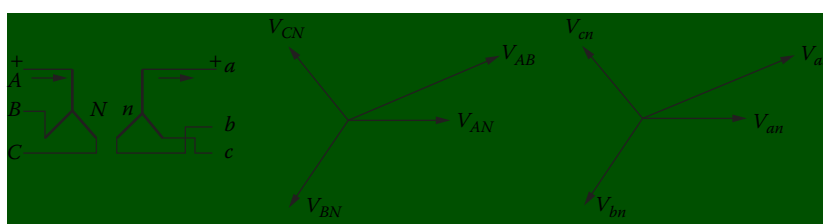
Figure 4.18 Y-Y transformer with 0^\circ phase shift between the primary and the secondary sides. (From [7]. Used with permission.)
