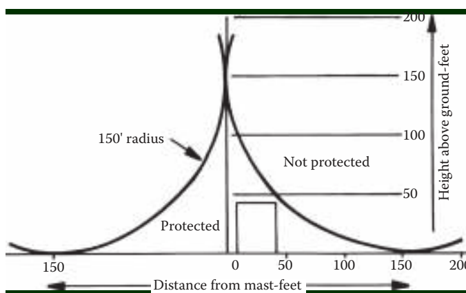
Figure 9.12 Protection zone for a tall tower under the “rolling sphere” theory.
