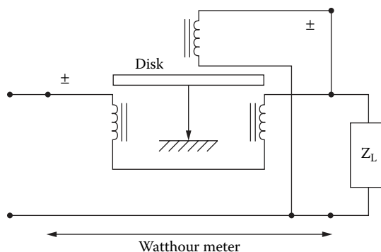
Figure 1.28 A watt-hour meter connected to a load. (From [10]. Used with permission.)
