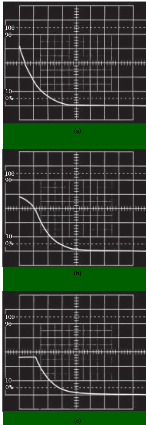
Figure 15.11 Voltage clamping performance comparison: (a) open-circuit transient pulse, vert. = 20 V/div, horiz. = 0.5 ms/div, V_{\text{peak}} = 90 V; (b) transient pulse with 27 V MOV applied, vert. = 10 V/div, horiz. = 0.5 ms/div, transient source impedance = 500\ \Omega , V_{\text{peak}} = 39.9 V; (c) transient pulse with 27 V zener applied, vert. = 10 V/div, horiz. = 0.5 ms/div, transient source impedance = 500\ \Omega , V_{\text{peak}} = 27 V. (Courtesy Motorola.)
