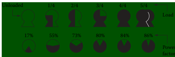
Figure 3.4 Changes in power factor for an induction motor as a function of motor loading.
