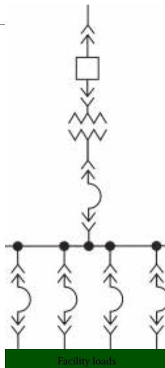
Figure 22.5 Secondary plant distribution using a simple radial configuration. (From [2]. Used with permission.)
