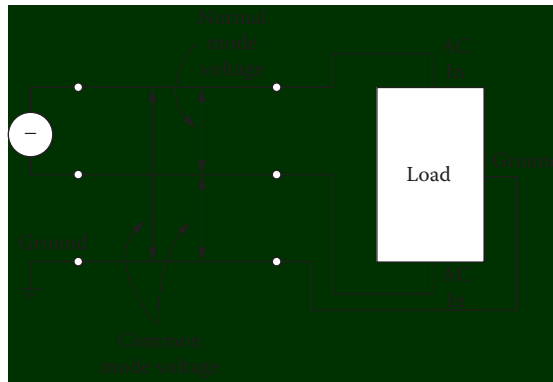
Figure 20.36 The principles of normal-mode and common-mode noise voltages as they apply to ac power circuits.
