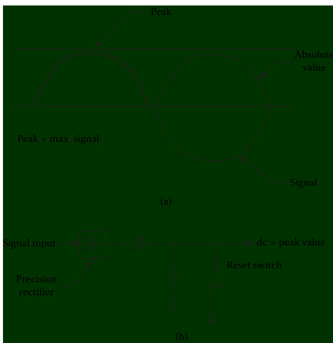
Figure 10.9 Peak voltage measurements: (a) illustration of peak detection, (b) peak measurement circuit.
