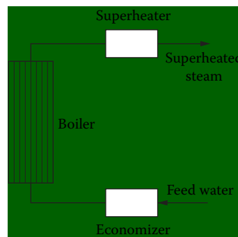
Figure 2.11 Block diagram of a once-through-type steam generator. (From [3]. Used with permission.)
