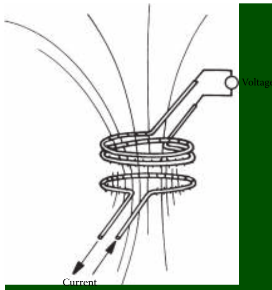
Figure 4.7 The basic principles of electromagnetic induction.
