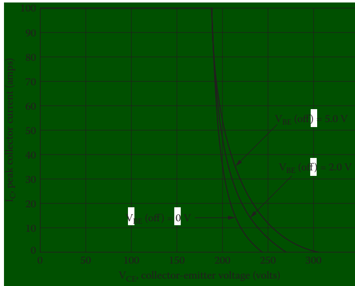
Figure 6.2 Reverse bias safe operating area curve for a bipolar transistor (MJH10610A). (Courtesy of Motorola.)
