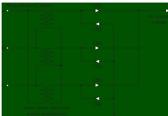
Figure 7.3 Three-phase, delta-connected high-voltage rectifier.
