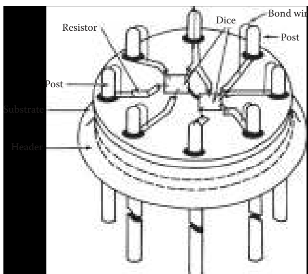
Figure 6.26 Basic construction of a multichip hybrid device. (After [1].)
