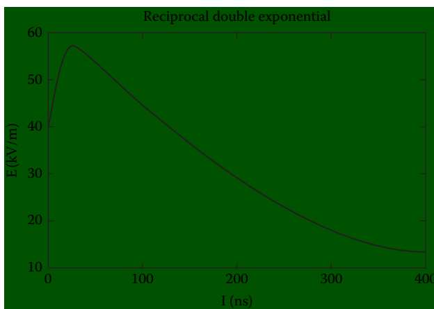
Figure 9.4 Discharge waveform for a typical lightning strike.
