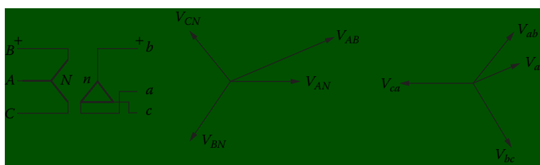
Figure 4.19 Y- \Delta transformer with the primary side lagging the secondary side by 30^\circ . (From [7]. Used with permission.)
