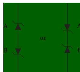
Figure 15.12 Zener arrangement for bidirectional clamping. (Courtesy of Motorola.)
