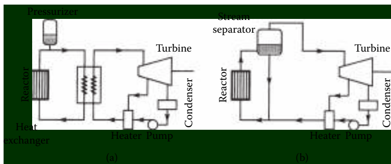
Figure 2.13 Types of nuclear power plants: (a) pressurized water reactor; (b) boiling-water reactor. (From [3]. Used with permission.)
