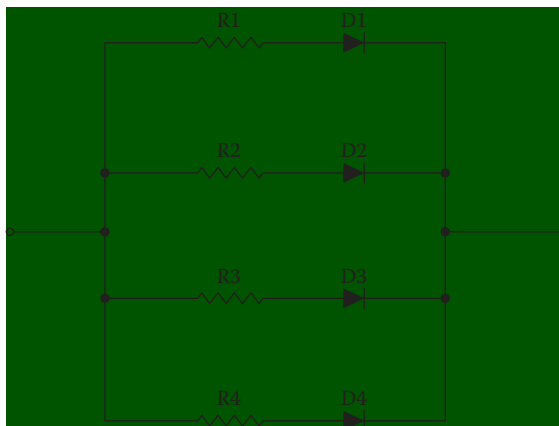
Figure 7.5 Using build-out resistances to force current sharing in a parallel rectifier assembly.
