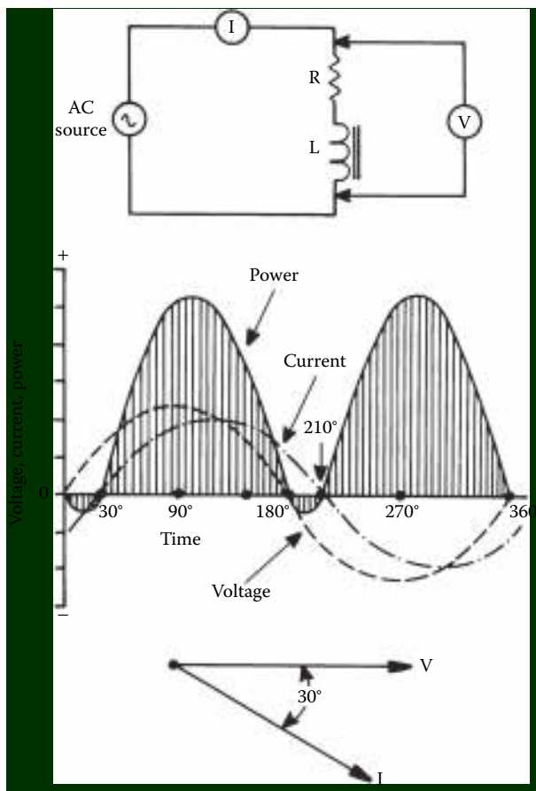
Figure 4.12 Resistive-inductive circuit: (a) circuit diagram; (b) representative waveforms; (c) vector representations.
