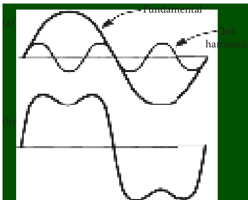
Figure 9.28 The addition of 60 Hz fundamental and 3^{\text{rd}} harmonic waveshapes: (a) individual waveforms, (b) resulting distorted waveshape. (From [5]. Used with permission.)
