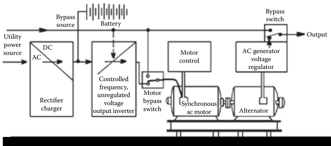
Figure 12.9 Uninterruptible m-g set using a synchronous ac motor. (After [1].)
