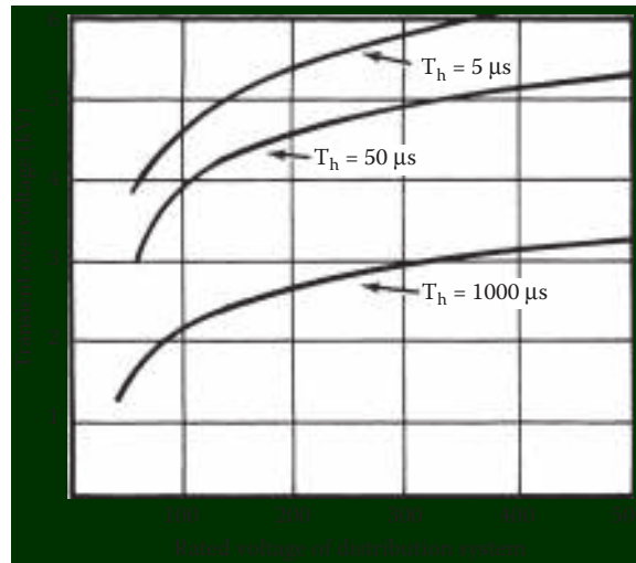
Figure 9.21 The relationship (computed and measured) between utility company system voltage and switching transient peaks. Switching transients are plotted as a function of nominal operating voltages for three values of the transient tail time to half-potential. It can be seen that there is no direct linear increase in transient amplitude as the system voltage is increased.
