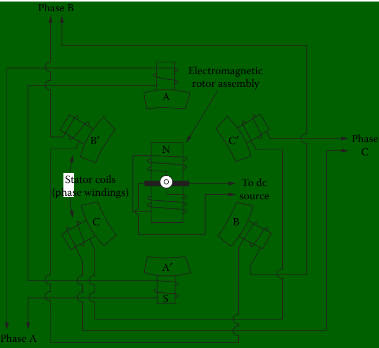
Figure 2.1 Simplified diagram of a three-phase ac generator.
