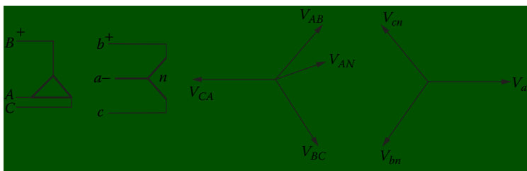
Figure 4.21 Δ-Y transformer with the primary side leading the secondary side by 30^\circ . (From [7]. Used with permission.)
