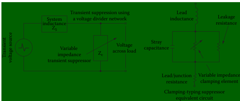
Figure 15.5 The mechanics of transient suppression using a voltage-clamping device.
