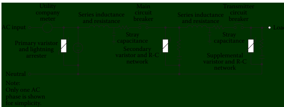
Figure 16.6 The use of ac system series inductance and resistance to aid transient suppressors in controlling line disturbances. This technique is known as staging .
