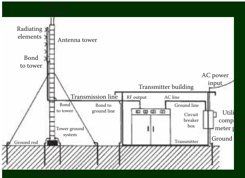
Figure 20.11 A common, but not ideal, grounding arrangement for a transmission facility using a grounded tower. A better configuration involves the use of a bulkhead panel through which all cables pass into and out of the equipment building.
