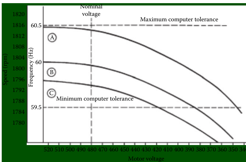
Figure 12.6 Generator output frequency vs. motor input voltage for an induction-motor-based m-g set.
