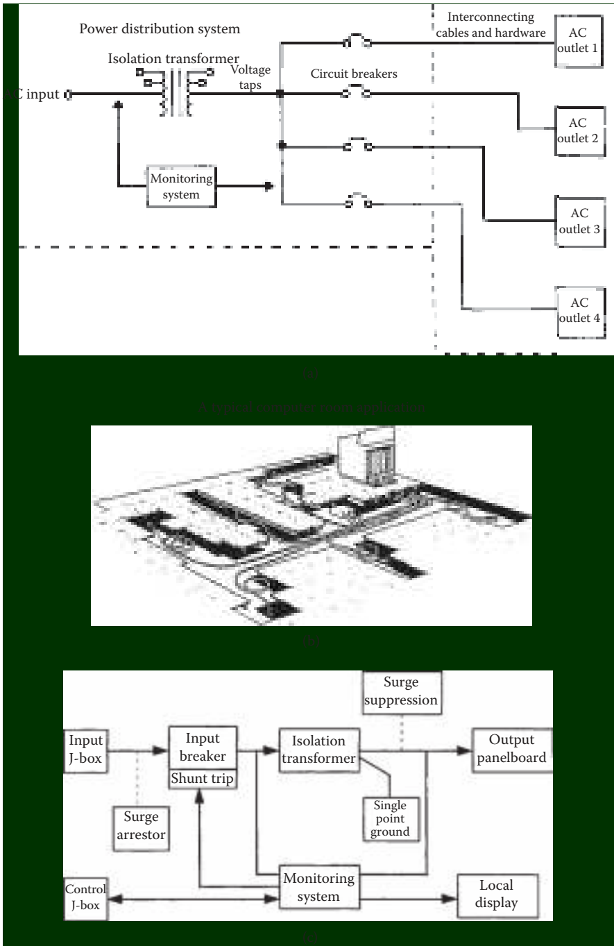
Figure 20.26 The basic concept of a computer-room modular power center: (a) basic line drawing of system, (b) typical physical implementation, (c) functional block diagram. Both single- and multiphase configurations are available. When ordering an MPC, the customer can specify cable lengths and terminations, making installation quick and easy. (After [7].)
