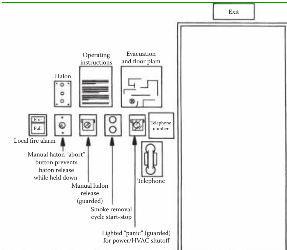
Figure 24.1 A well-organized life safety control station. (After [1].)
