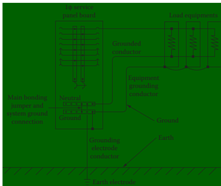
Figure 18.1 Equipment grounding and system grounding. (From [5]. Used with permission.)
