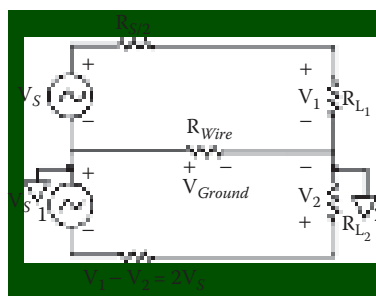
Figure 20.35 A balanced source configuration where the inherent amplitude error of the system shown in Figure 20.34 is eliminated.
