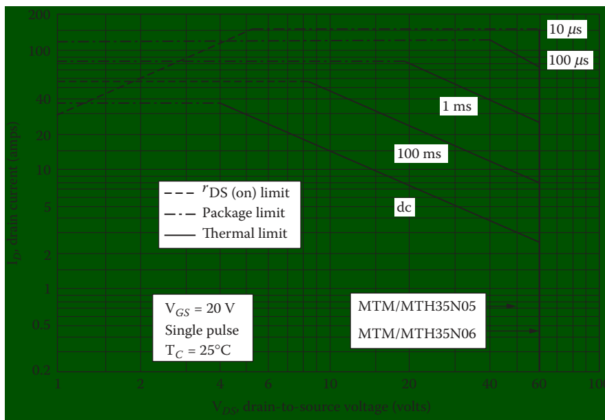
Figure 6.5 Safe operating area curve for a power FET device. (Courtesy of Motorola.)
