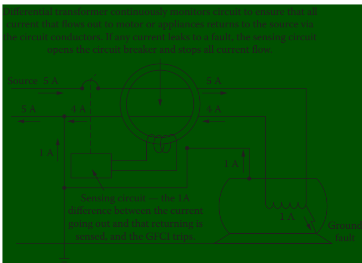
Figure 24.4 Basic design of a ground-fault current interrupter (GFCI).
