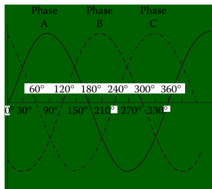
Figure 2.3 Output waveform of a three-phase generator.
