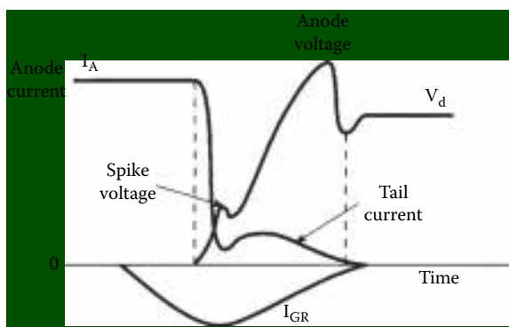
Figure 8.13 Turn-off characteristics of a GTO. (After [1] and [2].)
