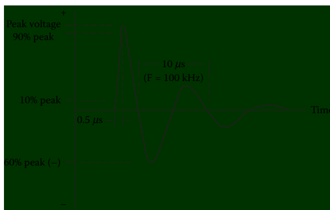
Figure 10.3 The suggested ANSI/IEEE indoor-type transient overvoltage test waveform (0.5 \mu s to 100 kHz ring wave, open-circuit voltage).
