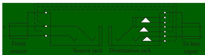
Figure 20.40 Patch-panel wiring for seven-terminal normalling jack fields. Use patch cords that connect ground (sleeve) at both ends.
