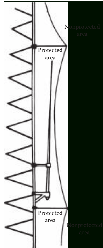
Figure 9.13 Protection zone for a side-mounted antenna under the “rolling sphere” theory.
