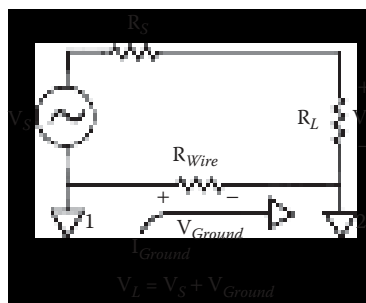
Figure 20.33 An unbalanced system in which each piece of equipment has one of its connections tied to ground.
