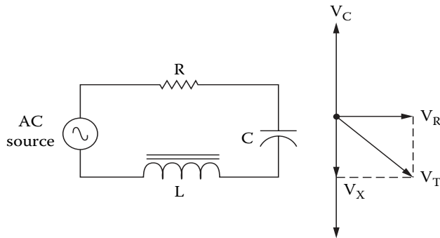
Figure 1.1 Voltage vectors in a series RLC circuit.
