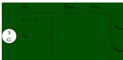
Figure 2.7 The basic power circuit of a generating system; V_s = E_g - I_a X_g . (From [1]. Used with permission.)
