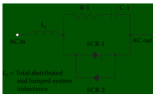
Figure 8.6 Protective RC snubber for a thyristor-based power controller.
