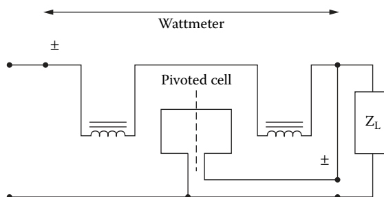
Figure 1.27 A wattmeter connected to a load. (From [10]. Used with permission.)
