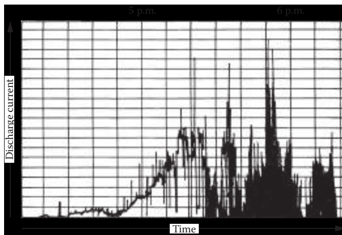
Figure 9.10 Measured discharge current of a lightning dissipation array.
