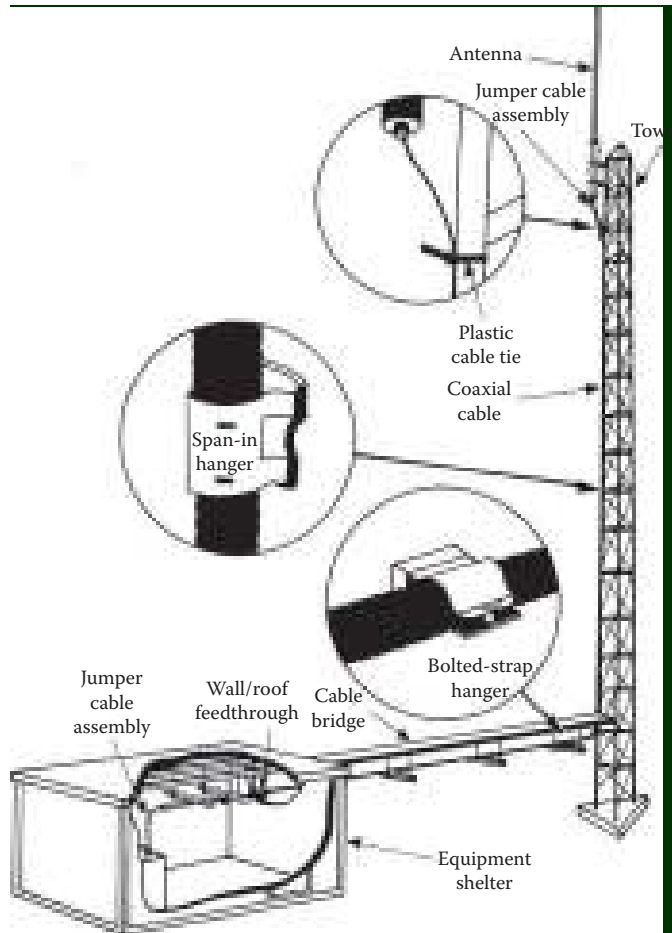
Figure 19.7 Transmission-line mounting and grounding procedures for a communications site.
