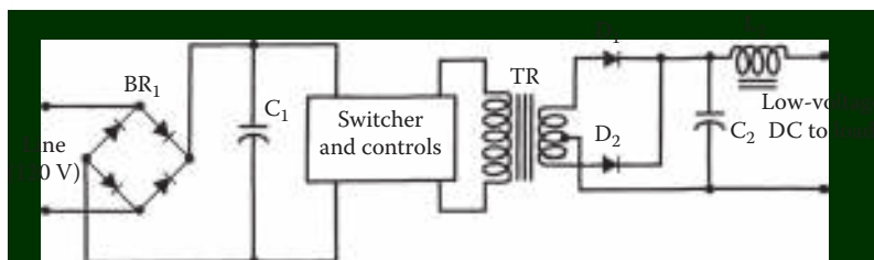
Figure 9.32 Simplified block diagram of a switching-mode power supply. (From [5]. Used with permission.)
