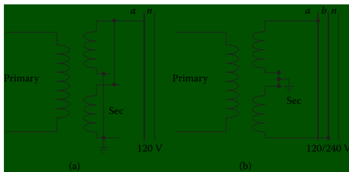
Figure 4.17 Connections for a single-phase distribution transformer: (a) parallel connection, (b) series connection. (From [7]. Used with permission.)
