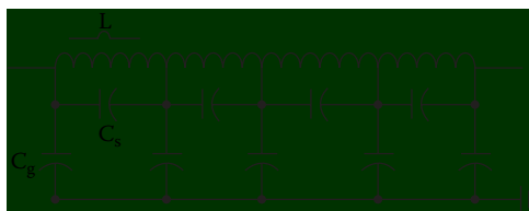
Figure 4.27 Capacitive distribution along the windings of a power transformer.
