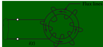
Figure 4.3 A toroid inductor. (After [3]. From [1]. Used with permission.)
