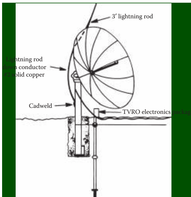
Figure 19.9 Addition of a lightning rod to a satellite antenna ground system. (After [9].)
