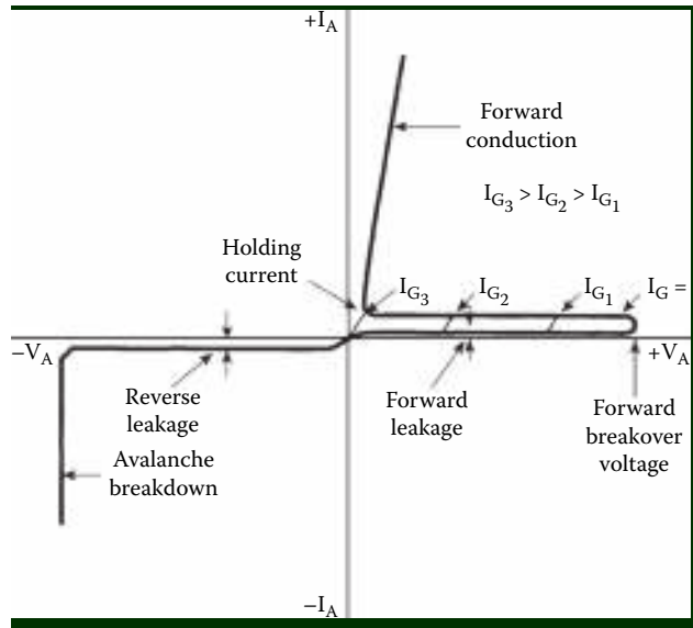
Figure 8.1 Voltampere characteristics of a thyristor. (After [1] and [2].)
