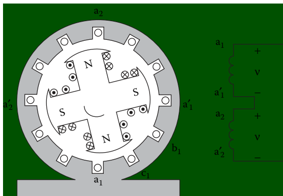
Figure 2.5 A four-pole synchronous machine: (a) cross section of the machine; (b) schematic diagram for the phase a windings. (From [1]. Used with permission.)
