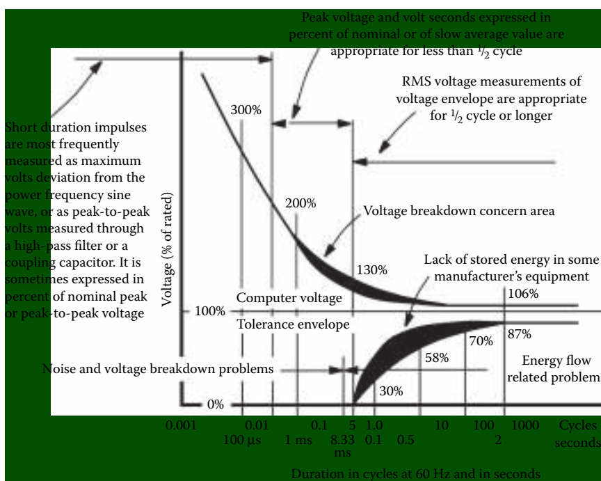
Figure 11.4 The CBEMA curve from FIPS Pub. 94. (From [2]. Used with permission.)
