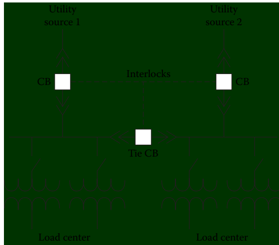
Figure 21.4 A dual-utility-feeder system with interlocked circuit breakers.
