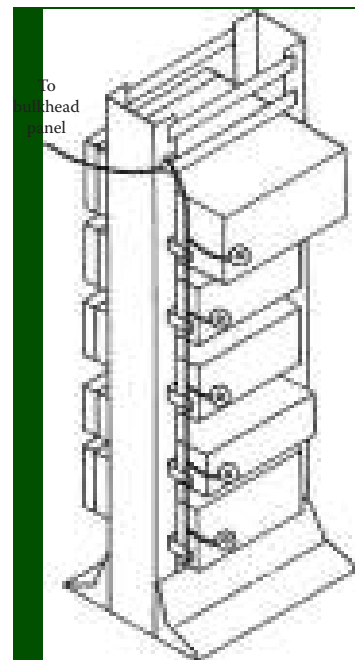
Figure 20.31 Ground bus for an open-frame equipment rack.
