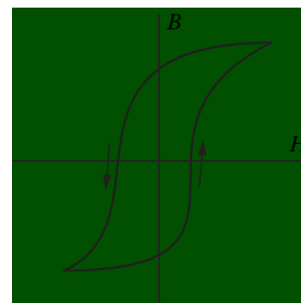
Figure 4.13 A typical magnetization curve. (From [6]. Used with permission.)
