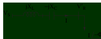
Figure 3.11 A distribution line with series-capacitor-compensation applied. (From [1]. Used with permission.)
