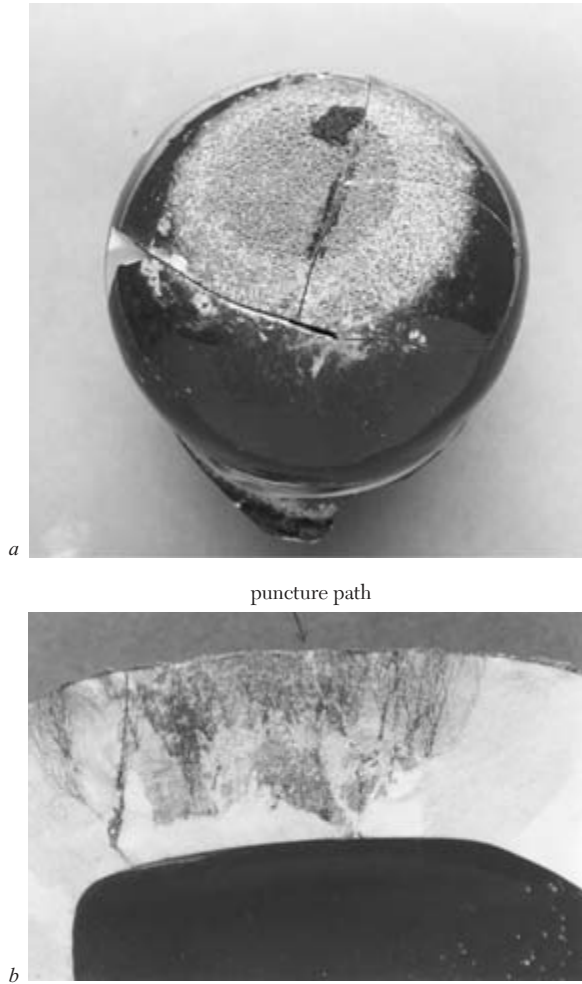
Figure 6.6 Cracks and puncture path in the head of the porcelain shell
