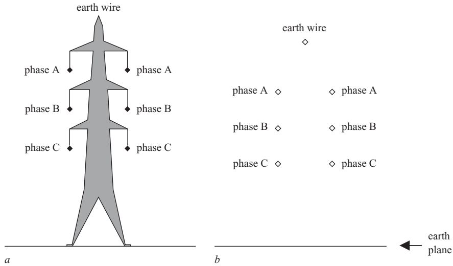
Figure 11.9 High voltage overhead cable arrangement a outline of pylon b position midway between pylons
