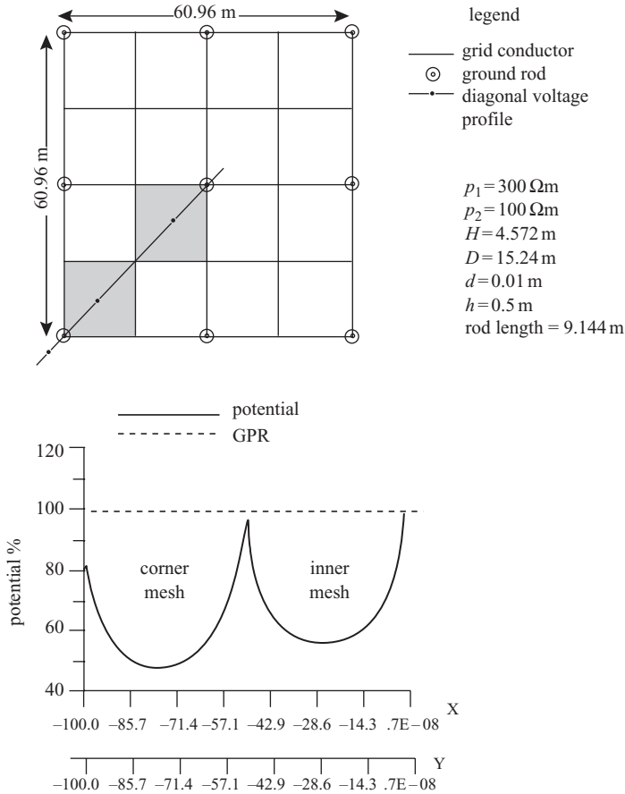
Figure 8.18 Diagonal voltage profile for a 16-mesh square grid with nine rods in a two layer soil (from IEEE Std.81 1983, IEEE Copyright 1983 and IEEE Std.80 2000. All rights reserved [30])
