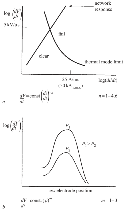
Figure 9.3 Typical circuit breaker characteristics (after Jones [4, chap. 7])
