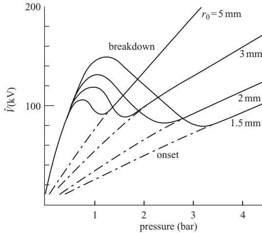
Figure 2.4 AC corona onset and breakdown characteristics for a 40 mm rod-plane gap in \text{SF}_6 [4]
