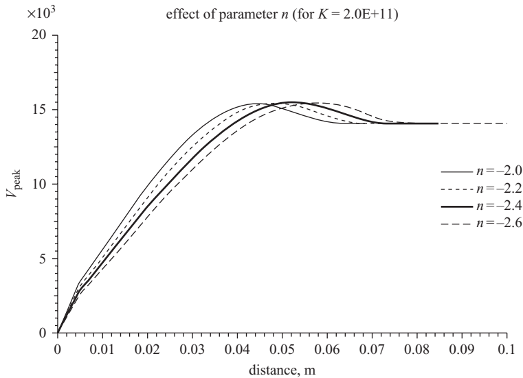
Figure 11.22 Variation of voltage with n (based on the paper 'Finite element modelling of non-linear stress grading materials for machine end windings', by A.E. Baker, A.M. Gully and J.C.G. Wheeler; as published on pp. 265–268 of the IEE Conference Publication (no. 487) on the International Conference of Power Electronics, Machines and Drives in Bath, 16–18th April 2002)
