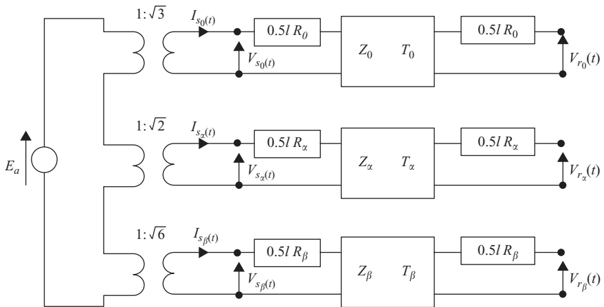
Figure 7.6 Interconnection of 0, \alpha , \beta network to simulate single pole closing
