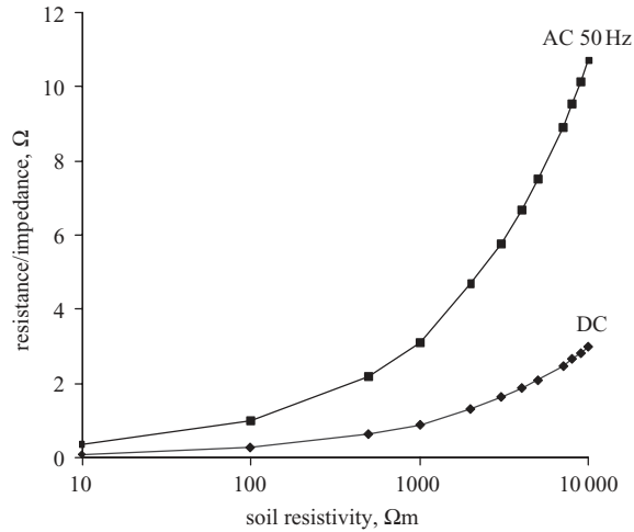
Figure 8.9 Comparison between DC chain resistance and AC (50 Hz) chain impedance for a 400 kV tower line (reproduced from [67])
