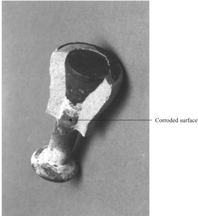
Figure 6.4 Corroded pin (with some mortar removed)
