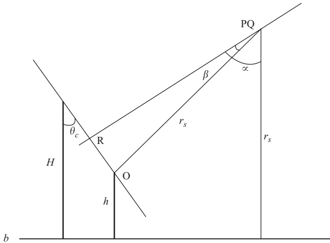
Figure 3.9 Electrogeometric modelling for overhead line shielding
