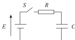
Figure 13.4 Resistive charging circuit for capacitor
