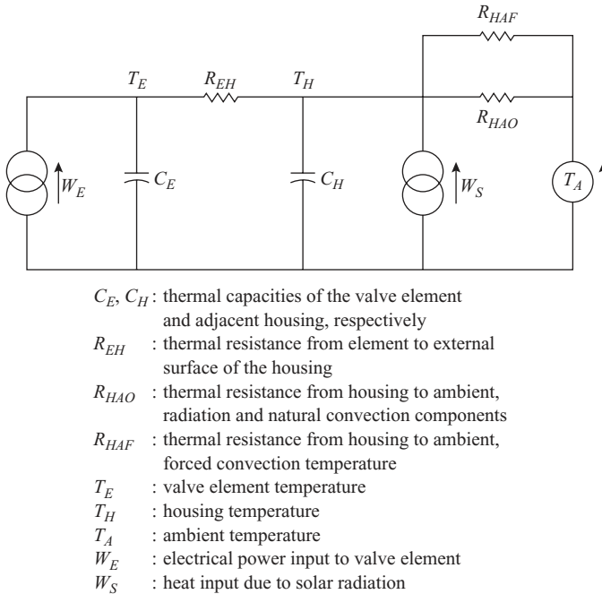
Figure 5.5 Thermal model of a ZnO arrester. (Courtesy of LAT, M.V.: 'Thermal properties of metal oxide surge arresters', IEEE Trans. PAS, 1983, PAS-102, (7), pp. 2194–2202, ©2003 IEEE)
