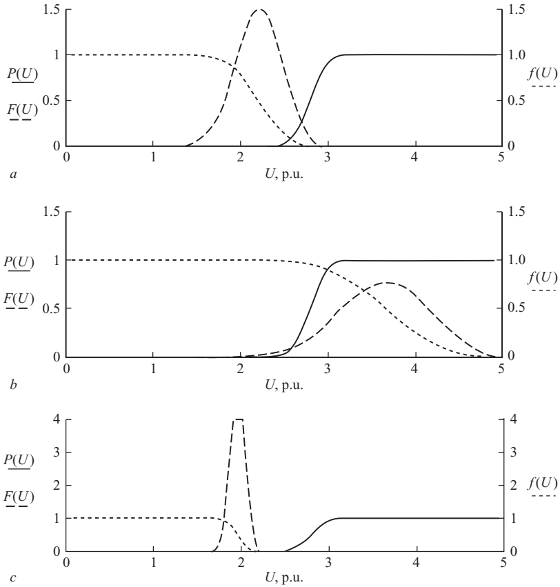
Figure 7.15 Weibull representation of f(U) , F(U) and P(U)
