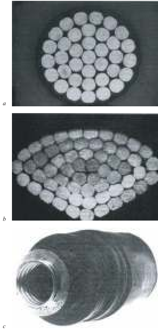
Figure 10.2 Methods of laying conductors
