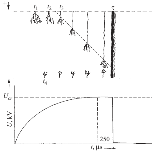
Figure 1.6 Simplified picture of streamer and leader development to breakdown in a rod-rod gap under an impulse voltage rising to peak in 250 \mu s
