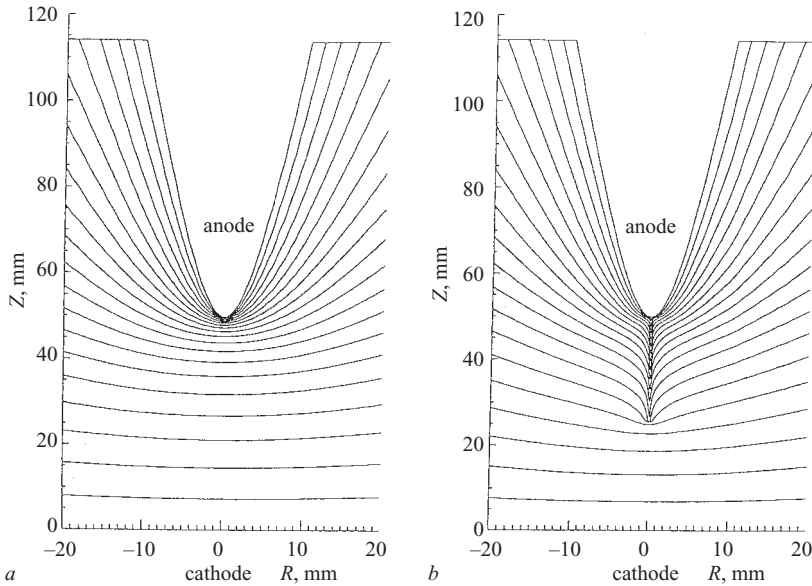
Figure 1.4 Potential distributions a before, b during development of a positive streamer from an electrode. Anode at 20 kV, equipotential intervals 1 kV. Streamer has progressed \sim 23 mm in 54 ns (after Morrow and Lowke [14])
