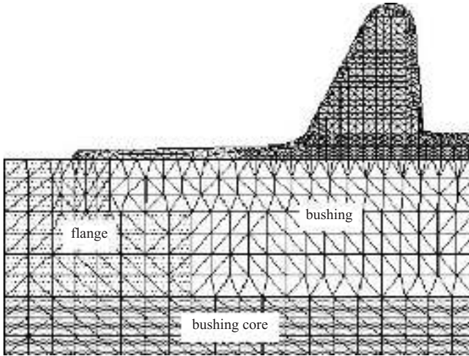
Figure 11.3 Example of a finite-element mesh
