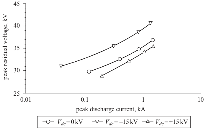
Figure 5.23 Typical effect of DC prestress (trapped charge) on the protective characteristic of a 15 kV-rated ZnO surge arrester
