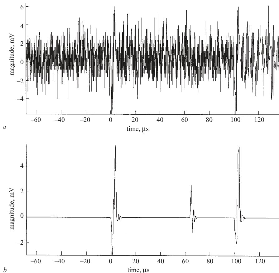
Figure 4.5 PD measurement in presence of noise
