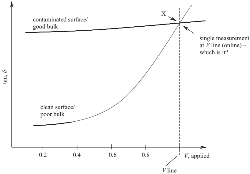
Figure 4.7 Tan \delta measured only at V line – problem of online measurement
