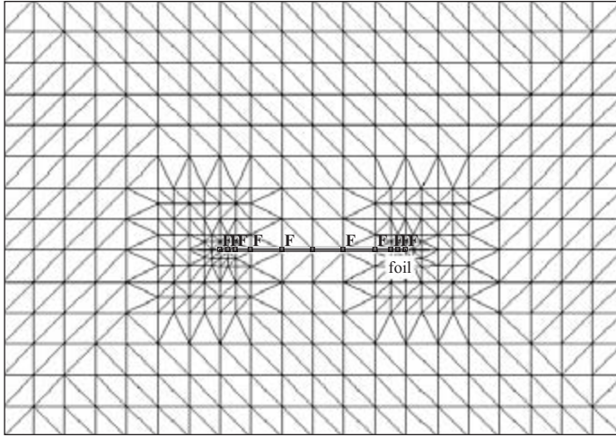
Figure 11.8 Foil representation
