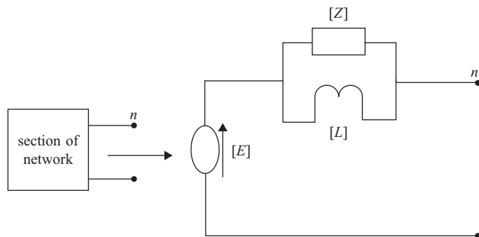
Figure 7.11 Equivalent circuit representing section of network
