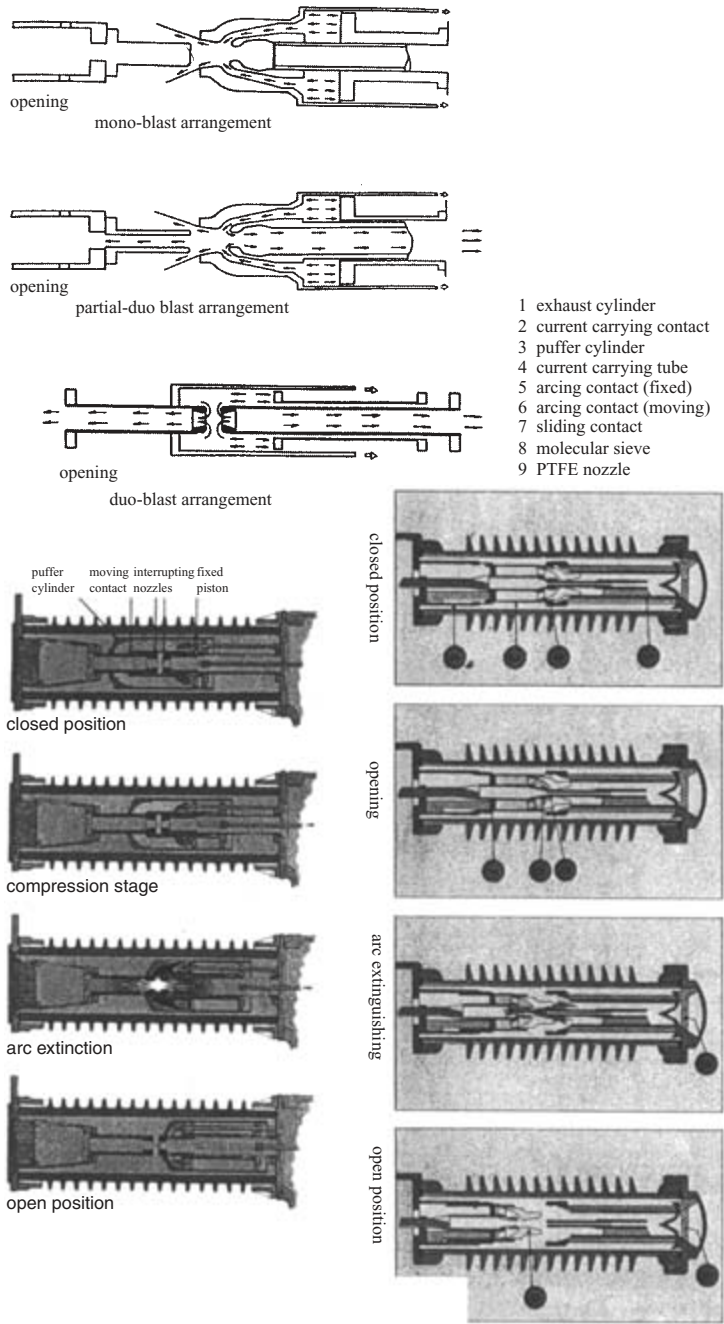
Figure 9.19 SF 6 puffer-type interrupters (after Ali [4, chap. 8]) a principles
