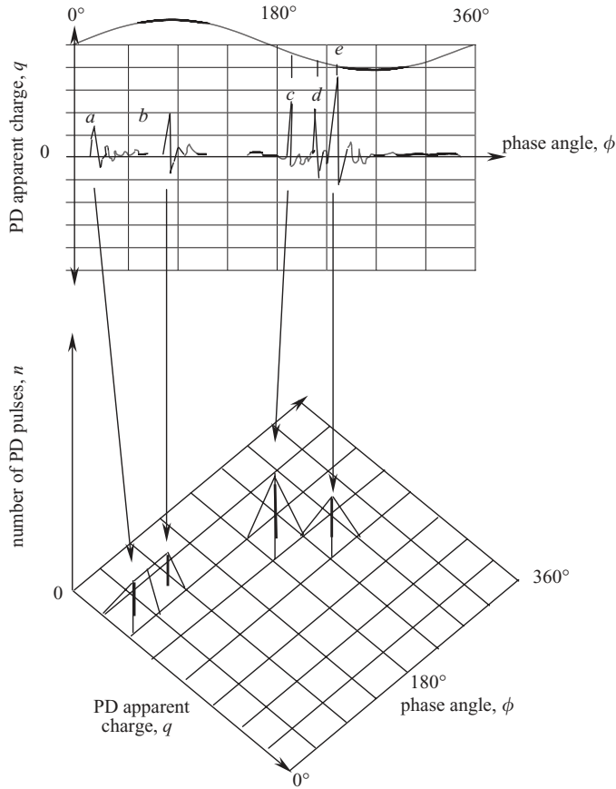
Figure 4.3 Build-up of \phi - q - n distribution
