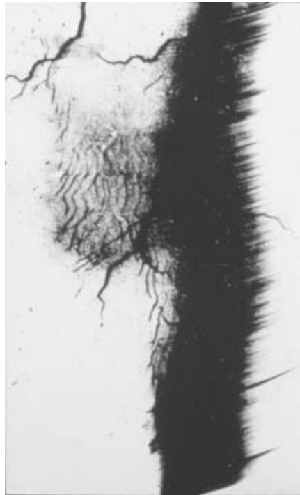
Figure 3.2 Spatial development of the negative downward flash (courtesy of 'Progressive lighting: A comparison of photographic and electrical studies of the discharge', by B.F.J. Schonland and H. Collens, Proceedings of the Royal Society. Series A , vol. 143, 1934, pp. 654–674)
