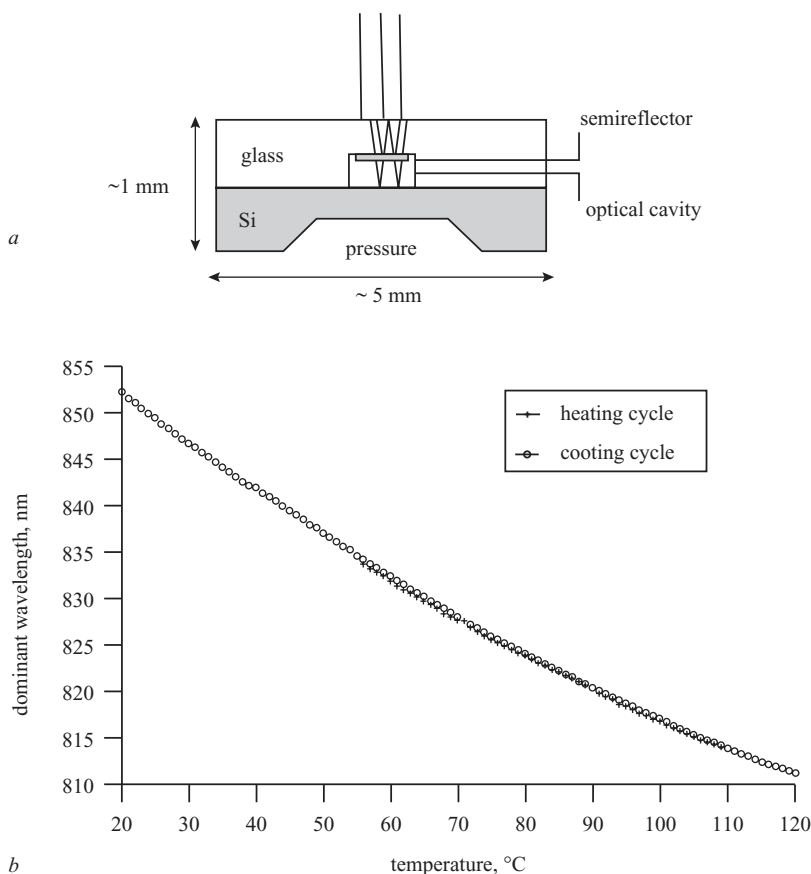
Figure 12.20 Chromatic Fabry-Perot temperature pressure transducer [29]
