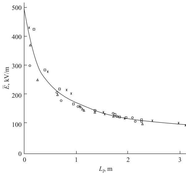
Figure 1.9 Average electric field along the leader channel as a function of its length [38]
