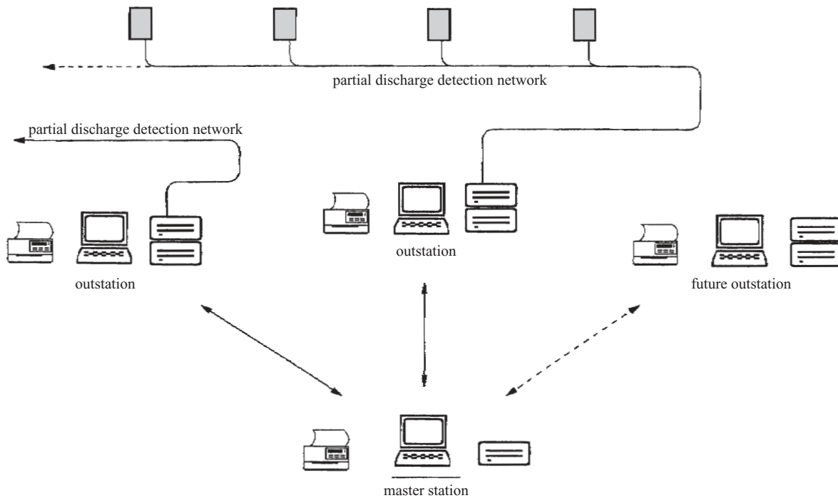
Figure 9.21 GIS continuous monitoring system and NGC partial discharge monitoring strategy (after Coventry [4, chap. 22])
