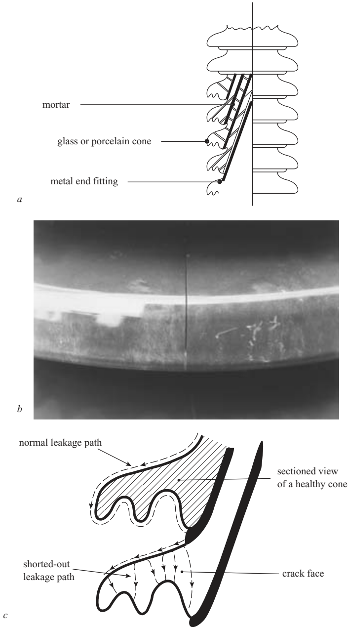
Figure 6.8 Multiple cone post
