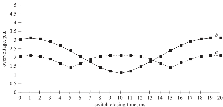
Figure 7.12 Variation of switching overvoltage with instant of switch closing t = 0 , when source voltage on phase a is maximum
