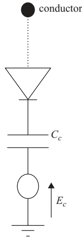
Figure 7.8 Circuit model for corona on line
