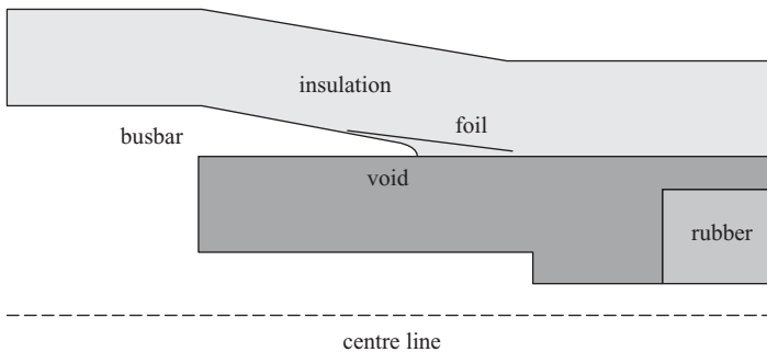
Figure 11.7 Conical bushing
