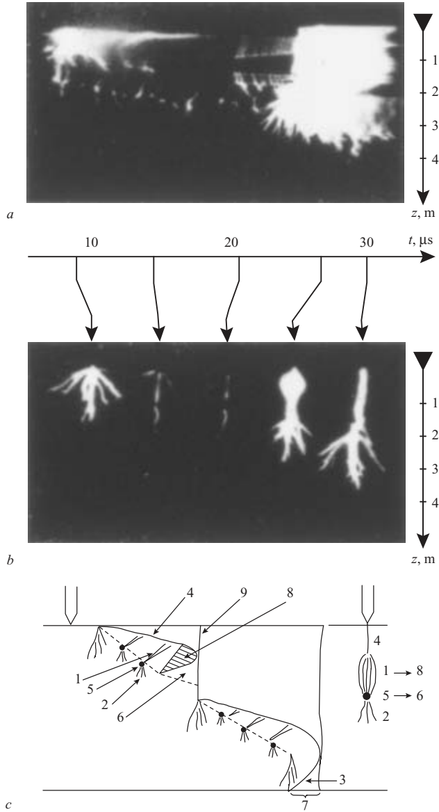
Figure 3.5 Negative space leaders in the 7 metre spark (Les Renardières) a Image-converter streak display; b Image-converter frame display (Courtesy of IEE Proceedings, Vol. 125, 1978, p. 1160); c Streak display interpretation (Courtesy of IEE Proceedings, Vol. 125, 1978, p. 1160): 1 retrograde positive corona; 2 negative corona; 3 upward positive leader; 4 downward negative leader; 5 space stem; 6 space leader elongation; 7 final jump duration; 8 leader corona region
