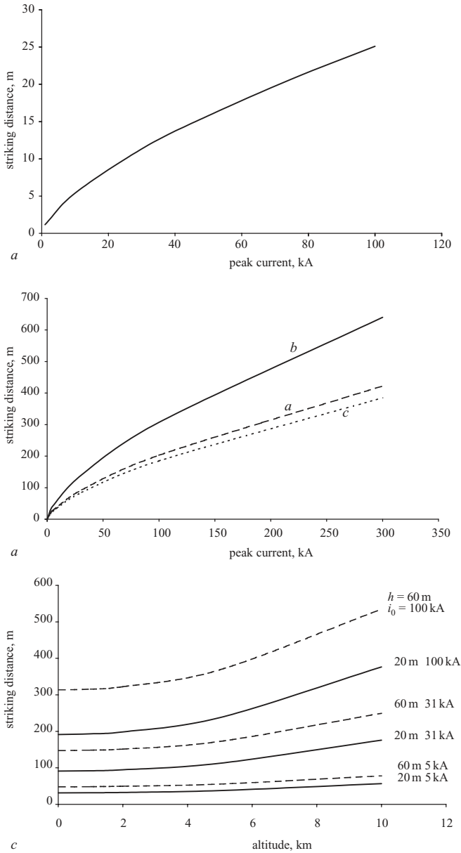
Figure 3.11 Petrov-Waters model
