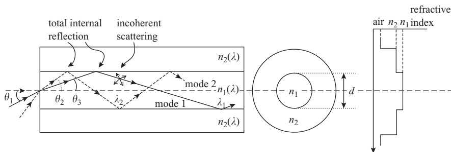
Figure 12.11 Propagation of polychromatic light in a step index optical fibre showing:
