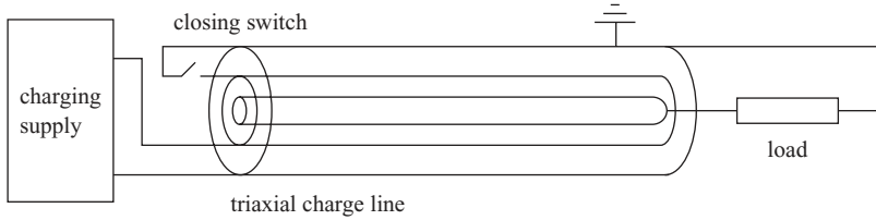
Figure 13.12 Coaxial Blumlein arrangement; the Blumlein outer conductor is usually grounded
