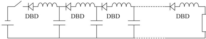
Figure 13.23 DBD-based pulse sharpening transmission line circuit
