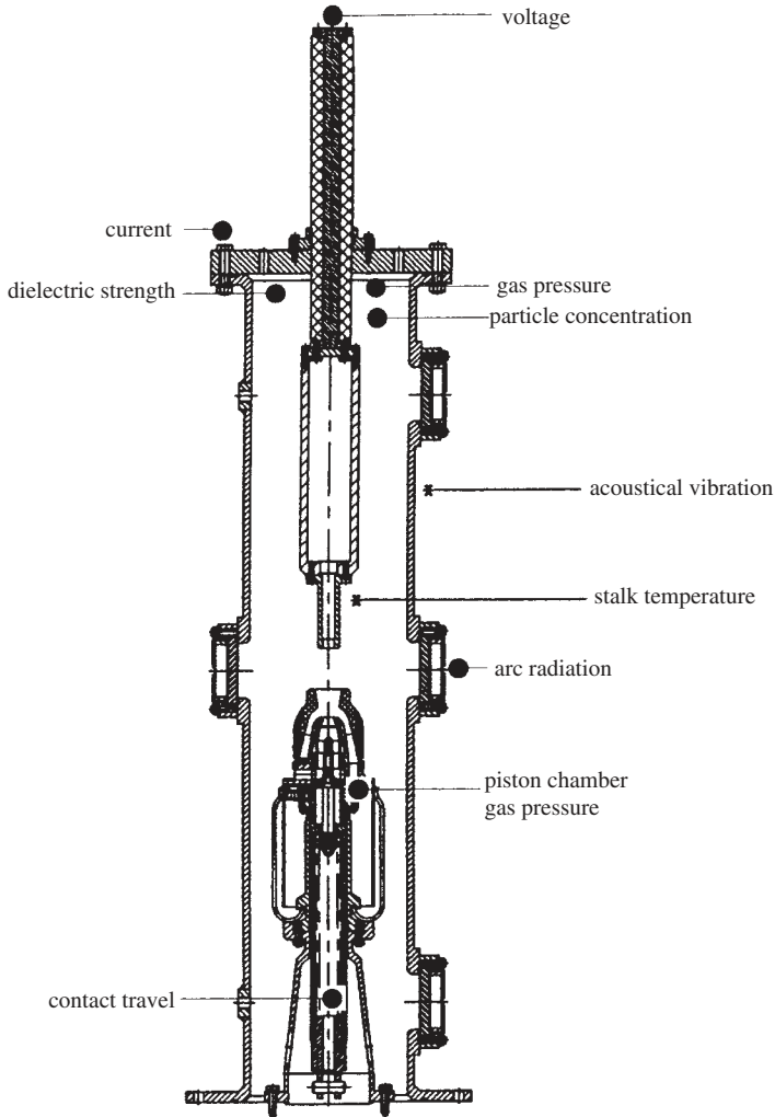
Figure 9.23 Location of various optical fibre sensors on a model high voltage \text{SF}_6 circuit breaker (after Jones et al. [4, chap. 22])
