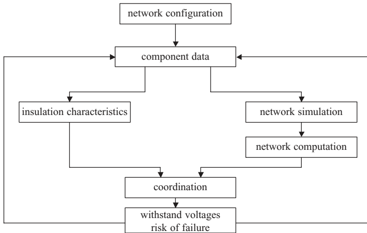
Figure 7.1 Insulation coordination
