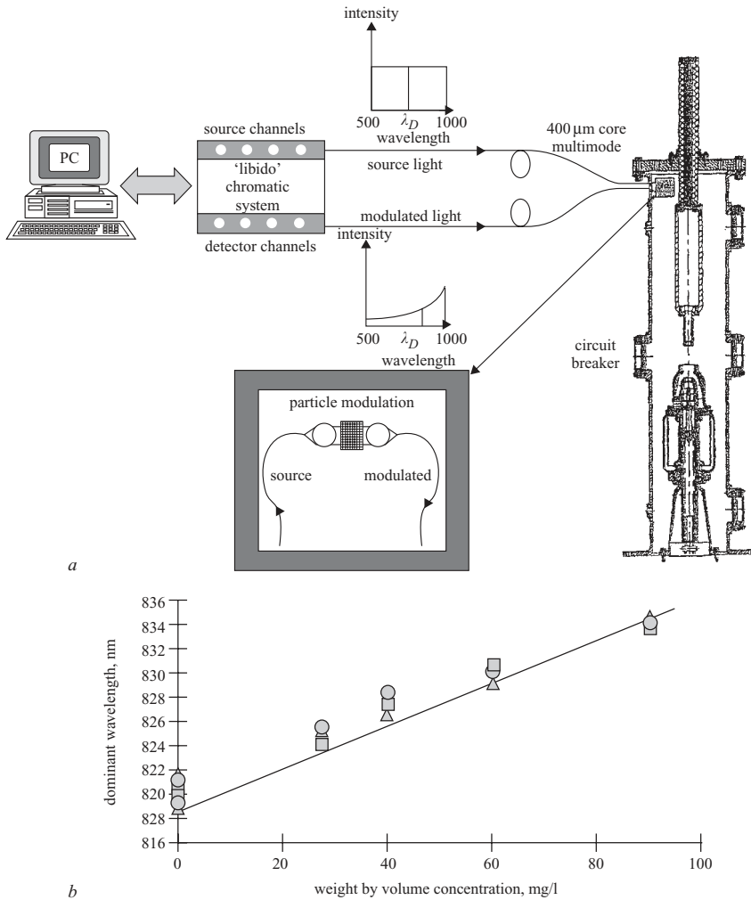
Figure 12.21 Plasma and particulate chromatic monitoring [30]
