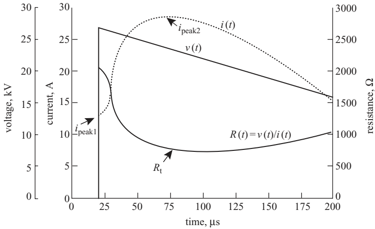
Figure 8.24 Typical voltage and current records in the ionisation region, and the ratio R(t) derived from v(t)/i(t) (water content, wc = 3\% , V_{ch} = 27 \text{ kV} [154])
