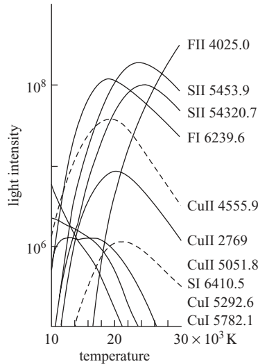
Figure 12.4 Variation of selected S, F and Cu line intensities with temperature for an \text{SF}_6 -Cu plasma (courtesy of G.R. Jones, 'High pressure arcs in industrial devices: diagnostic and monitoring techniques', published by Cambridge University Press, 1988)
