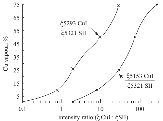
Figure 12.5 Variation of CuI: SII line intensity ratios with percentage of copper vapour impurity in \text{SF}_6 ( T = 17000 \text{ K} , P = 2 \text{ bar} ) (courtesy of D.R. Airey, PhD thesis, University of Bath, 1977)
