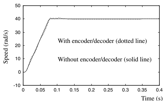
Figure 5.23 Speed responses of 0.147 kW induction motor with and without an encoder of 200 000 pulses/revolution.
