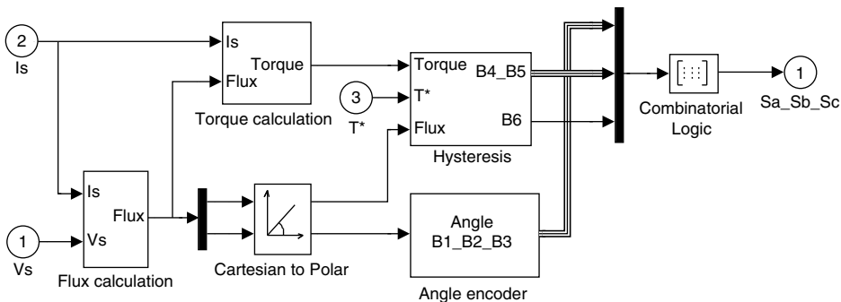
Figure 7.29 Simulink model of direct self controller.
