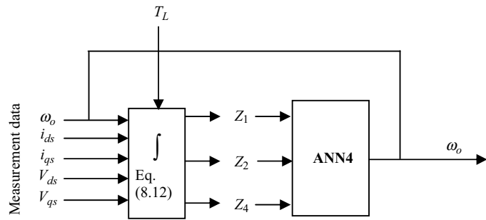
Figure 8.7 Completed ANN-based mechanical model of induction motor.
