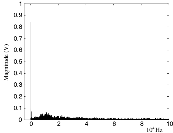
Figure 10.20 Spectrum of GA-optimized random-pulse-position PWM inverter output.
