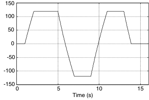
Figure 6.19 Speed response of FOC controller.
