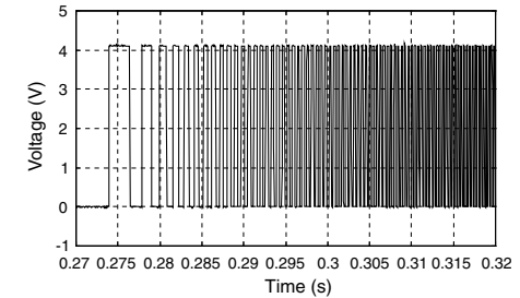
Figure 11.13 Encoder output signal acquired at a sampling rate of 20 kHz.
