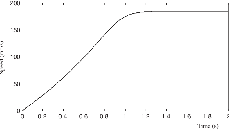
Figure 3.21 Speed response of the induction motor with direct-on-line starting.
