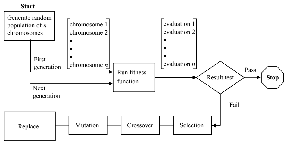
Figure 4.31 Calculation process of basic genetic algorithm.
