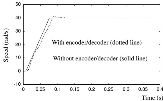
Figure 5.22 Speed responses of 0.147 kW induction motor with and without an encoder of 20 000 pulses/revolution.
