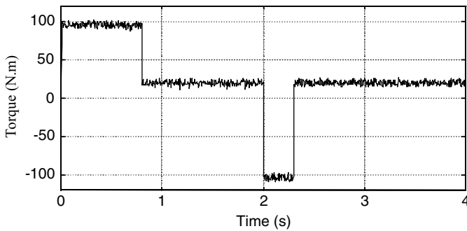
Figure 7.19 Torque response of ANN-DSC with 25 \mu s delay. (Reproduced by permission of K.L. Shi, T.F. Chan, Y.K. Wong and S.L. Ho, “Direct self control of induction motor based on neural network,” IEEE Transactions on Industry Applications , 37 (5), 2001: 1290–1298. © 2001 IEEE.)
