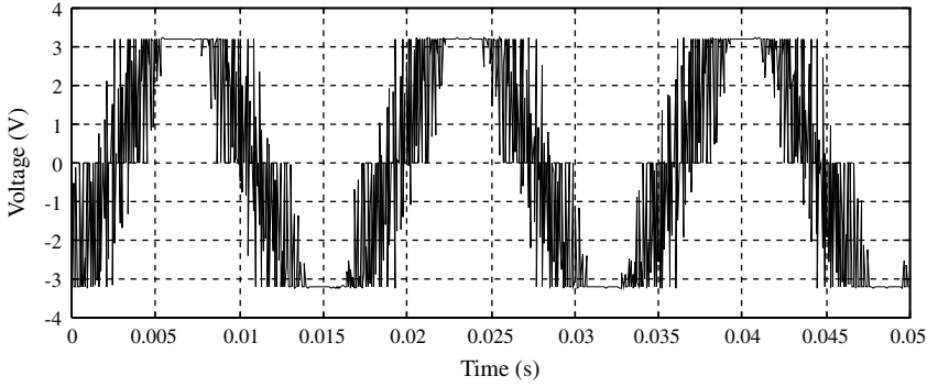
Figure 11.8 Output line voltage V_{ab} of the inverter PowIRtrain acquired at a sampling rate of 20 kHz.
