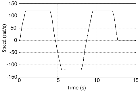
Figure 6.18 Speed response of fuzzy controller.
