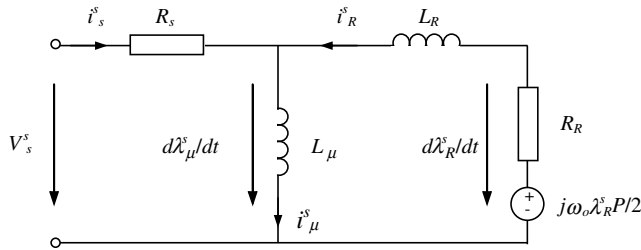
Figure A.1 ‘ \Gamma ’ equivalent circuit model of an induction motor.
