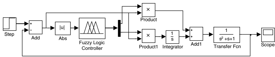
Figure 4.5 Modeling fuzzy PI control system in Simulink.
