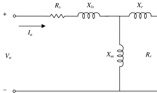
Figure H.4 Equivalent circuit of three-phase induction motor under locked-rotor test.
