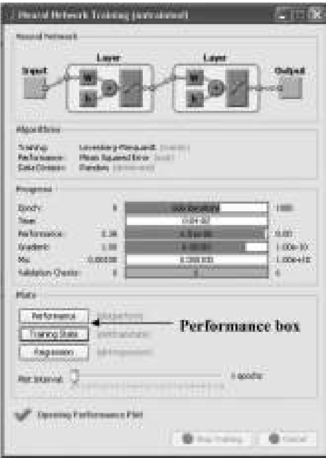
Figure 4.17 Training window.
