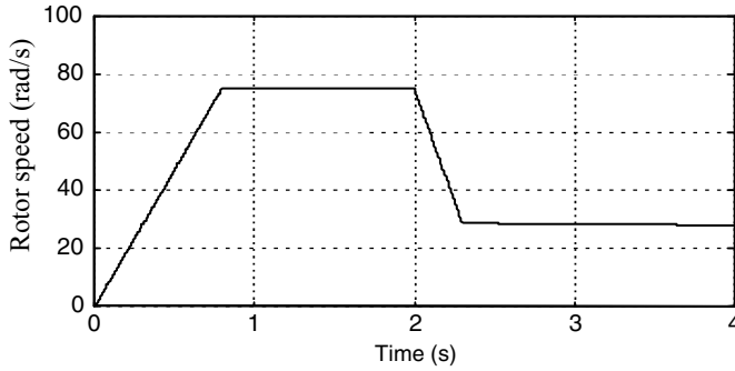
Figure 7.18 Speed response of DSC with 100 \mu s delay. (Reproduced by permission of K.L. Shi, T.F. Chan, Y.K. Wong and S.L. Ho, “Direct self control of induction motor based on neural network,” IEEE Transactions on Industry Applications , 37 (5), 2001: 1290–1298. © 2001 IEEE.)
