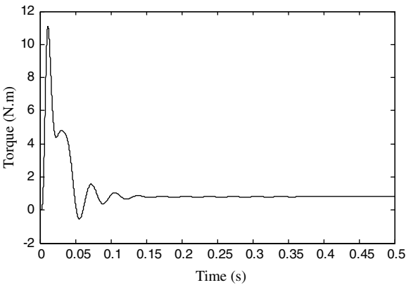
Figure 6.42 Torque of the 0.147 kW induction motor.
