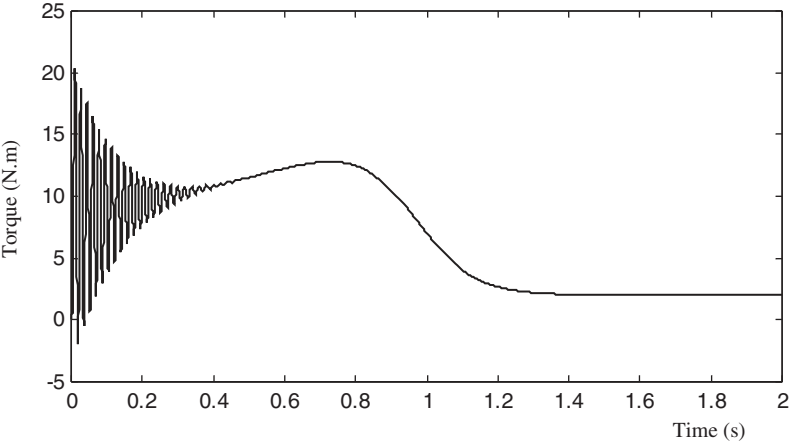
Figure 3.20 Torque response of the induction motor with direct-on-line starting.
