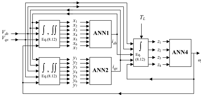
Figure 8.9 ANN model of induction motor.
