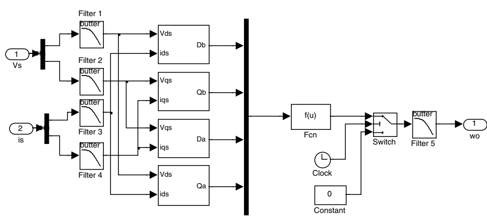
Figure 8.32 Speed estimation model.
