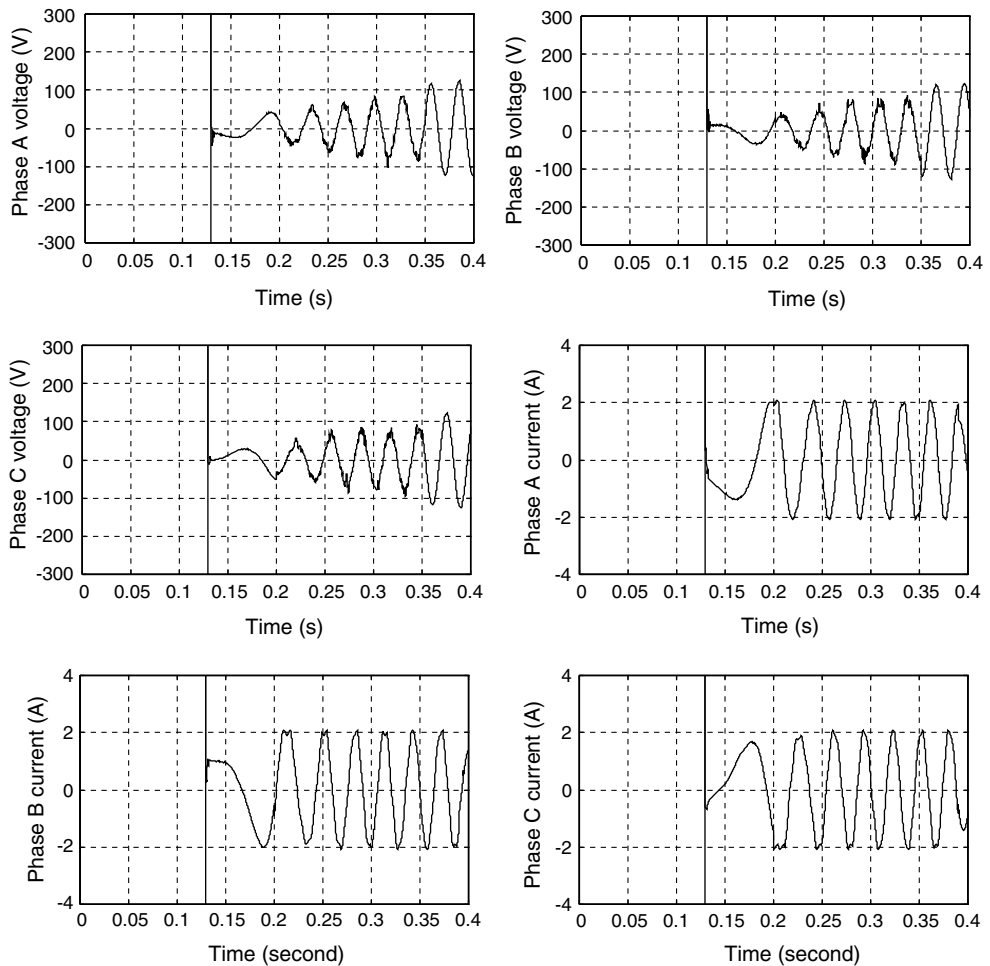
Figure 11.21 Three-phase stator voltages and currents in the acceleration stage.
