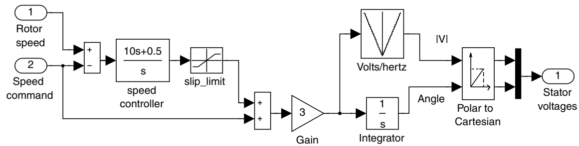
Figure 9.3 Simulink program of closed-loop V/Hz controller.
