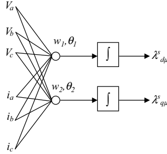
Figure 7.3 A dynamic net of the flux estimation. (Reproduced by permission of K.L. Shi, T.F. Chan, Y.K. Wong and S.L. Ho, "Direct self control of induction motor based on neural network," IEEE Transactions on Industry Applications , 37 (5), 2001: 1290–1298. © 2001 IEEE.)
