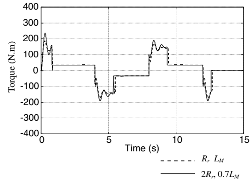
Figure 6.21 Torque response of fuzzy controller with parameter variations.
