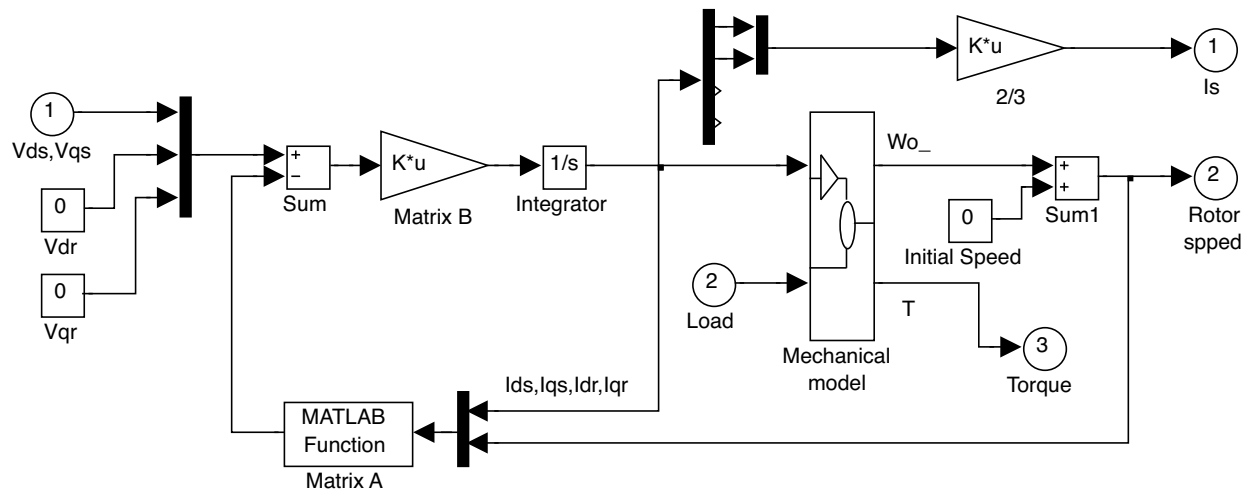
Figure 6.37 Voltage-input model of 0.147 kW induction motor.
