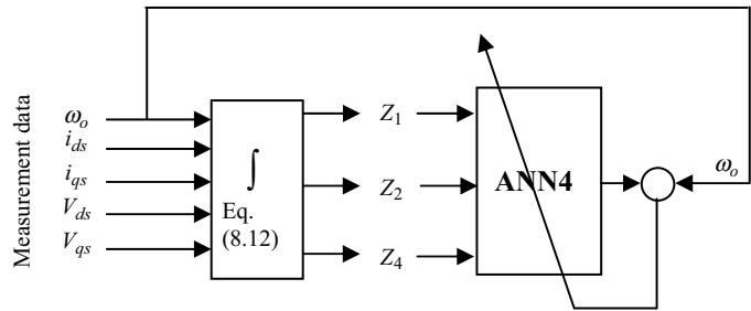
Figure 8.6 Training scheme of ANN-based mechanical model of induction motor with T_L = 0 .
