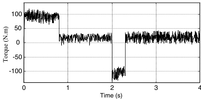
Figure 7.17 Torque response of DSC with 100 \mu s delay. (Reproduced by permission of K.L. Shi, T.F. Chan, Y.K. Wong and S.L. Ho, “Direct self control of induction motor based on neural network,” IEEE Transactions on Industry Applications , 37 (5), 2001: 1290–1298. © 2001 IEEE.)
