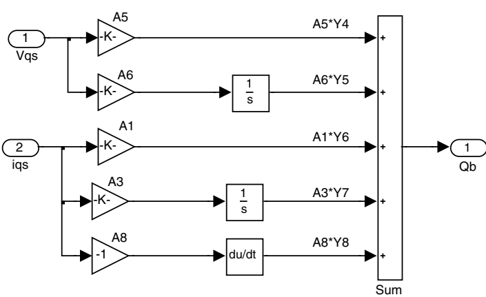
Figure 8.31 Simulink model of Q_b .
