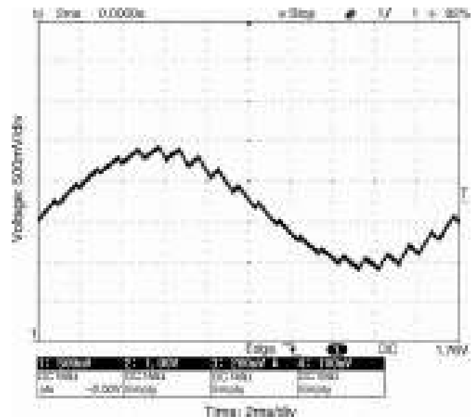
Figure 11.35 Filter output waveform from PWM1A.
