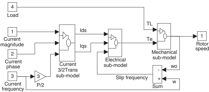
Figure 3.1 Current-input model of an induction motor in Simulink.
