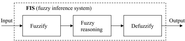
Figure 4.1 A basic fuzzy inference system.
