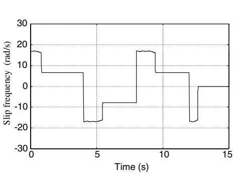
Figure 6.14 Slip frequency of fuzzy controller.
