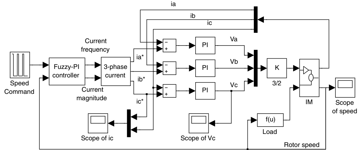
Figure 6.31 Simulink program of fuzzy/PI control system with voltage-input model of induction motor. (Reproduced by permission of K.L. Shi, T.F. Chan, Y.K. Wong and S.L. Ho, “A novel hybrid fuzzy/PI two-stage controller for an induction motor drive,” IEEE International Electric Machines and Drives Conference (IEMDC 2001), pp. 415–421, June 17–20, 2001, Cambridge, MA, U.S.A. © 2001 IEEE.)
