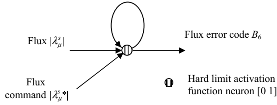
Figure 7.11 Flux hysteresis comparator of neural network. (Reproduced by permission of K.L. Shi, T.F. Chan, Y.K. Wong and S.L. Ho, “Direct self control of induction motor based on neural network,” IEEE Transactions on Industry Applications , 37 (5), 2001: 1290–1298. © 2001 IEEE.)
