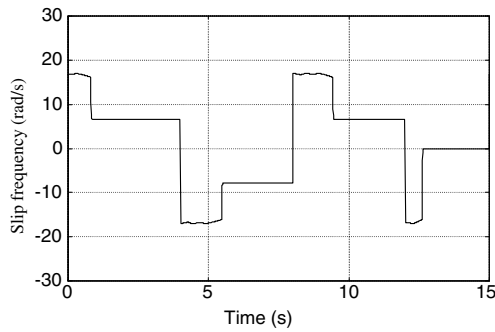
Figure 6.29 Slip with load torque variation.
