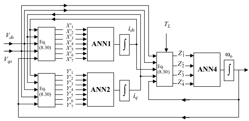
Figure 8.10 ANN model of induction motor without involving double integrals.
