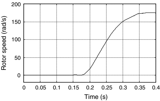
Figure 11.19 Rotor speed response in the acceleration stage.
