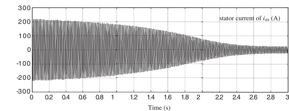
Figure 3.9 Stator current when internal resistance of power supply is 0.2\Omega . (Reproduced by permission of K.L. Shi, T.F. Chan and Y.K. Wong, “Modelling of the three-phase induction motor using SIMULINK”, The 1997 IEEE Biennial International Electrical Machines and Drives Conference , Paper WB3-6, 18–21 May 1997, Milwaukee, Wisconsin, U.S.A. © 1997 IEEE.)
