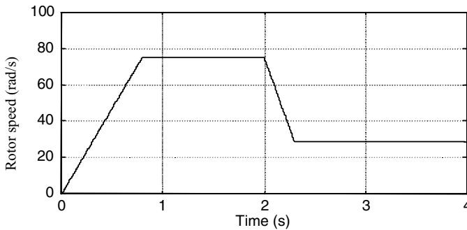
Figure 7.20 Speed response of ANN-DSC with 25 \mu s delay. (Reproduced by permission of K.L. Shi, T.F. Chan, Y.K. Wong and S.L. Ho, “Direct self control of induction motor based on neural network,” IEEE Transactions on Industry Applications , 37 (5), 2001: 1290–1298. © 2001 IEEE.)
