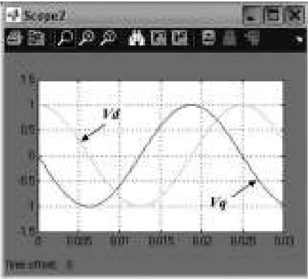
Figure 3.60 Simulation results of Example 3.6.
