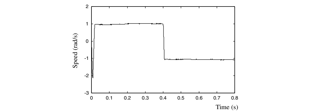
Figure 5.20 Speed response of 0.147 kW induction motor when speed command is 1 rad/s and -1 rad/s.
