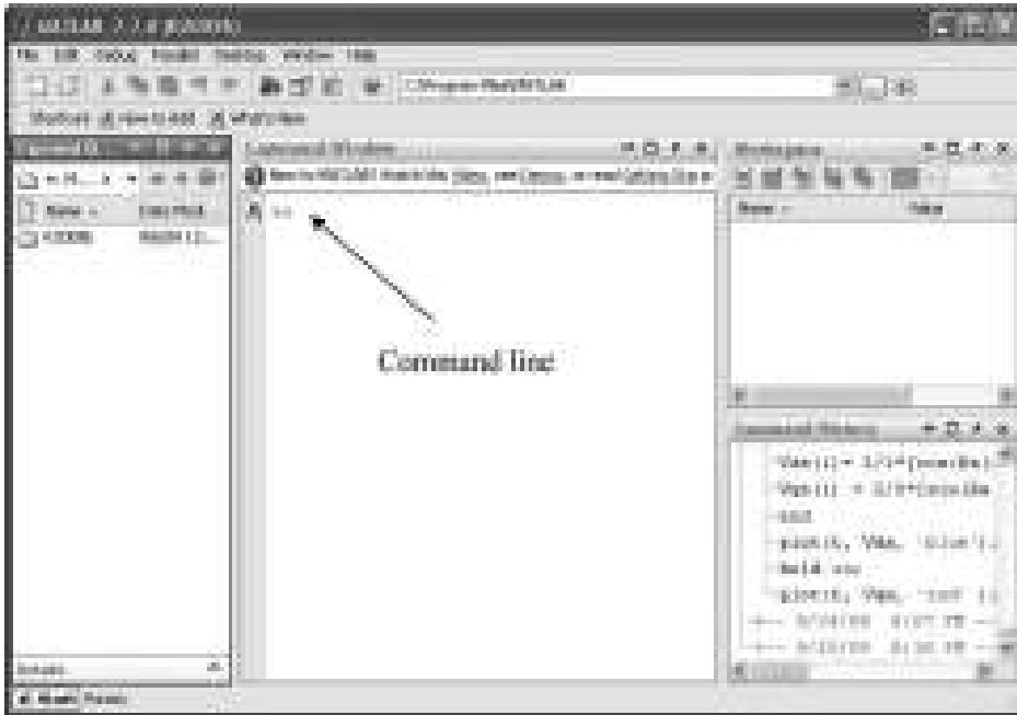
Figure 3.42 MATLAB® window.
