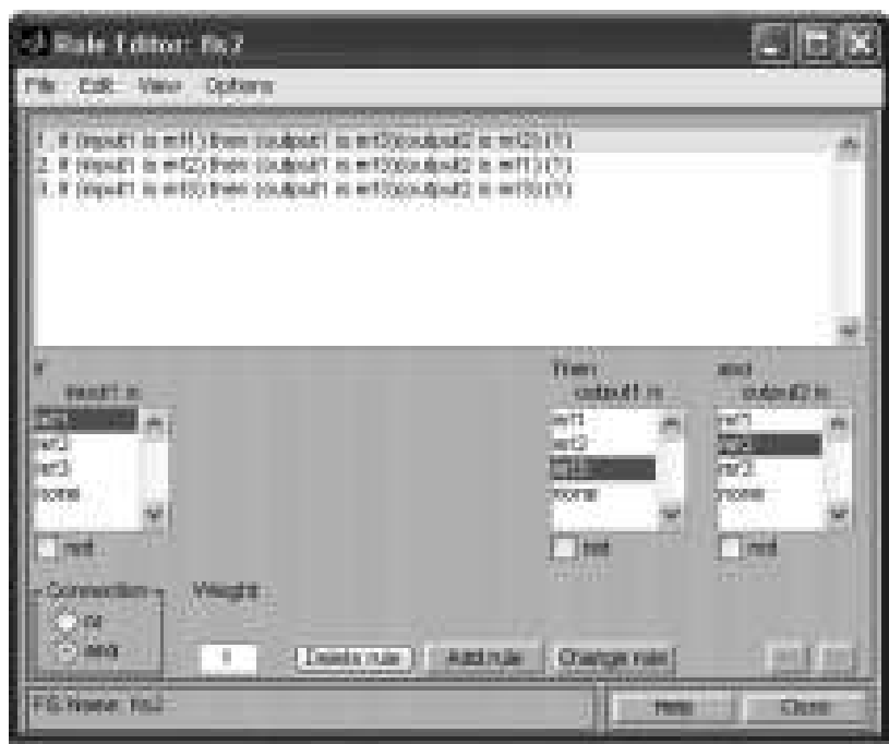
Figure 4.10 Rule editor.
