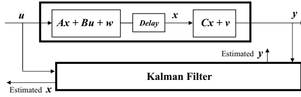
Figure 4.25 A system model and a basic Kalman Filter.
