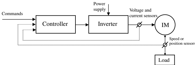
Figure 1.1 An induction motor control system.
