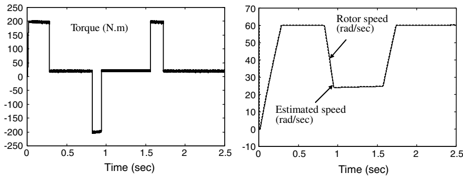
Figure 9.9 Torque, rotor speed, and estimated speed of the sensorless direct self controller.
