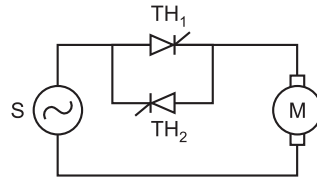
Fig. 8.3. Reversible 1-pulse converter
