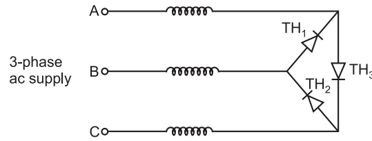
Fig. 8.13. Neutral point regulator
