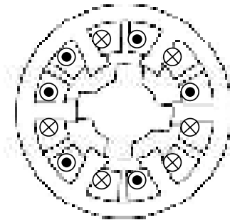
Figure 4.40. Variable reluctance motor, with 3 phases, 6 teeth and 4 rotor poles with winding
