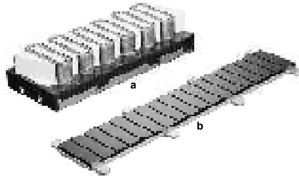
Figure 4.46. Components of a linear synchronous motor with permanent motors: a) polyphased structure; b) track with permanent magnets
