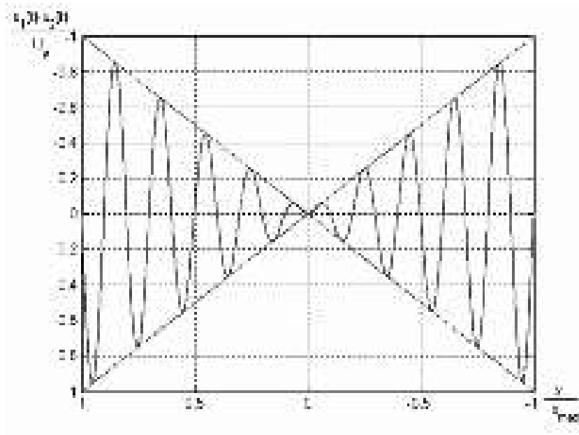
Figure 10.10. LVDT sensor – signal measurement, amplitude and phase
