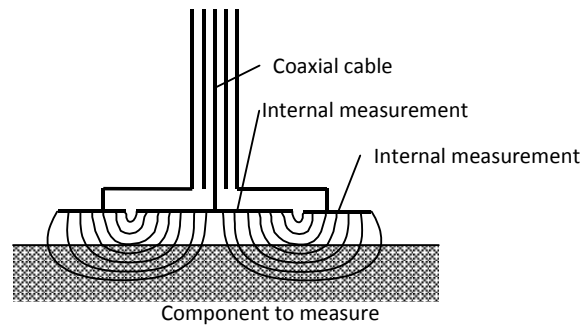
Figure 10.19. Capacitive measuring principle
