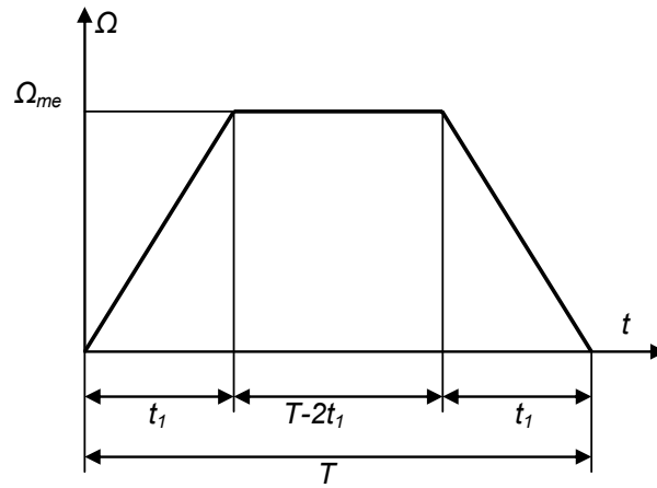
Figure 6.1. Trapezium shape speed profile
