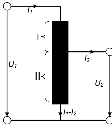
Figure 8.2. Autotransformer
