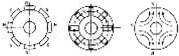
Figure 4.27. a) Rotor structures of PM synchronous motors
