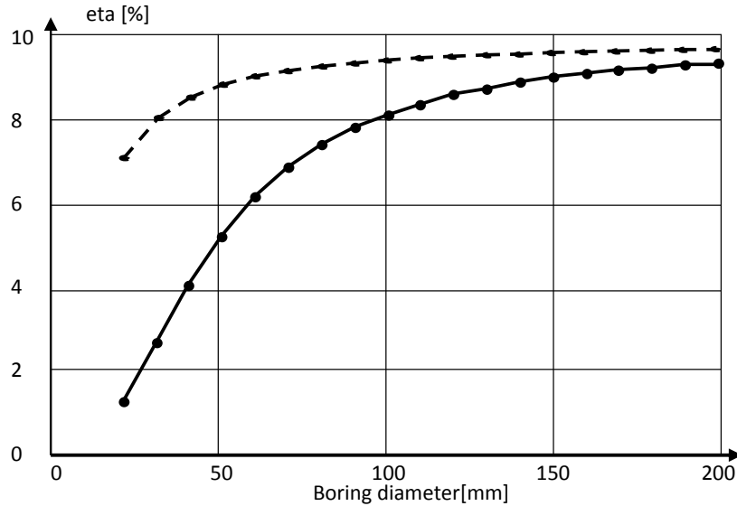
Figure 11.4. PM and induction motors – efficiency comparison according to the diameter
