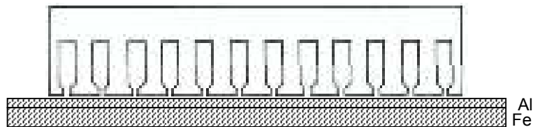
Figure 4.43. Structure of an asynchronous linear motor with a single armature in Al and Fe
