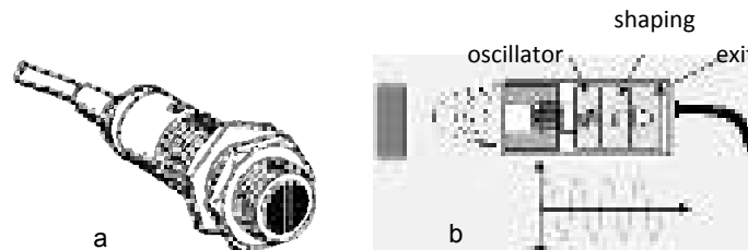
Figure 10.5. Inductive proximity sensor: a) probe; b) structure
