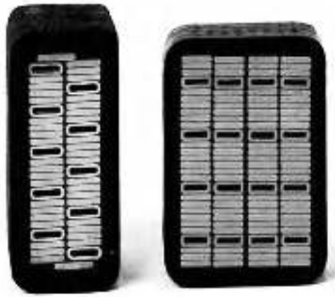
Figure 7.12. Roebel's bars with water tube distribution, arranged between partial conductors
