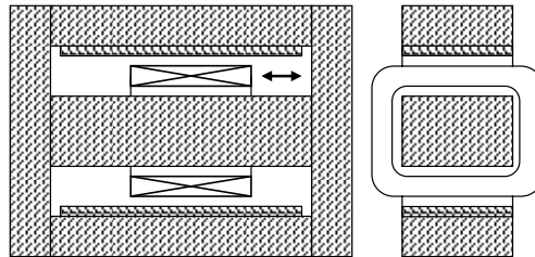
Figure 4.52. Elimination of the reluctance effect of reluctance by a symmetrical ferromagnetic circuit
