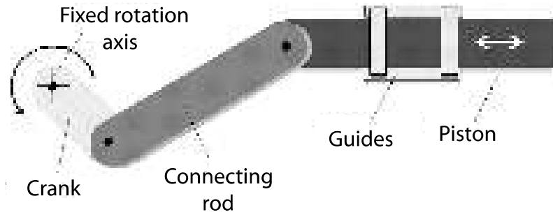
Figure 3.7. Rod system
