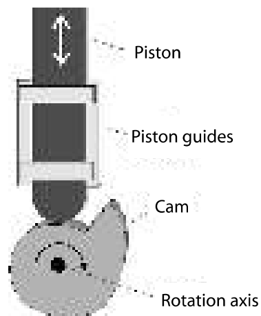
Figure 3.6. Cam system
