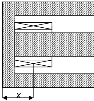
Figure 4.49. Coil position
