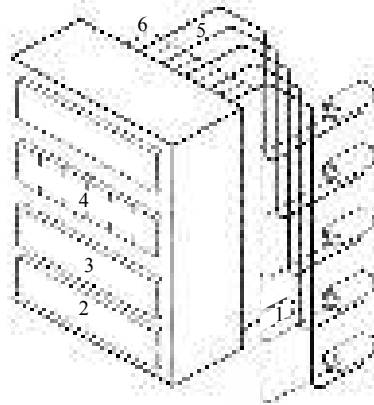
Figure 12.4. Power and control of a 5 axis robot to a central cabinet and corresponding cabling; 1) AC supply; 2) transformer-rectifier; 3) axis control; 4) motor supply and control; 5) motor 3-phase cables; 6) sensor cables
