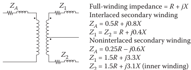
Figure 5.8 Model of a 120/240-V secondary winding with all impedances in percent. (Impedance data from Hopkinson, F. H., Approximate distribution transformer impedances , General Electric Internal Memorandum , 1976. As cited by Kersting, W. H. and Phillips, W. H., Modeling and analysis of unsymmetrical transformer banks serving unbalanced loads , Rural Electric Power Conference , 1995.)
