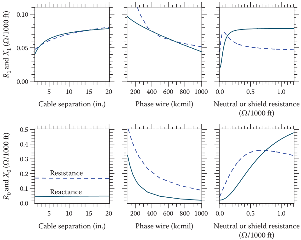
Figure 4.7 Effect of various parameters on the positive-sequence (top row) and zero-sequence impedances (bottom row) with a base case having 500-kcmil aluminum cables with 1/3 neutrals, 220-mil insulation, a horizontal configuration with 7.5 in. between cables, and \rho = 100 \Omega\text{-m} .
