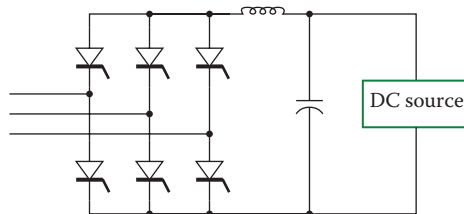
Figure 15.3 Common three-phase bridge inverter line-commutated configuration with thyristors.
