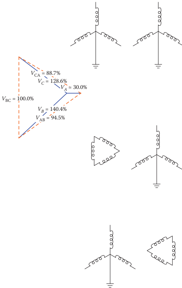
Figure 15.9 Line-to-line and line-to-ground voltages on the primary and secondary of several transformer connections for an overvoltage due to a neutral shift for a fault on primary phase A. (From EPRI 1005917, Distributed Generation Relaying Impacts on Power Quality , Electric Power Research Institute, Palo Alto, CA, 2001. Copyright 2001. Reprinted with permission.)
