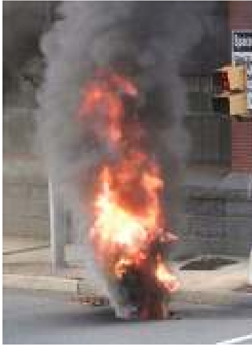
Figure 14.33 Example manhole event. (From EPRI 1015889, Manhole Event Risk Management Strategies: High-Level Overview , Electric Power Research Institute, Palo Alto, CA, 2008. Copyright 2008. Reprinted with permission.)
