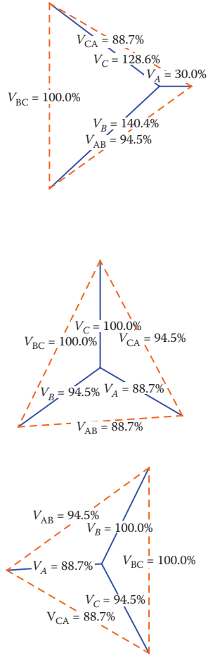
Figure 15.9 Line-to-line and line-to-ground voltages on the primary and secondary of several transformer connections for an overvoltage due to a neutral shift for a fault on primary phase A. (From EPRI 1005917, Distributed Generation Relaying Impacts on Power Quality , Electric Power Research Institute, Palo Alto, CA, 2001. Copyright 2001. Reprinted with permission.)
