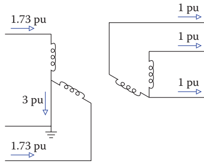
Figure 5.16 Current flow in an open wye–open delta transformer with balanced three-phase load.
