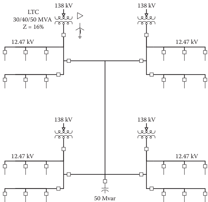
Figure 1.14 Example of an urban distribution substation.
