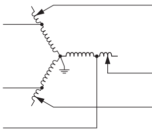
Open-delta connection
