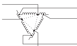
Closed-delta (leading) connection
