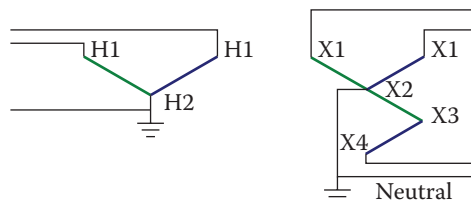
Figure 5.17 Quasiphasor diagram of an open-wye primary connection supplying a wye four-wire neutral service such as 208Y/120 V. (ANSI/IEEE C57.105-1978, IEEE Guide for Application of Transformer Connections in Three-Phase Distribution Systems . © 1978 IEEE.)
