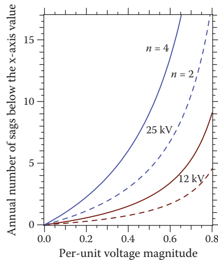
Figure 11.8 Cumulative distribution of substation bus voltage sags per year for the given (25-MVA, 10% transformer, 500-kcmil feeder, n = 2 or 4 feeders off of the bus, \lambda = 1 faults/phase/mile of mains/year, assumes line-to-ground faults only). (From EPRI 1001665, Power Quality Improvement Methodology for Wires Companies , Electric Power Research Institute, Palo Alto, CA, 2003. Copyright 2003. Reprinted with permission.)
