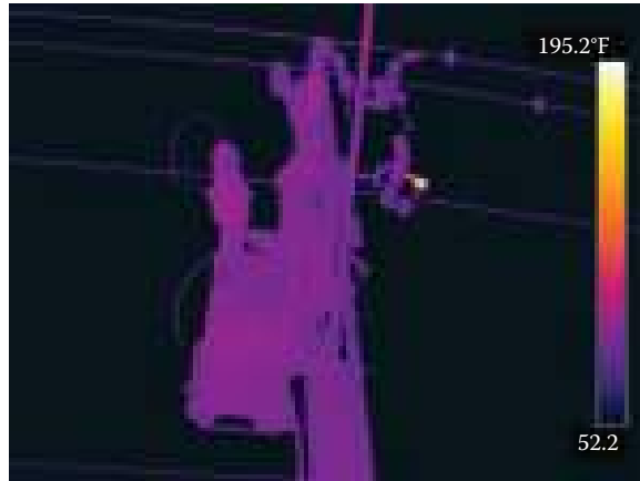
Figure 7.24 Hot capacitor cutout. Note the blown fuse on another phase. (Courtesy of Osmose Utilities Services, Inc.)
