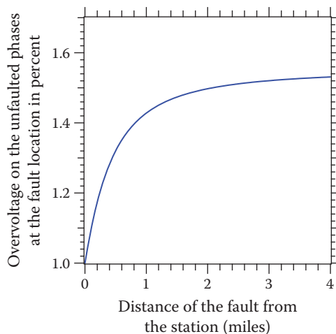
Figure 14.9 Voltage on the unfaulted phases for a system with 500-kcmil, triplex, copper-conductor, tape-shield cables. 12.47 kV, Z_1 = 0.0292 + j0.0355 \Omega/1000 \text{ ft} , Z_0 = 0.3765 + j0.2882 \Omega/1000 \text{ ft} , Z_{src} = j0.7 \Omega .
