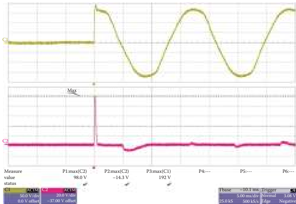
Figure 11.34 Example inrush after an interruption when energized at voltage peak. (From EPRI 1012451, The Effects of Post-Sag Inrush on Residential Equipment , Electric Power Research Institute, Palo Alto, CA, 2006. Copyright 2006. Reprinted with permission.)
