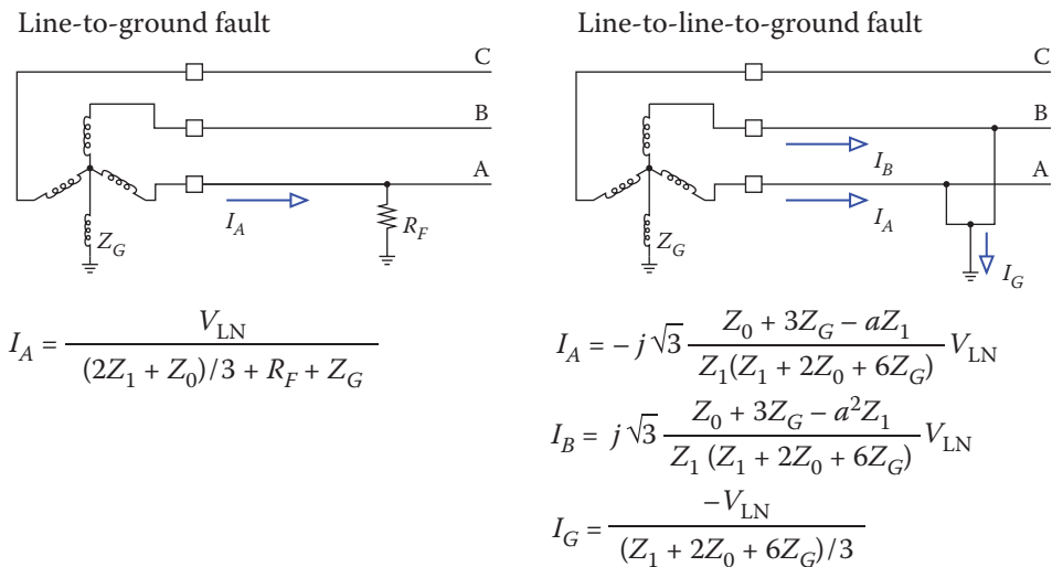
Figure 8.8 Fault-current calculations with a neutral reactor on the substation transformer.
