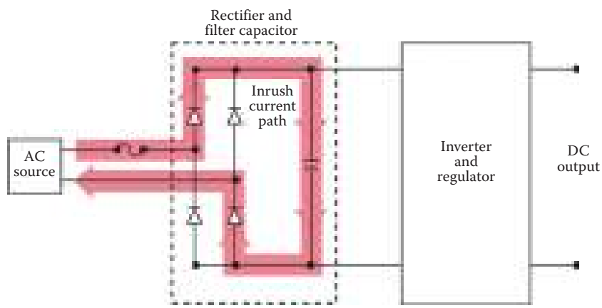
Figure 11.33 Post-sag inrush path through a power supply. (From EPRI 1012451, The Effects of Post-Sag Inrush on Residential Equipment , Electric Power Research Institute, Palo Alto, CA, 2006. Copyright 2006. Reprinted with permission.)
