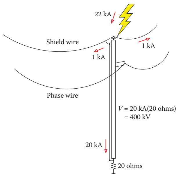
Figure 13.28 Shield-wire lightning protection system.
