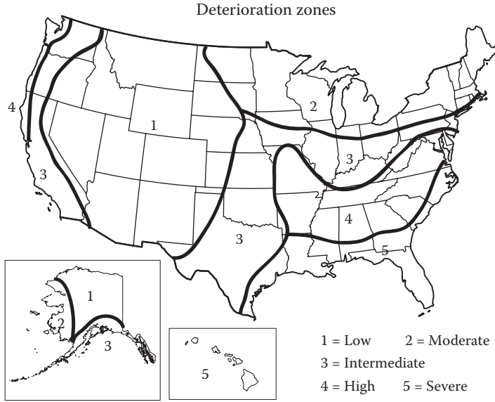
Figure 3.25 Wood pole deterioration zones from AWP Standard U1 (2013). (Courtesy of the American Wood Protection Association.)
