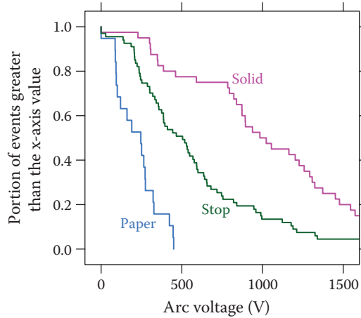
Figure 8.33 Estimates of arc voltage by splice failure type (utility C). (Adapted from EPRI 1012438, Distribution Fault Location: Field Data and Analysis , Electric Power Research Institute, Palo Alto, CA, 2006.)
