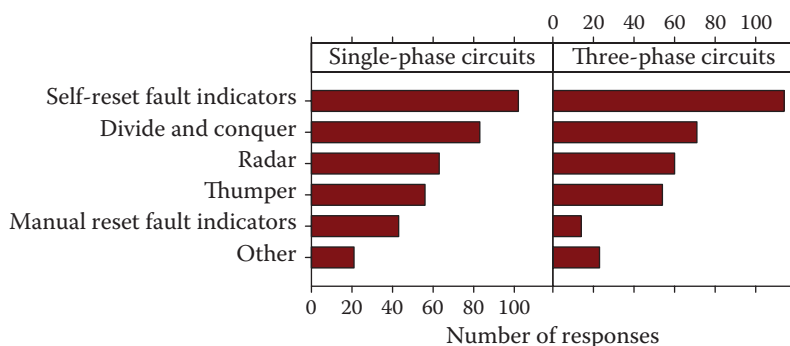
Figure 4.22 Utility use of fault-locating techniques (204 utilities surveyed, multiple responses allowed). (Data from Boucher, R., A summary of the regional underground distribution practices for 1991, Regional Underground Distribution Practices, IEEE paper 91 TH0398-8-PWR, 1991.)
