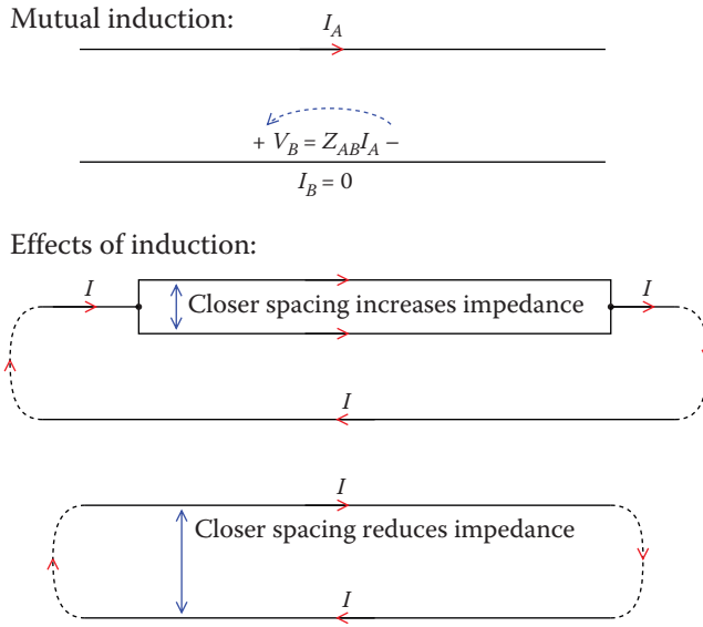
Figure 2.6 Mutual induction.
