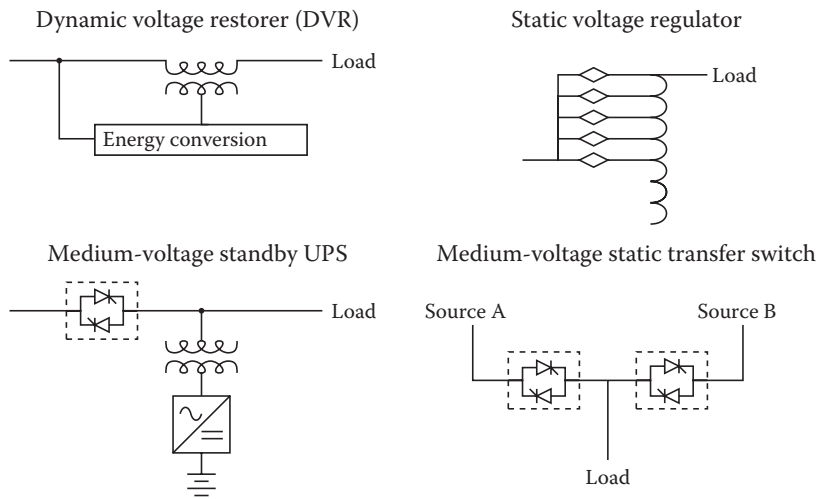
Figure 11.39 Common custom-power devices.
