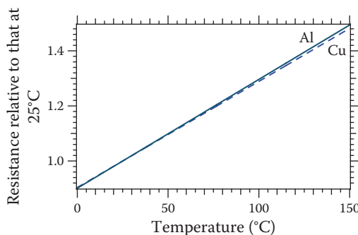
Figure 4.5 Resistance change with temperature.
