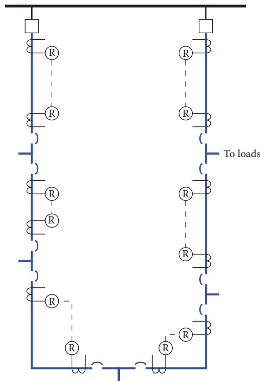
Figure 1.7 Example of a closed-loop distribution system.
