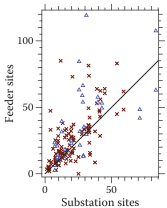
Figure 11.16 SARFI ITIC at substation sites plotted against SARFI ITIC at that substation's feeder sites (triangles indicate rural sites).
