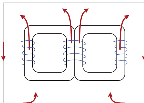
Stray flux in the tank due to zero sequence current
