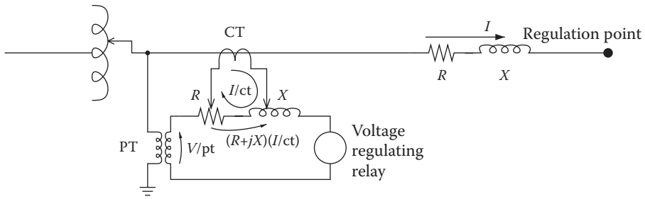
Figure 6.6 Line drop compensator circuit.
