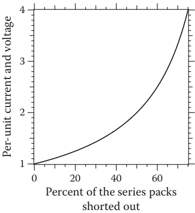
Figure 7.16 Per-unit current drawn by a failing bank depending on the portion of the bank that is failing (assuming an infinite bus). This is also the per-unit voltage applied on the series sections still remaining.
