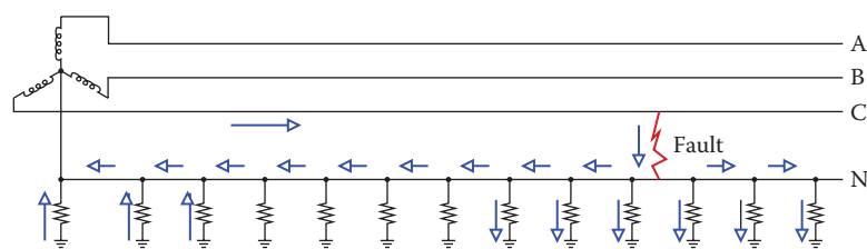
Figure 14.5 Fault current paths for a line-to-ground fault.
