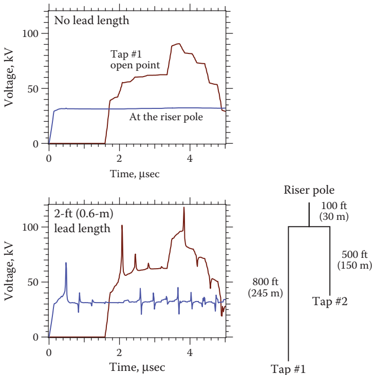
Figure 13.23 Transient simulation of traveling waves on a tapped cable (0.5-μsec risetime).
