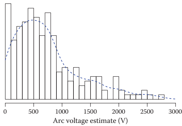
Figure 8.29 Histogram of arc voltages in the DPQ study. (From EPRI 1012438, Distribution Fault Location: Field Data and Analysis , Electric Power Research Institute, Palo Alto, CA, 2006. Copyright 2009. Reprinted with permission.)
