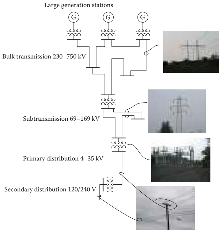
Figure 1.2 Overview of the electricity infrastructure.
