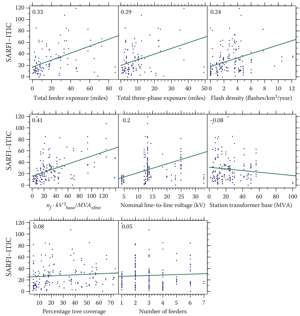
Figure 11.19 Variations in the number of excursions below the lower ITI curve (which are mainly voltage sags) versus various site parameters. The correlation coefficients (r) are given in the upper-left corner of each plot.
