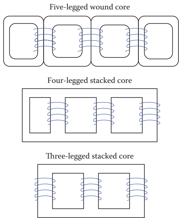
Figure 5.11 Three-phase core constructions.
