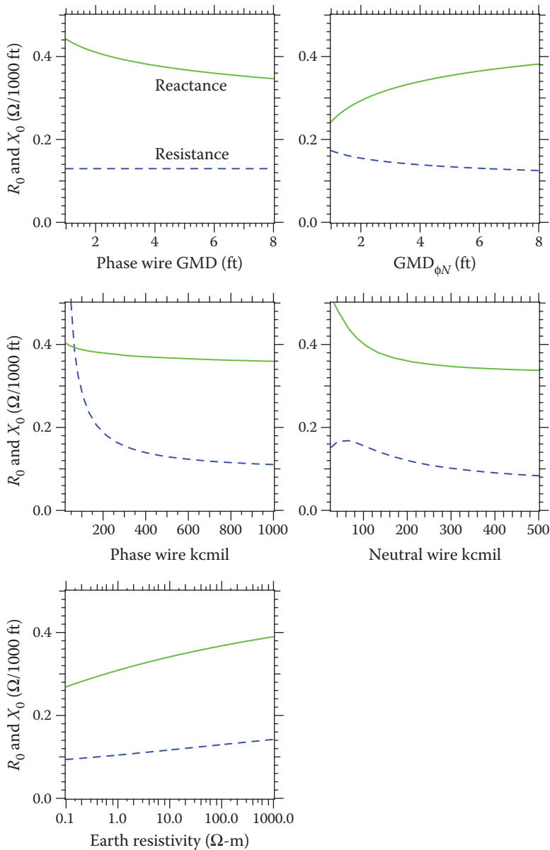
Figure 2.11 Effect of various parameters on the zero-sequence impedance with a base case of AAC 500-kcmil phases, 3/0 neutral (168 kcmil), \text{GMD}_\phi = 5 ft, \text{GMD}_{\phi N} = 6.3 ft, and \rho = 100 \Omega\text{-m} .
