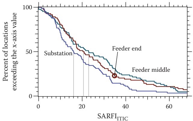
Figure 11.15 Comparison of feeder sites and substation sites in the DPQ data for SARFI ITIC .
