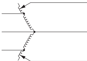
Figure 6.4 Three-phase regulator connections.
