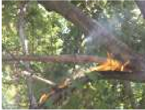
Figure 14.28 Open flame on a silver maple branch energized at 7.6 kV. (From EPRI 1016219, Optimal Design of Overhead Distribution Systems: Understanding Touch Voltage Potential Risks Due to Tree-to-Conductor Contacts on Distribution Circuits , Electric Power Research Institute, Palo Alto, CA, 2007. Copyright 2007. Reprinted with permission.)
