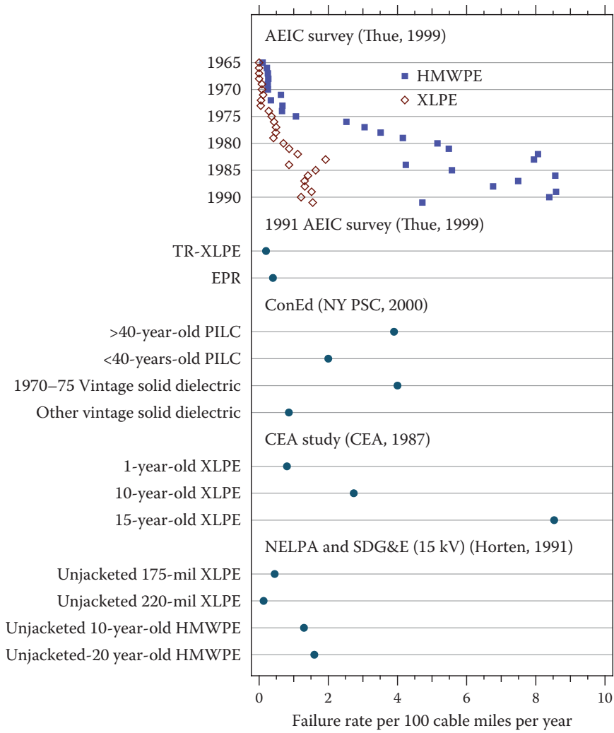
Figure 4.17 Cable failure rates found in different studies and surveys (in cable miles, not circuit miles). (Data from CEA 117 D 295, Survey of Experience with Polymer Insulated Power Cable in Underground Service , Canadian Electrical Association, 1987; Horton, W. F. and Golberg, S., Determination of failure rates of underground distribution system components from historical data , IEEE/PES Transmission and Distribution Conference , 1991; State of New York Department of Public Service, A report on consolidated Edison's July 1999 system outages , March 2000; Thue, 1999.)
