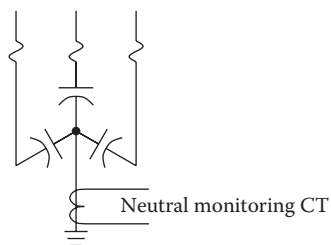
Figure 7.26 Neutral monitoring of a capacitor bank.
