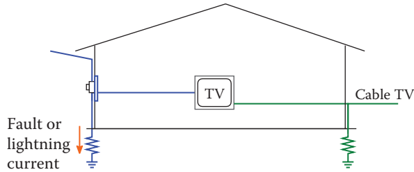
Figure 12.5 Example of a two-port voltage stress at a television between its power source and the cable TV cable.
