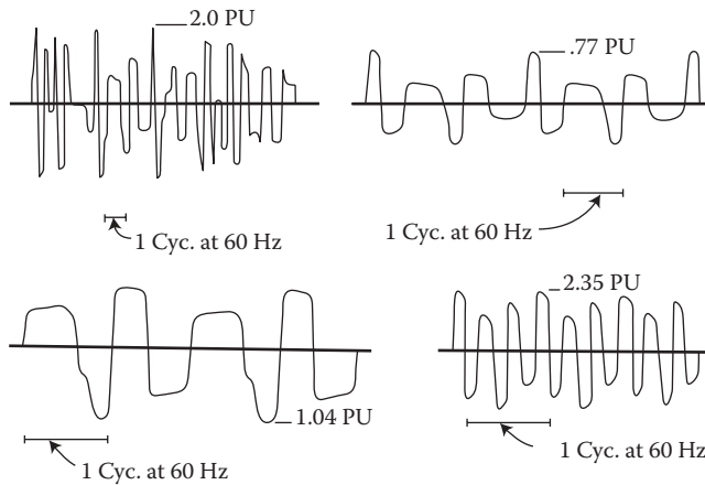
Figure 5.28 Example of ferroresonance. (From Smith, D. R., Swanson, S. R., and Borst, J. D., IEEE Transactions on Power Apparatus and Systems , PAS-94(5), 1843–53, 1975. Copyright 1975 IEEE. With permission.)
