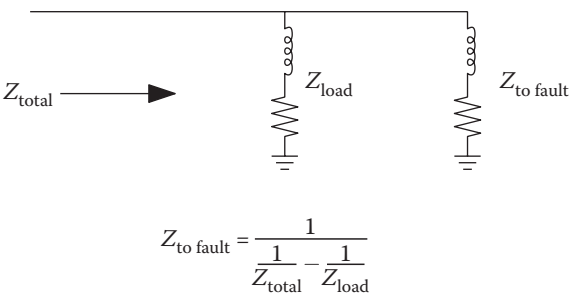
Figure 8.22 Constant-impedance load model.
