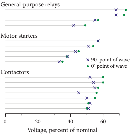
Figure 11.26 Voltage magnitude for dropout of several relays and contactors for a five-cycle voltage sag. (Data from EPRI PEAC Brief No. 44, The Effects of Point-on-Wave on Low-Voltage Tolerance of Industrial Process Devices , EPRI PEAC, Knoxville, TN, 1998.)
