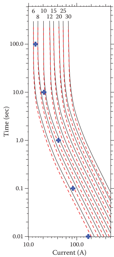
Figure 9.11 Transformer inrush and cold-load pickup points for a single-phase, 50-kVA, 7.2-kV transformer. The minimum-melt curves and damage curves (dotted lines) for K-link fuses are also shown.
