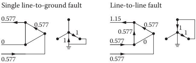
Figure 8.9 Per-unit fault currents on both sides of a delta-grounded-wye transformer.
