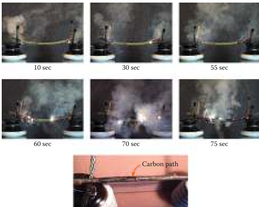
Figure 3.5 Progression of arcing and carbonization of a branch. (From Goodfellow, J., BioCompliance Consulting, Inc. With permission.)
