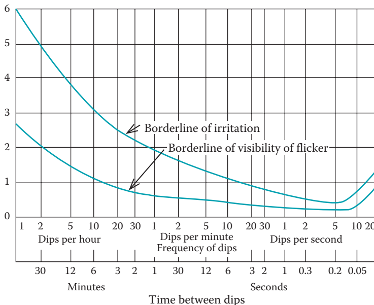
Figure 12.21 GE flicker curve. (IEEE Std. 141-1993, IEEE Recommended Practice for Electric Power Distribution for Industrial Plants . © 1994 IEEE.)
