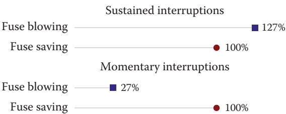
Figure 9.20 Comparison of fuse saving and fuse blowing on a hypothetical circuit. Mains: 10 miles (16.1 km), fault rate = 0.5/mile/year (0.8/km/year), 75% temporary. Taps: 10 miles (16.1 km) total, 20 laterals, fault rate = 2/mile/year (3.2/km/year), 75% temporary. It also assumes that fuse saving is 100% successful.
