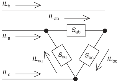
FIGURE 21.26 Delta connected load.
