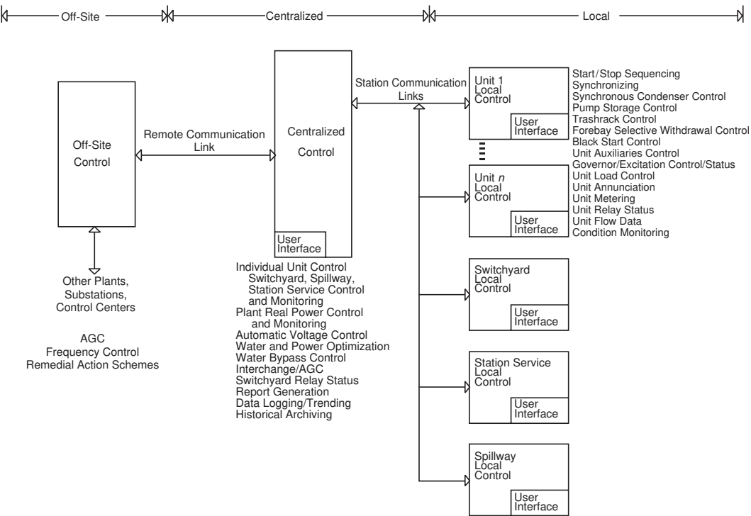
FIGURE 4.5 Relationship of local, centralized, and off-site control. (From IEEE Standard 1249, IEEE Guide for Computer-Based Control for Hydroelectric Power Plant Automation.)
