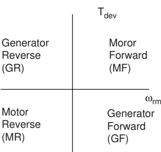
FIGURE 27.2 Operating modes.
