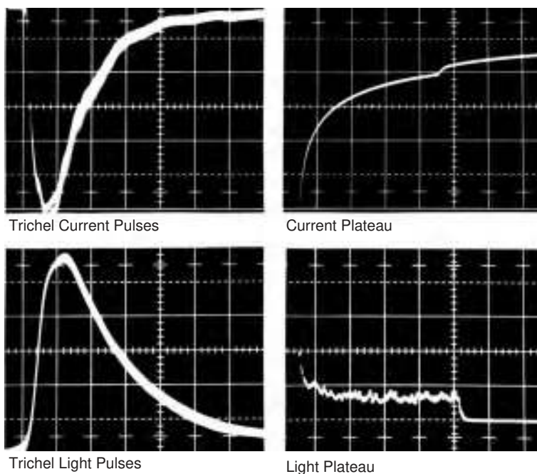
FIGURE 15.3 Current and light characteristics of Trichel streamer. Cathode: spherical protrusion ( d = 0.8 cm) on a sphere ( D = 7 cm); gap 19 cm. Scales: current 350 \mu\text{A}/\text{div.} , 50 \text{ ns}/\text{div.} (left), 50 \mu\text{A}/\text{div.} , 2 \mu\text{s}/\text{div.} (right). Light: 0.5 \text{ V}/\text{div.} , 20 \text{ ns}/\text{div.} (left), 0.2 \text{ V}/\text{div.} , 2 \mu\text{s}/\text{div.} (right). (From Trinh, N.G. and Jordan, I.B., IEEE Trans. , PAS-87, 1207, 1968; Trinh, N.G., IEEE Electr. Insul. Mag. , 11, 23, 1995a.)
