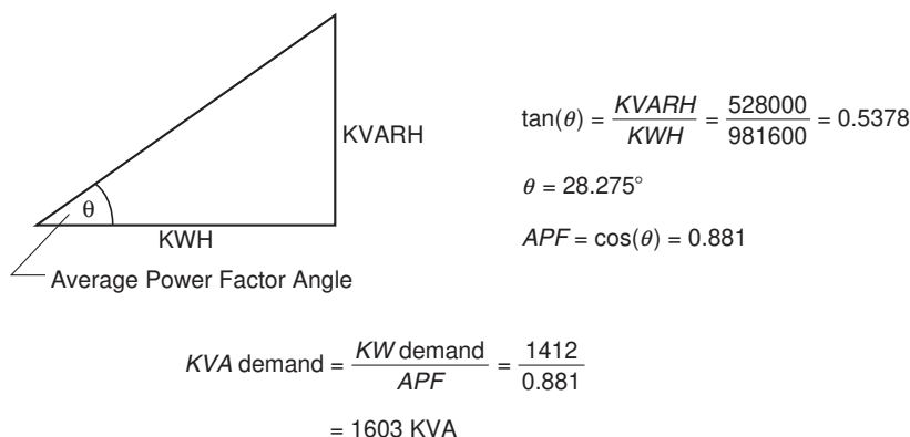
FIGURE 25.6 Calculation of kVA demand using the Average Power Factor method.
