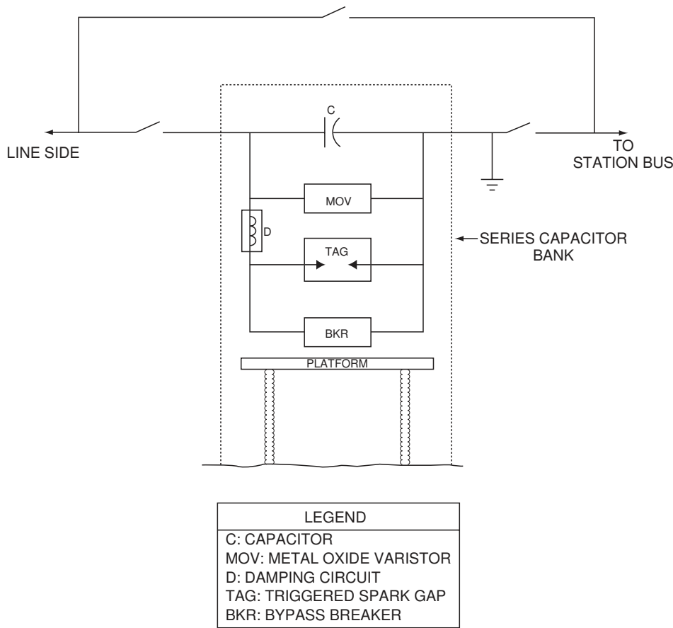
FIGURE 18.6 Schematic one-line diagram of series capacitor bank.
