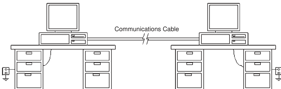
FIGURE 29.5 Circuit with a ground loop.
