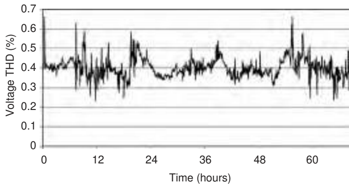
FIGURE 30.4 Example of time-varying nature of voltage THD.
