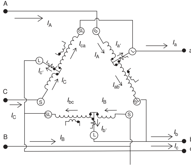
FIGURE 21.19 Delta connected type B regulators.
