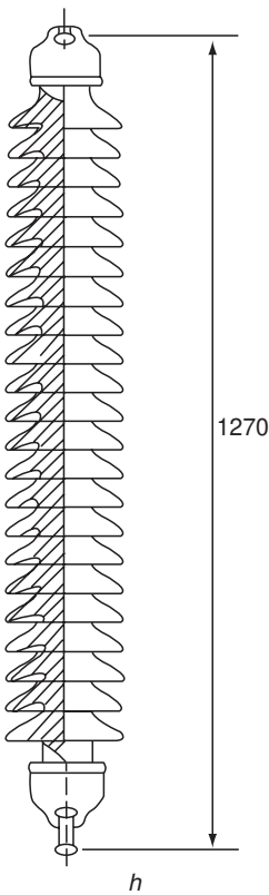
FIGURE 10.9 Long rod insulator.
