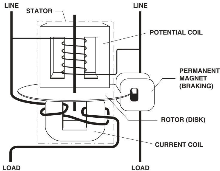
FIGURE 25.1 Main components of electromechanical meter.
