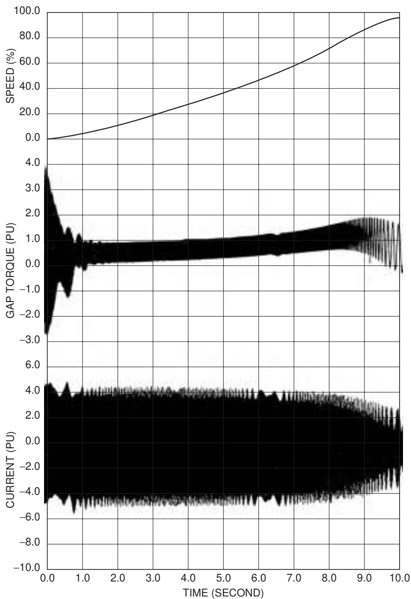
FIGURE 5.6 Synchronous motor and condensor starting.
