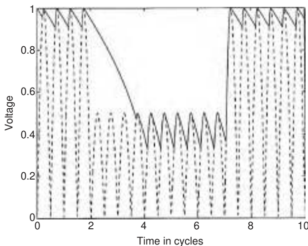
FIGURE 31.11 Absolute value of AC voltage (dashed) and DC bus voltage (solid line) for a sag down to 50%.
