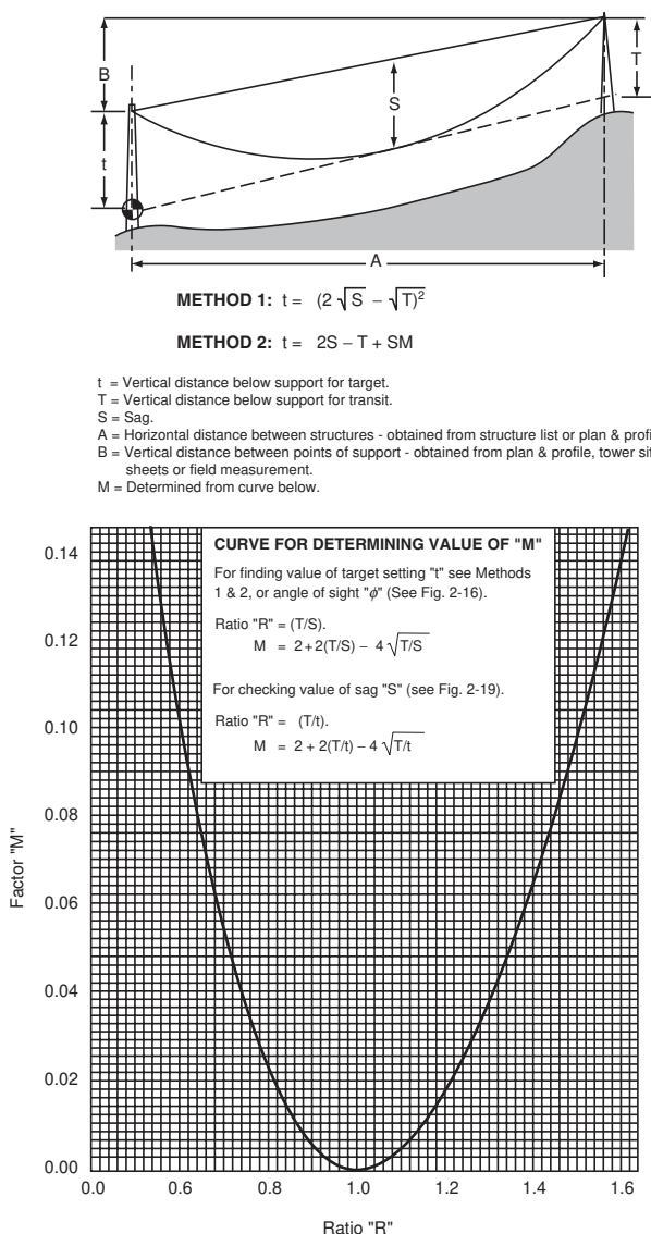
FIGURE 14.17 Conductor sagging by calculated target method.
