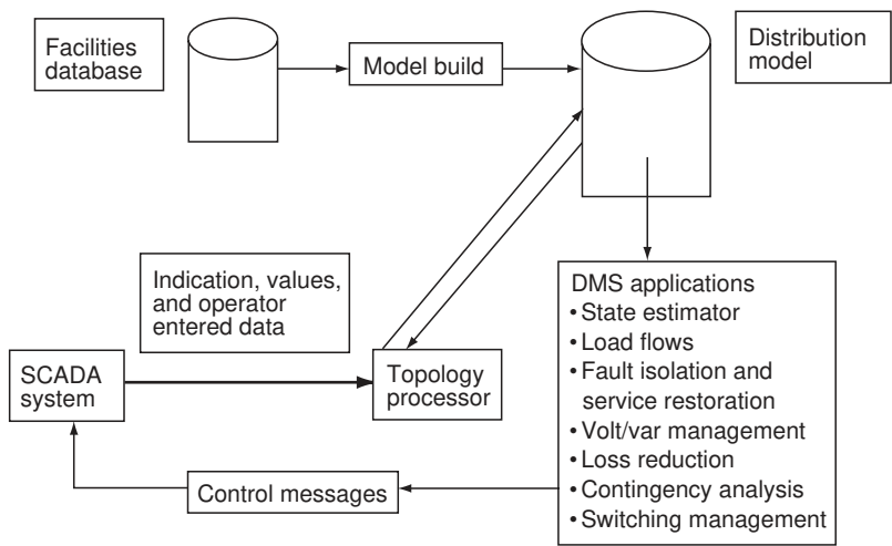
FIGURE 22.2 A DMS platform with SCADA interface.
