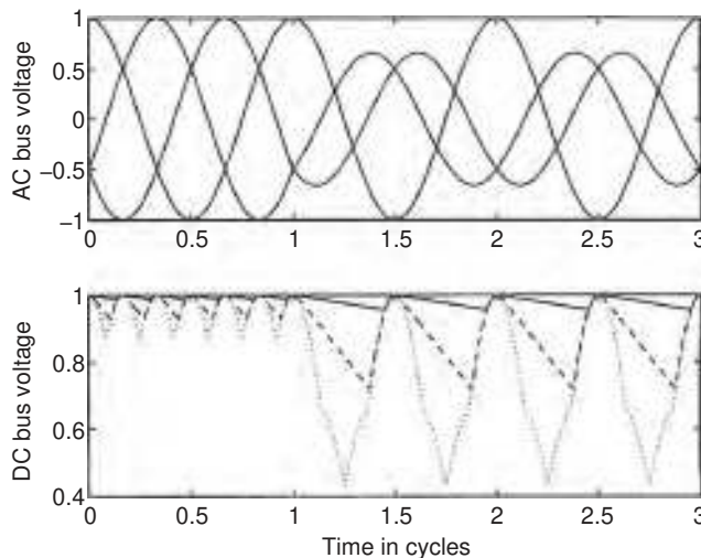
FIGURE 31.12 AC and DC side voltages for a three-phase rectifier during a sag of type C.
