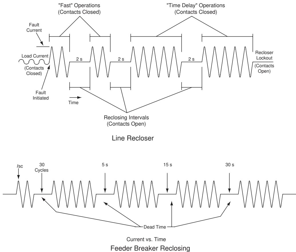
FIGURE 23.4 Reclosing sequences.
