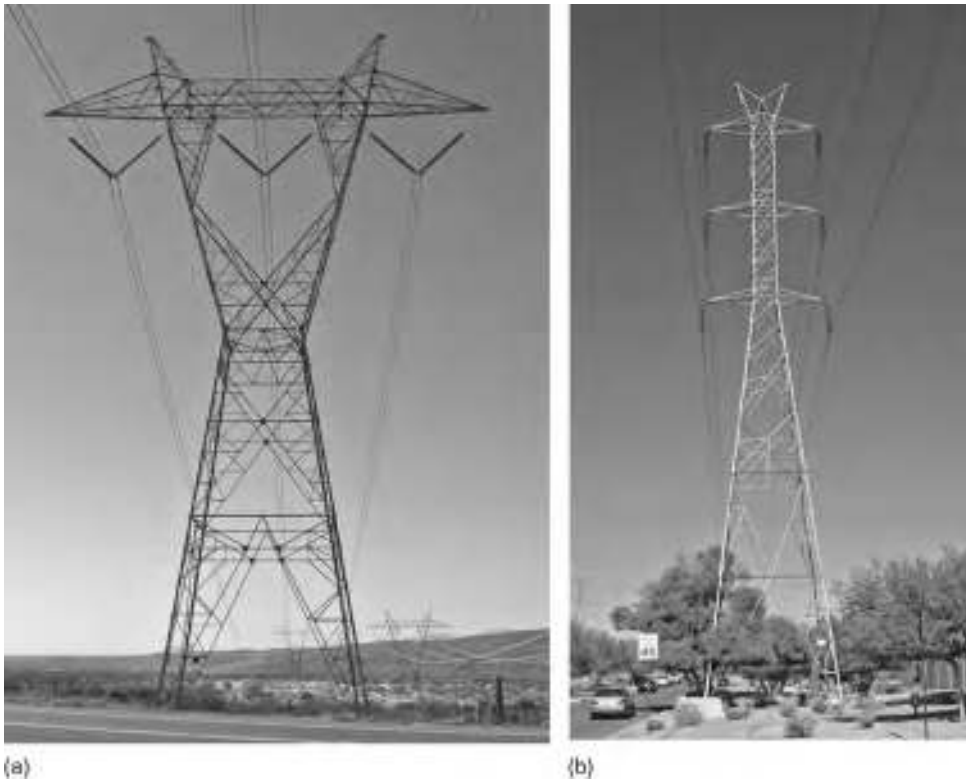
FIGURE 19.2 High-voltage transmission lines. (a) Single circuit line with horizontally arranged conductors. (b) Double circuit line with vertically arranged conductors.
