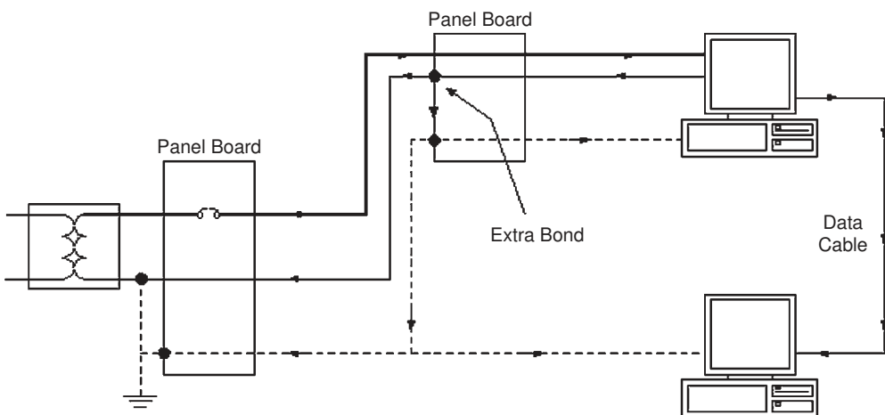
FIGURE 29.9 Neutral current flow with and extra neutral-to-ground bond.
