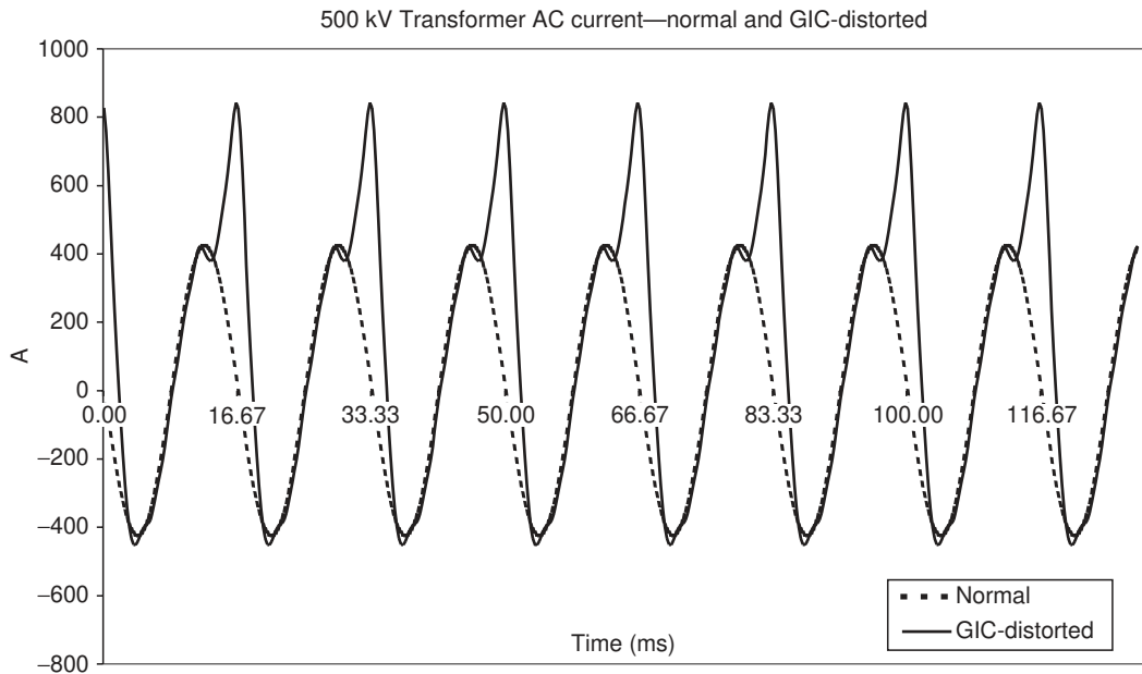
FIGURE 16.14 500 kV Simple demonstration circuit simulation results: transformer AC currents and distortion due to GIC.
