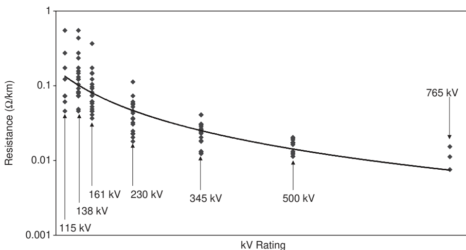
FIGURE 16.12 Range of transmission line resistance for the major kilovolt-rating classes for transmission lines in the US electric power grid infrastructure population. Also shown is a trend line of resistance weighted to average. The lower R for the higher voltage lines will also cause proportionately larger GIC flows in this portion of the power grid. (Derived from data in EHV Transmission Line Reference Book and from US Department of Energy, Energy Information Agency and FERC Form 1 Database.)
