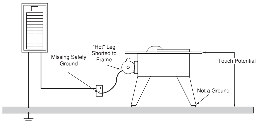
FIGURE 29.2 Illustration of a dangerous touch potential situation.
