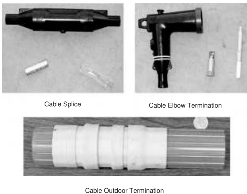
FIGURE 12.5 Cable accessories.
