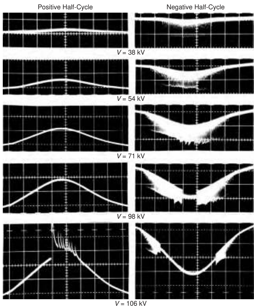
FIGURE 15.7 Corona modes under AC voltage. Electrode: conical protrusion ( \theta = 30^\circ ) on a sphere ( D = 7 cm); gap 25 cm; R = 10 k \Omega . Scales: 50 \mu A/div., 1.0 ms/div. (From Trinh, N.G. and Jordan, I.B., IEEE Trans. , PAS-87, 1207, 1968; Trinh, N.G., IEEE Electr. Insul. Mag. , 11, 23, 1995a.)
