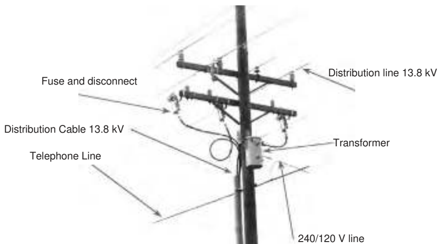
FIGURE 8.13 Service drop.
