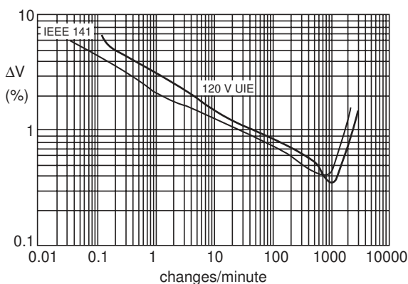
FIGURE 32.7 Threshold of irritation flicker curve and P_{st} = 1.0 curve from a flicker meter.
