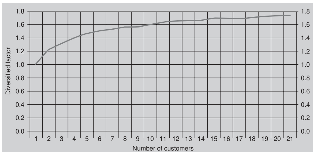
FIGURE 24.8 Diversity factor curve for residential class for weekdays during February at normal weather conditions.
