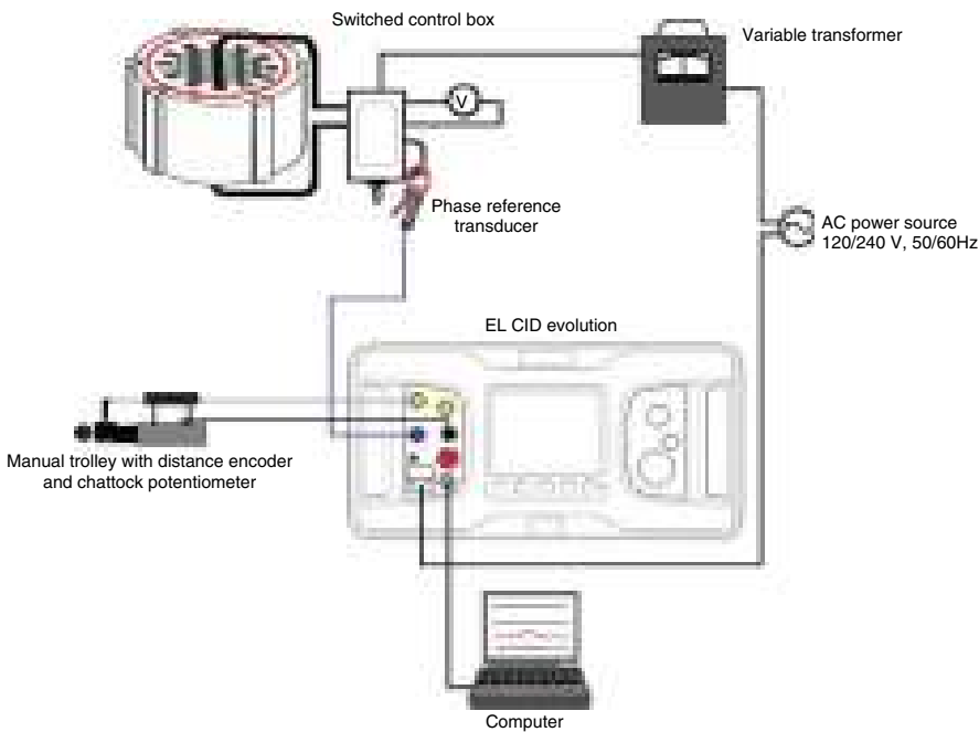
Figure 17.14 Setup of EL-CID test on a stator core with a simulated plot on the computer of slot milliampere versus distance along core showing a lamination insulation defect. (Source: Courtesy of Iris Power-Qualitrol.)
