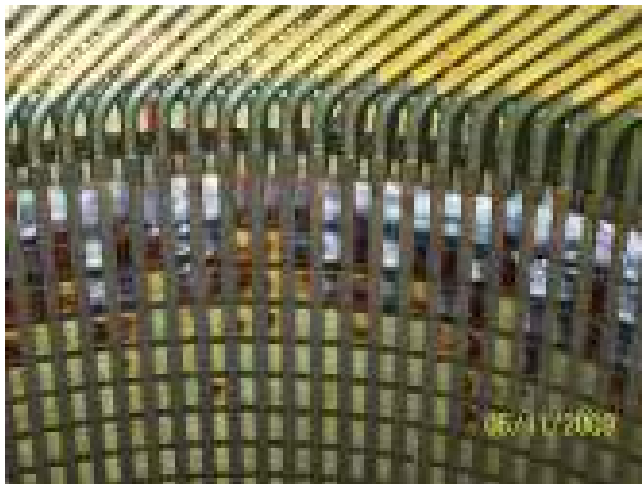
Figure 13.2 Stator core burning that resulted from excessive oven temperatures during stator winding burnout prior to rewind.
