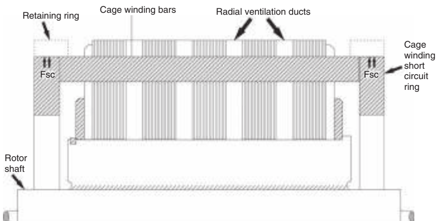
Figure 12.1 Different mechanical forces that occur in an SCI rotor.
