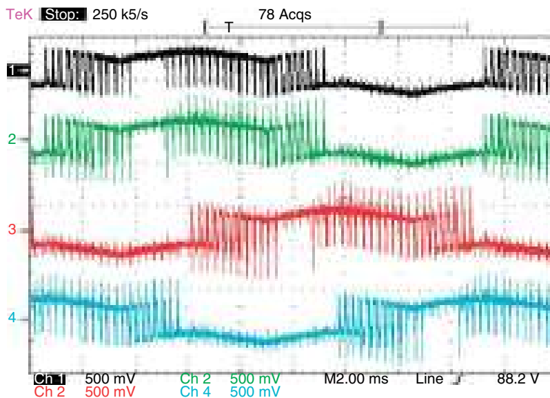
Figure 8.15 Digital oscilloscope image of the voltage waveform measured at Phase A at the inverter (top trace) and the voltage on three phases at the stator winding (lower three traces). The motor was rated 440 V. The horizontal time base is 2 ms/division and the vertical scale 1000 V/division.
