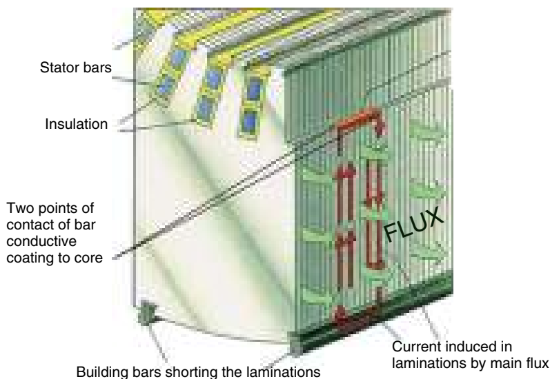
Figure 8.11 Sketch of the current loop formed by the flow of current through the core lamination, the building (or key) bars and the slot conductive coating on a stator bar.
