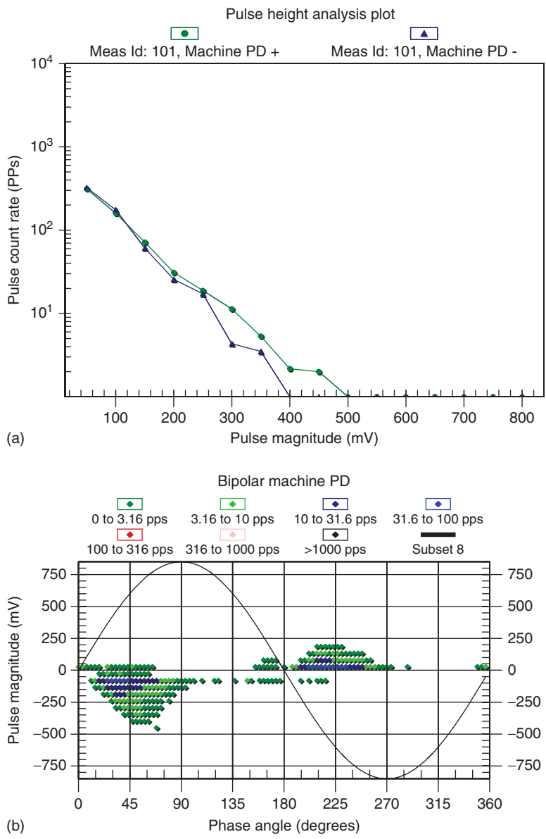
Figure 16.6 (a) Pulse magnitude and (b) pulse phase analysis plots from online PD detection. (Source: Iris Power-Qualitrol.)
